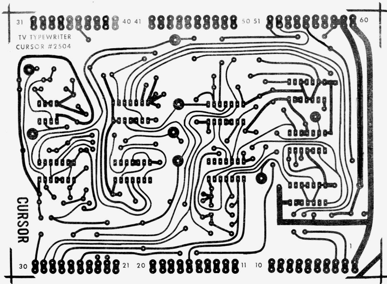
FIG. 16 -- FULL SIZE FOIL PATTERN for cursor board.
