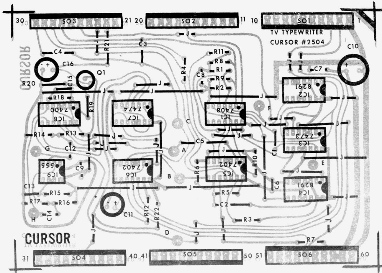
FIG. 17 -- PARTS PLACEMENT on cursor
