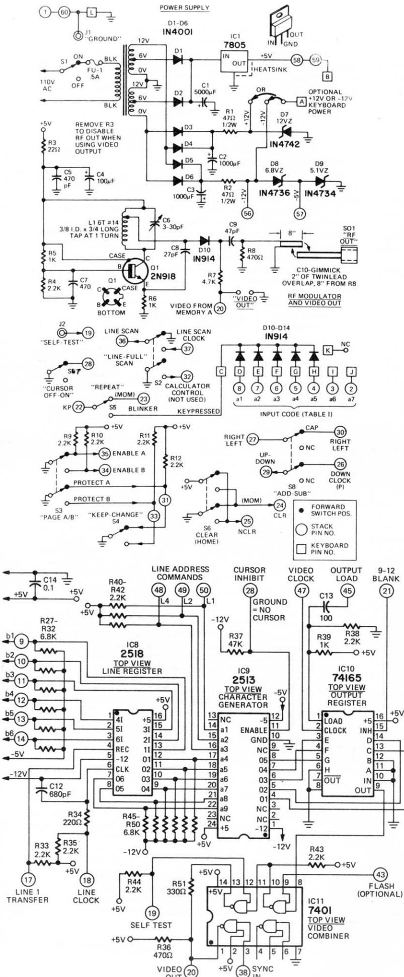
ABOVE FIG. 4 -- PAGE "A" OR PAGE "B" memory circuitry.
