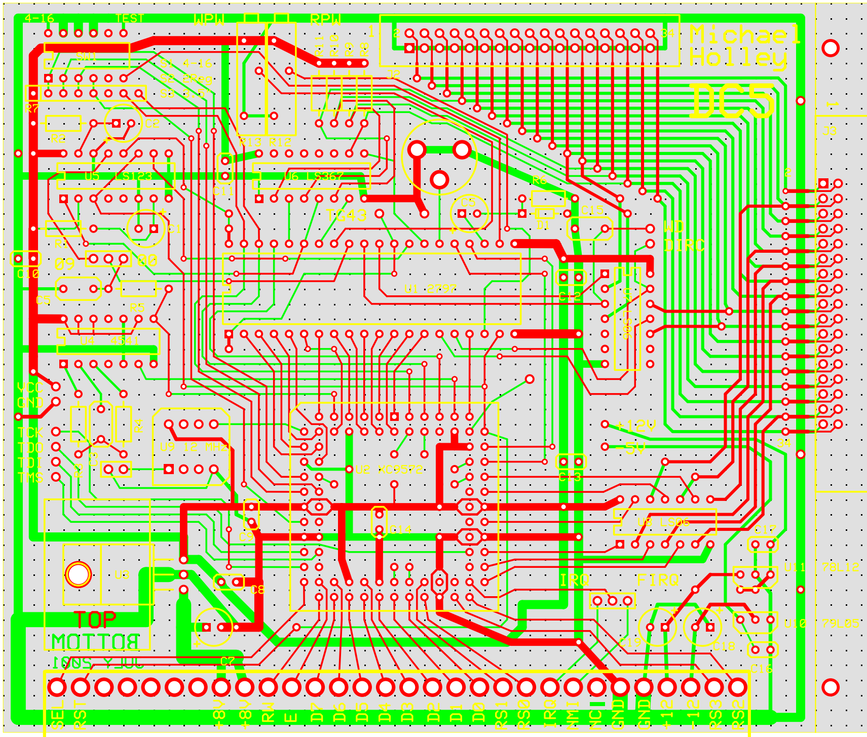
C:\Program Files\ExpressPCB\FDC2a.pcb (Silkscreen, Top layer, Bottom layer)
