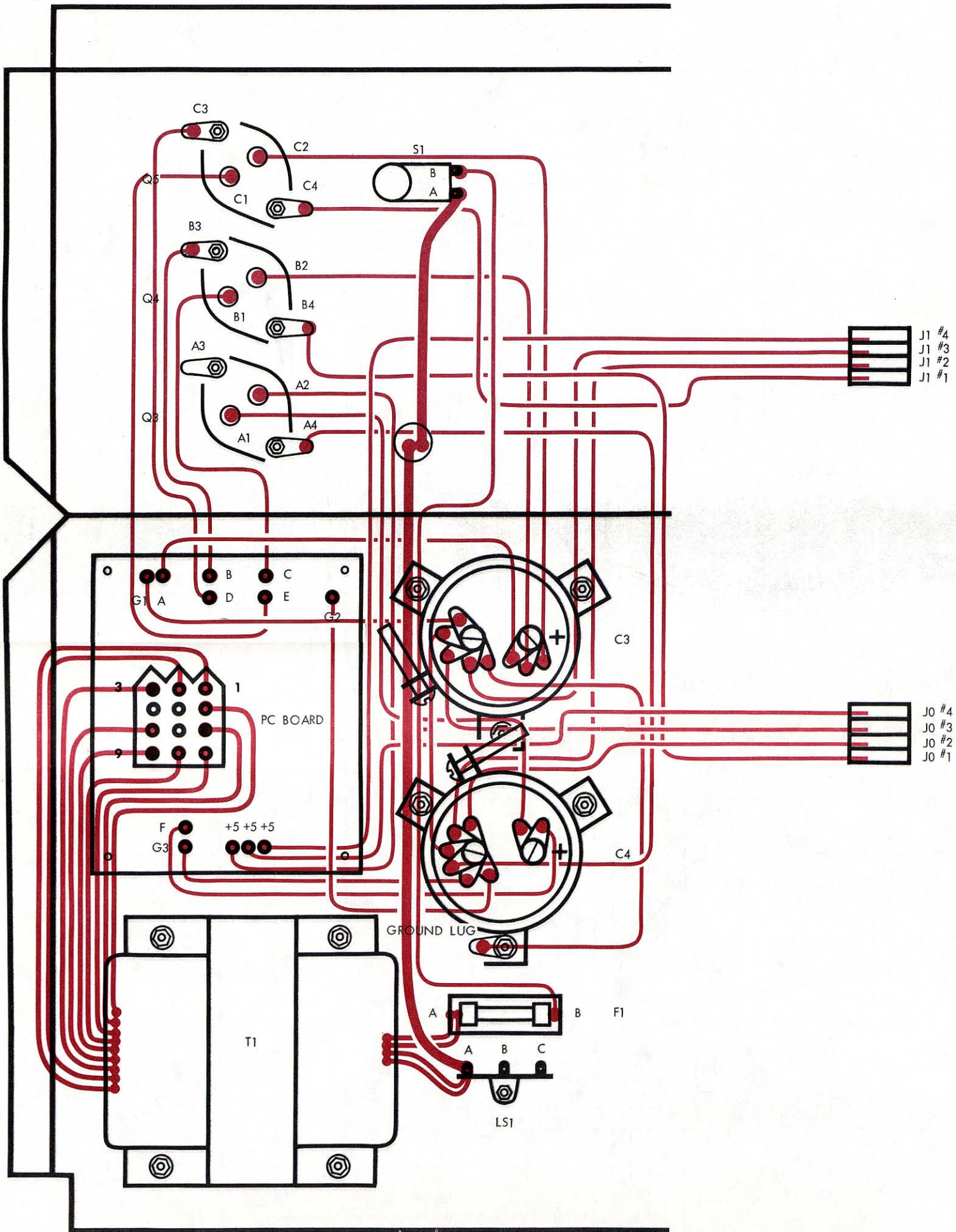
MF-68 MINIFLOPPY DISK SYSTEM WIRING PICTORIAL
