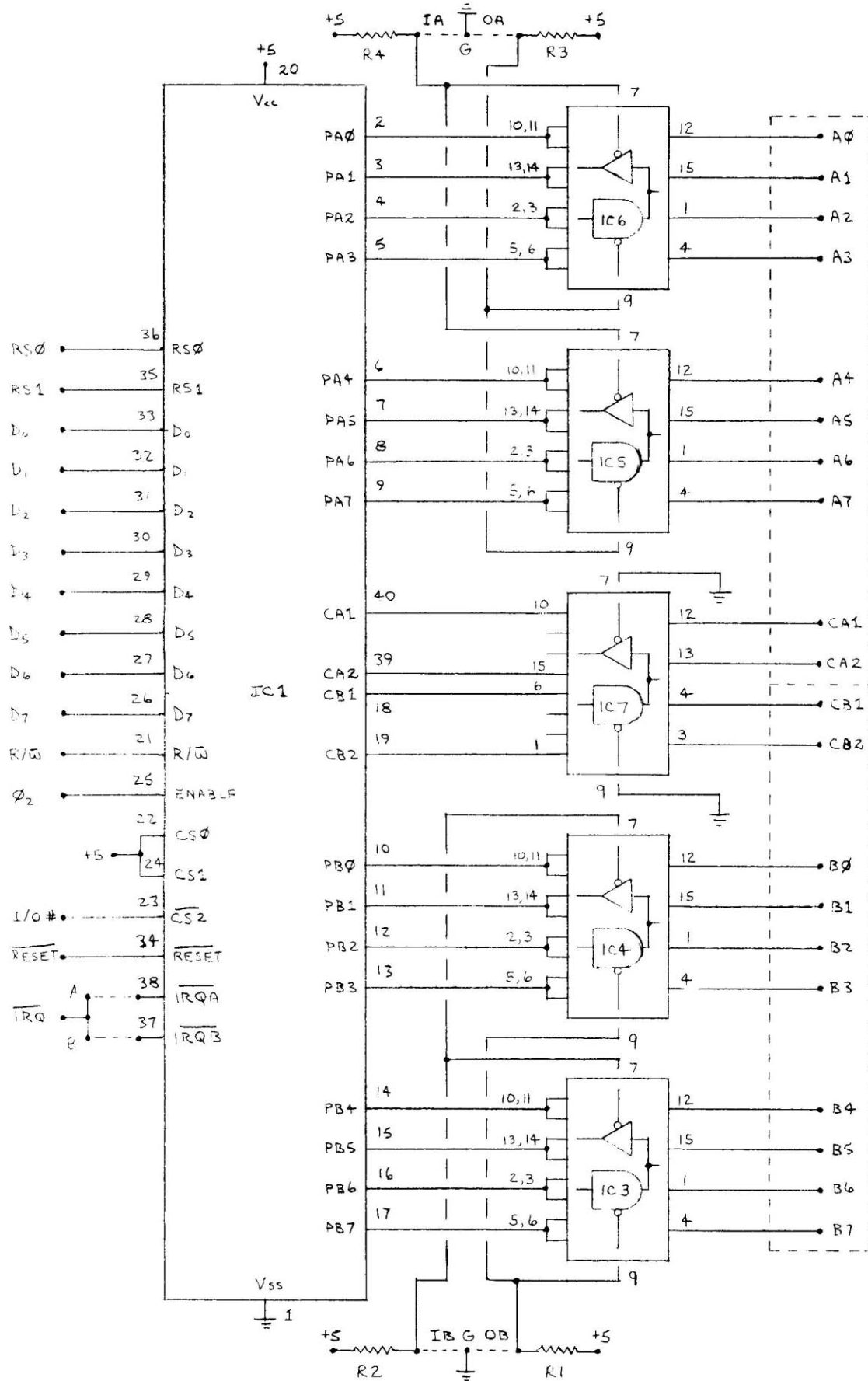
Schematic MP-LA Parallel Interface Option
