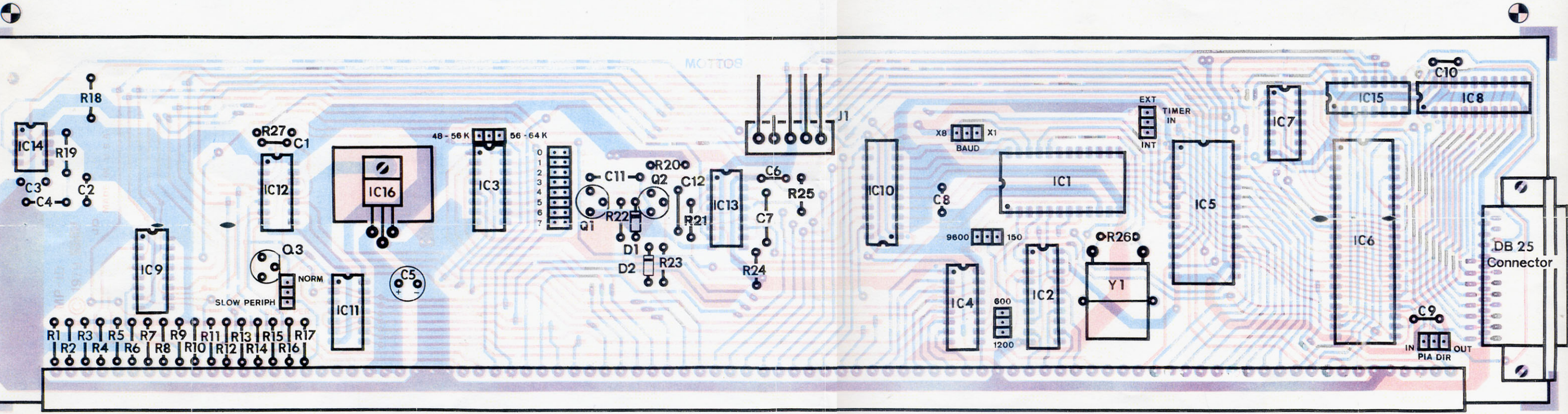
INTERFACE DRIVER BOARD MP-ID
