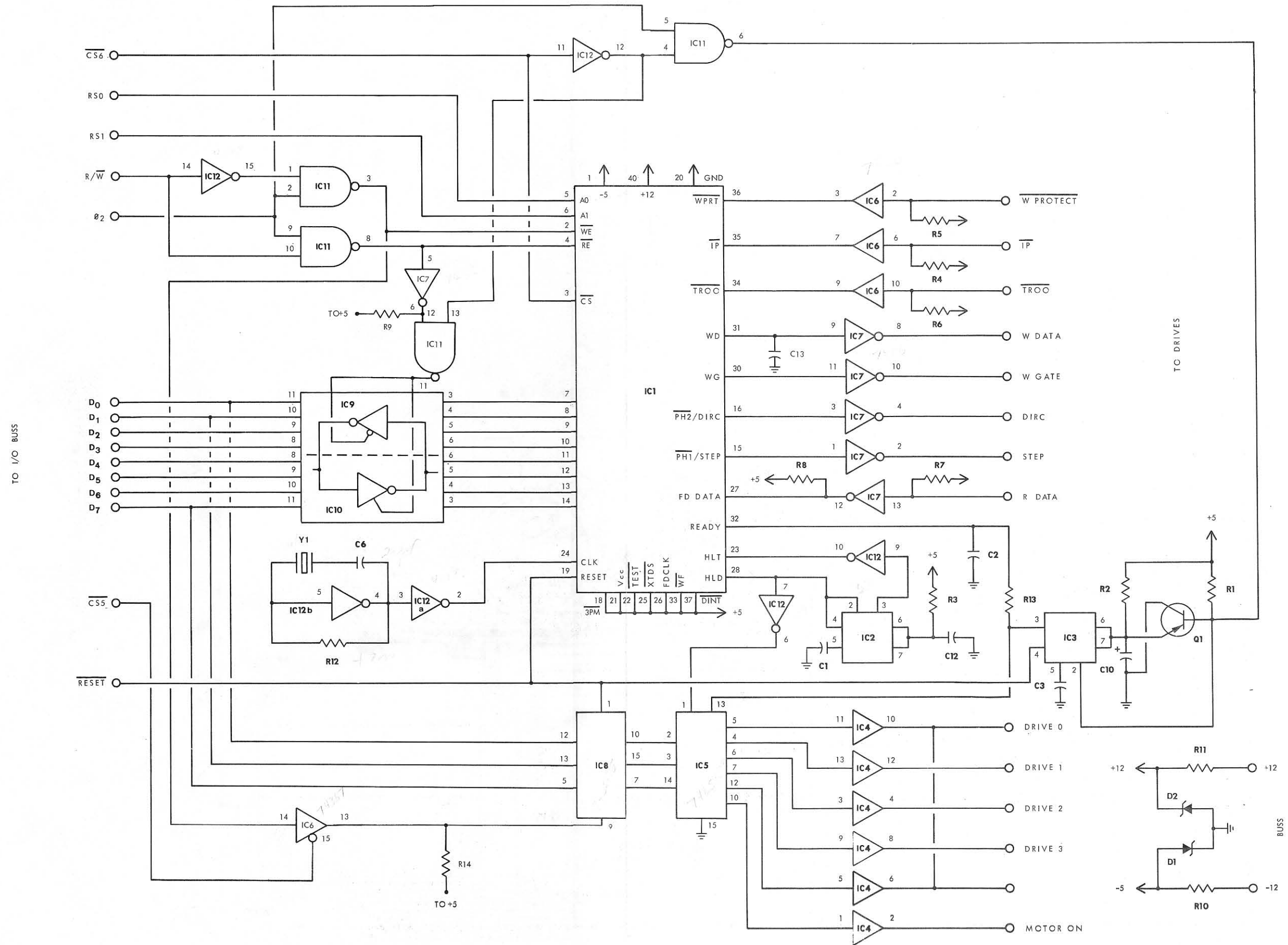
Schematic - DC-2 Minifloppy Disk Controller
