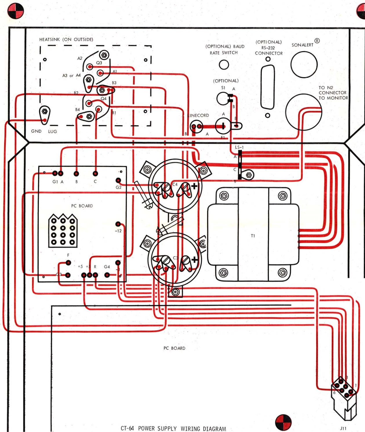
CT-64 POWER SUPPLY WIRING DIAGRAM
