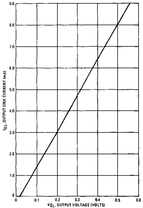
OUTPUT SINK CURRENT versus OUTPUT VOLTAGE
