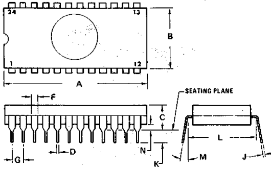
FRIT SEAL PACKAGE CASE 623A-03
