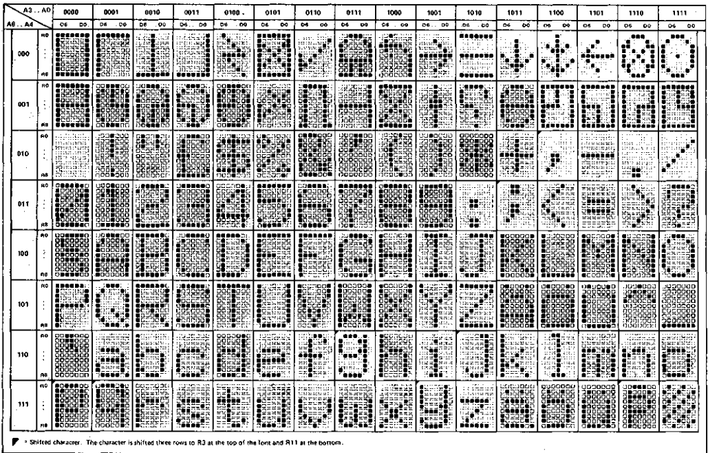
FIGURE 15 - MCM66770 PATTERN
