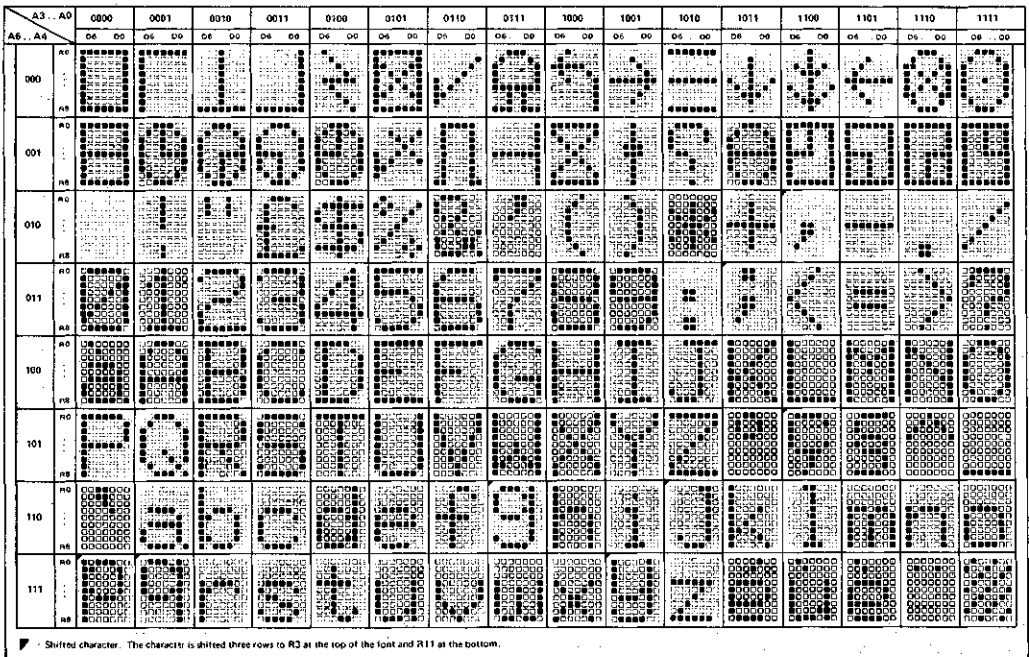
FIGURE 16 - MCM66780 PATTERN
