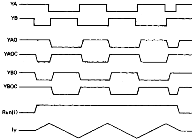
FIGURE 3 — TYPICAL COIL WAVEFORMS (X-COIL IDENTICAL, PHASE SHIFTED) (1) ASSUMING X-COIL ALREADY BEING DRIVEN
