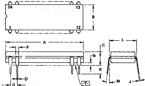
CERAMIC PACKAGE CASE 748-01
