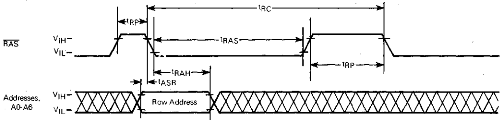
READ-WRITE/READ-MODIFY-WRITE CYCLE
