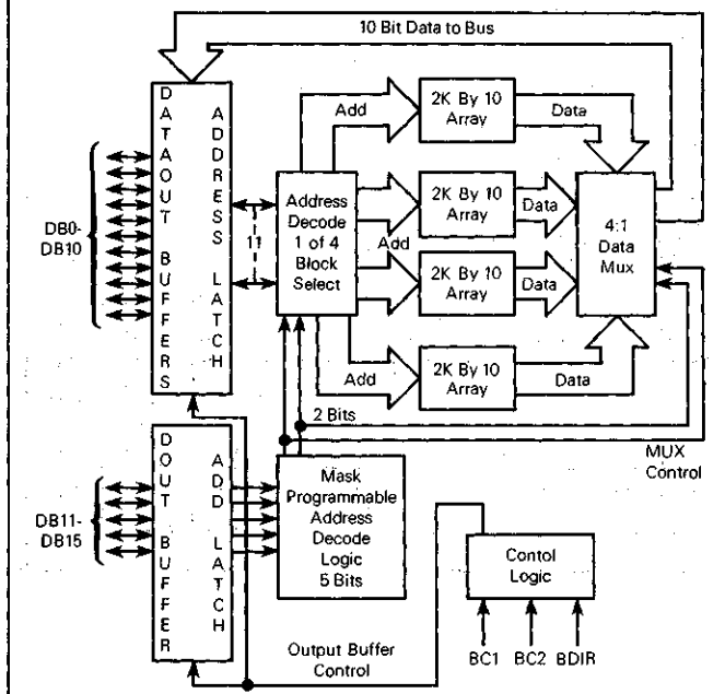
BLOCK DIAGRAM 80K - ROM
