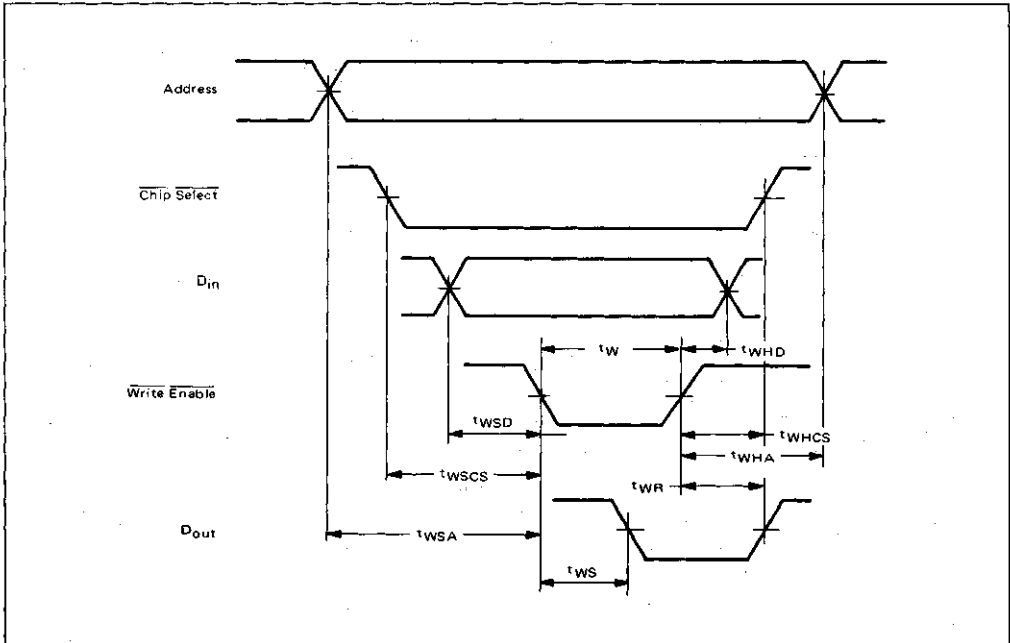
FIGURE 4 – WRITE MODE
