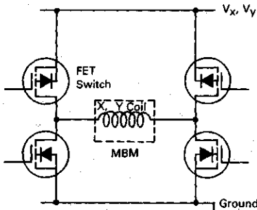
(a.) TYPICAL DRIVE CIRCUIT
