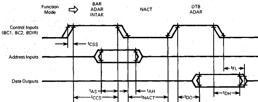
TIMING WAVEFORMS
