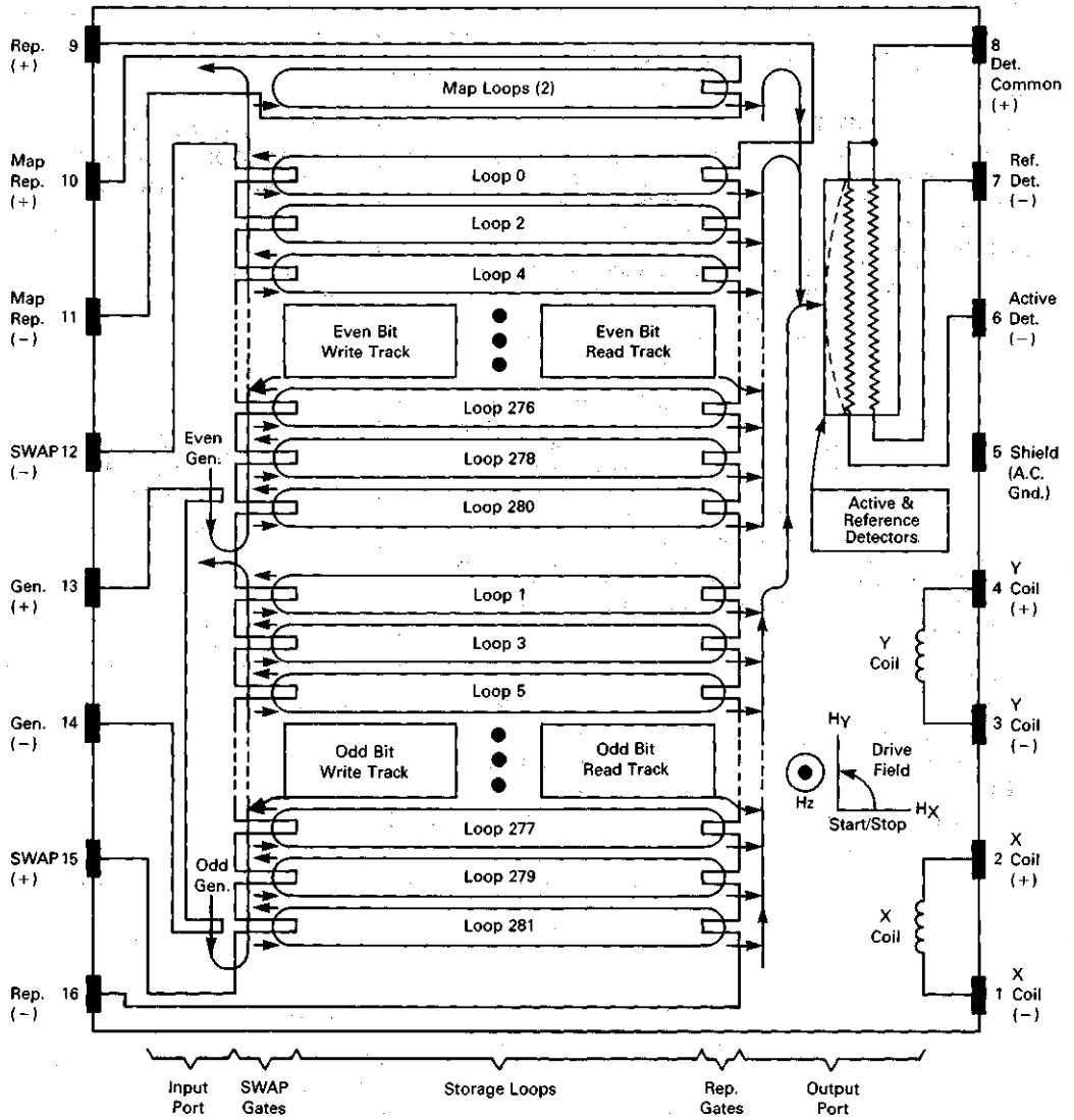
FIGURE 1 — BLOCK DIAGRAM
