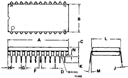
PLASTIC PACKAGE CASE 709-02
