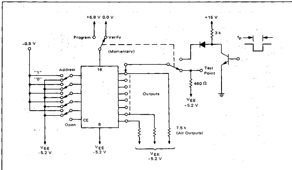
FIGURE 4 – MANUAL PROGRAMMING CIRCUIT
