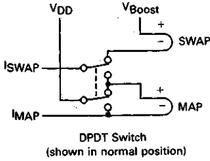
FIGURE 6 — MAP WRITE SWITCH
