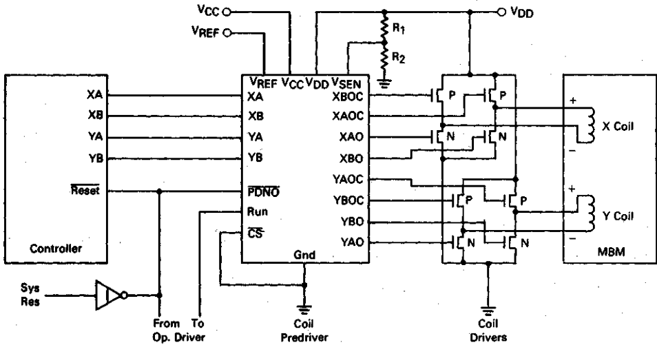
FIGURE 4 — TYPICAL APPLICATION
