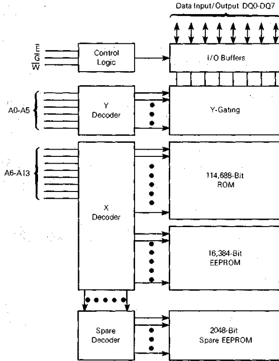
FIGURE 1 — MCM6836E16E EPROM MEMORY UNIT BLOCK DIAGRAM
