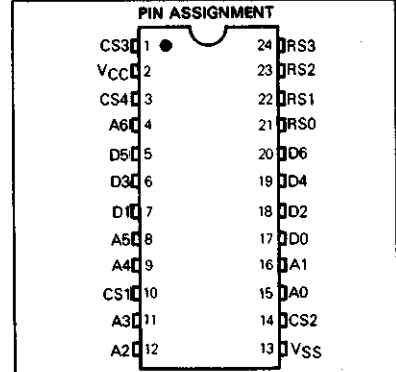
P SUFFIX PLASTIC PACKAGE CASE 709-02
