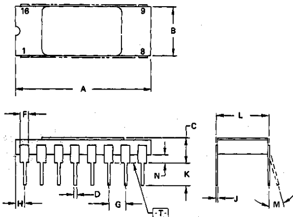
CERAMIC PACKAGE CASE 690-13
