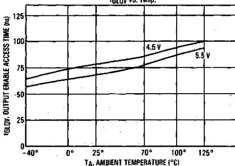
FIGURE 4 — OUTPUT ENABLE ACCESS VERSUS TEMPERATURE
