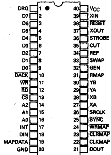
FIGURE 1 — PIN ASSIGNMENTS
