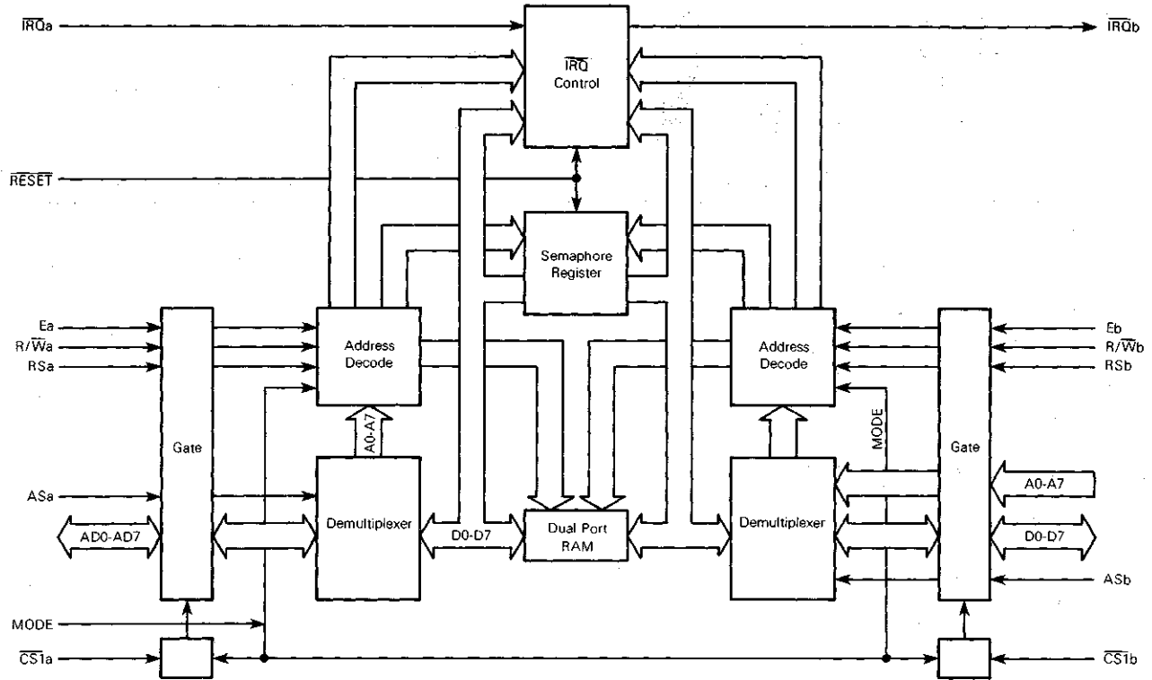
FIGURE 1 - BLOCK DIAGRAM
