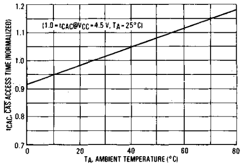
FIGURE 5 — \overline{\text{CAS}} ACCESS TIME versus AMBIENT TEMPERATURE
