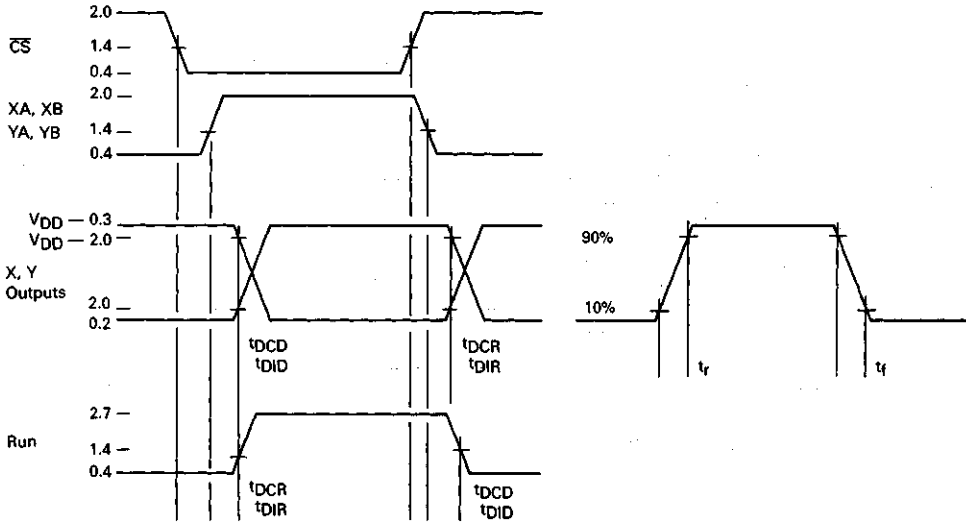
FIGURE 2 — SIGNAL WAVEFORMS
