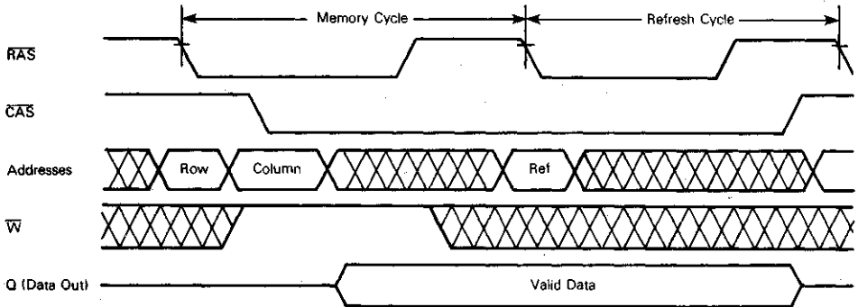
HIDDEN RAS-ONLY REFRESH CYCLE
