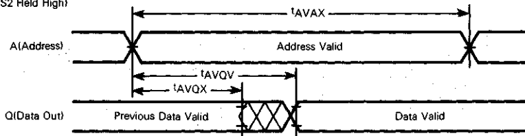
Read Cycle Timing 1 (S1, S2 Held High)
