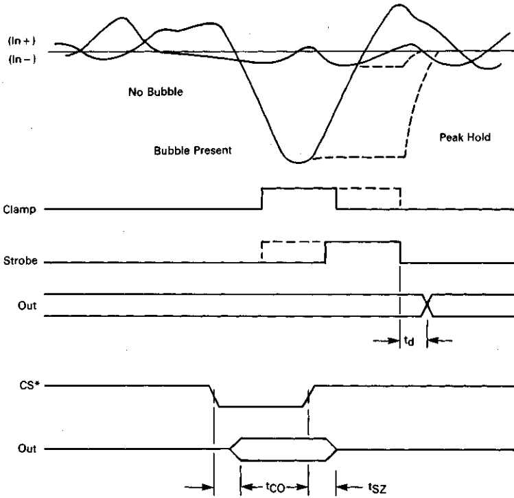
FIGURE 3 — TYPICAL APPLICATION
