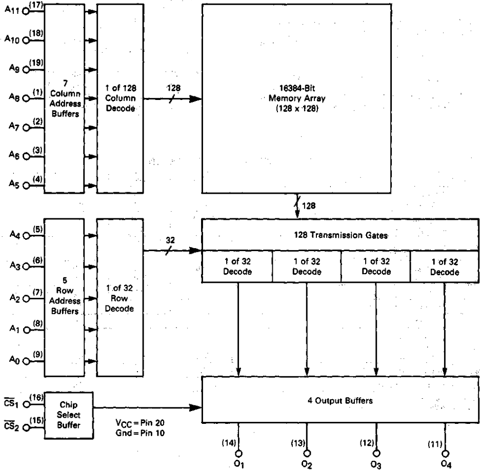
MCM76165/165A BLOCK DIAGRAM
