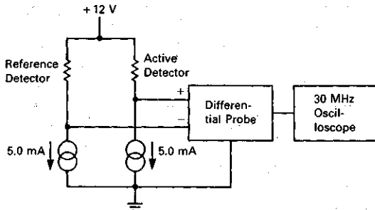
(b) MEASUREMENT SETUP
