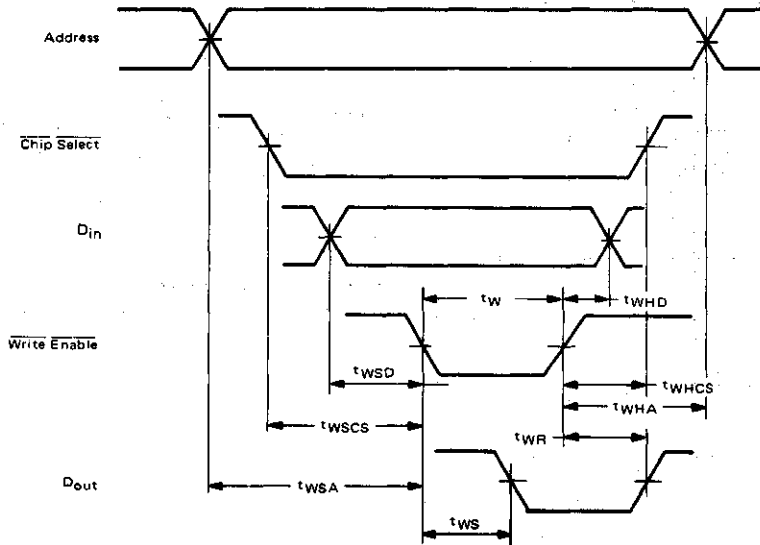
FIGURE 4 – WRITE MODE
