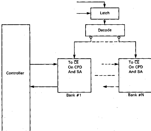
FIGURE 3c — MULTIPLE-BANK SYSTEM
