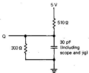
FIGURE 1 -- DC OUTPUT LOAD
