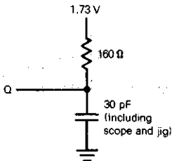
FIGURE 1 — DC OUTPUT LOAD
