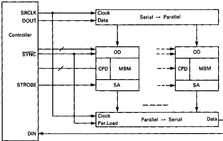
FIGURE 3b — MULTIPLE-MBM SYSTEM
