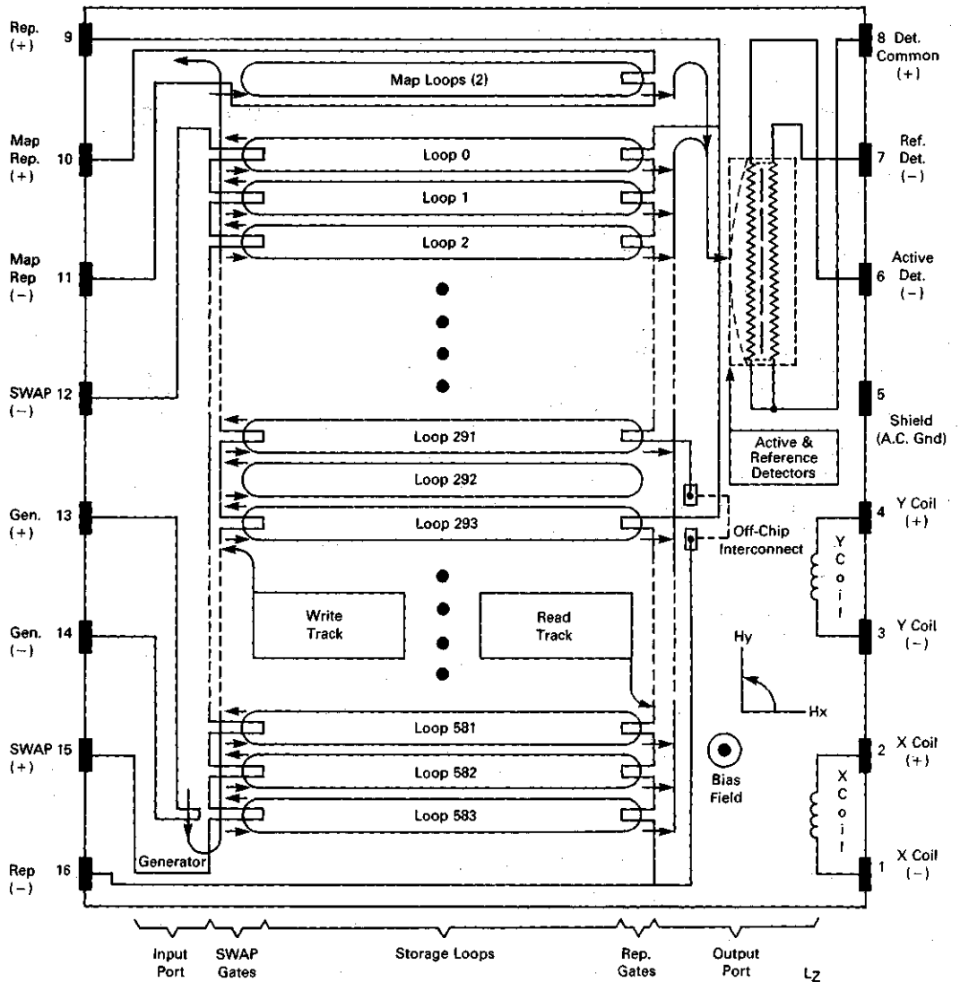
FIGURE 1 — BLOCK DIAGRAM
