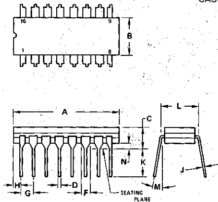
CERAMIC PACKAGE CASE 620-08
