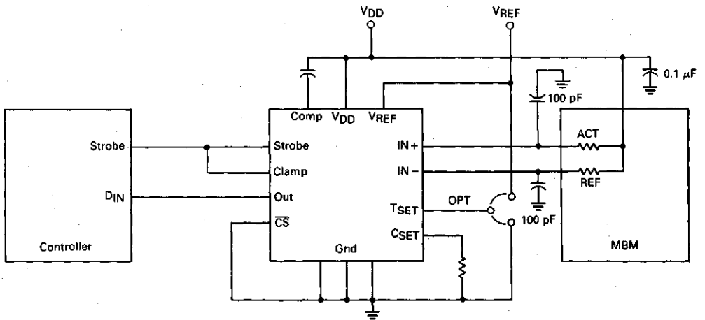
FIGURE 3 — TYPICAL APPLICATION
