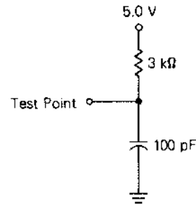
Load B ( \overline{IRQ} Only)
