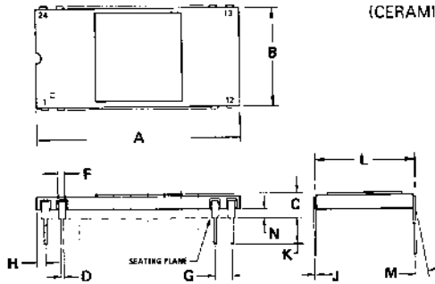
CASE 716-06 (CERAMIC)
