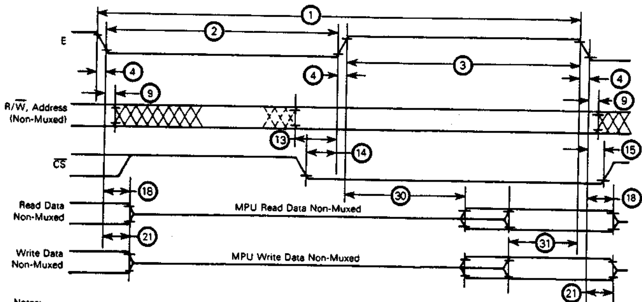
FIGURE 1 - BUS TIMING
