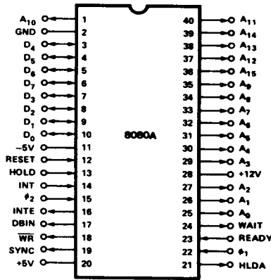
Figure 2. Pin Configuration
