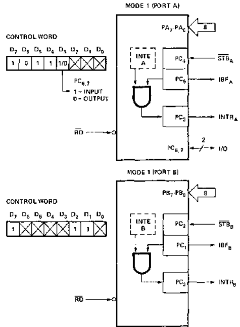
Figure 6. MODE 1 Input
