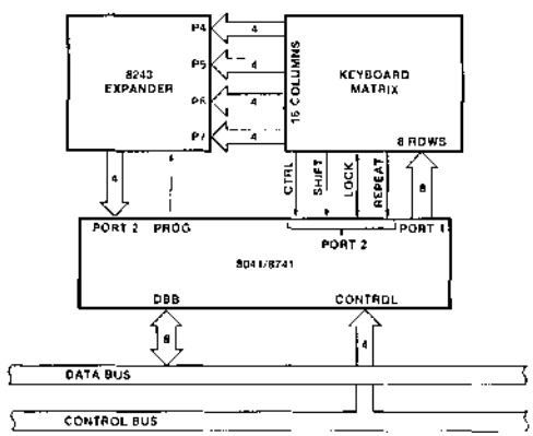
Figure 2. 8041-8243 Keyboard Scanner
