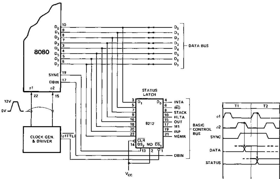
Figure 8. 8080 Status Latch
