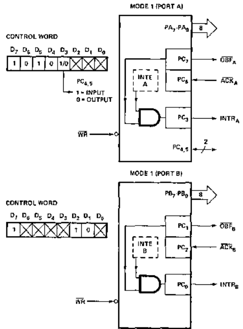
Figure 8. MODE 1 Output
