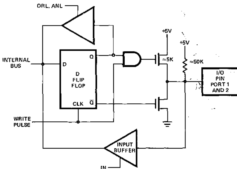
"QUASI BI DIRECTIONAL" PORT STRUCTURE
