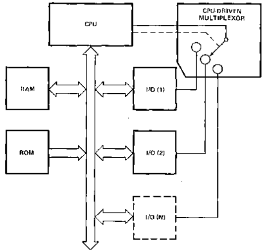
Figure 1. Polled Method
