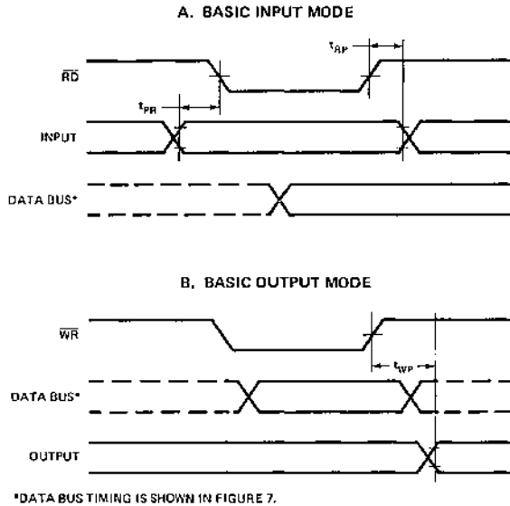
FIGURE 9. BASIC I/O TIMING WAVEFORM.
