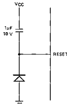
FIGURE 7. POWER ON RESET
