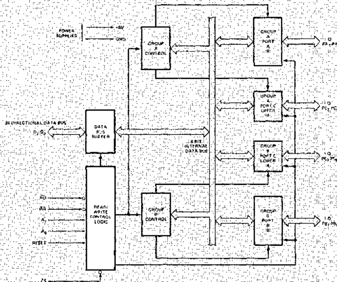
Figure 1. 8255A Block Diagram Showing Data Bus Buffer and Read/Write Control Logic Functions
