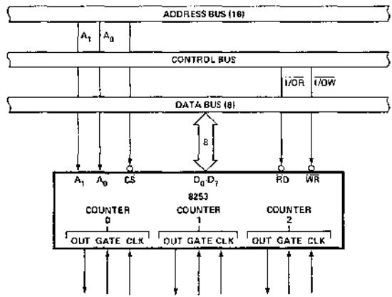
Figure 3. 8253 System Interface
