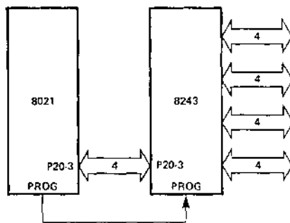
FIGURE 5. I/O EXPANDER INTERFACE
