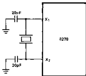
1-6 MHz CRYSTAL
