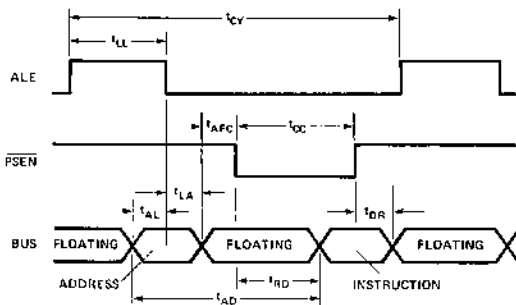
Instruction Fetch From External Program Memory
