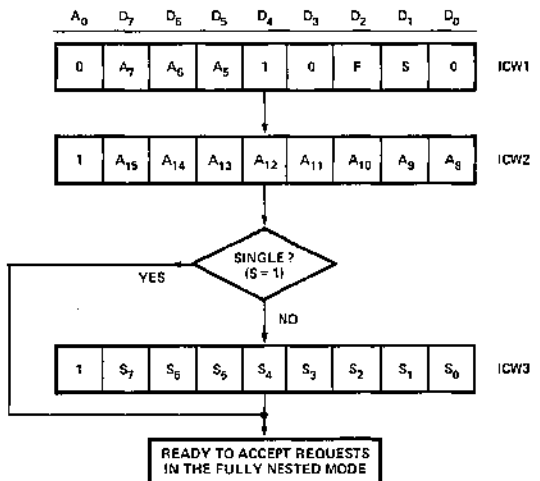
Figure 8. Initialization Sequence
