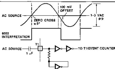
ZERO-CROSS DETECTION
