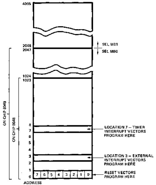
MCS-48™ PROGRAM MEMORY MAP
