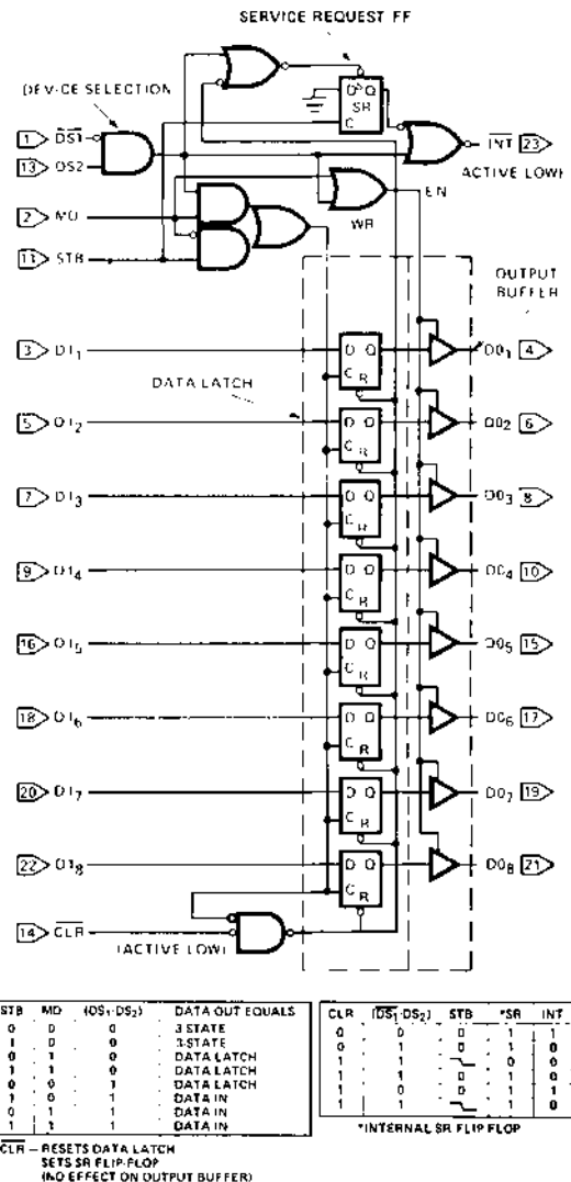
Figure 1. Service Flip-Flop Function
