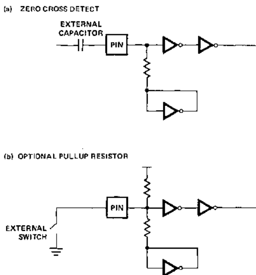
FIGURE 4. TEST 1 PIN
