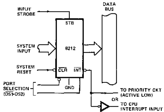
Figure 5. Interrupting Input Port
