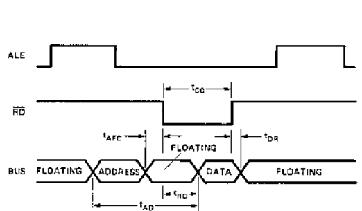
Read From External Data Memory
