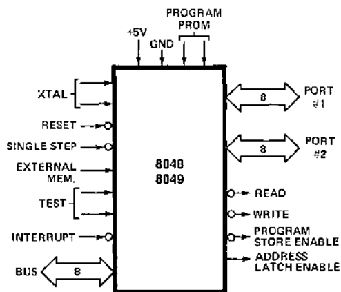
8048 LOGIC SYMBOL
