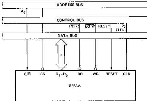
Figure 4. 8251A Interface to 8080 Standard System Bus
