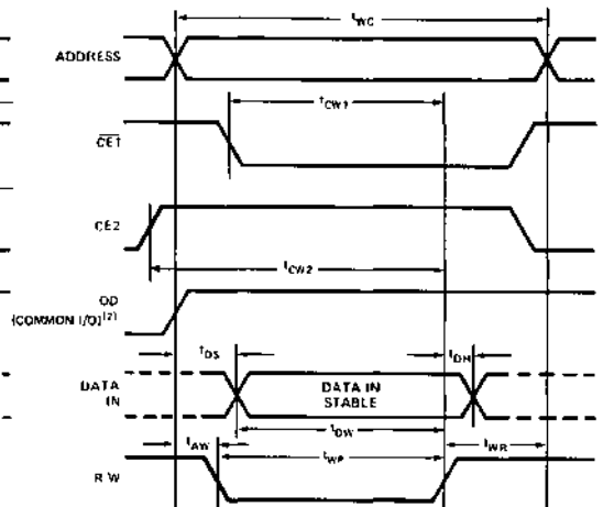
WRITE CYCLE
