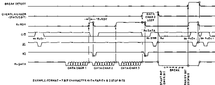
EXAMPLE FORMAT - 7 BIT CHARACTER WITH PARITY & 2 STOP BITS
