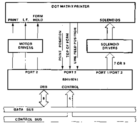
Figure 3. 8041 Matrix Printer Interface
