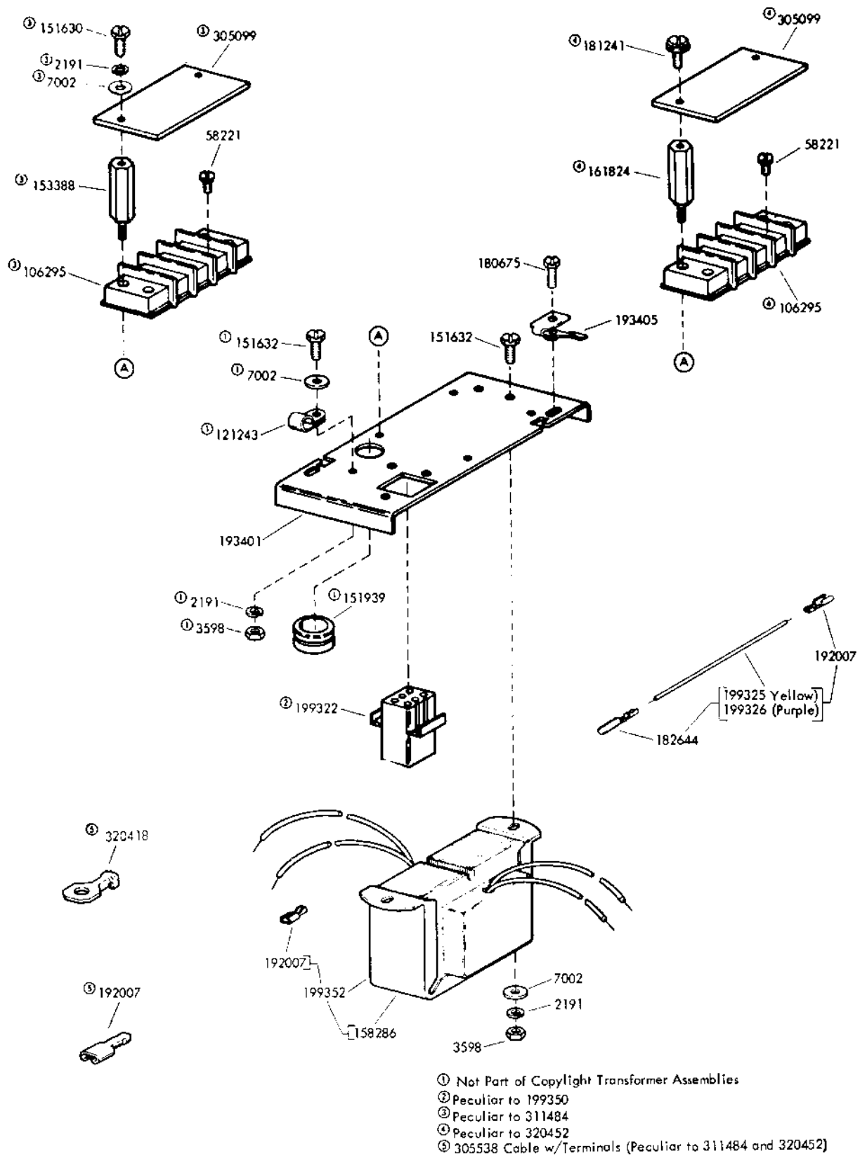
FIGURE 15. 199350, 311484 and 320452 COPYLIGT TRANSFORMER ASSEMBLIES
