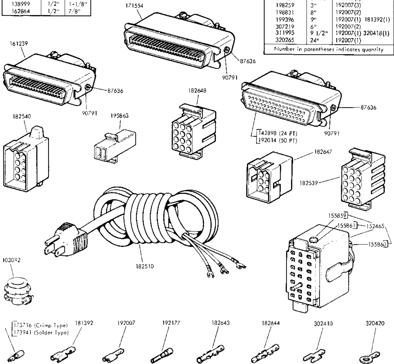
FIGURE 26. CABLE COMPONENTS
