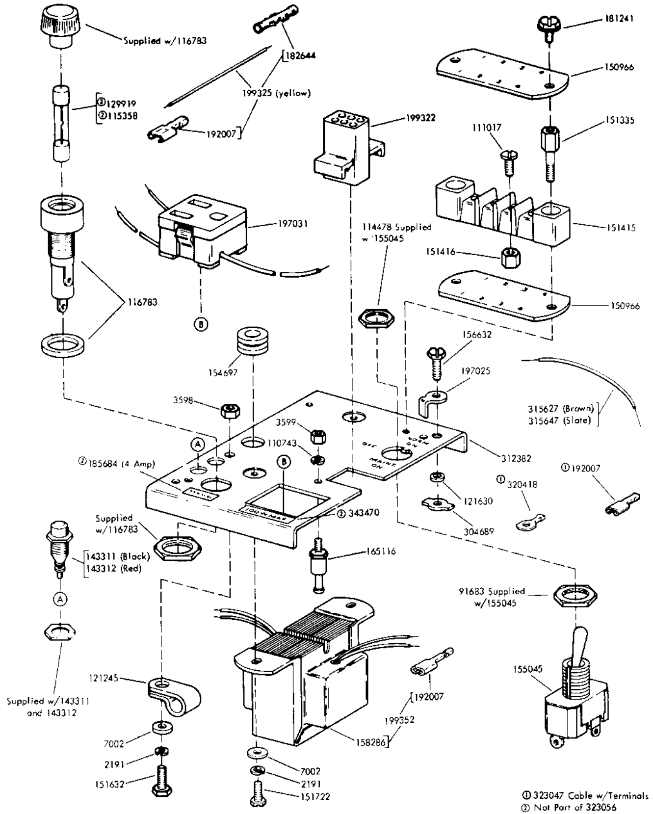
FIGURE 10. 323056 POWER DISTRIBUTION ASSEMBLY
