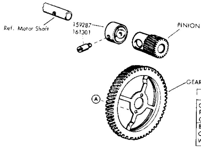
FIGURE 3. GEARSETS
