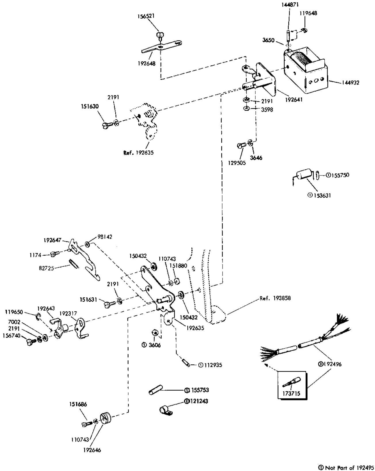
FIGURE 26. 192495 FORM-OUT SOLENOID ASSEMBLY
