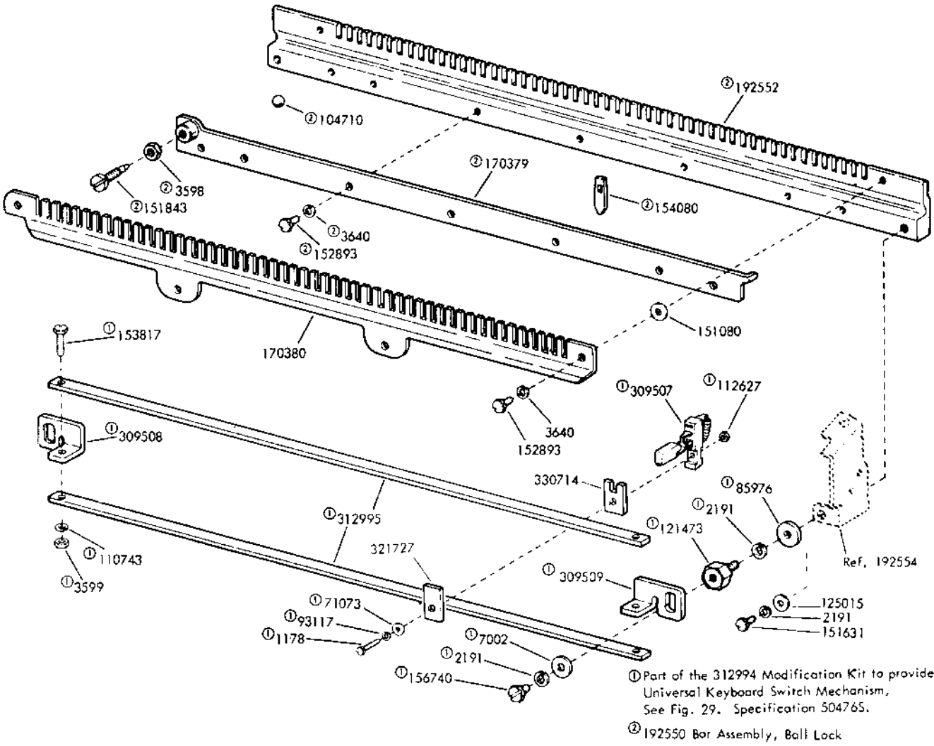
FIGURE 13. 170332 UNIVERSAL BAIL ASSEMBLY
