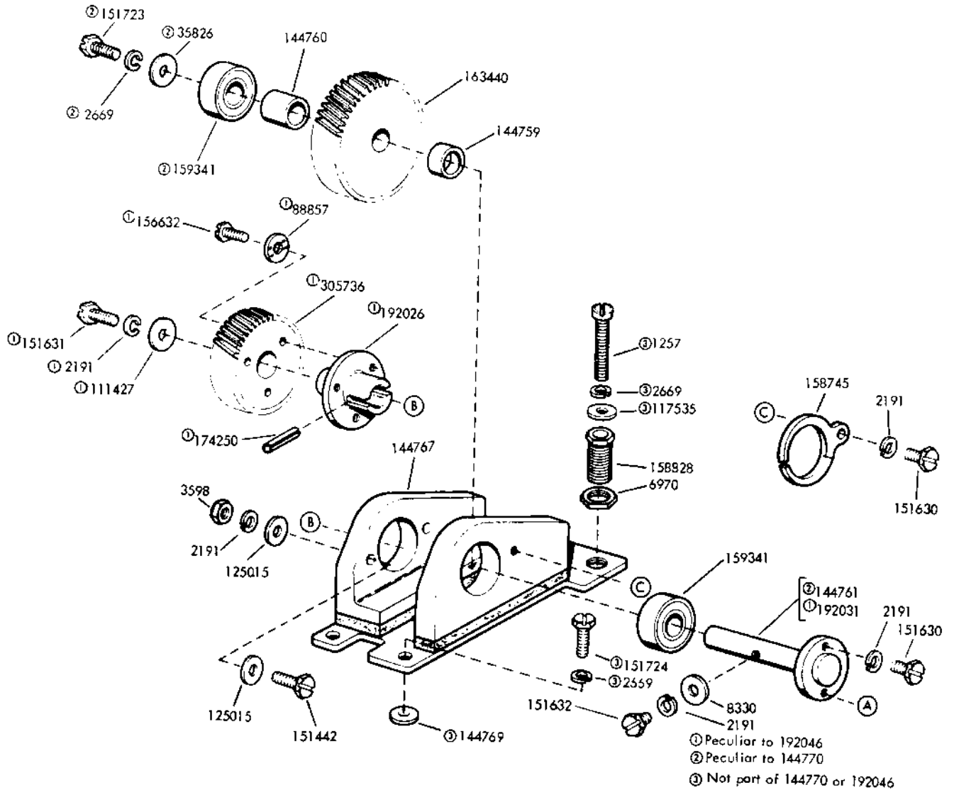
FIGURE 3. GEARSETS
