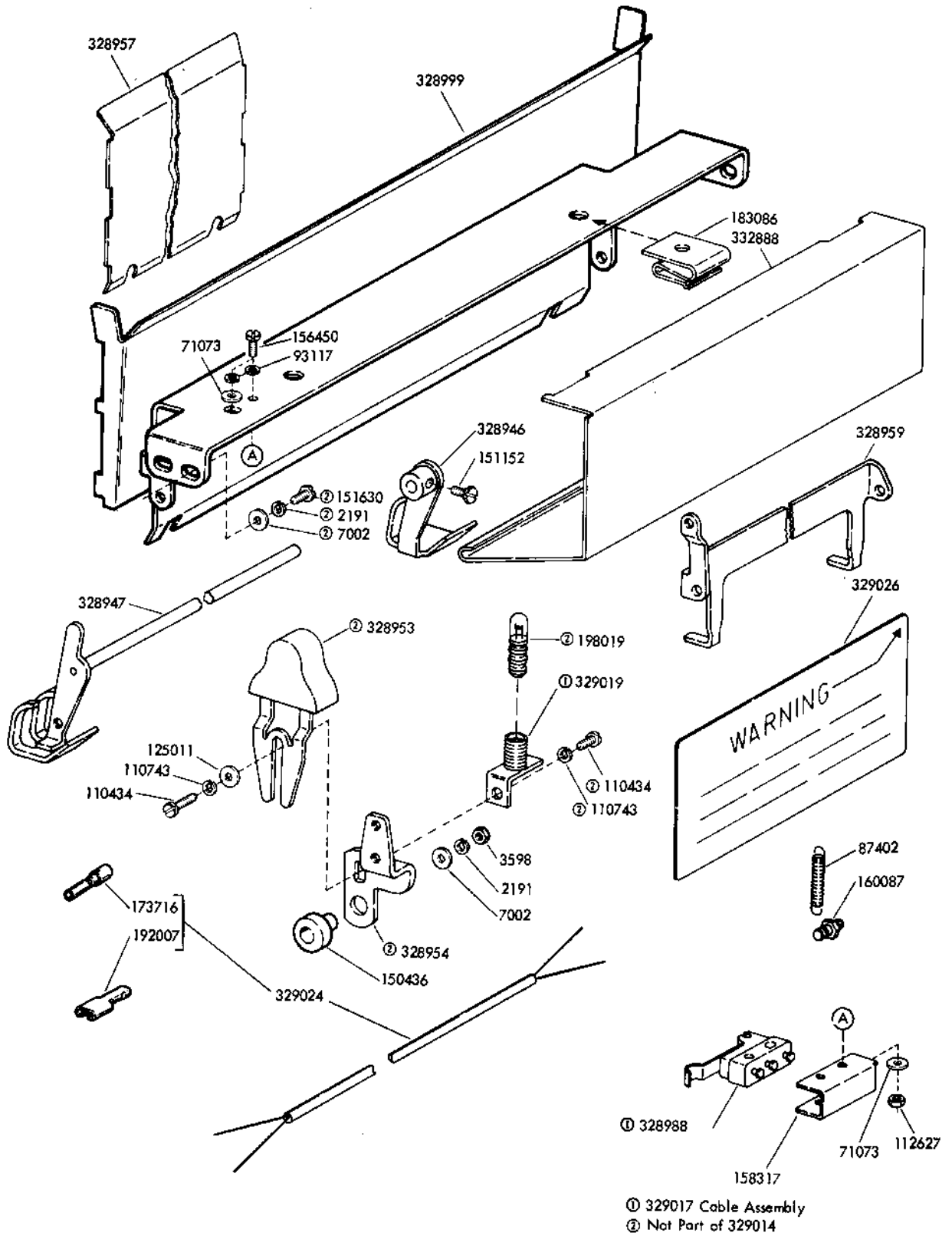
FIGURE 68. 329014 PAPER CHUTE ASSEMBLY
