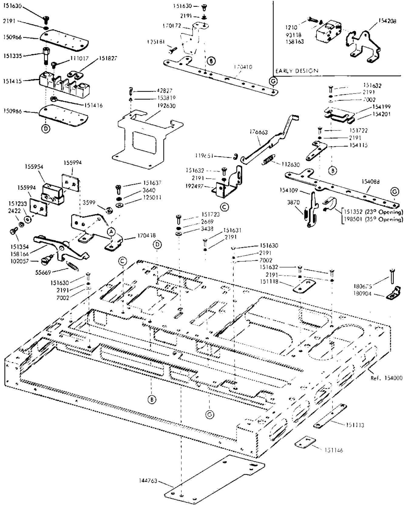
FIGURE 2. BASE (Continued)
