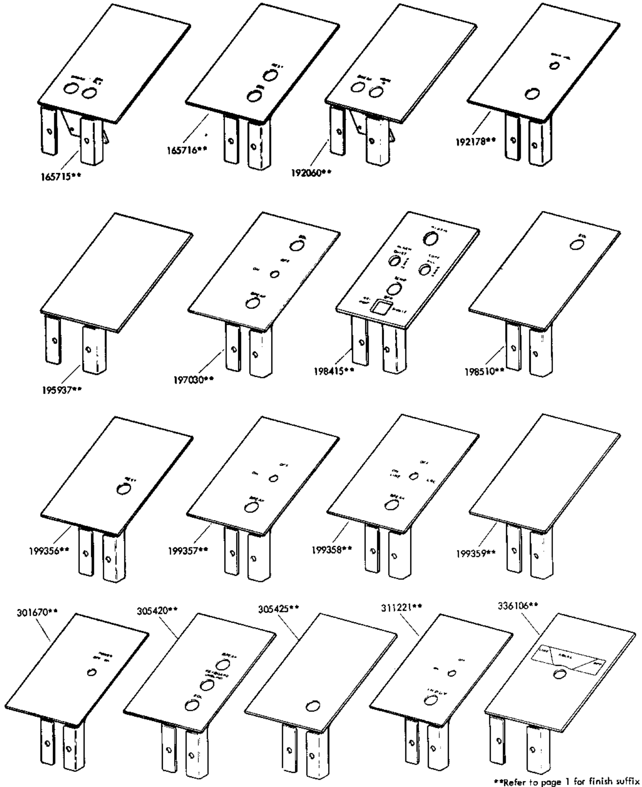
FIGURE 10. CONTROL PANELS
