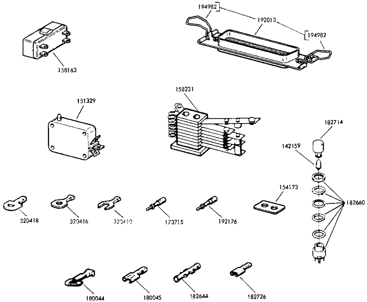
FIGURE 28. CABLE COMPONENTS
