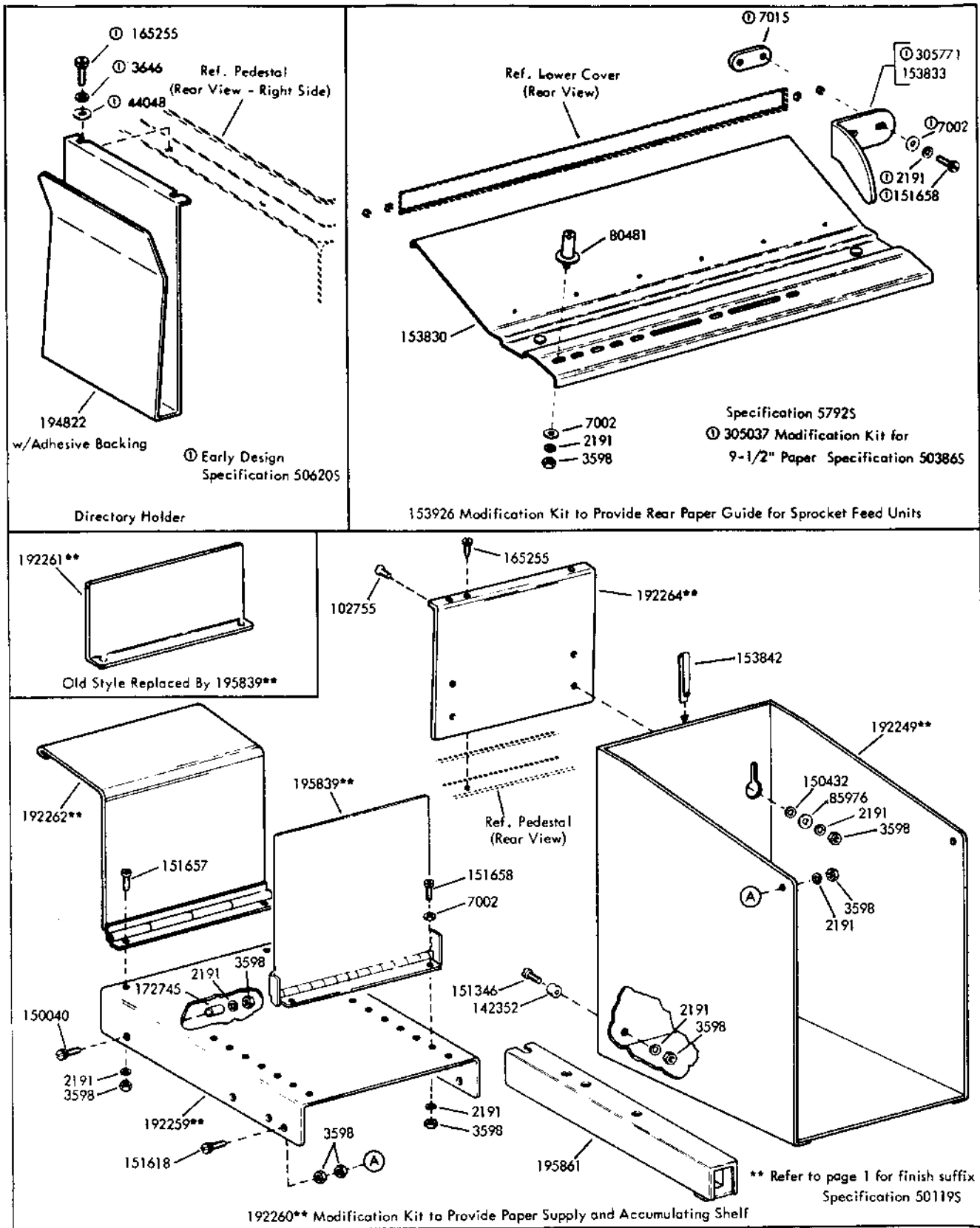
FIGURE 15. PAPER HANDLING AND DIRECTORY HOLDER MODIFICATION KITS
