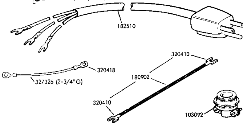
FIGURE 12. CABLE COMPONENTS
