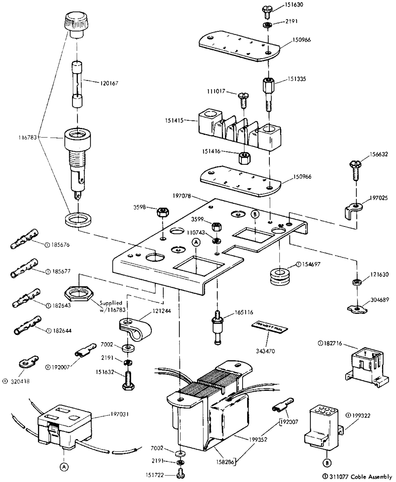
FIGURE 8. 311076 POWER DISTRIBUTION ASSEMBLY
