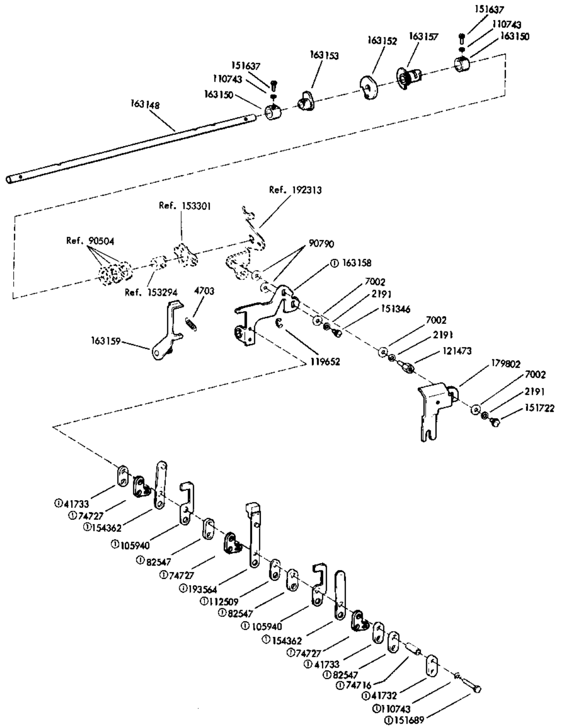
①163147 Contact Assembly Specification 58045
