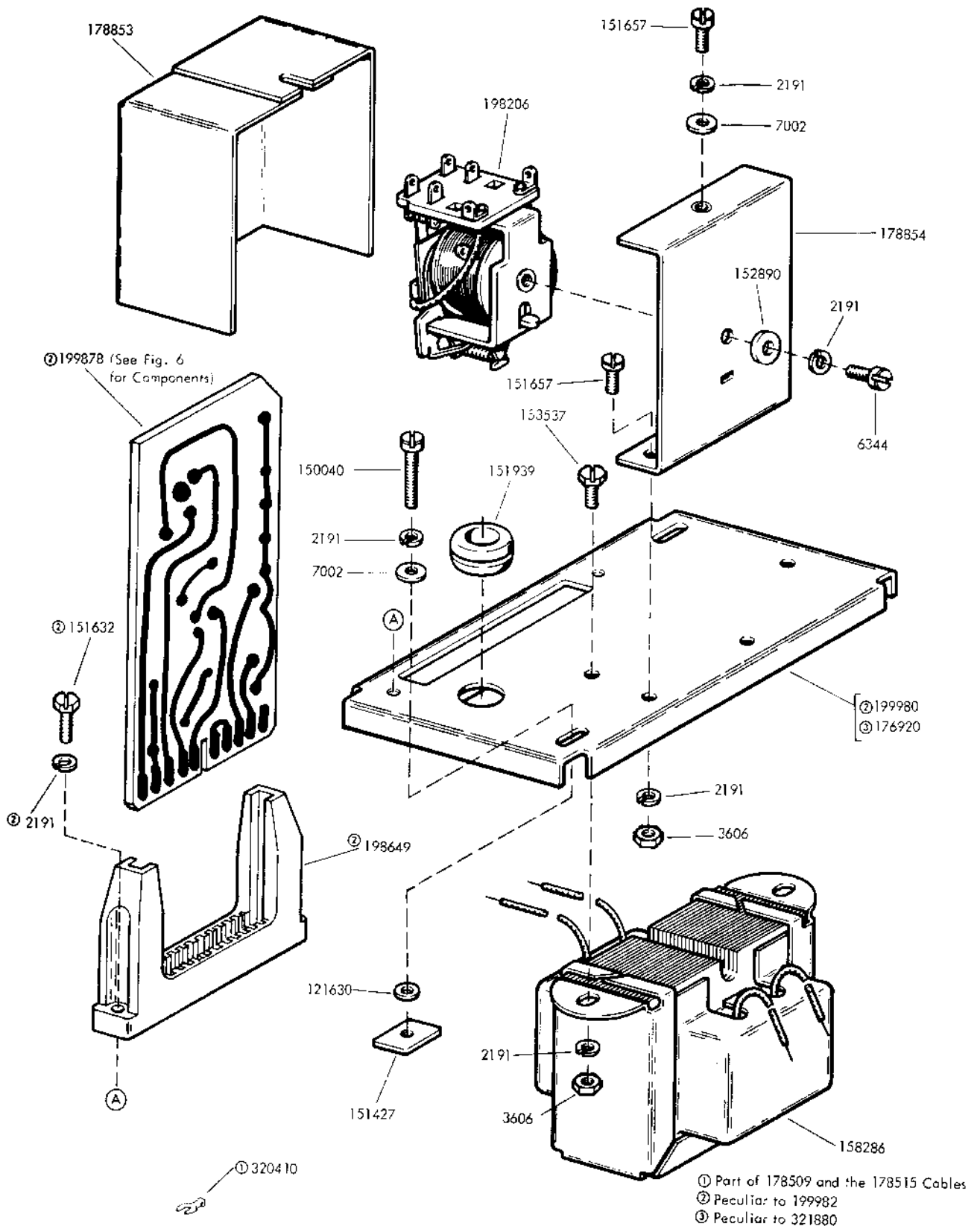
FIGURE 4. 199982 LINE SHUNT RELAY ASSEMBLY WITH AUXILIARY POWER SUPPLY AND THE 321880 LINE SHUNT RELAY ASSEMBLY
