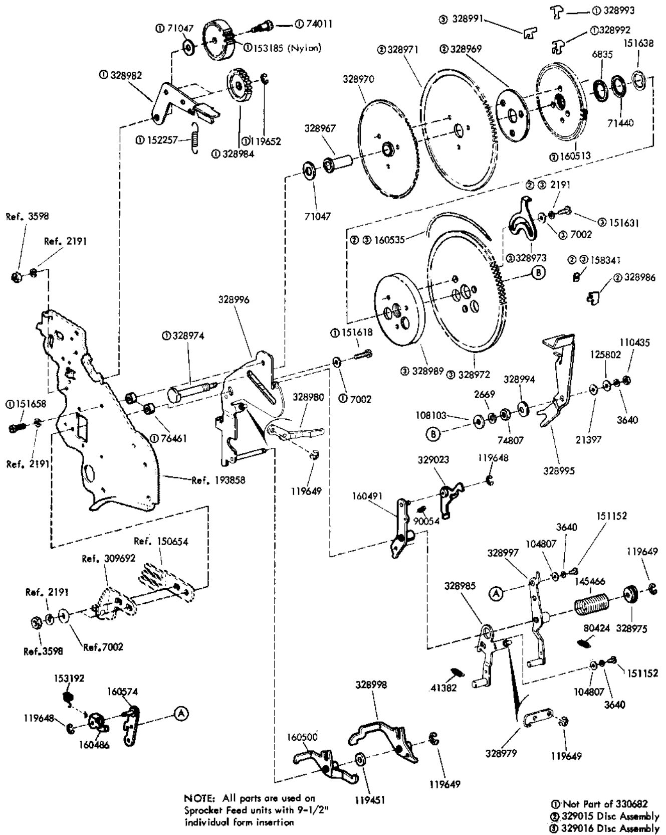
FIGURE 11. 330682 VERTICAL TABULATION ASSEMBLY
