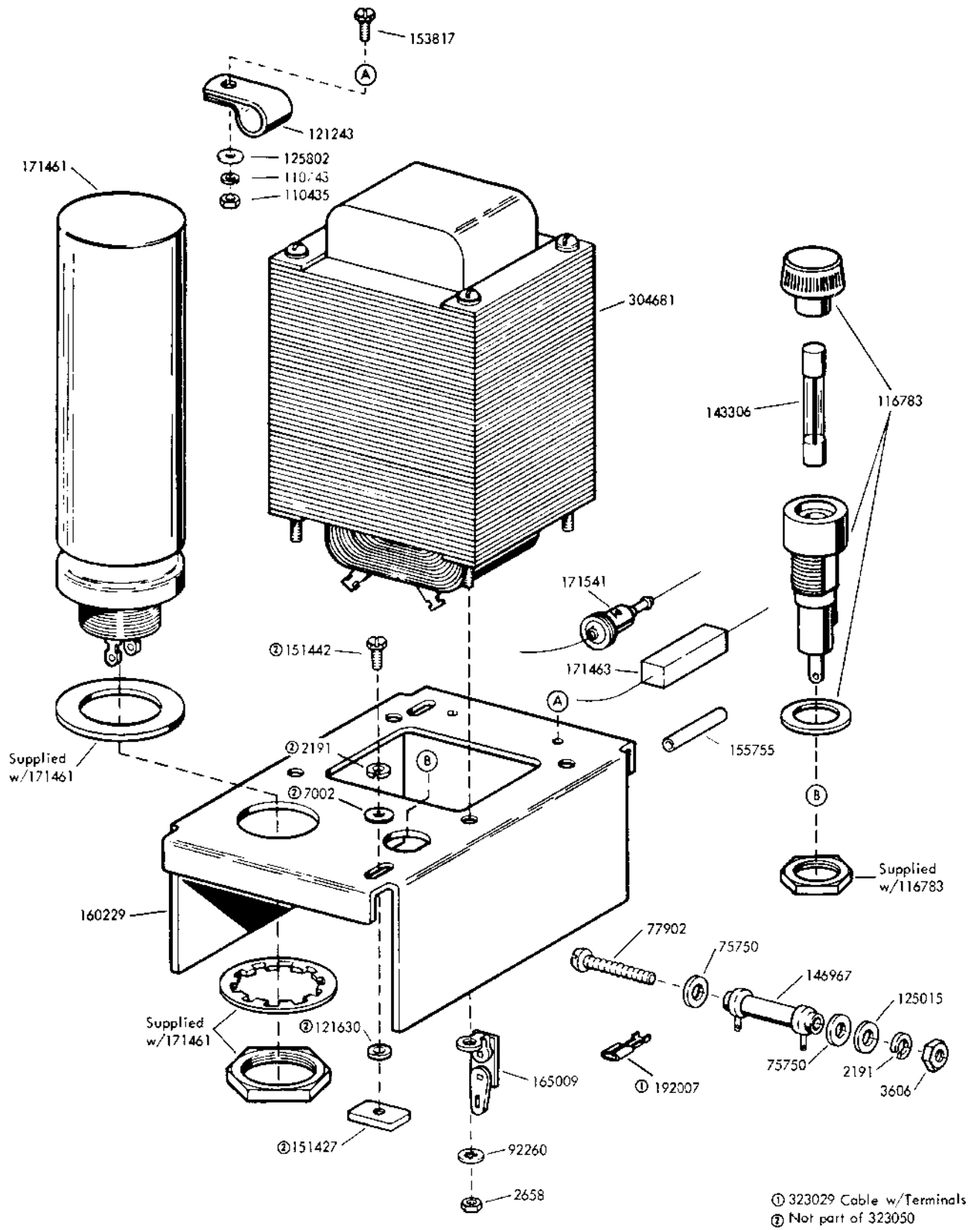
FIGURE 23. 323050 RECTIFIER ASSEMBLY
