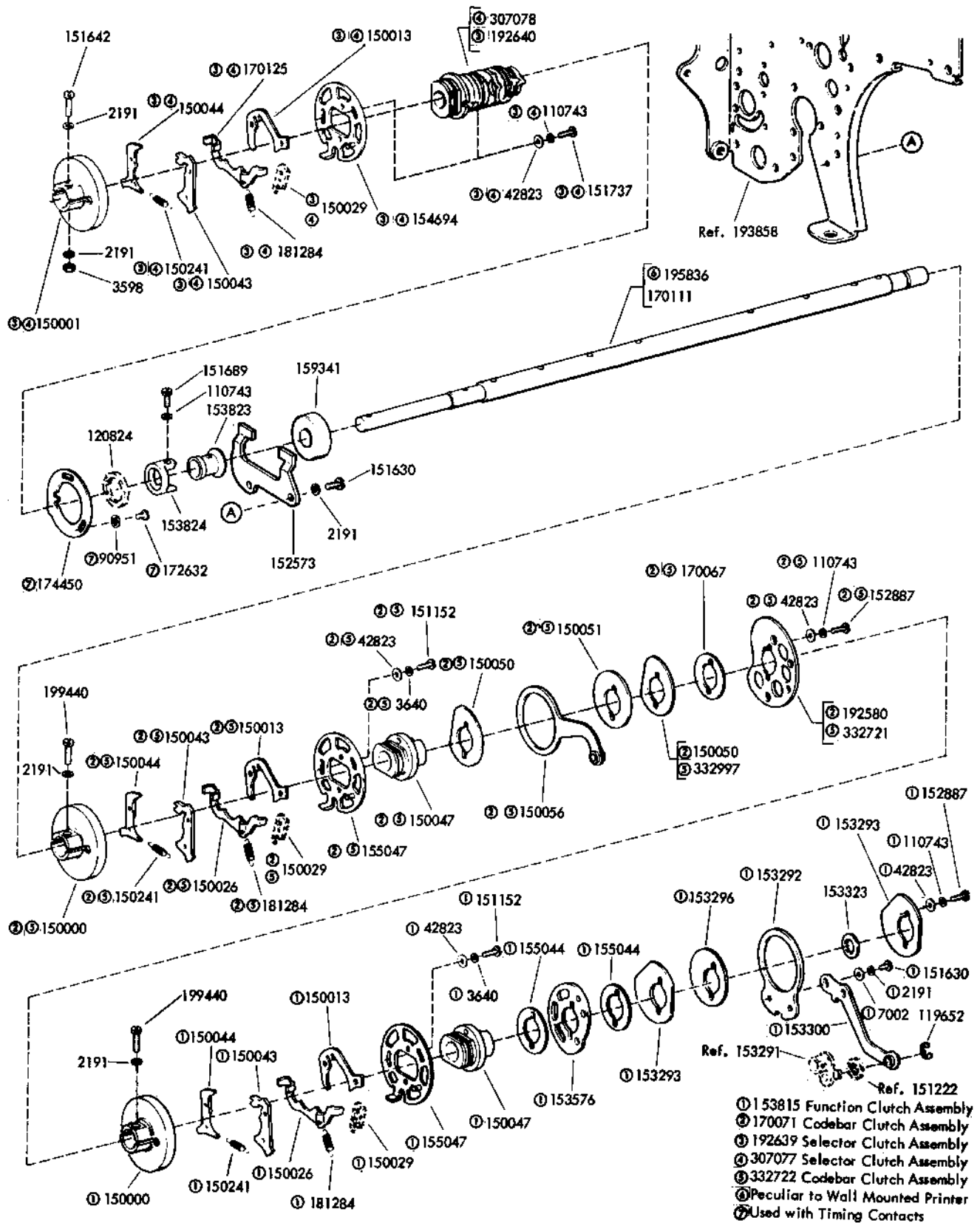
FIGURE 13. MAIN SHAFT MECHANISM
