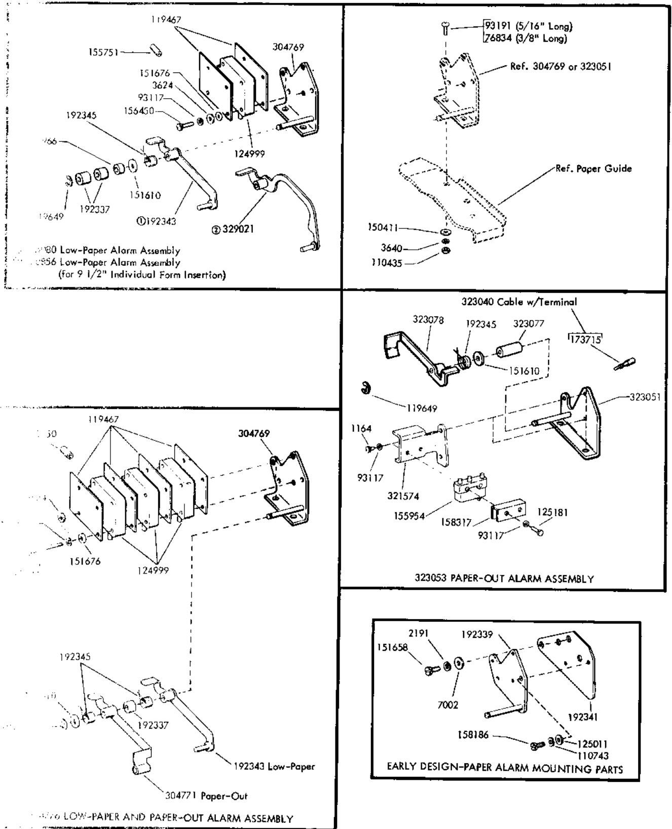
FIGURE 29. LOW-PAPER AND PAPER-OUT ALARMS
