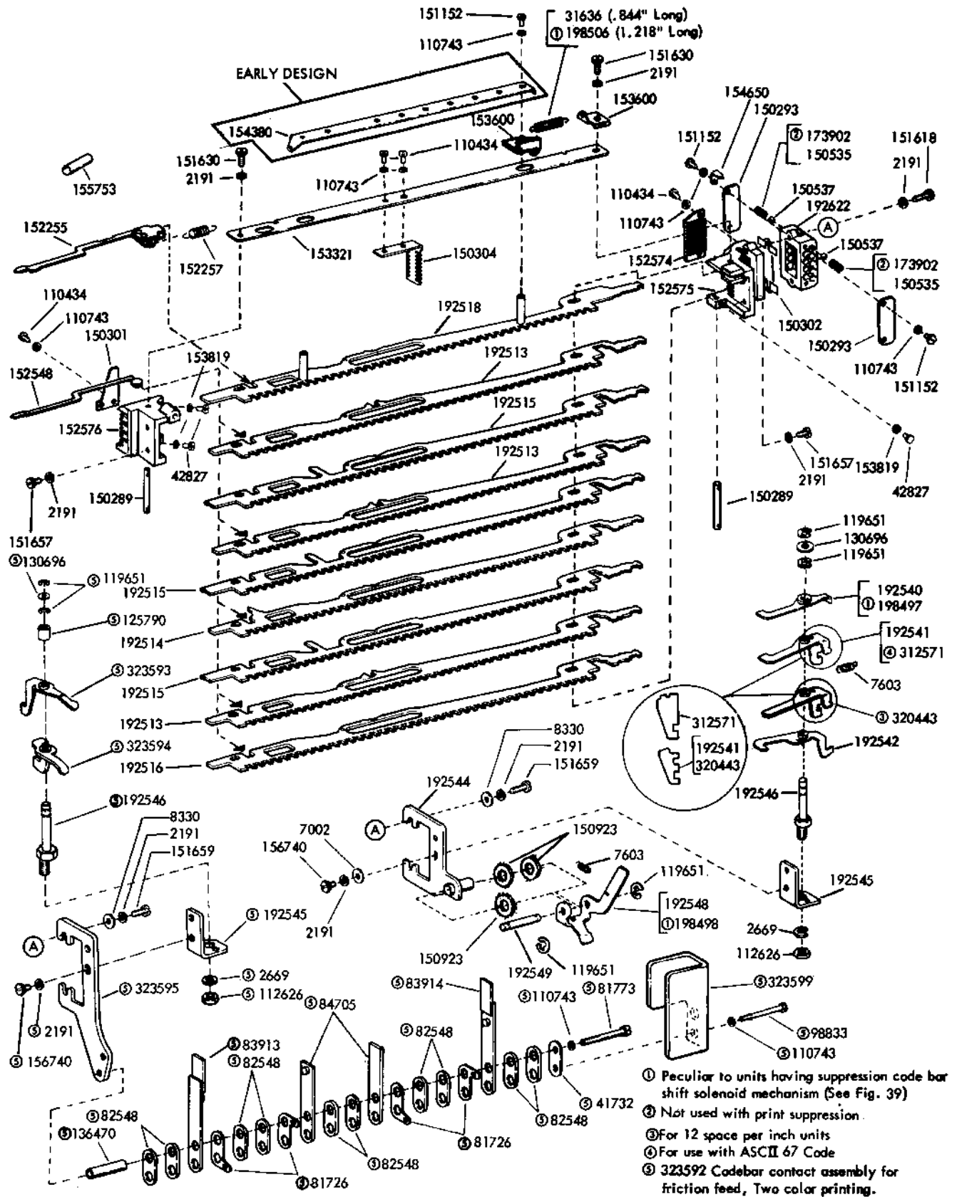
FIGURE 35. CODEBAR MECHANISM
