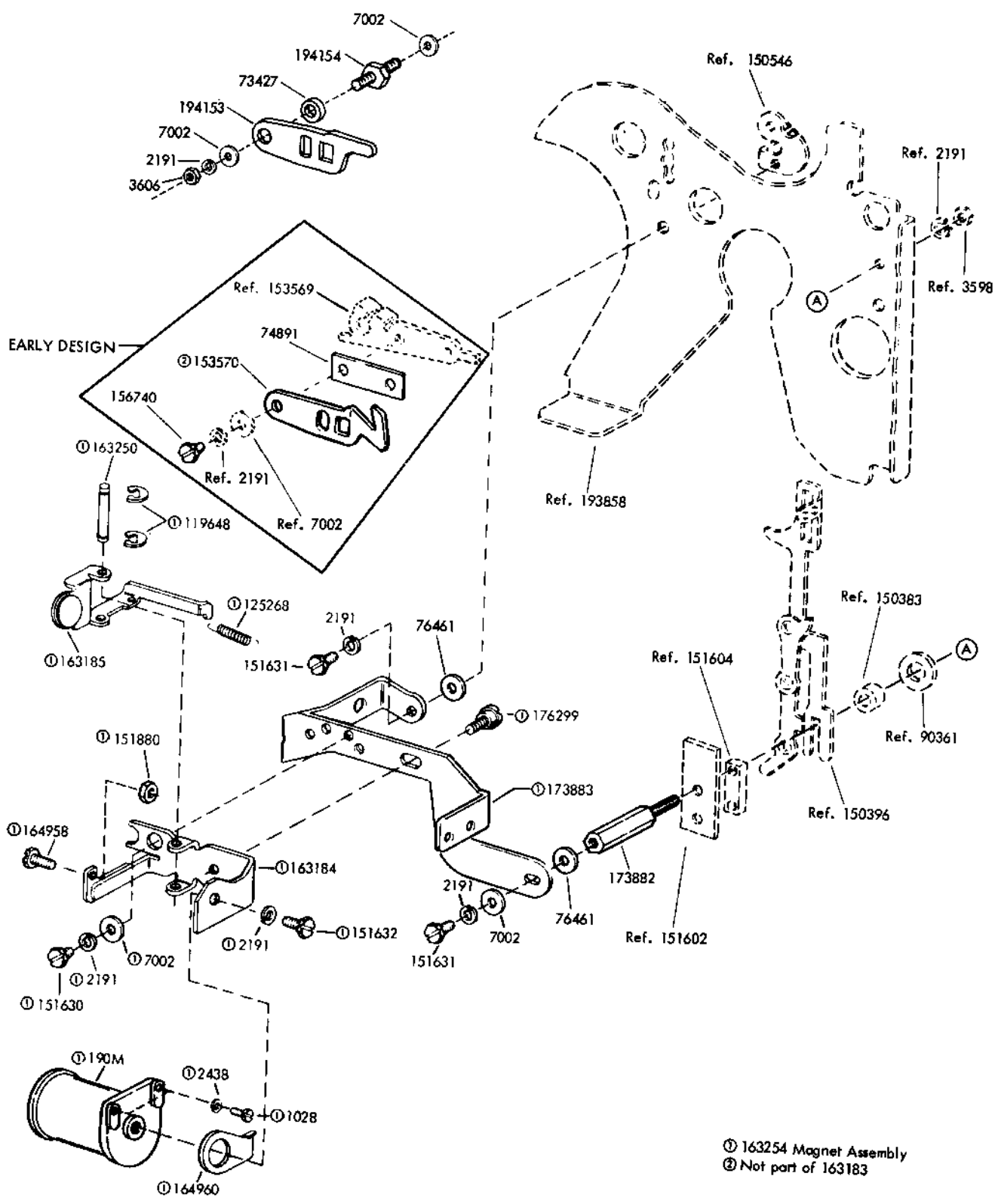
FIGURE 66. 163183 MODIFICATION KIT TO PROVIDE D.C. MAGNET OPERATED PRINT SUPPRESSION
