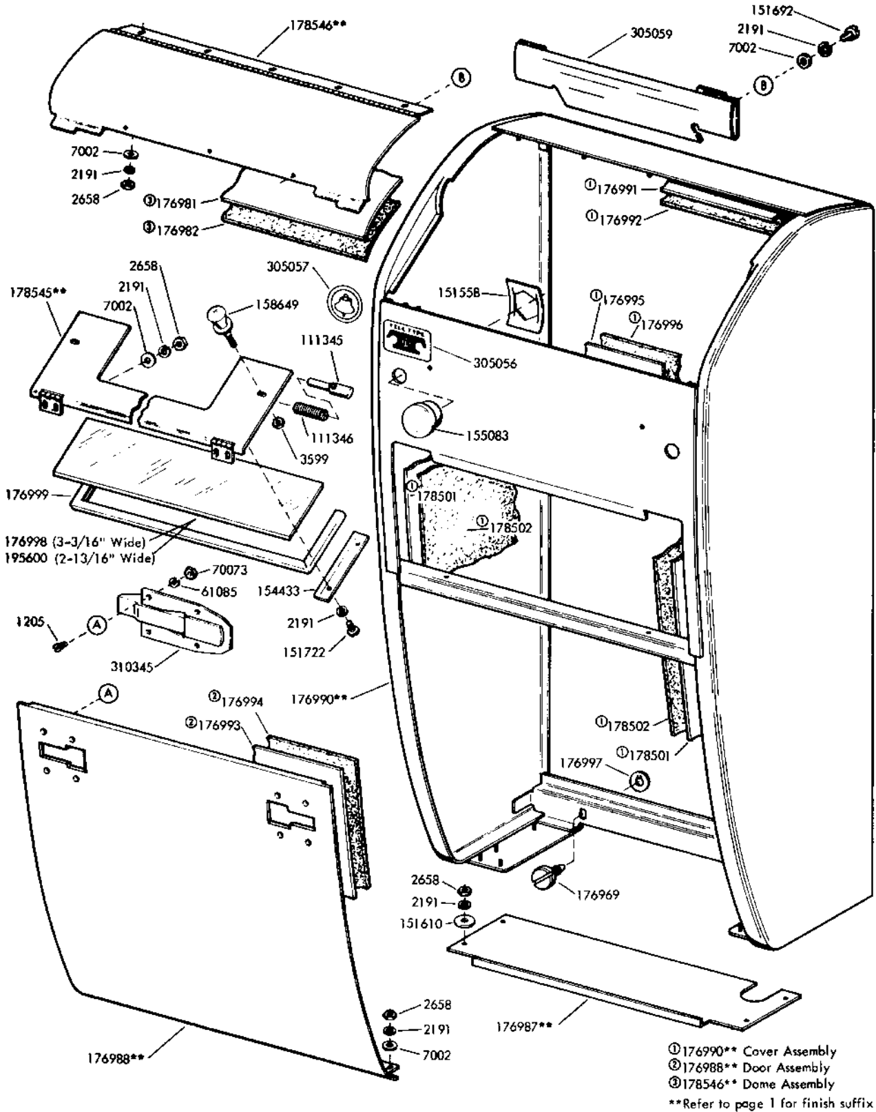
FIGURE 1. COVER
