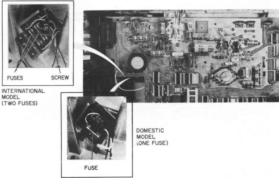
Figure 6-3. Location of Fuses
