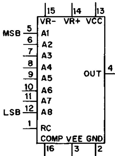
Logic Symbol
