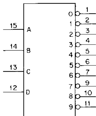
Logic Symbol
