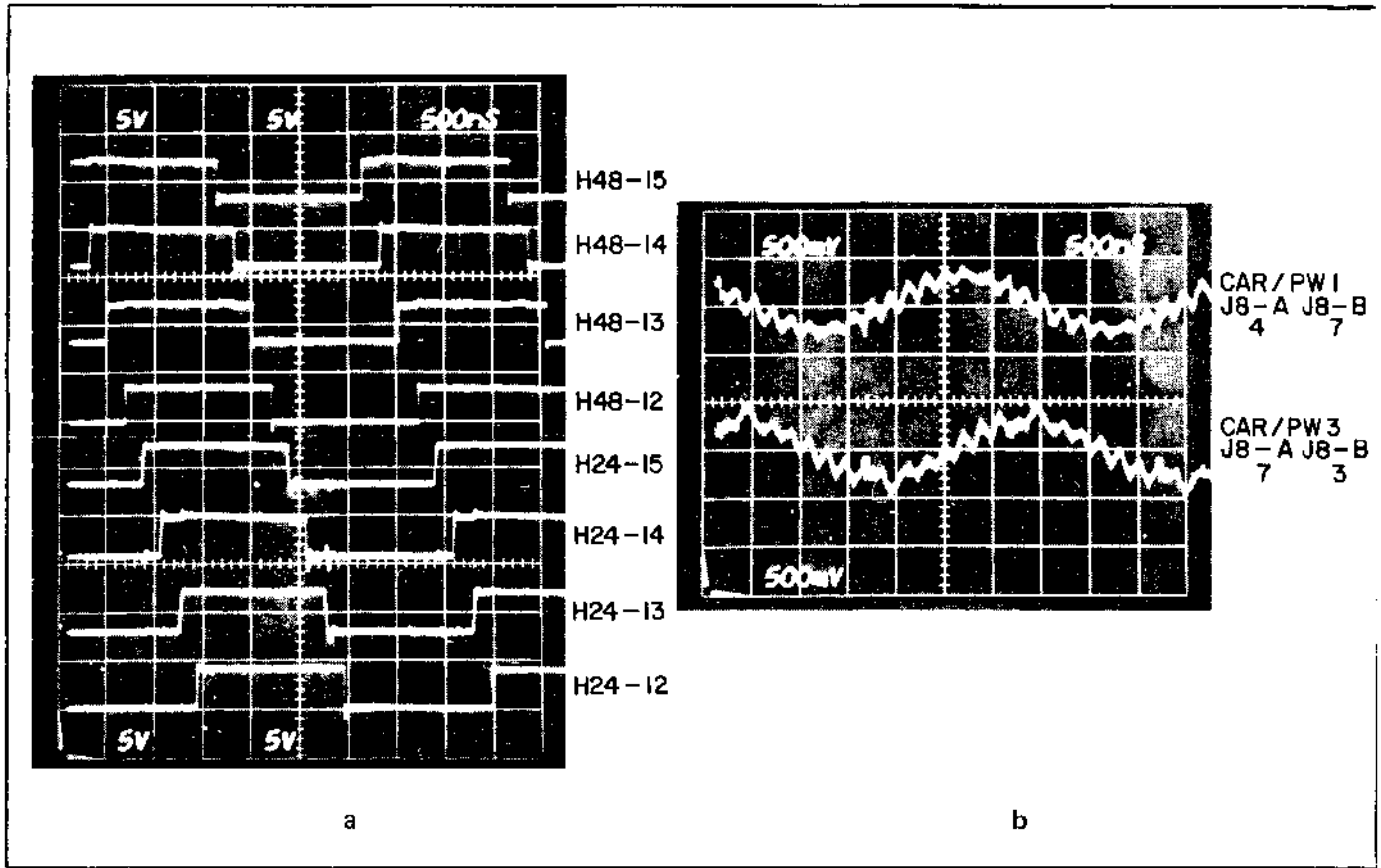
Figure 2-19. Sinewave Drive Generator Waveforms
