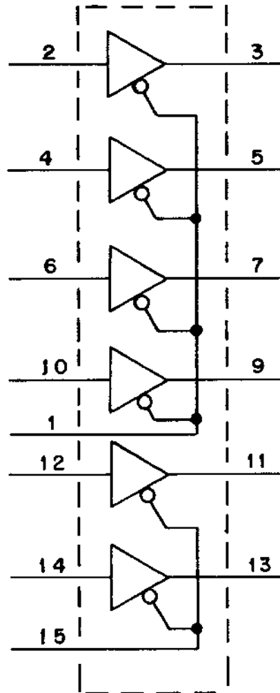
Logic Symbol
