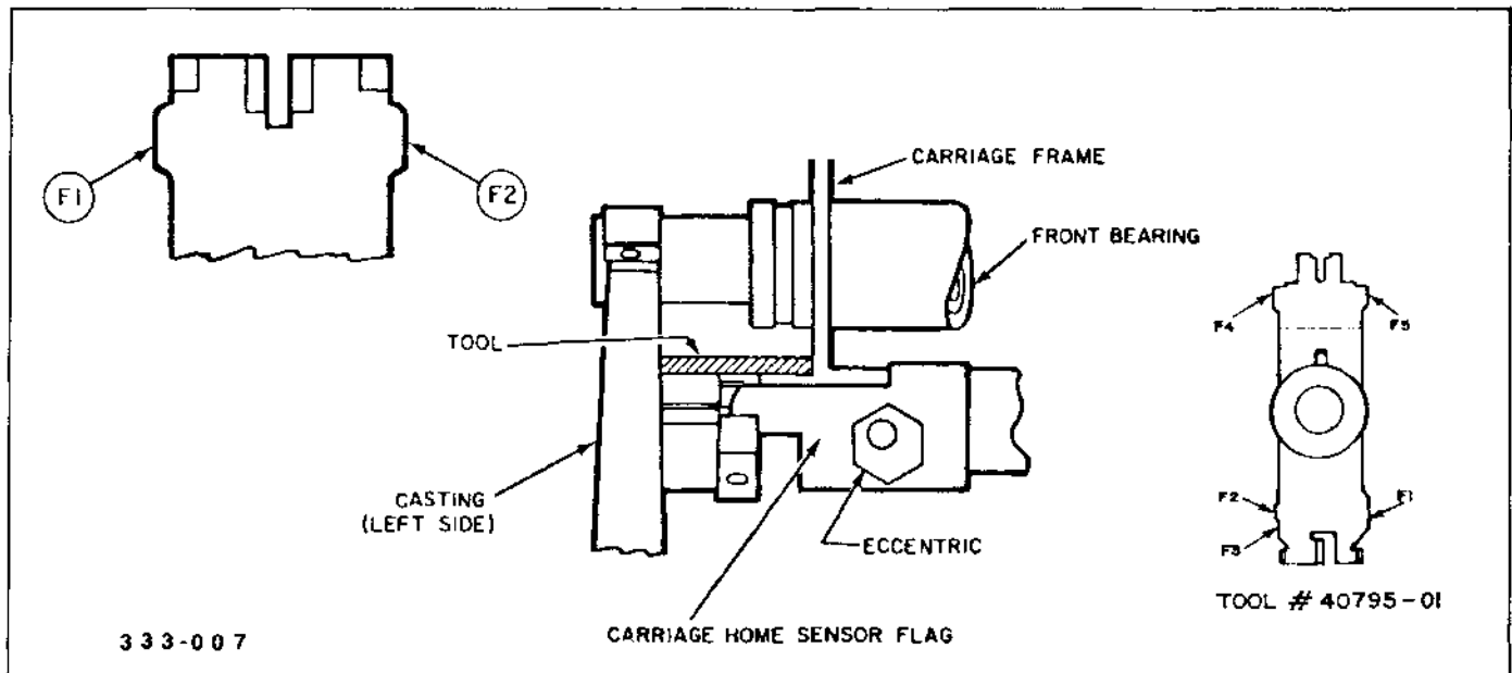
Figure 3-30. Carriage Home Adjustment
