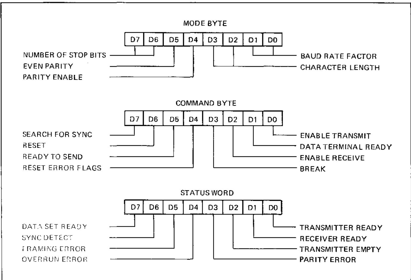
Figure 2-7. USART Control/Status Words
