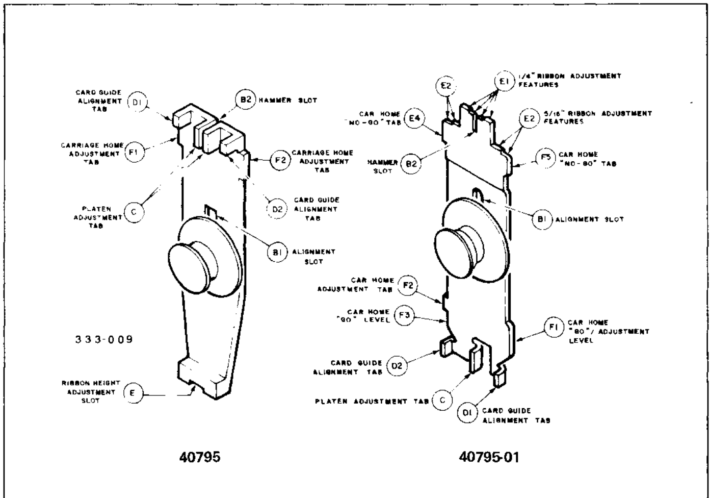
Figure 3-23. Adjustment Tools
