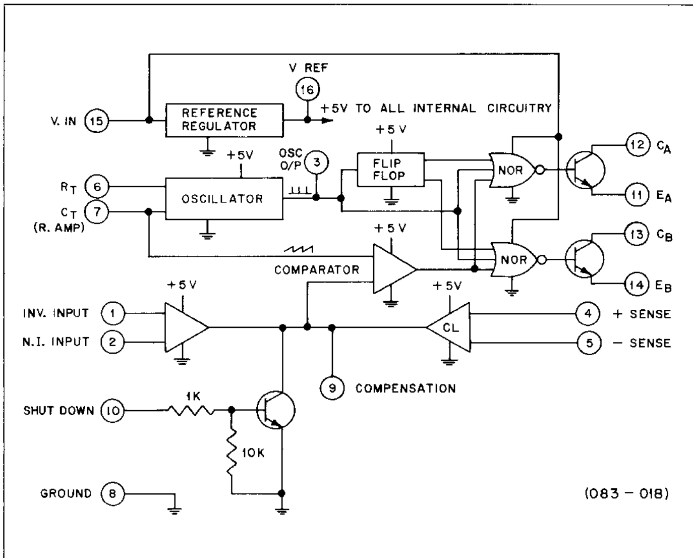
Figure 2-48. LHR Control Module Block Diagram
