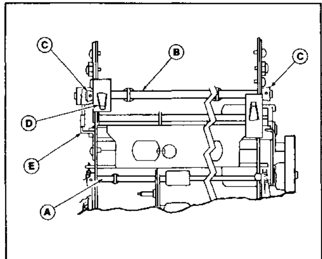
Figure 3-18. Carrier Assembly Adjustment
