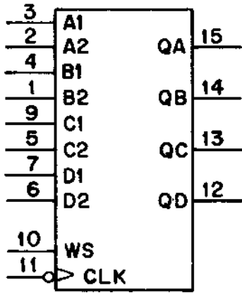
Logic Symbol
