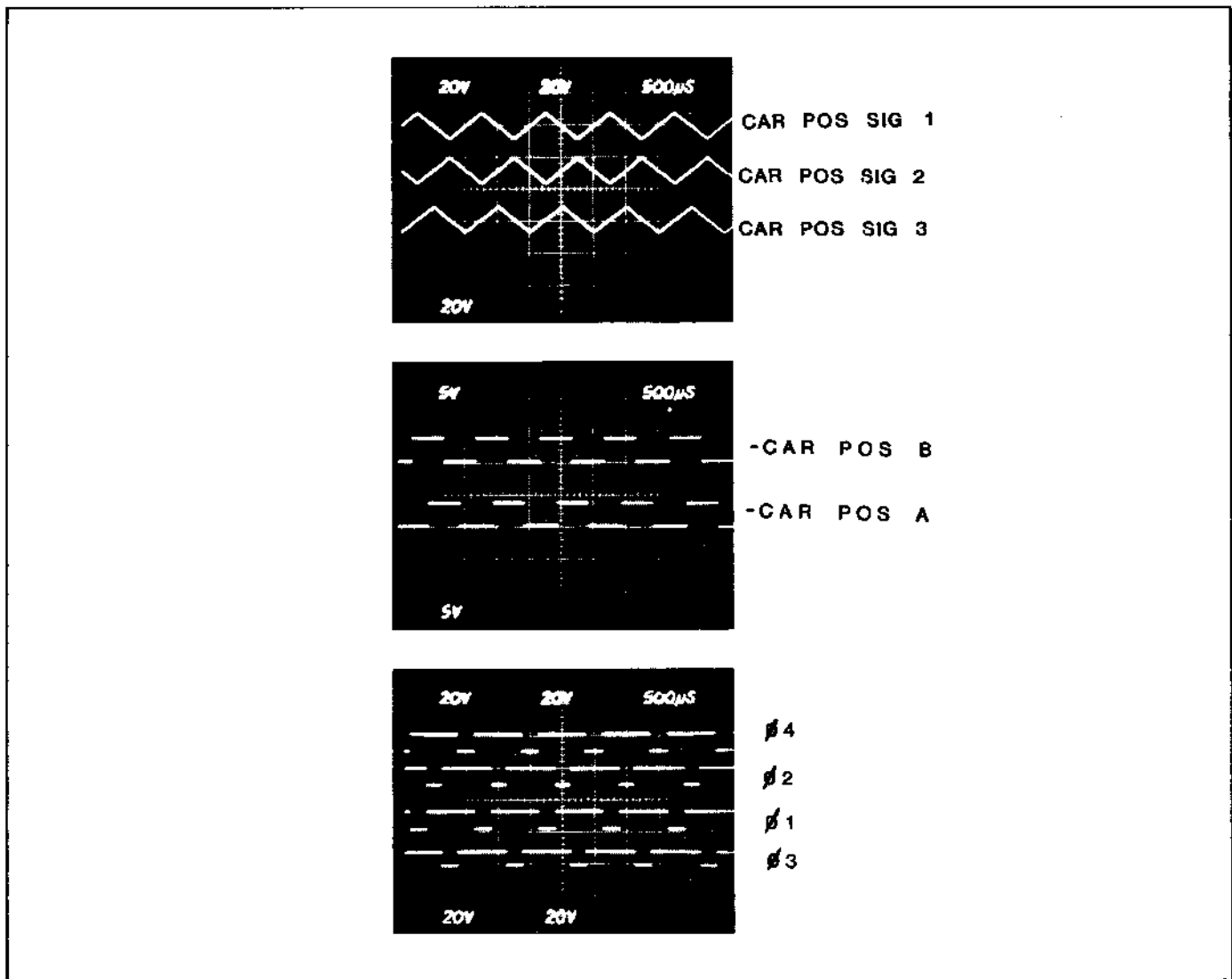
Figure 2-17. CAR POS Tachometer Waveforms
