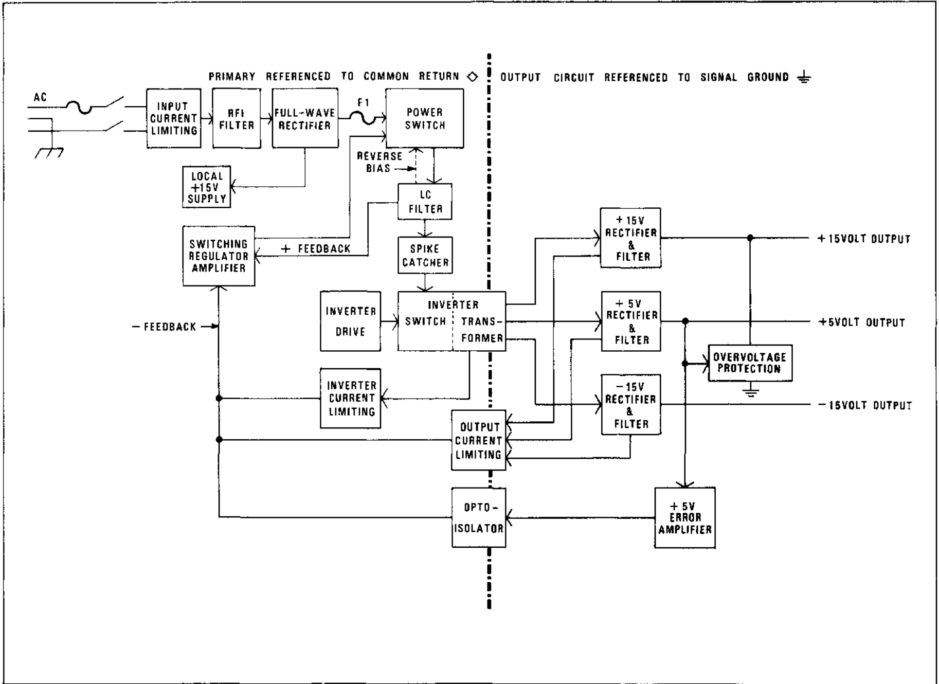
Figure 2-42. Block Diagram, Boschert Power Supply
