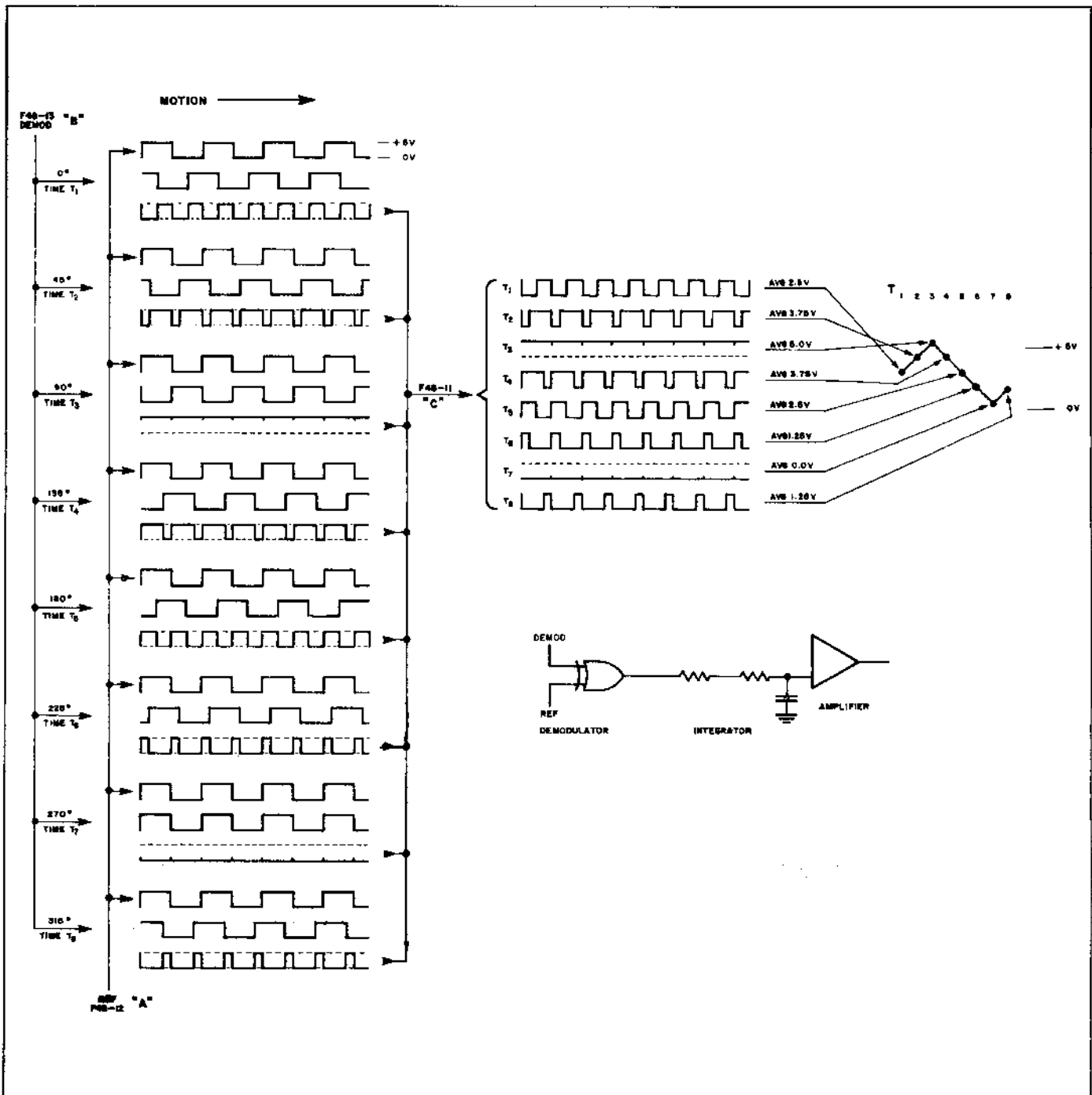
Figure 2-25. CAR POS SIG Development
