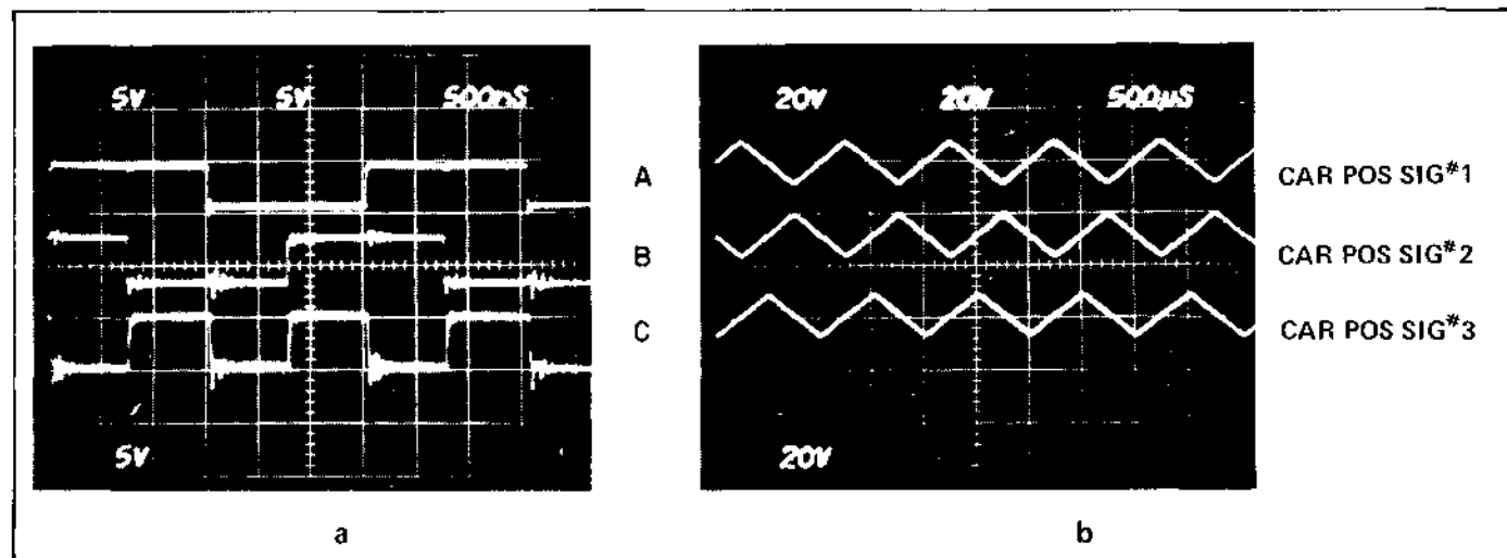
Figure 2-24. Servo Feedback Demodulator/Integrator/Amplifier Waveforms
