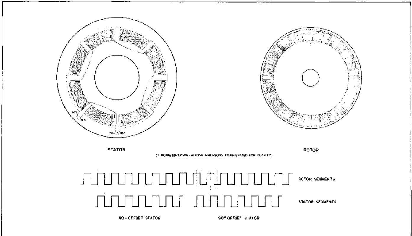
Figure 2-20. Servo Position Transducer
