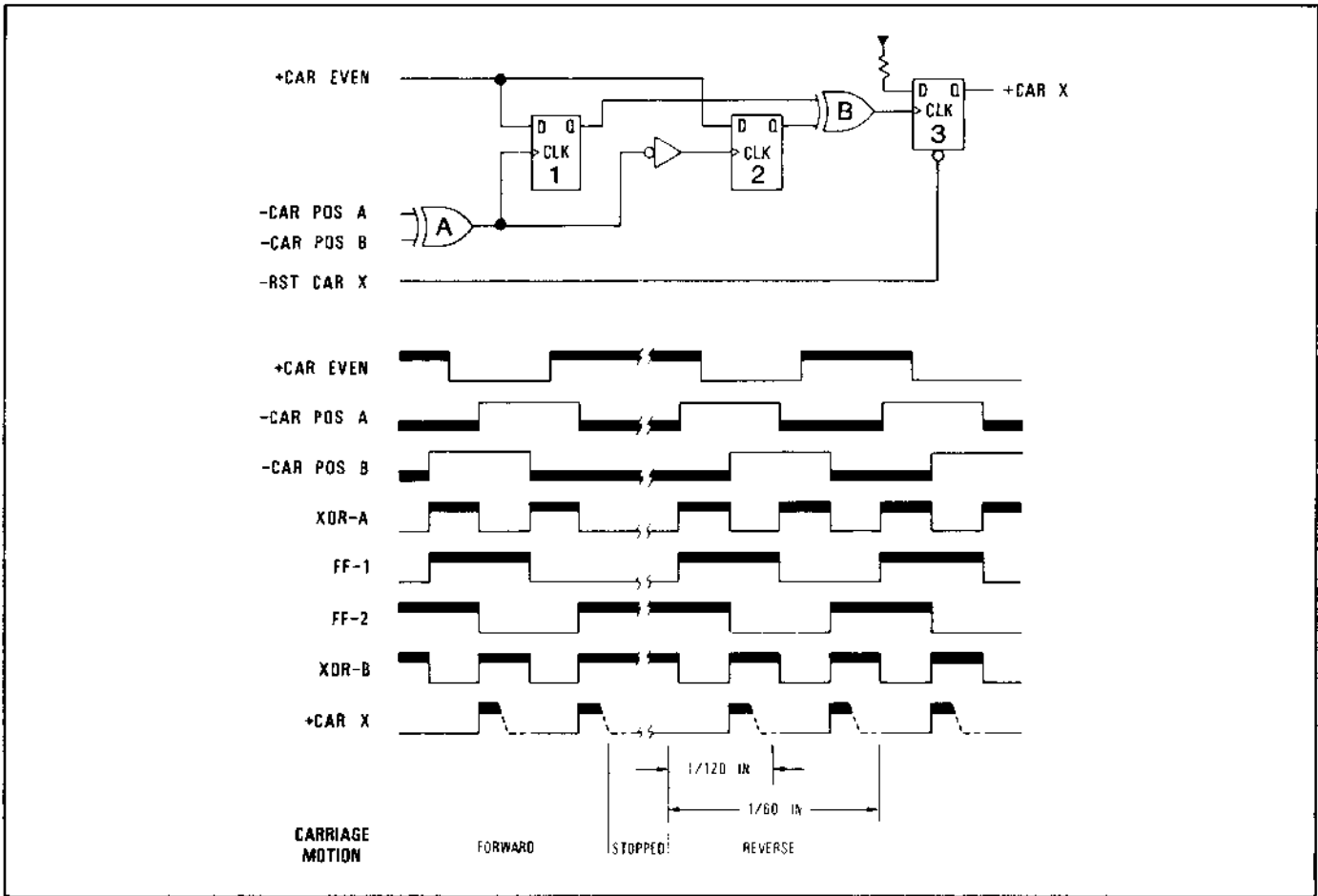
Figure 2-9. Carriage Counter Decrement Control
