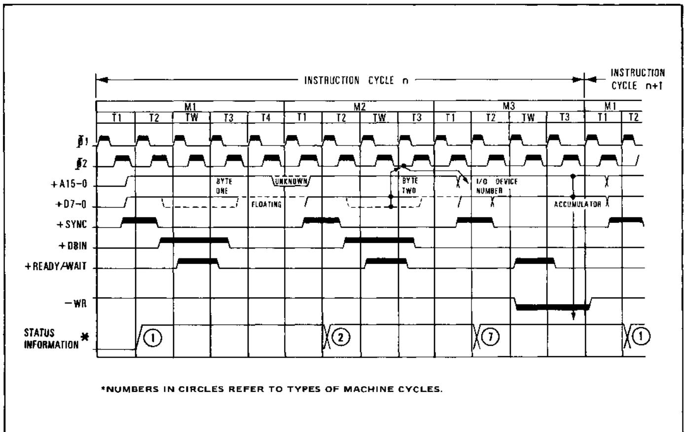
Figure 2-3. Typical Instruction Cycle (Output Instruction)
