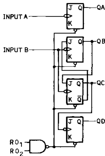
Alternate Symbol
