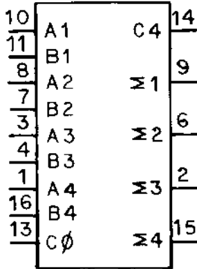
Logic Symbol
