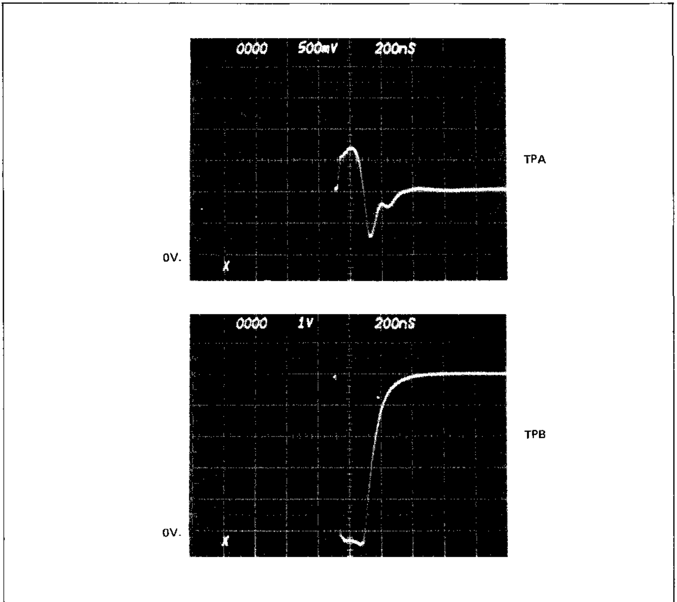
Figure 2-41. Sense Amplifier TPA and TPB
