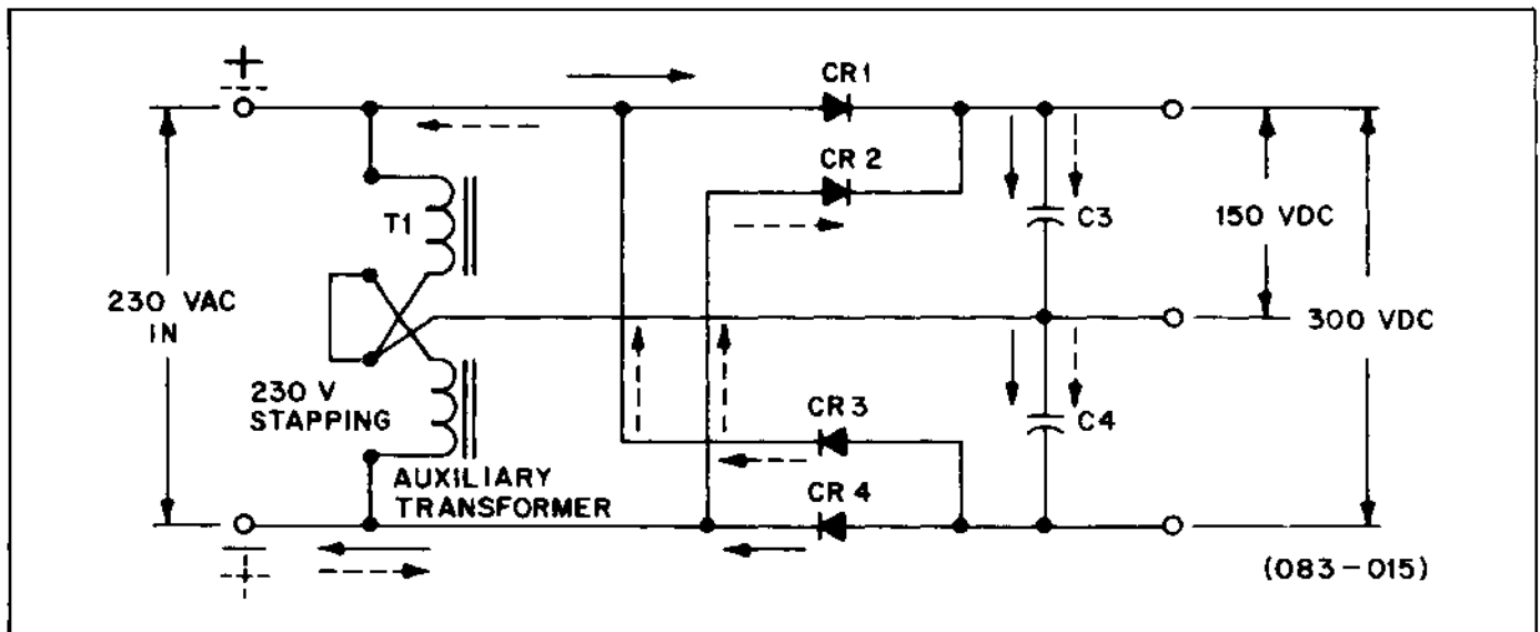
Figure 2-45. LHR Simplified Input Rectifier/Filter Doubler Section (230 VAC Input Strapping)
