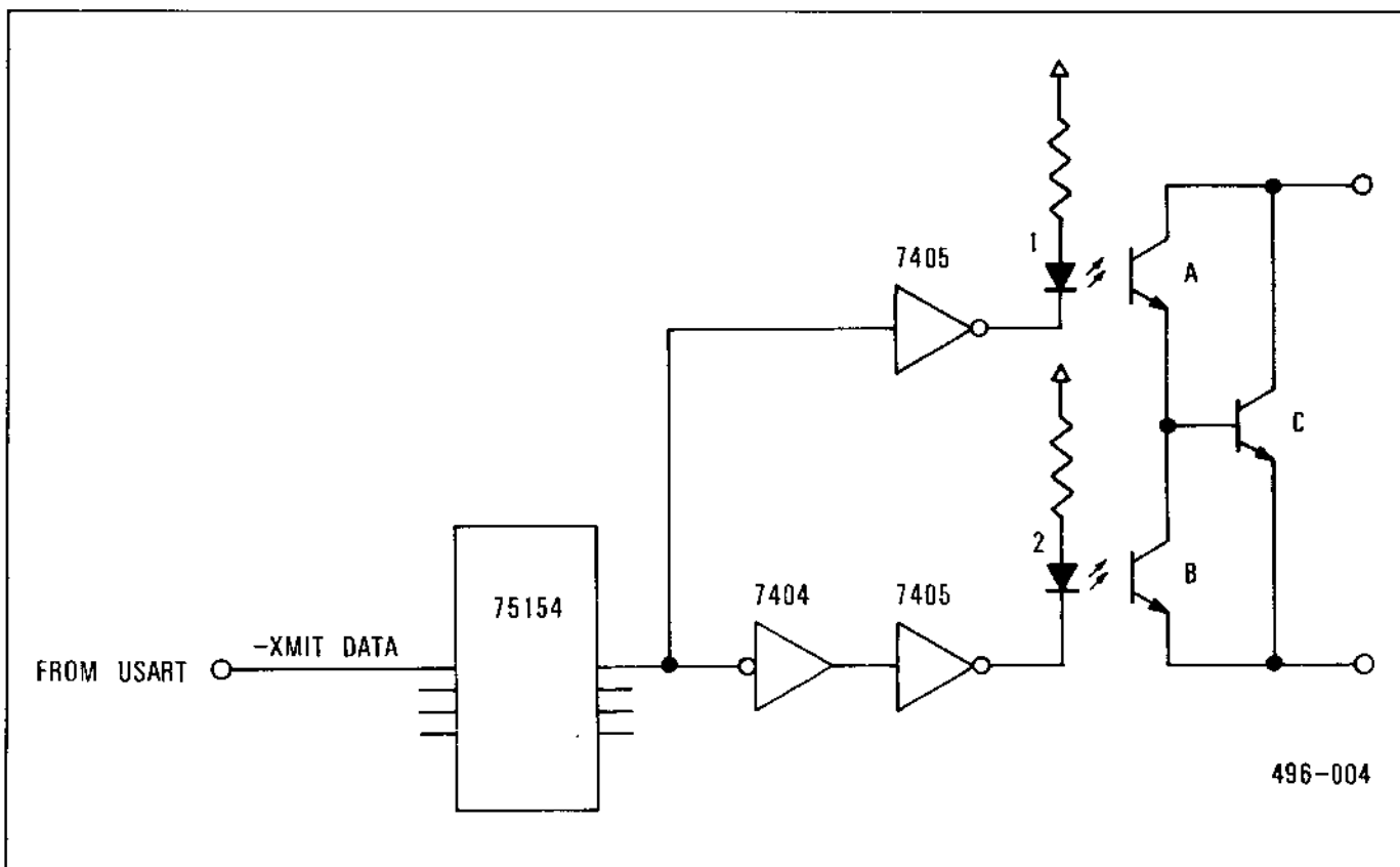
Figure 2-34. Transmitter Circuit
