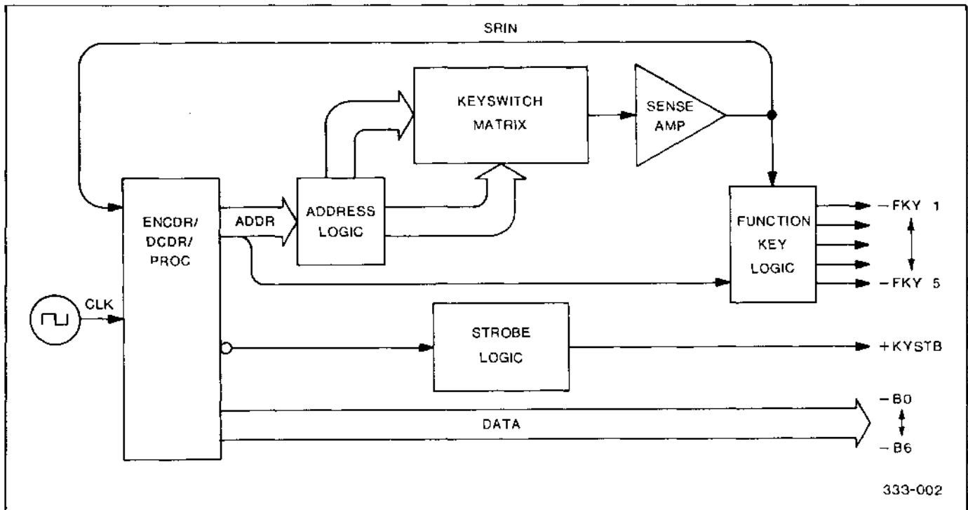
Figure 2-39. Block Diagram, Saturable-Core Keyboard
