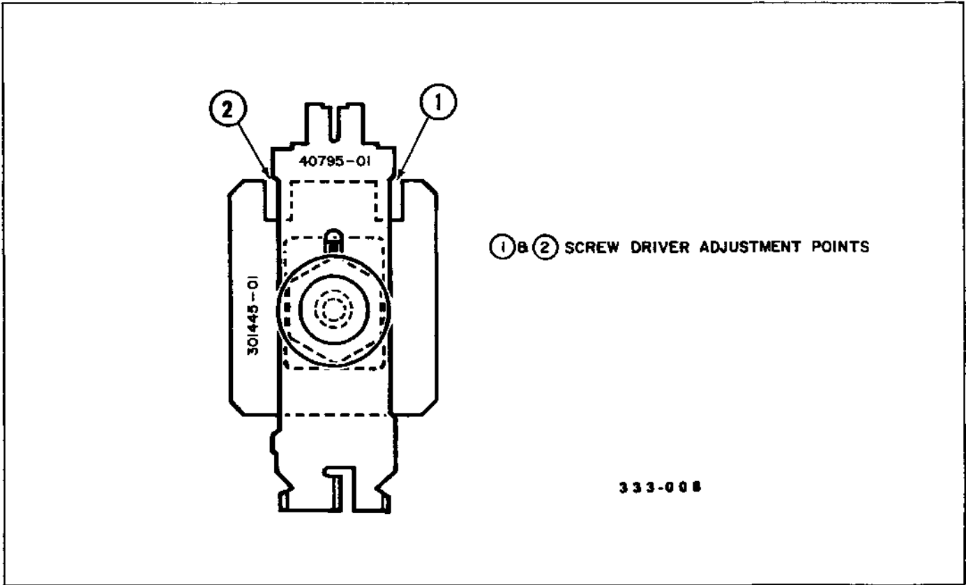
Figure 3-24b. Printwheel Alignment
