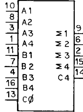
Alternate Symbol
