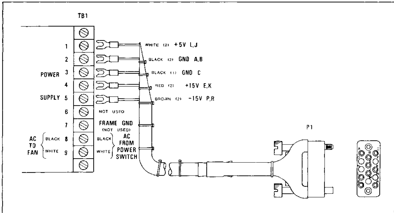
Figure 3-39. Power Supply Connections
