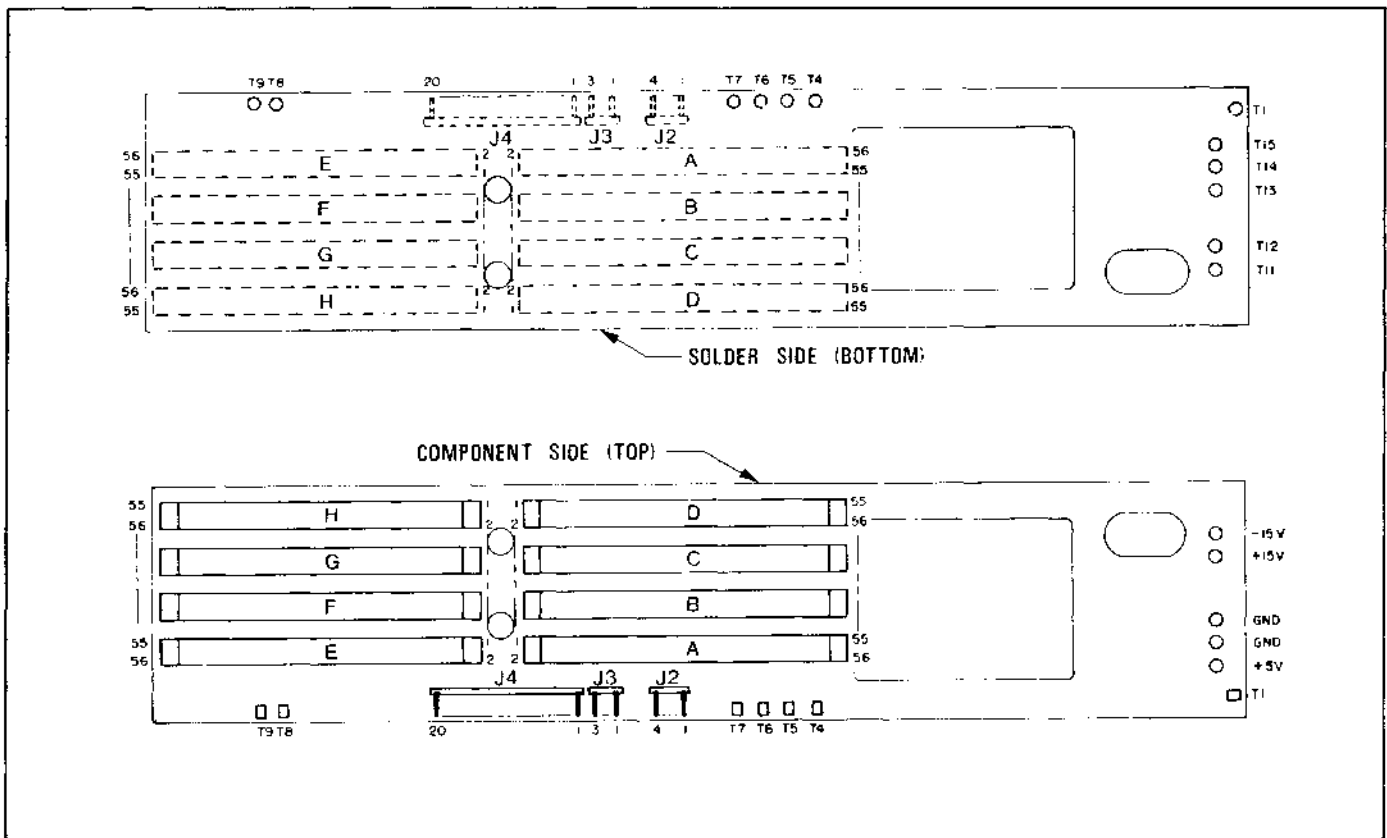
Figure 3-35b. Mother Board Pin Numbering (No. 46080)
