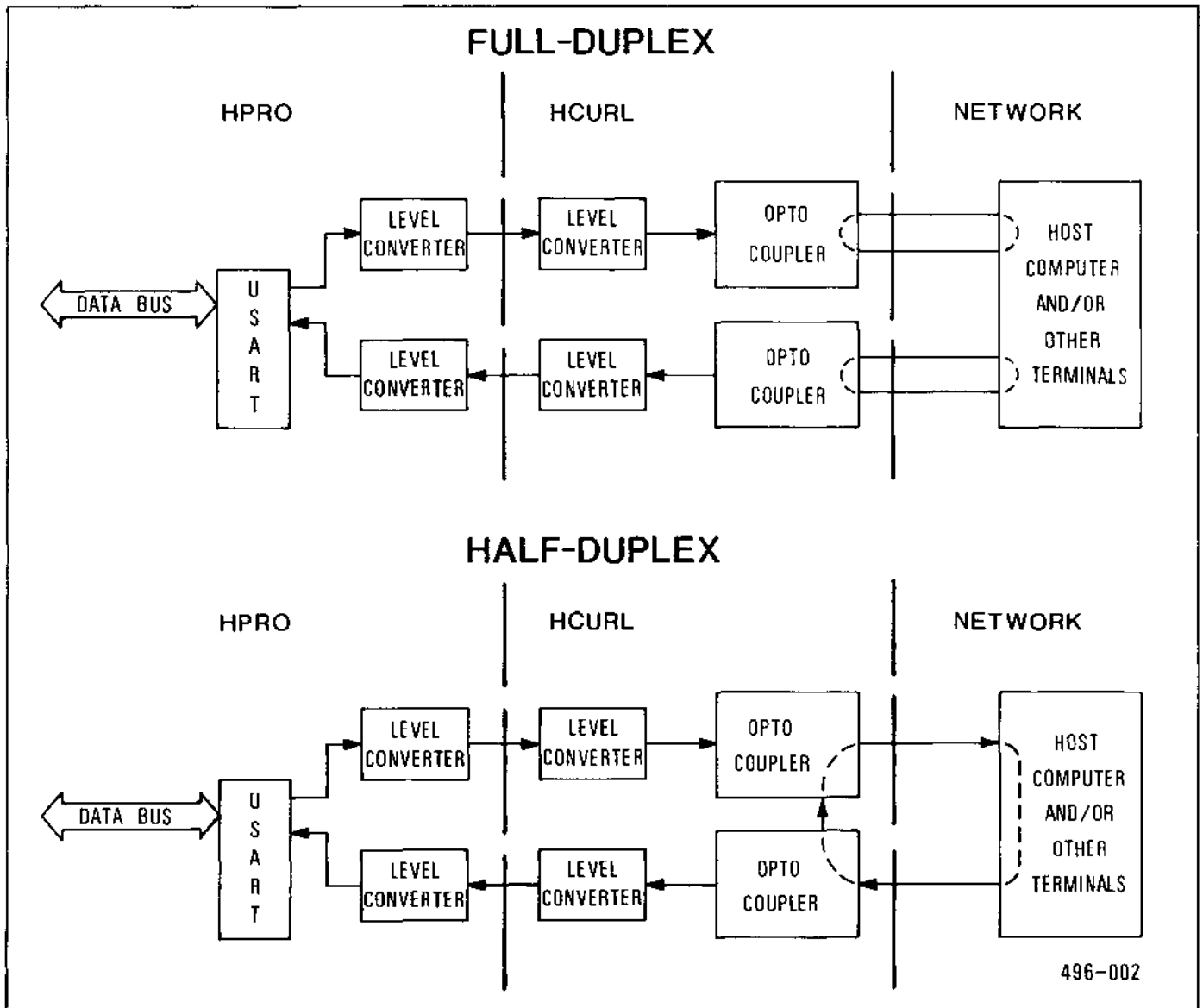
Figure 2-32. Block Diagram, Current Loop Data Flow
