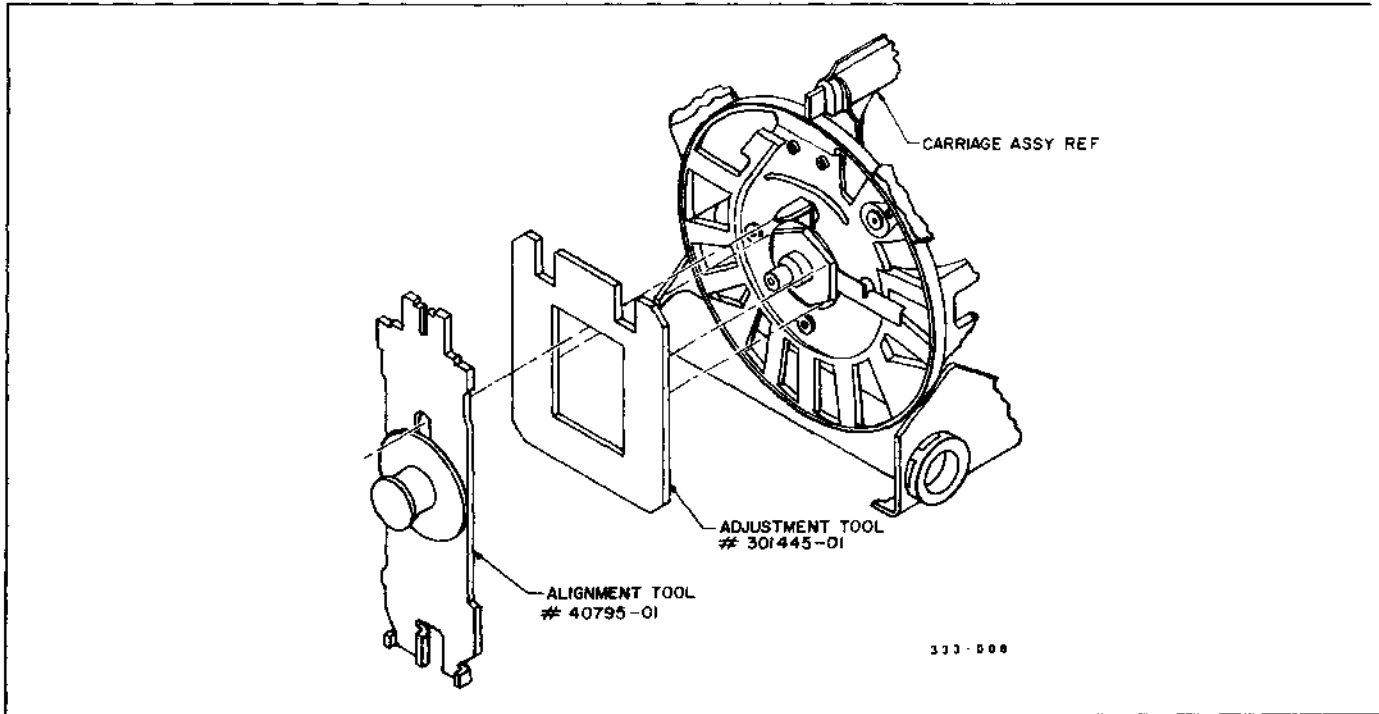
Figure 3-24a Printwheel Alignment
