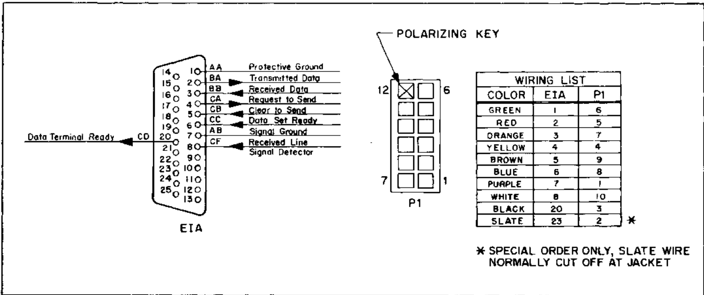
Figure 3-38. EIA Cable Pin Identification
