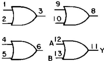
Logic Symbol
