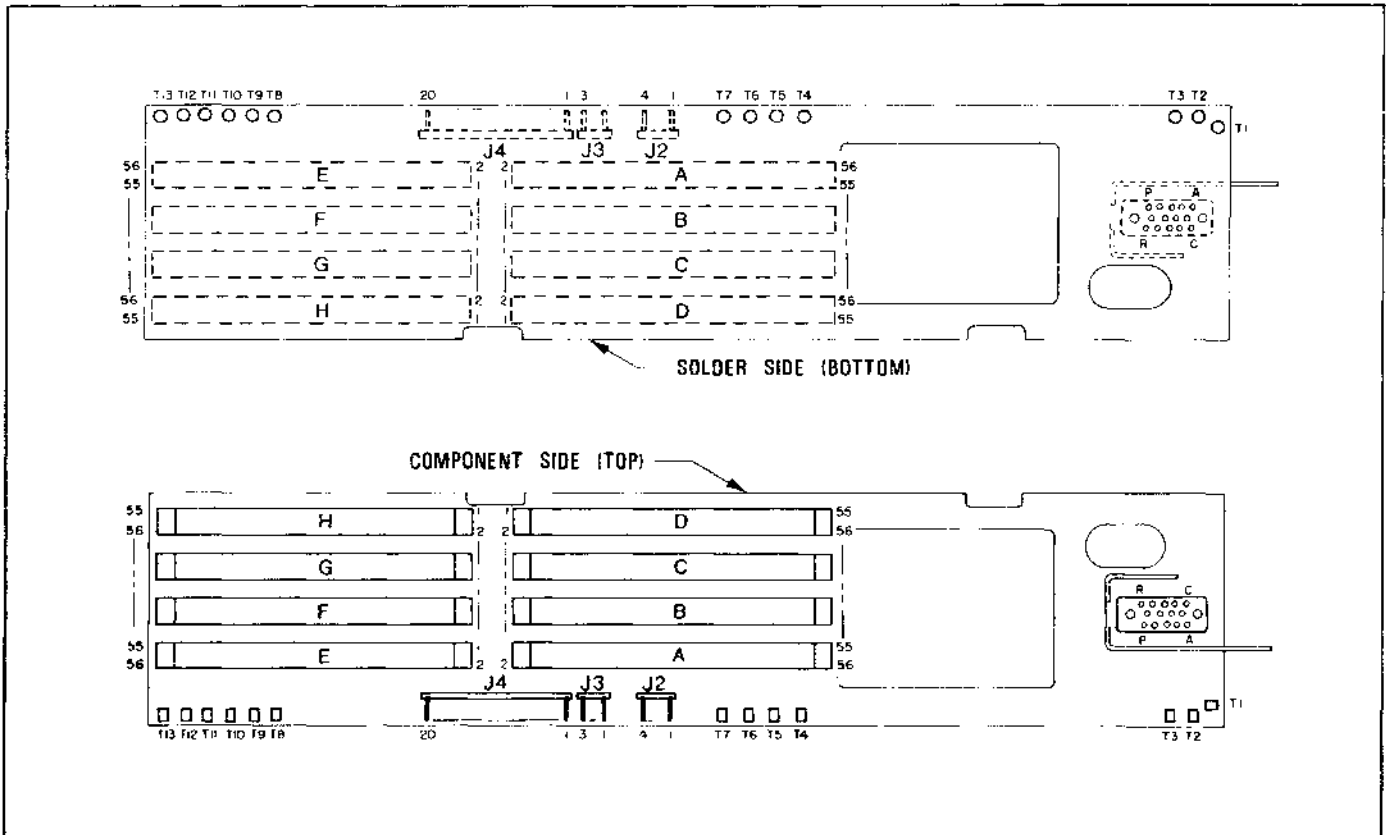
Figure 3-35a. Mother Board Pin Numbering (No. 40614)
