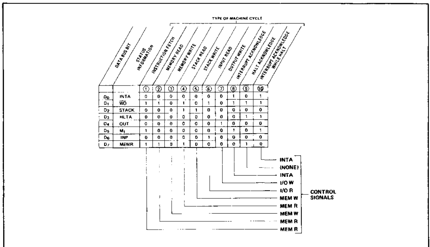
Figure 2-5. MPU Status and Resultant Control Signals
