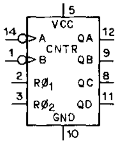
Logic Symbol
