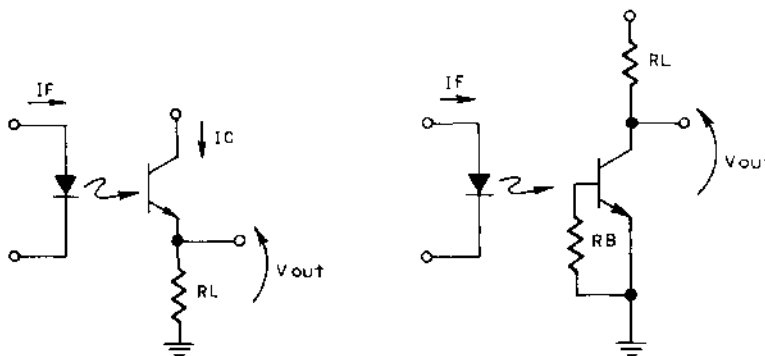
Circuit 1
