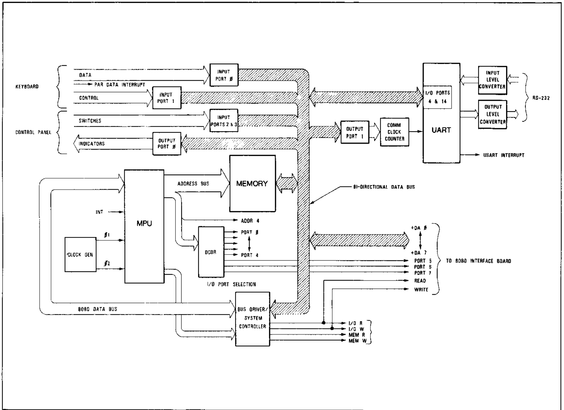
Figure 2-2. HPRO Board Block Diagram
