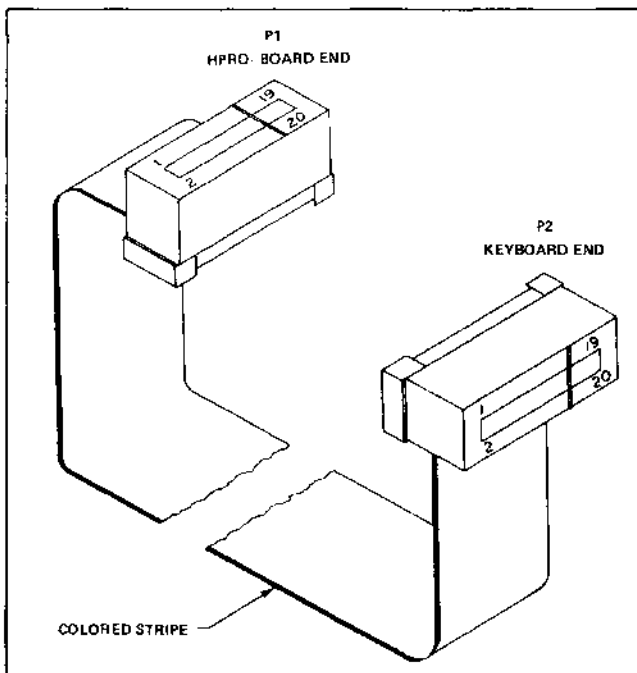
Figure 3-36. Keyboard Cable
