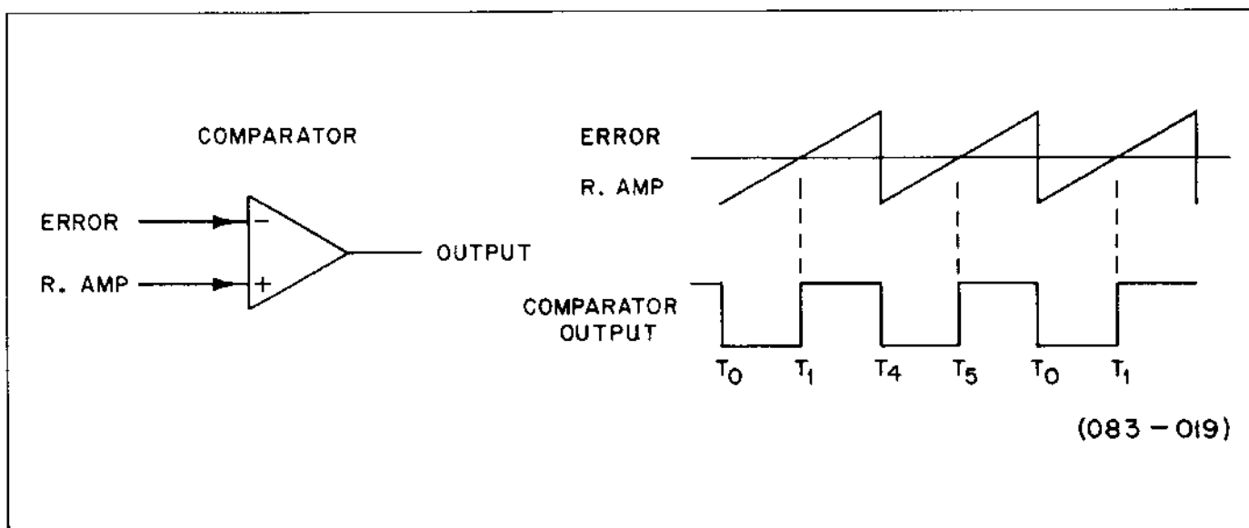
Figure 2-49. LHR Control Module Timing Diagram (SG3524)
