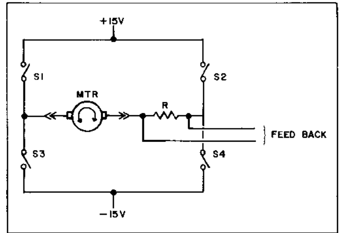
Figure 2-26. Simplified Diagram, Carriage Power Amplifier
