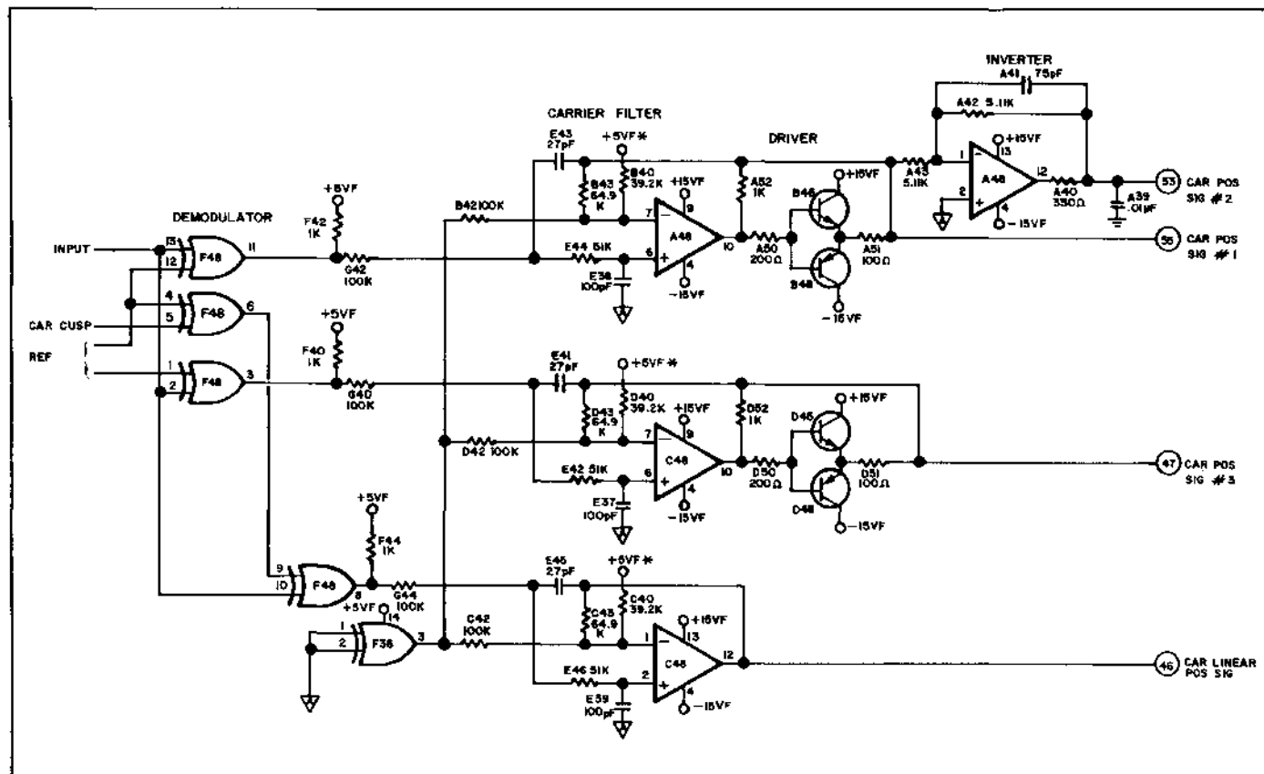
Figure 2-23. Servo Feedback Demodulator/Integrator/Amplifier
