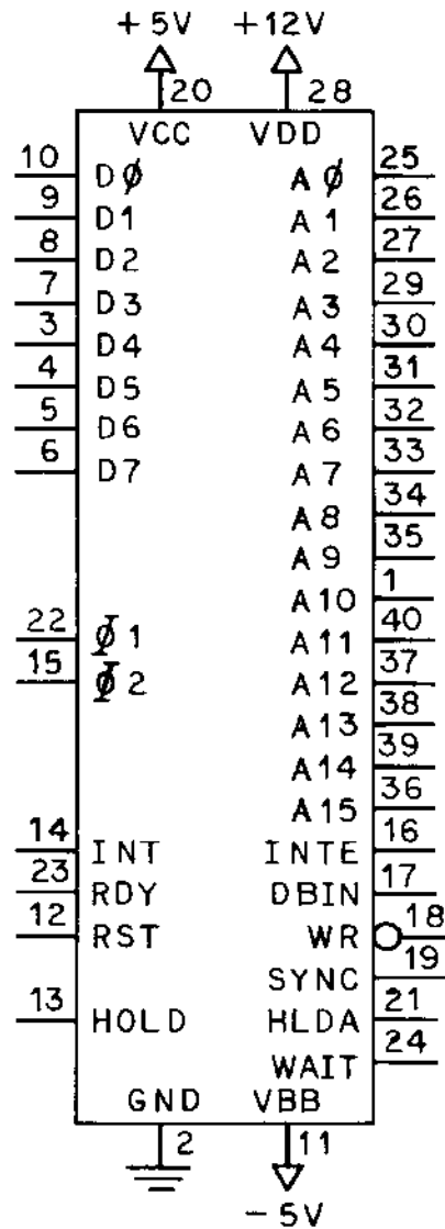
Logic Symbol
