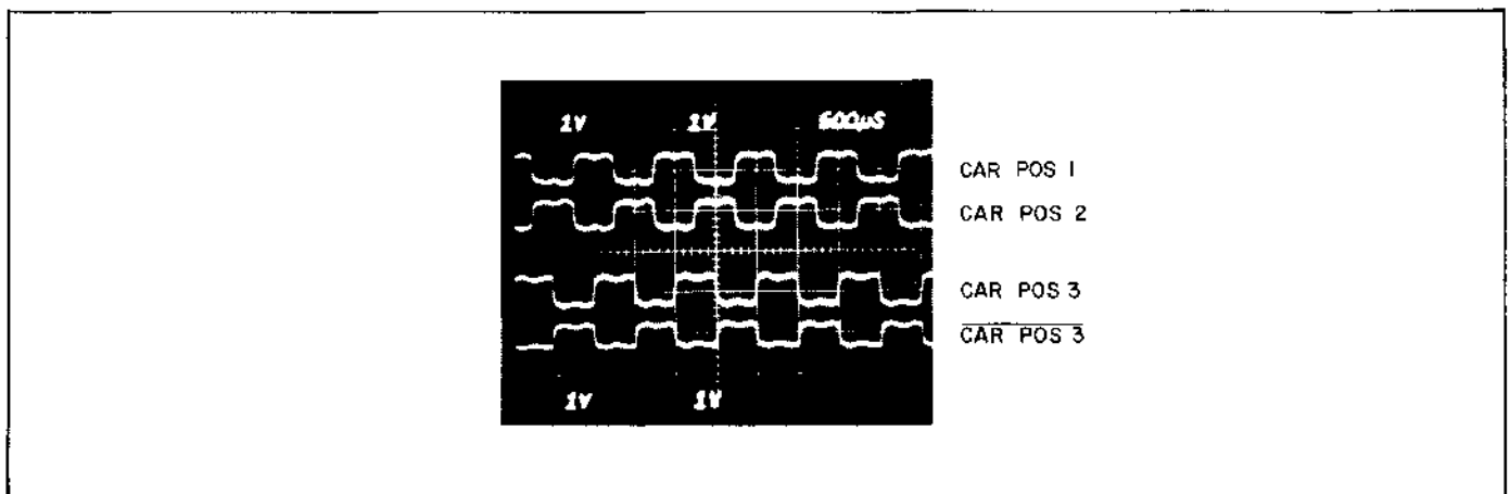
Figure 2-18. CAR POS FET Input Waveforms
