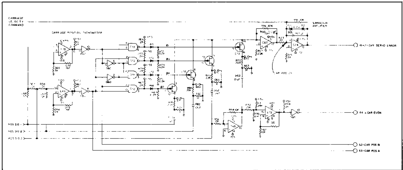
Figure 2-16. Carriage Position Tachometer Circuit
