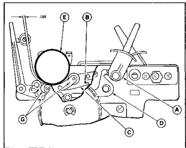
Figure 3-19. Paper Feed Adjustments
