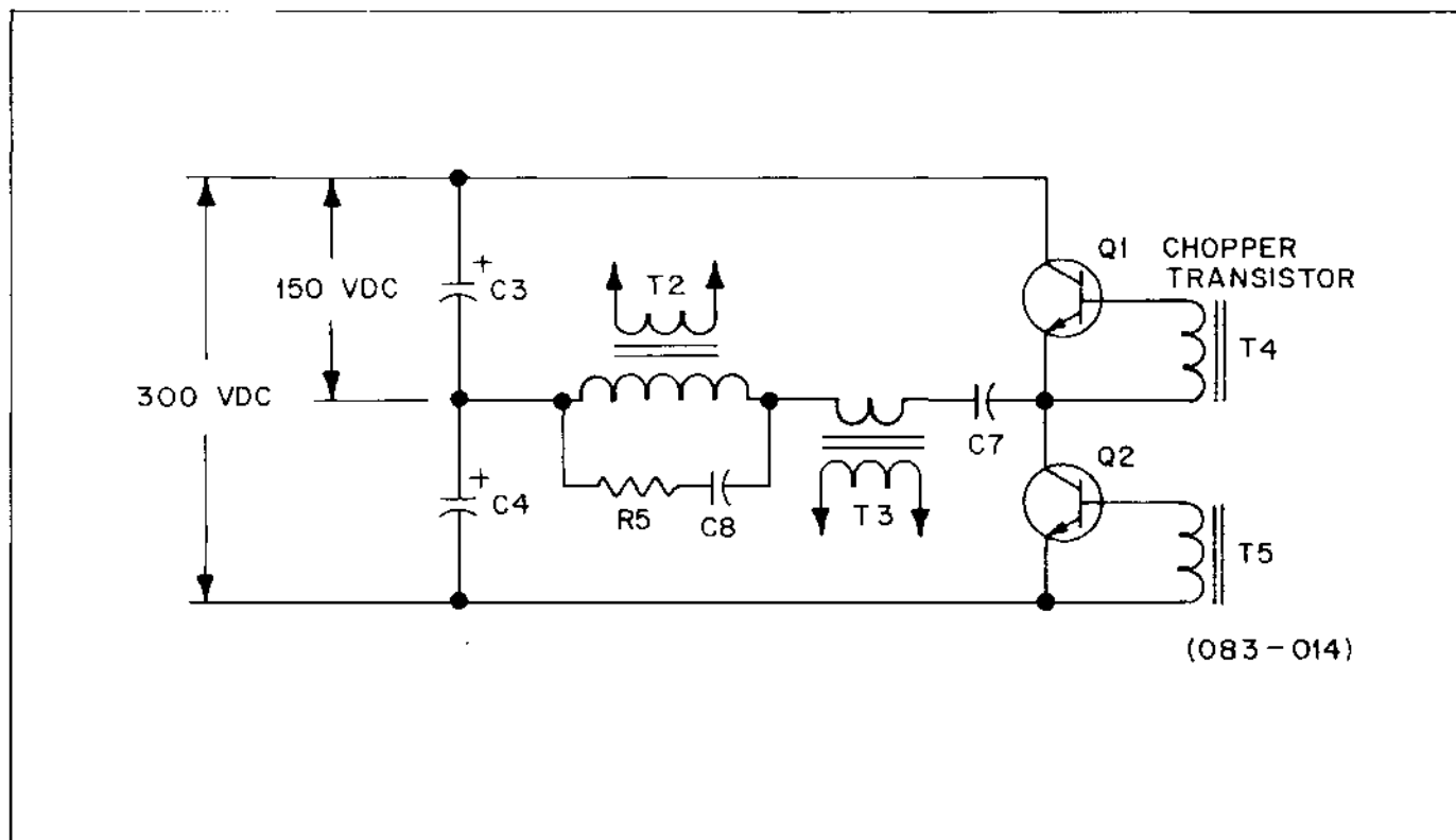
Figure 2-46. LHR Simplified Transistor Chopper (Half-Wave)
