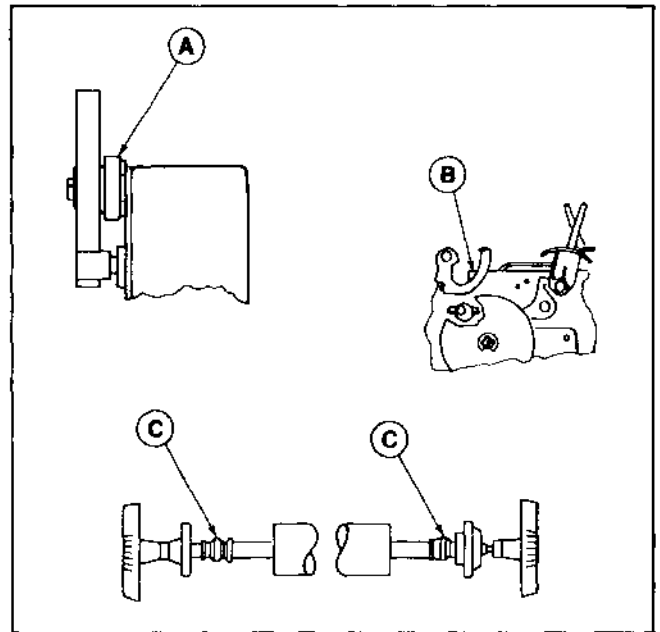
Figure 3-3. Platen System Lubrication Points
