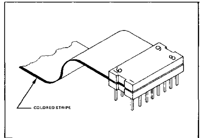
Figure 3-37. Control Panel Cable Pin Numbering
