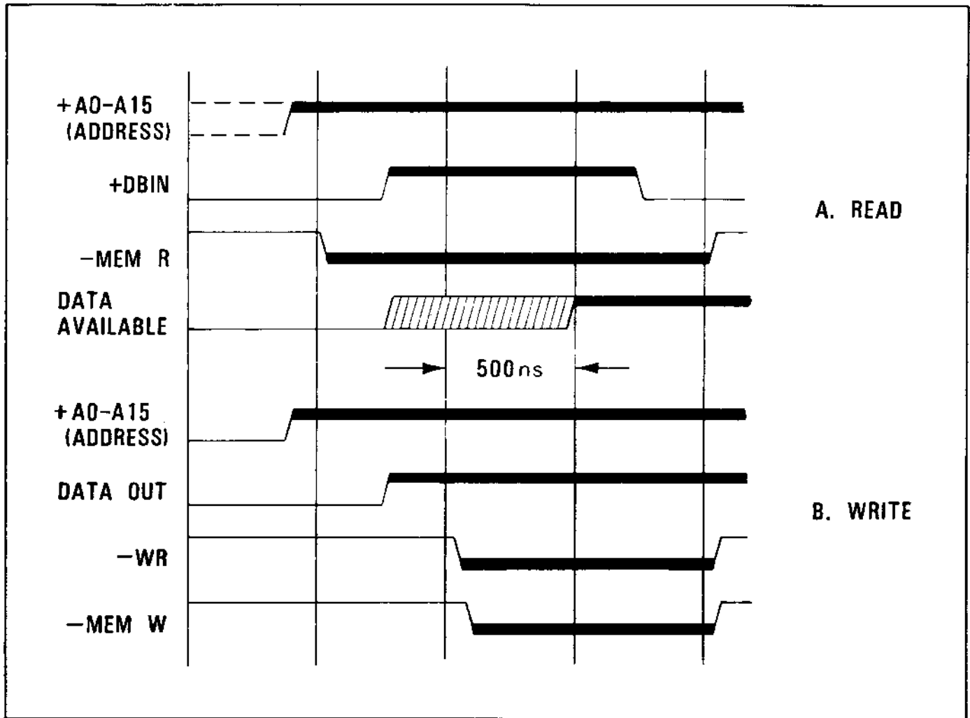
Figure 2-6. Memory Timing
