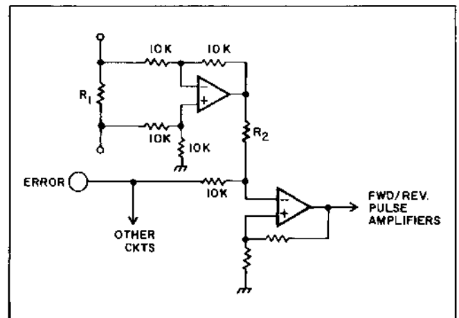
Figure 2-27. Servo Feedback Circuit
