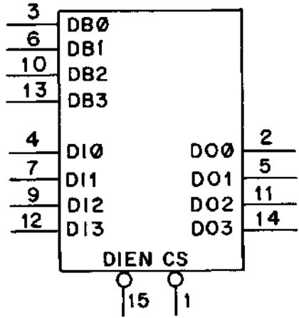
Logic Symbol
