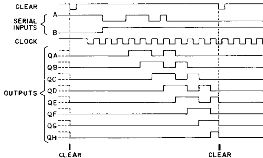
Timing Waveforms
