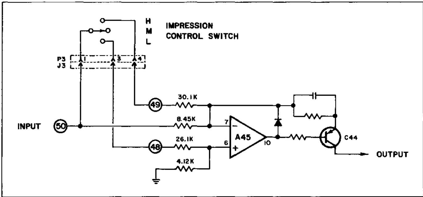
Figure 2-31. Hammer Energy Control Circuit
