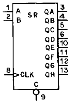
Logic Symbol
