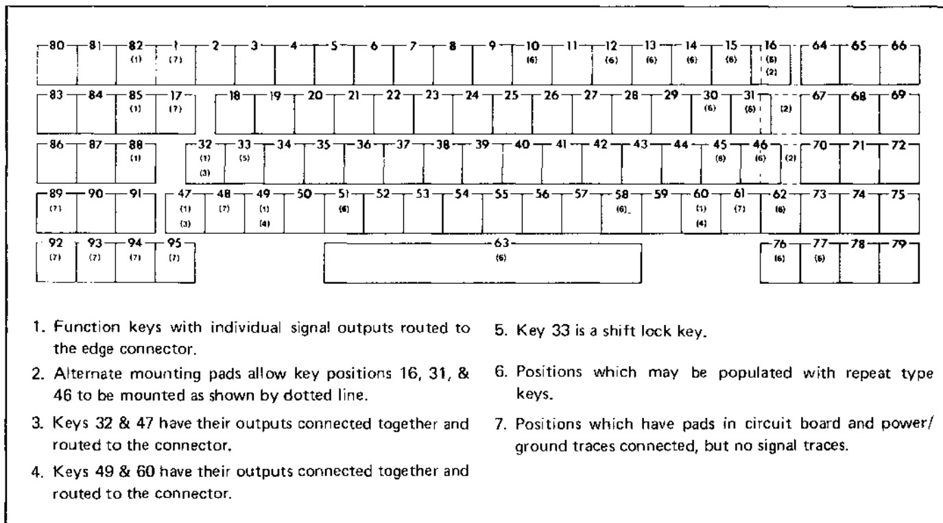
Figure 2-36. Key Positions of Hall-Effect and Saturable-Core Keyboards
