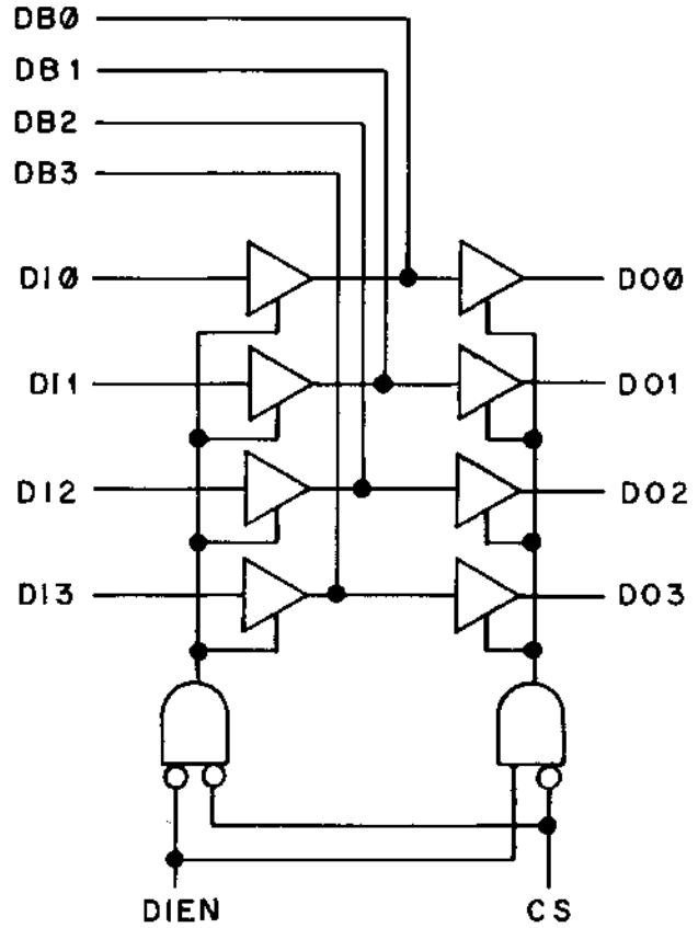
Logic Diagram
