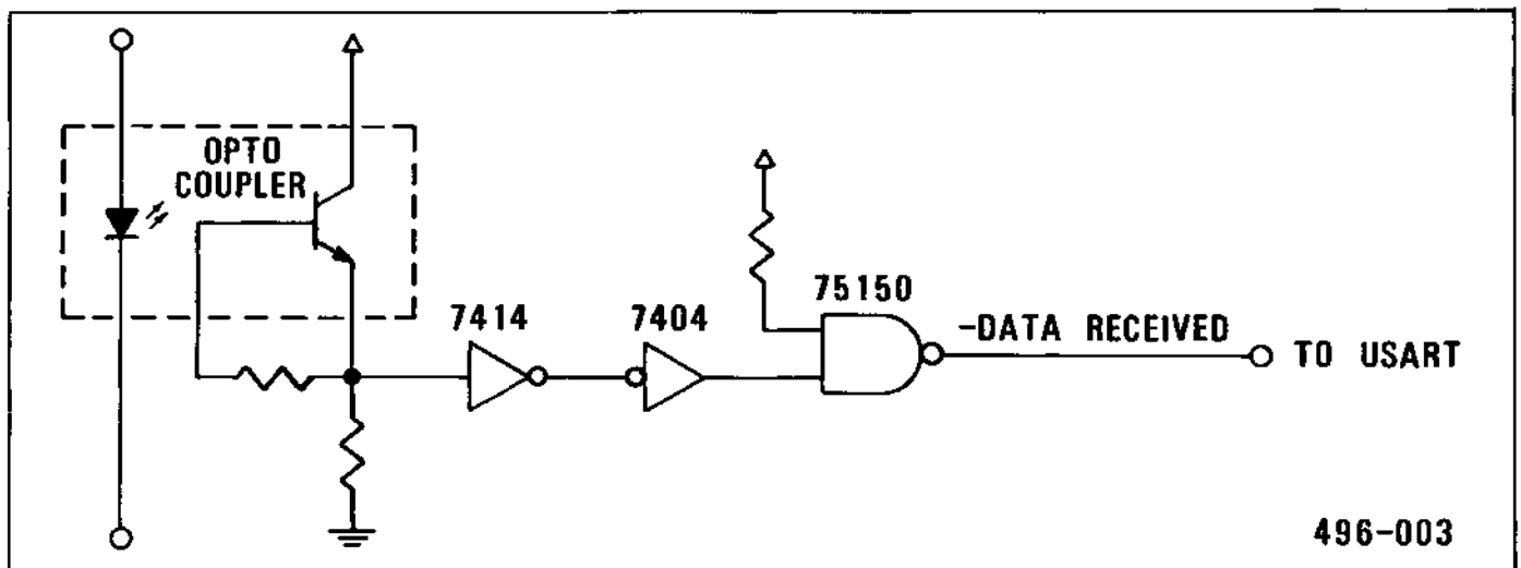
Figure 2-33. Receiver Circuit
