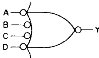
Alternate Symbol
