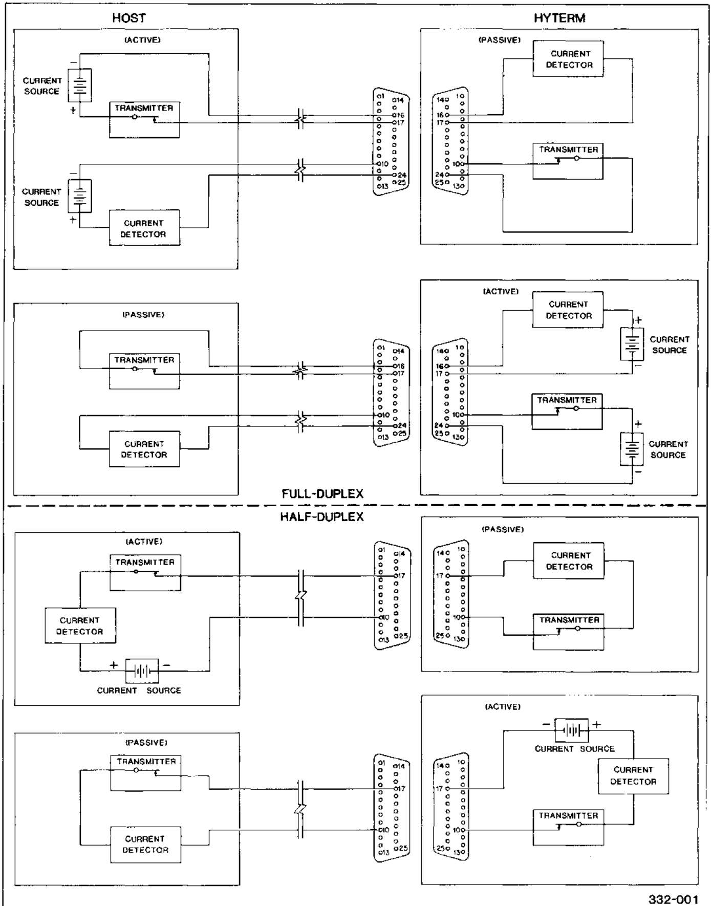
Figure 3-5. Current Loop Connections
