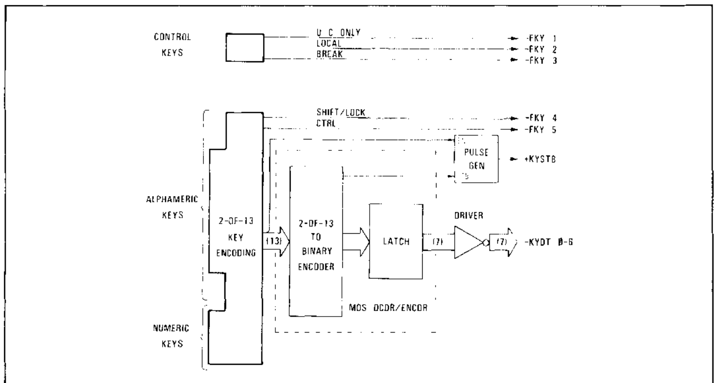
Figure 2-37. Block Diagram Hall-Effect Keyboard
