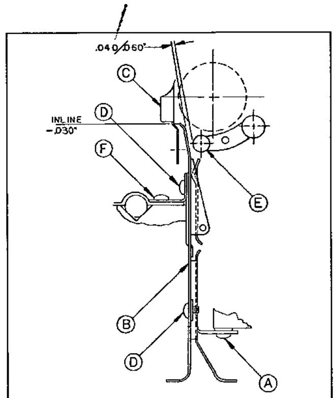
Figure 3-31. Paper Chute Adjustment
