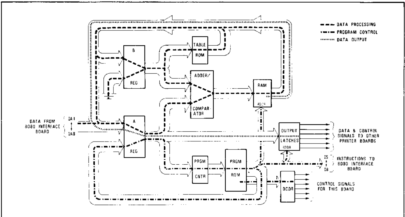
Figure 2-10. Block Diagram, LOGIC-2 Board
