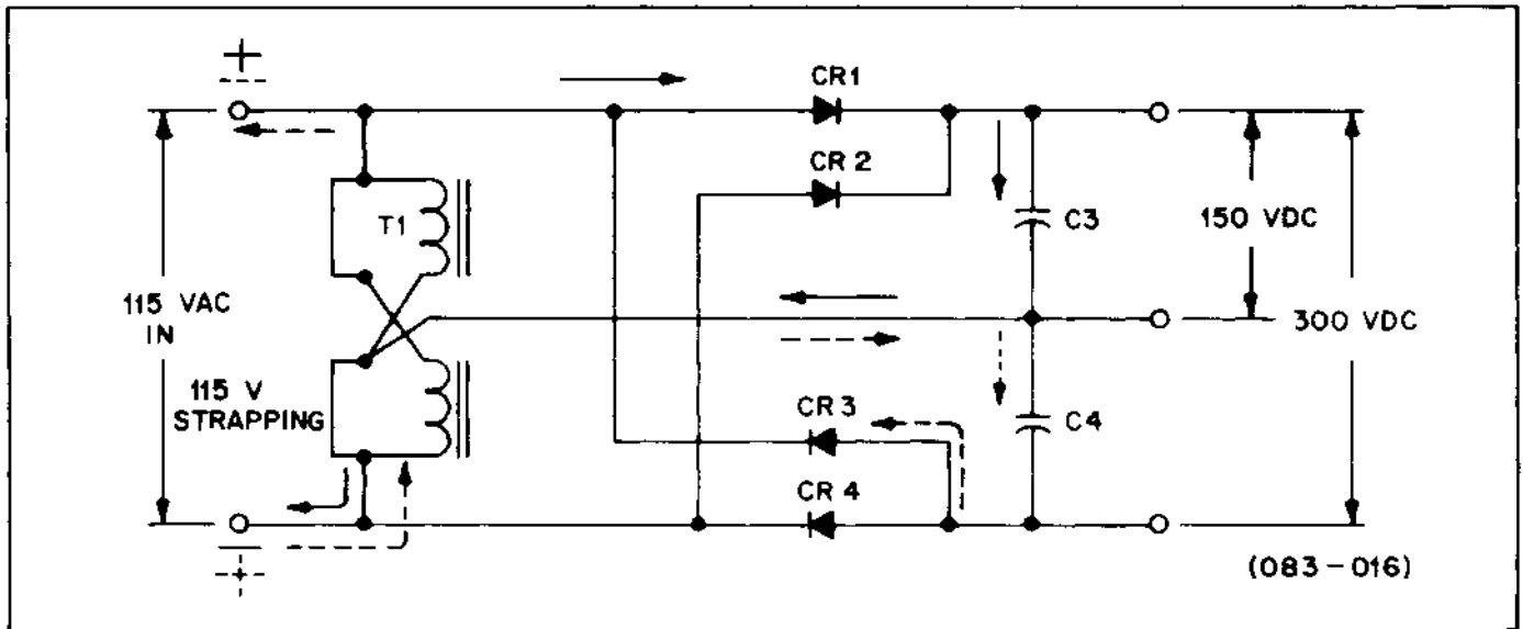
Figure 2-44. LHR Simplified Input Rectifier/Filter Doubler Section (115 VAC Input Strapping)
