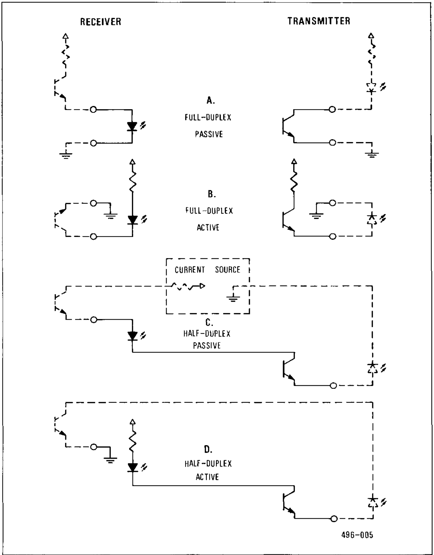
Figure 2-35. Current Loop Operation
