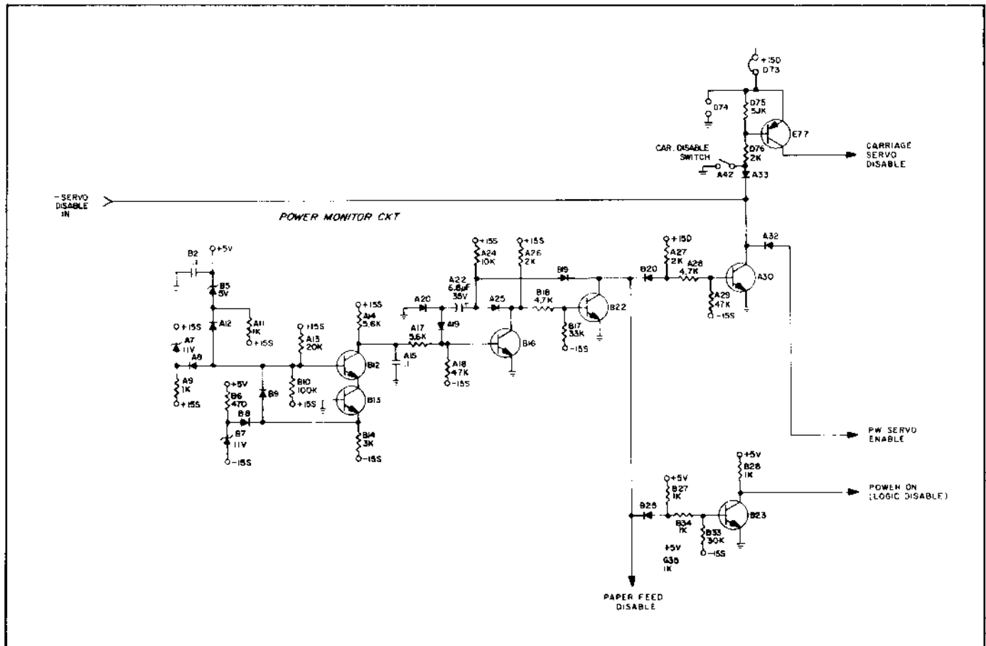
Figure 2-28. Power Monitor Circuit
