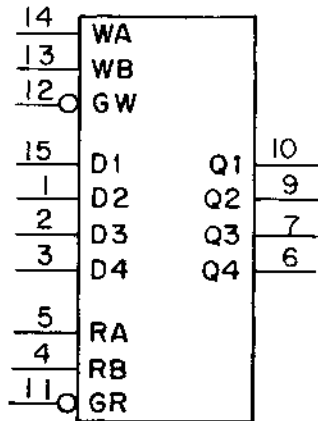
Logic Symbol
