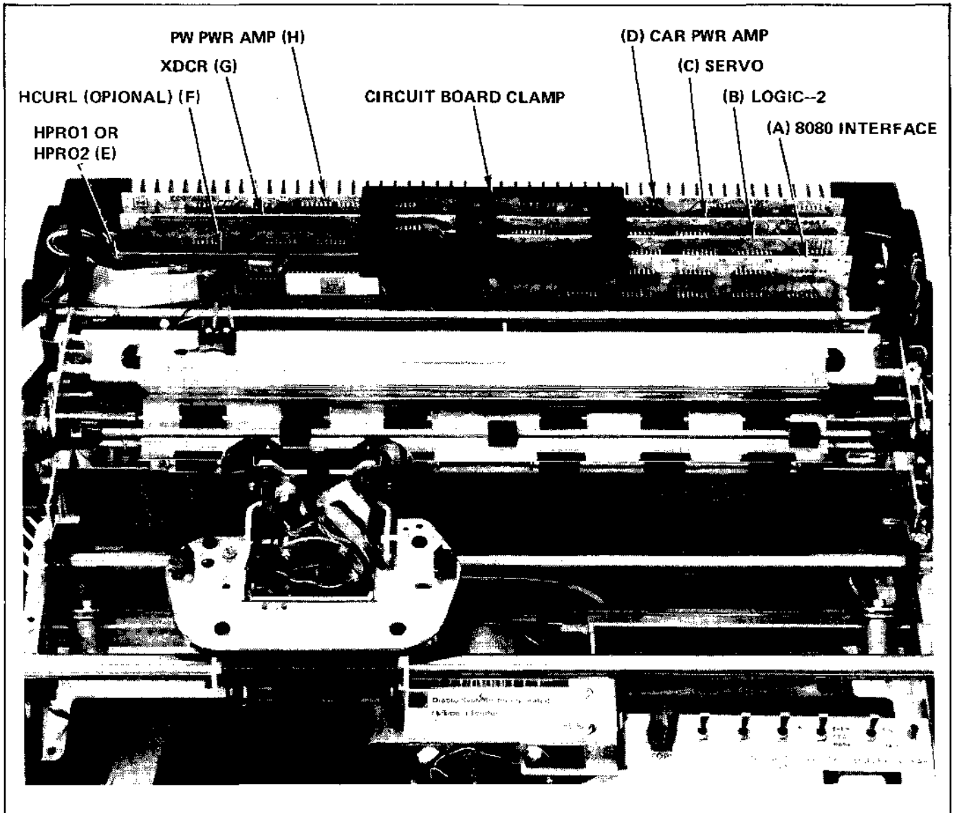
Figure 3-4. Circuit Board Location
