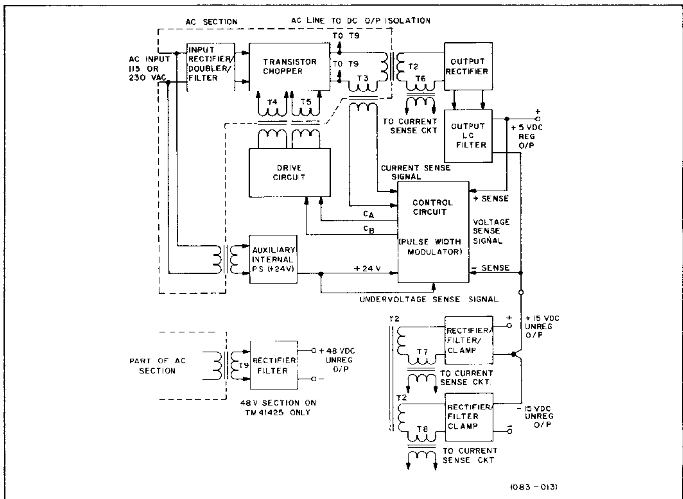
Figure 2-43. Block Diagram, LHR Power Supply
