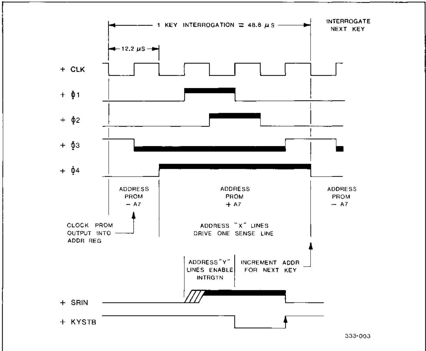
Figure 2-40. Timing Cycle, Cortron Keyboard
