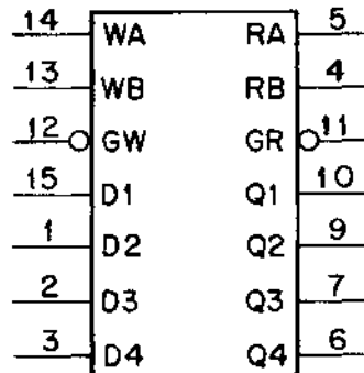
Alternate Symbol
