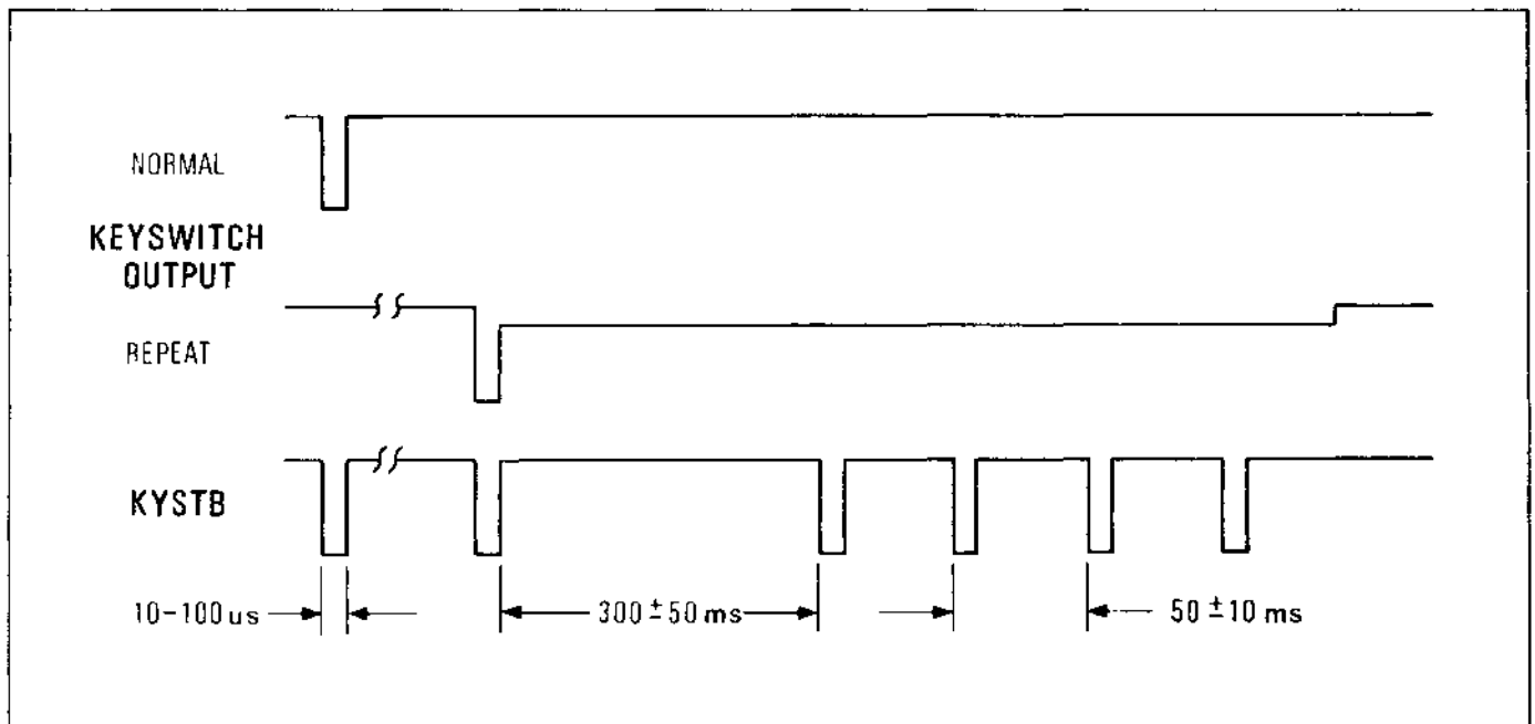
Figure 2-38. Keyboard Strobe Generation
