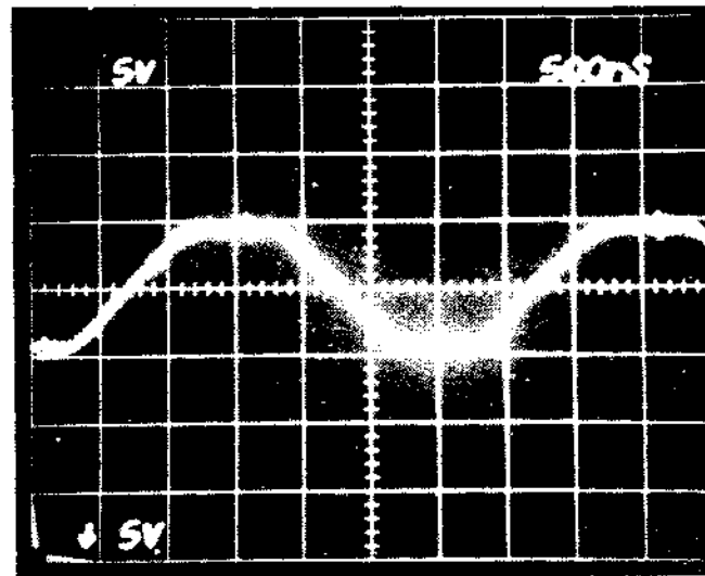
Figure 2-22. Servo Feedback Amplifier Waveforms
