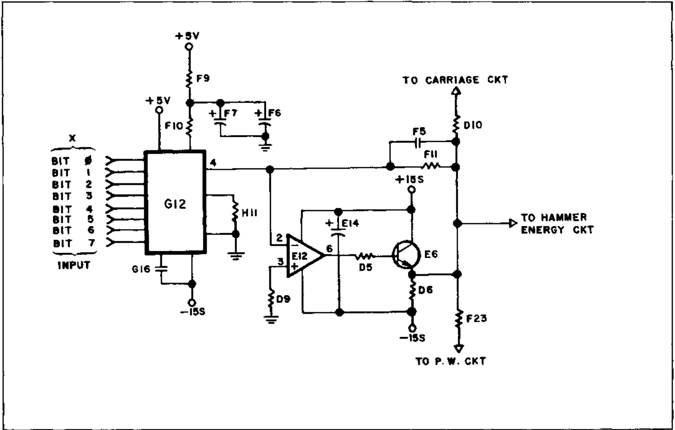
Figure 2-14. D-A Converter
