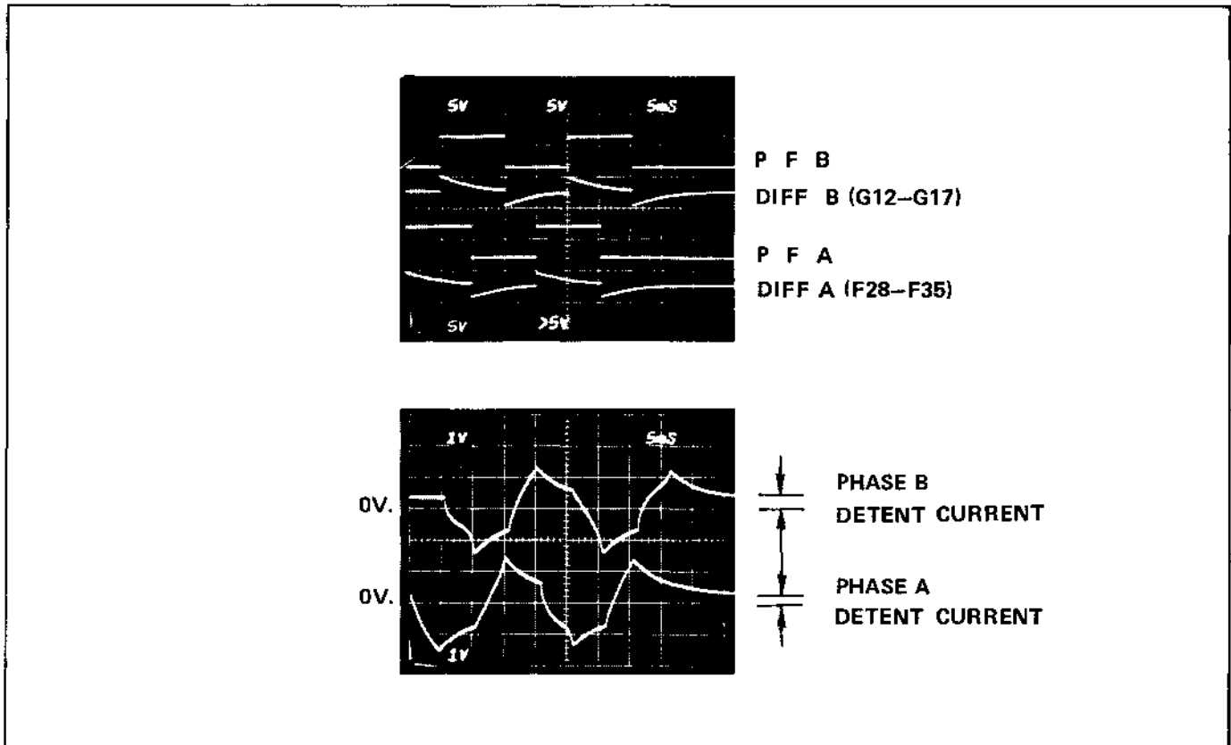
Figure 2-30. Paper Feed Drive Waveforms
