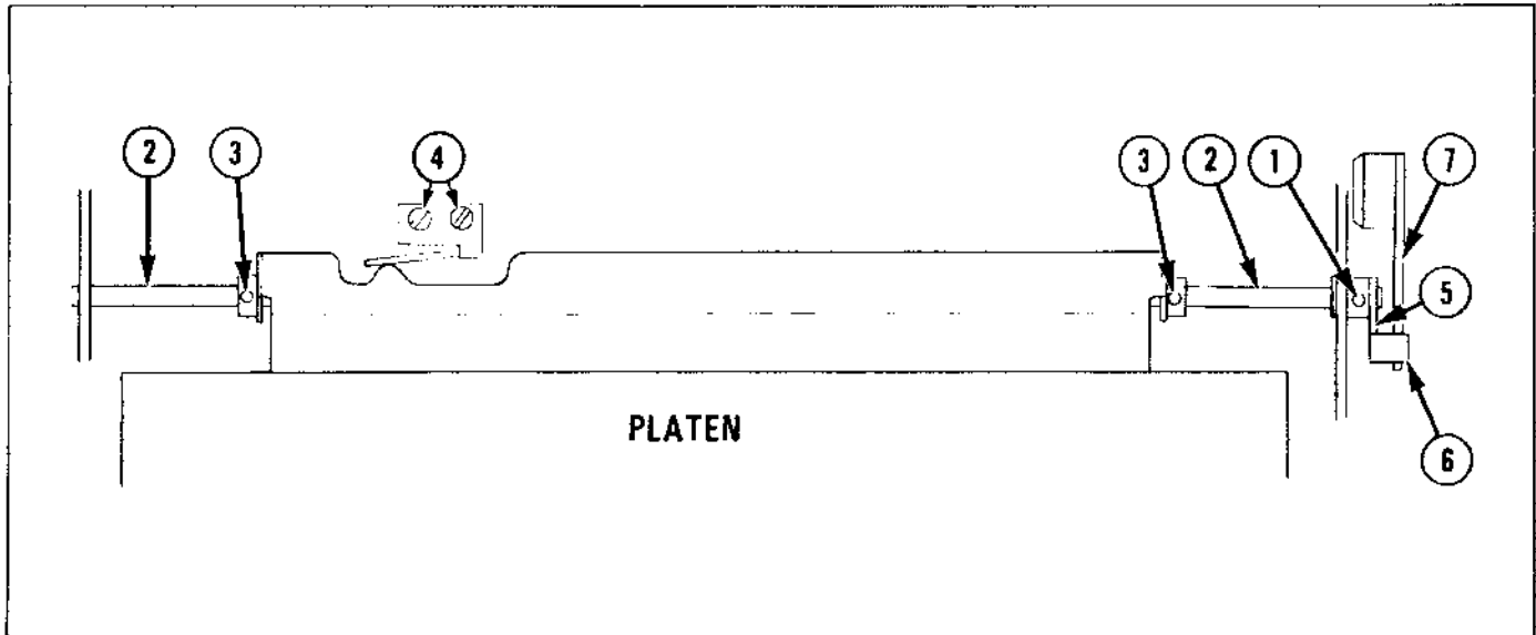
Figure 3-32. Paper-Out Switch Adjustment
