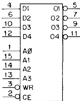
Logic Symbol
