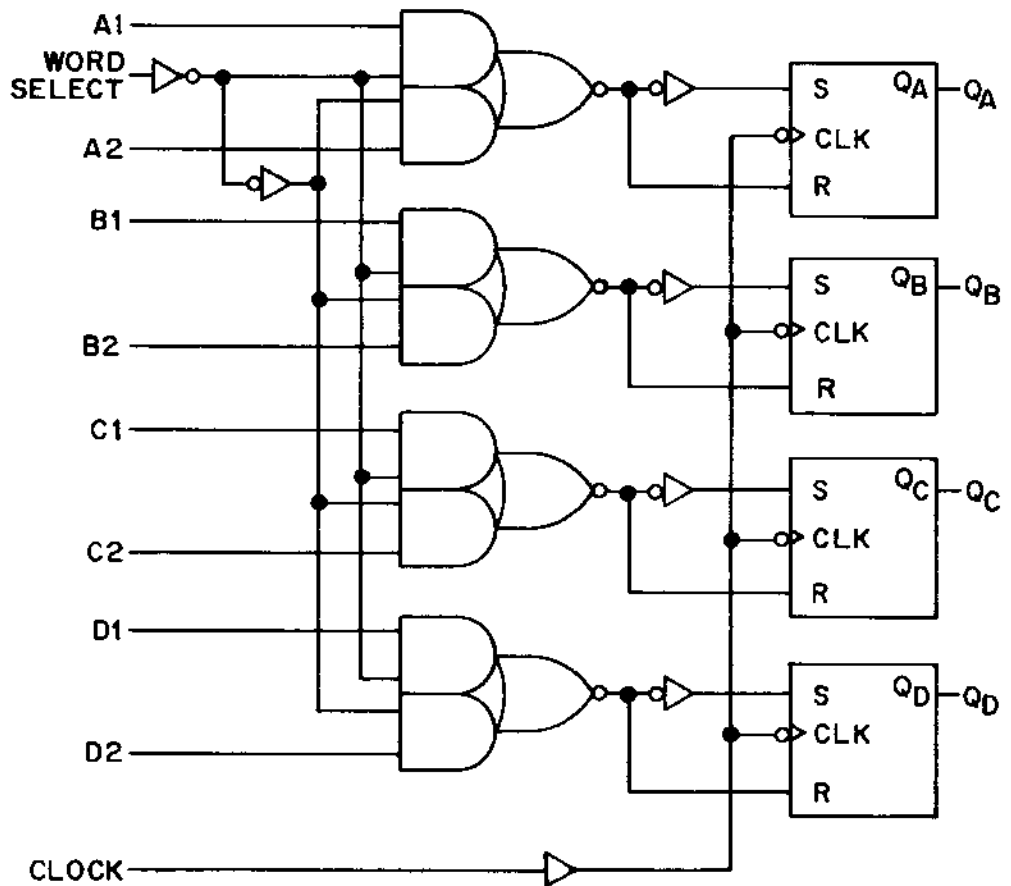
Logic Diagram
