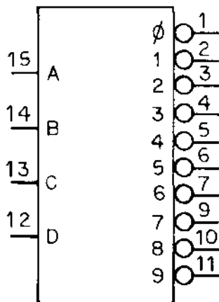
Logic Symbol
