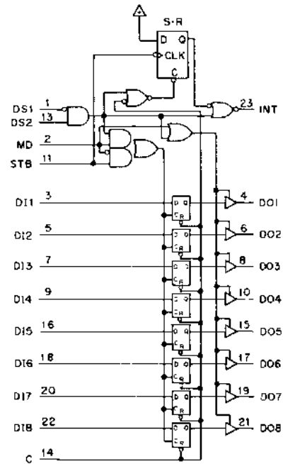
Logic Diagram
