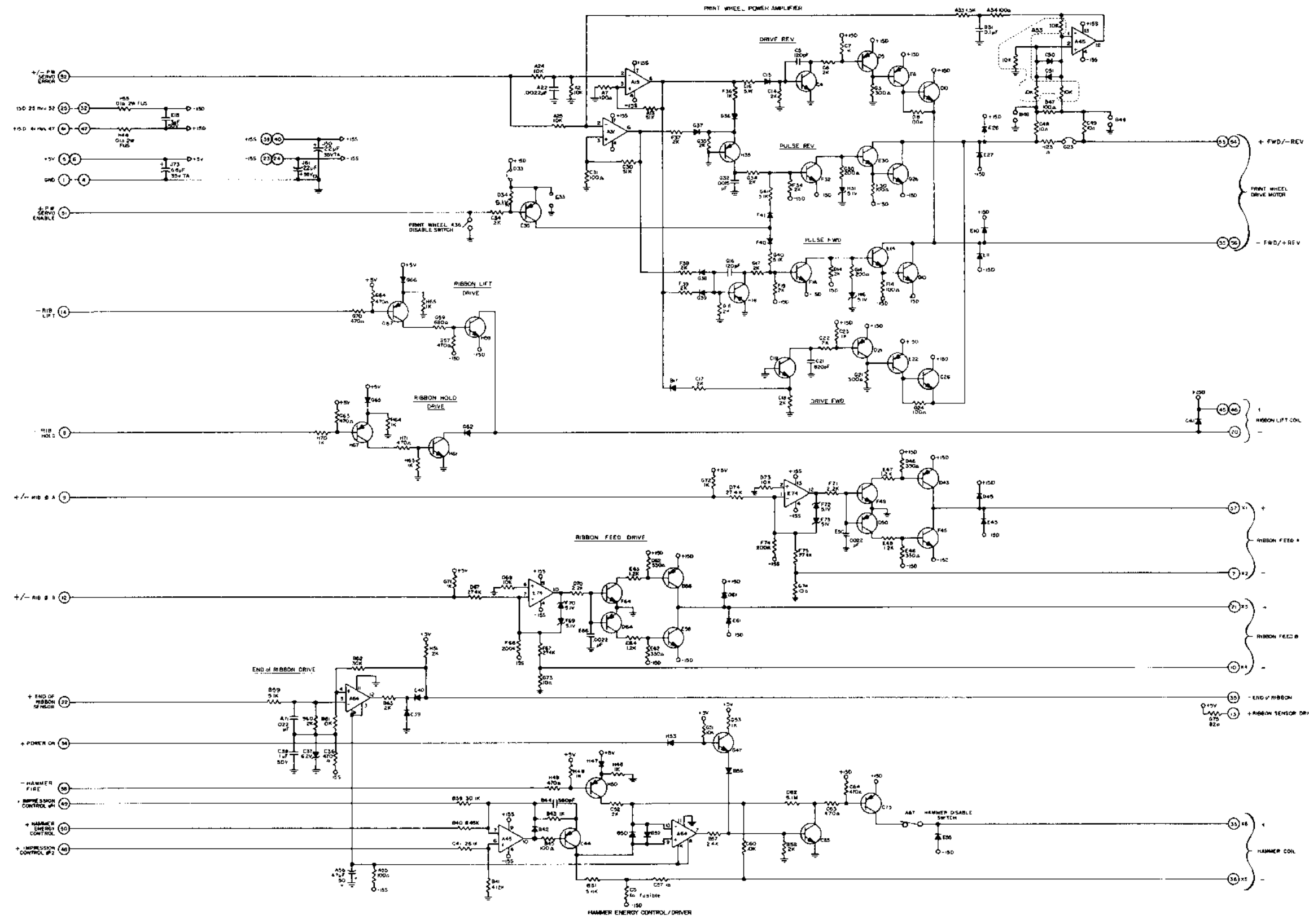
PW PWR AMP 40530-08 REV. C
