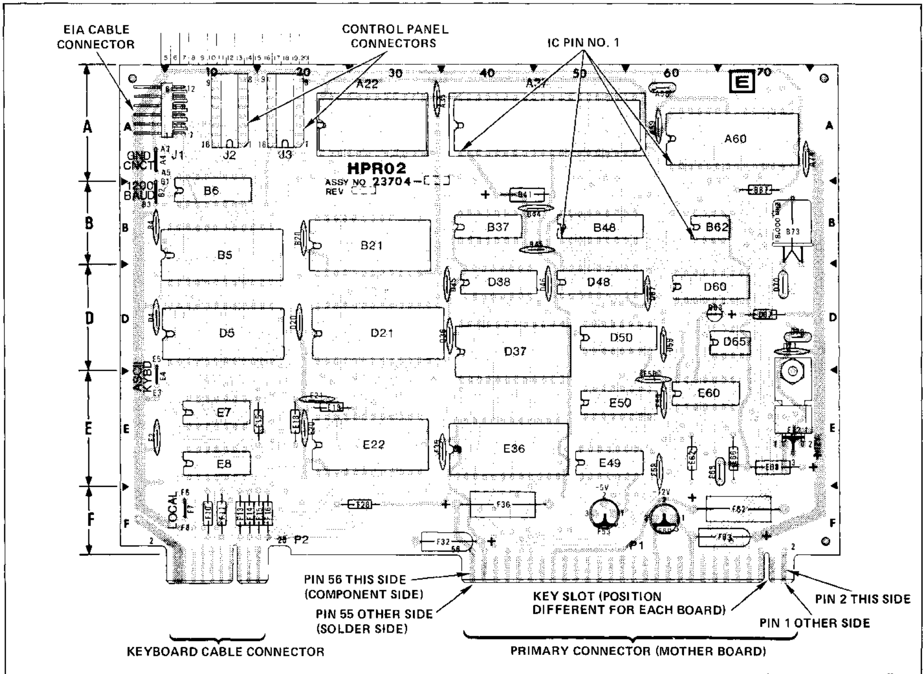
Figure 3-33. Circuit Board Component Location and Pin Numbering
