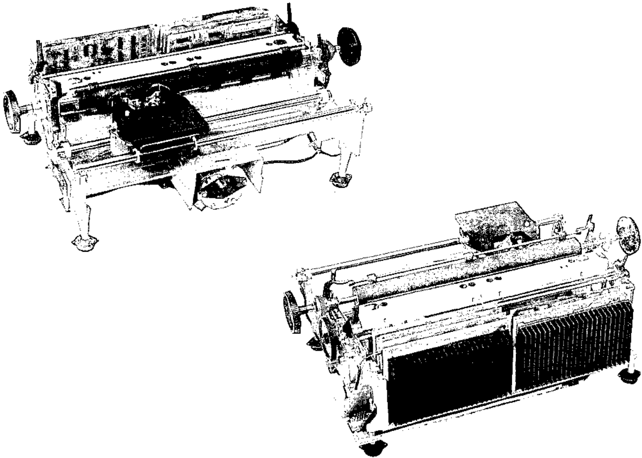
Figure 1-1. SERIES 1300 HYTYPE II PRINTER
