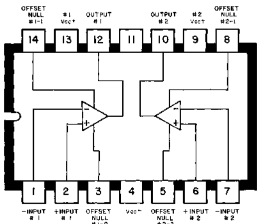
SCHEMATIC (each amplifier)
