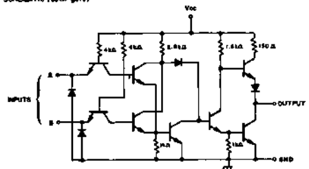
SCHEMATIC (each gate)
