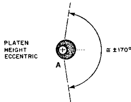
Figure 5-26 PLATEN HEIGHT ECCENTRICS ADJUSTMENT LIMITS
