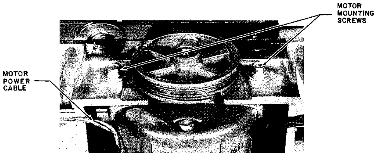
Figure 5-34 CARRIAGE SERVO MOTOR MOUNTING SCREWS
