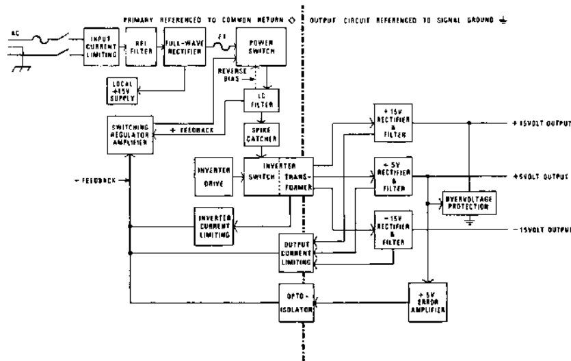
Figure 4-31 OPTIONAL INTERNAL POWER SUPPLY BLOCK DIAGRAM (B)
