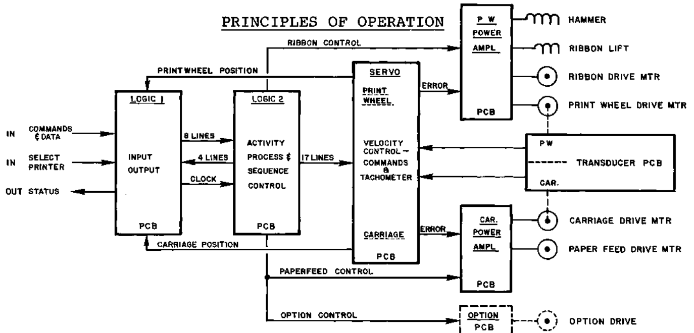
Figure 4-1 HyTYPE II PRINTER BLOCK DIAGRAM
