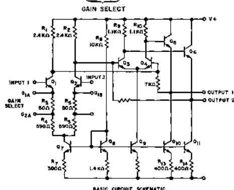
DIFFERENTIAL AMPLIFIER 733 / N5733C / LM733CN
