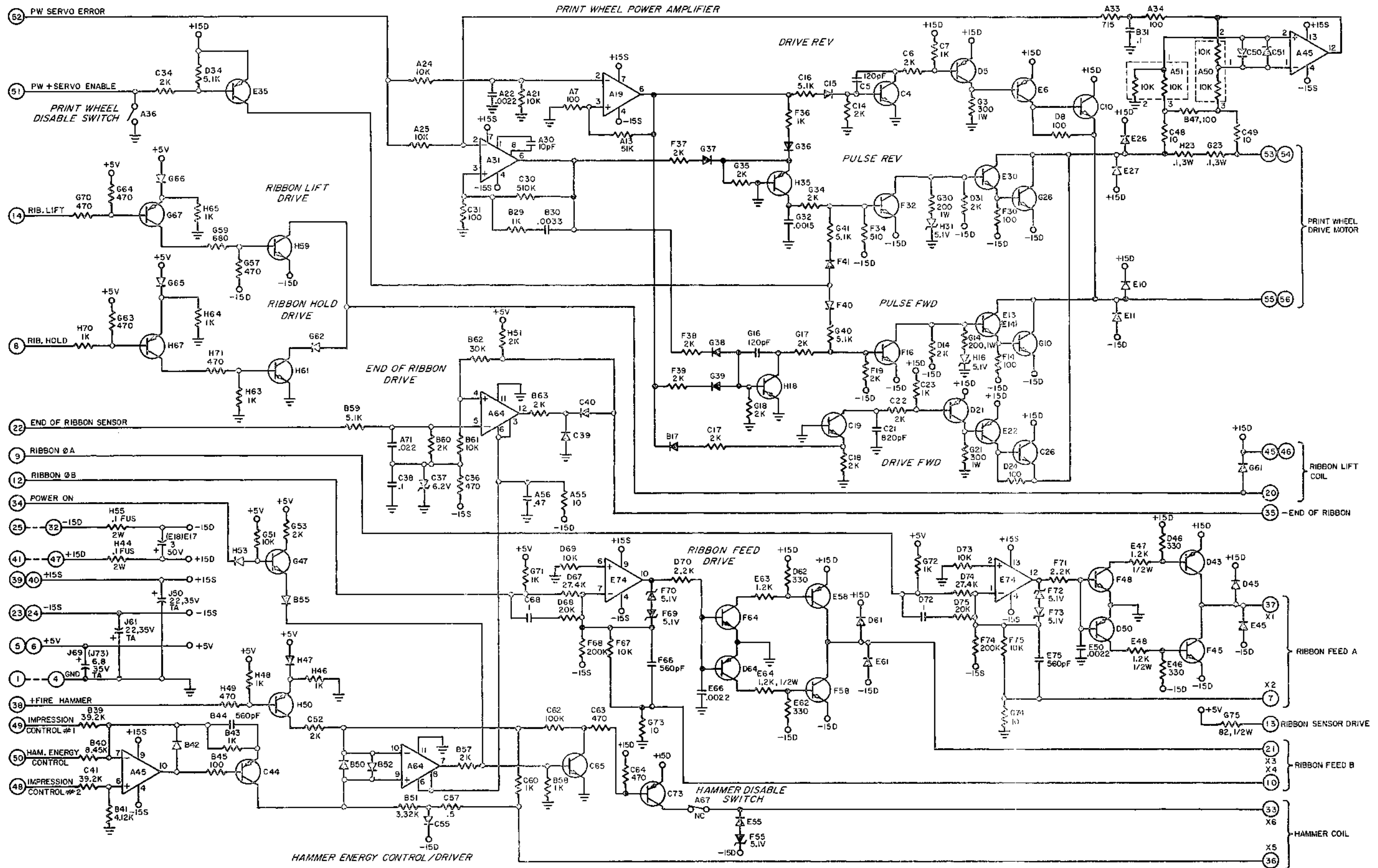
Figure 7-7b P W Power Amp PCB Assy, 1355 #40730-10 Rev B
