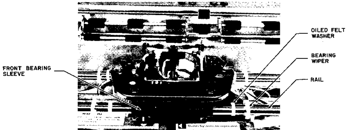
Figure 5-19 CARRIAGE AND RAIL REASSEMBLY
