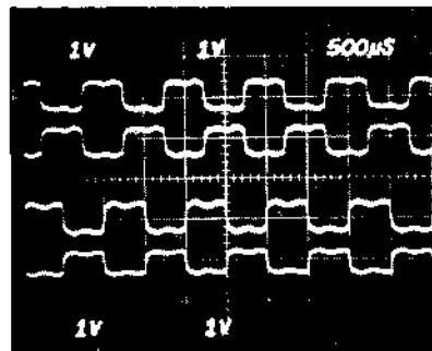
Figure 4-20 CAR. POS FET INPUT WAVEFORMS
