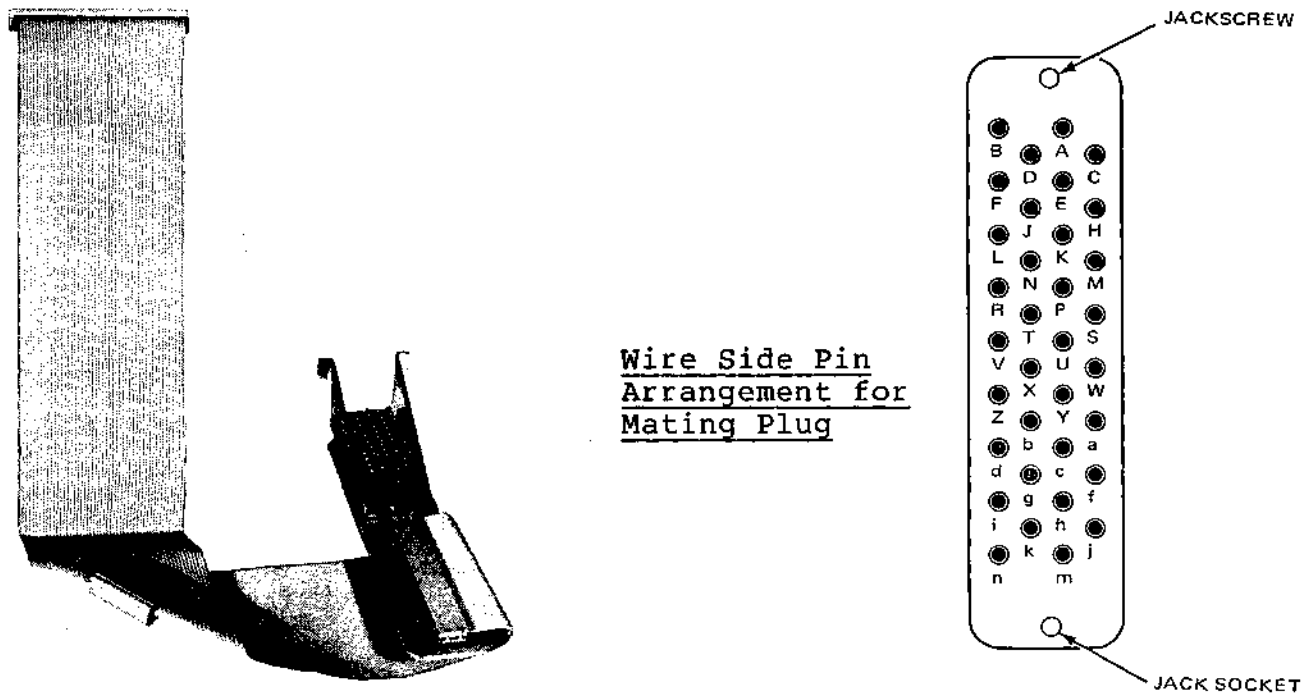
Figure 2-12 HyTYPE II to HyTYPE I ADAPTER CABLE
