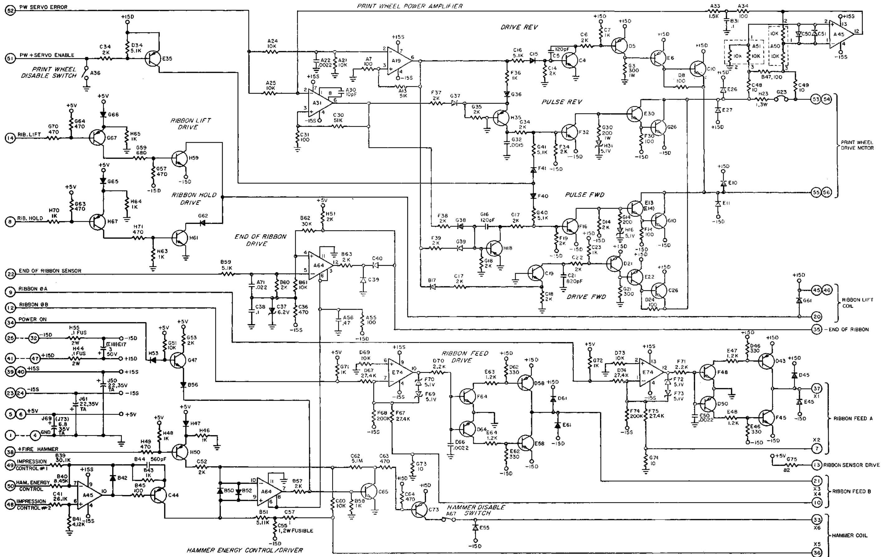
Figure 7-7a P W Power Amp PCB Assy, Standard #40530-10 Rev B
