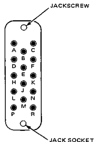
Figure 2-10 POWER CONNECTOR PIN ARRANGEMENT (wire side)
