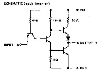
HEX INVERTER 7404 / DM7404N / SN7404N
