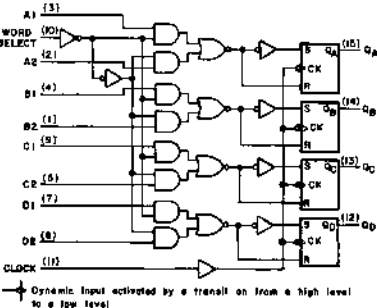
QUAD 2-INPUT MULTIPLEXER WITH STORAGE 74298 / SN74298N
