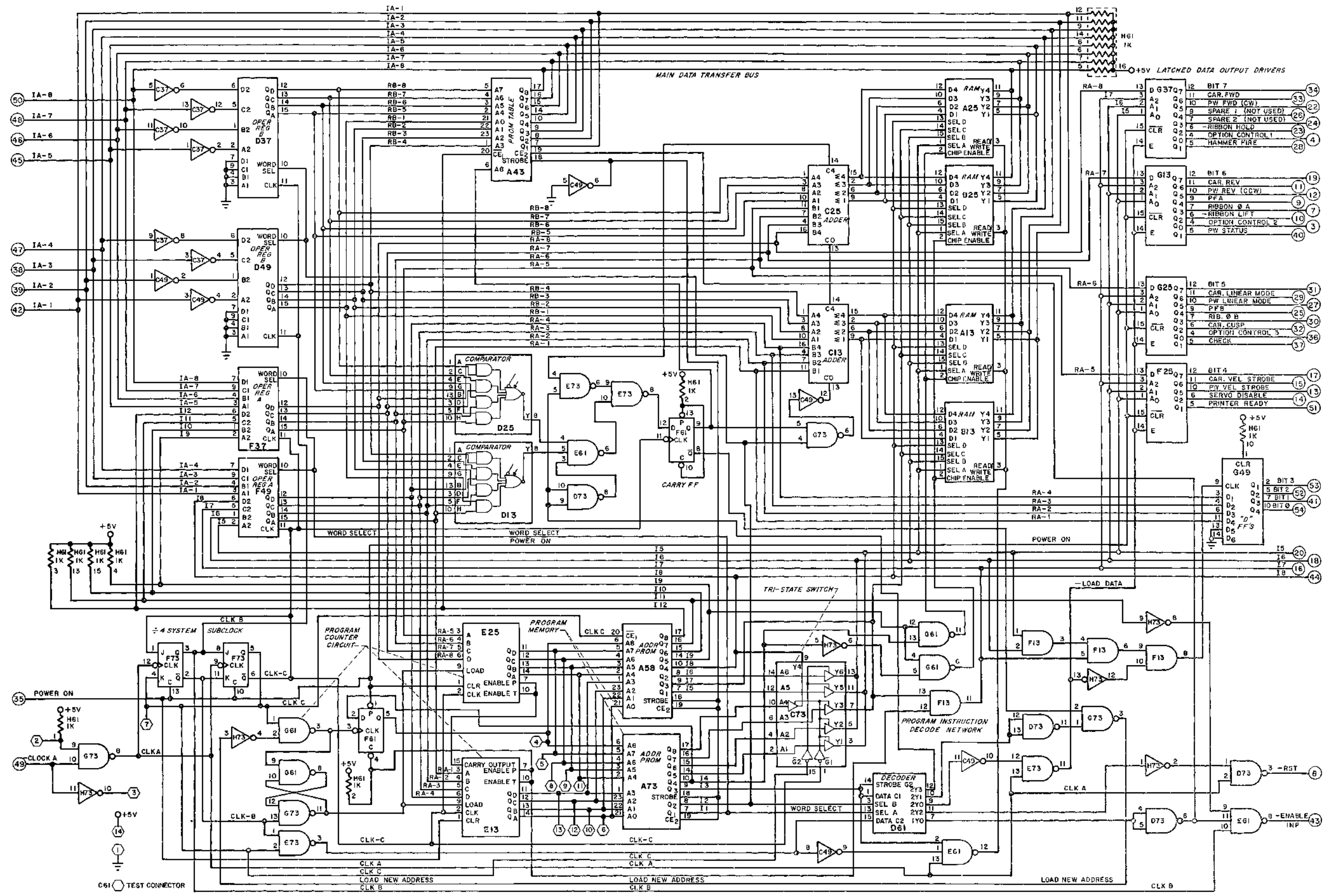
Figure 7-3a Logic #2 PCB Assy, Standard #40510-XX Rev AJ
