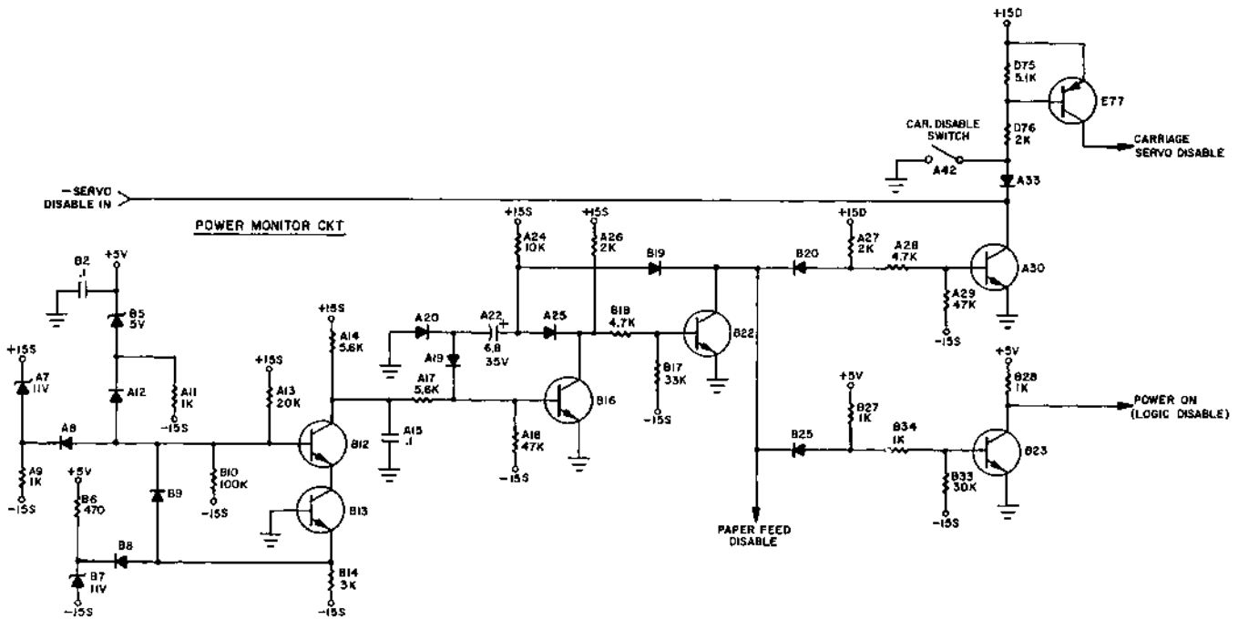
Figure 4-24 POWER MONITOR CIRCUIT
