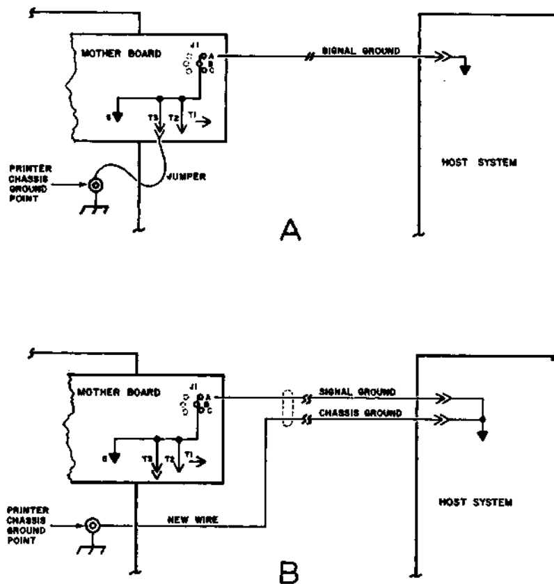
Figure 2-9 NOISE IMMUNITY GROUNDING
