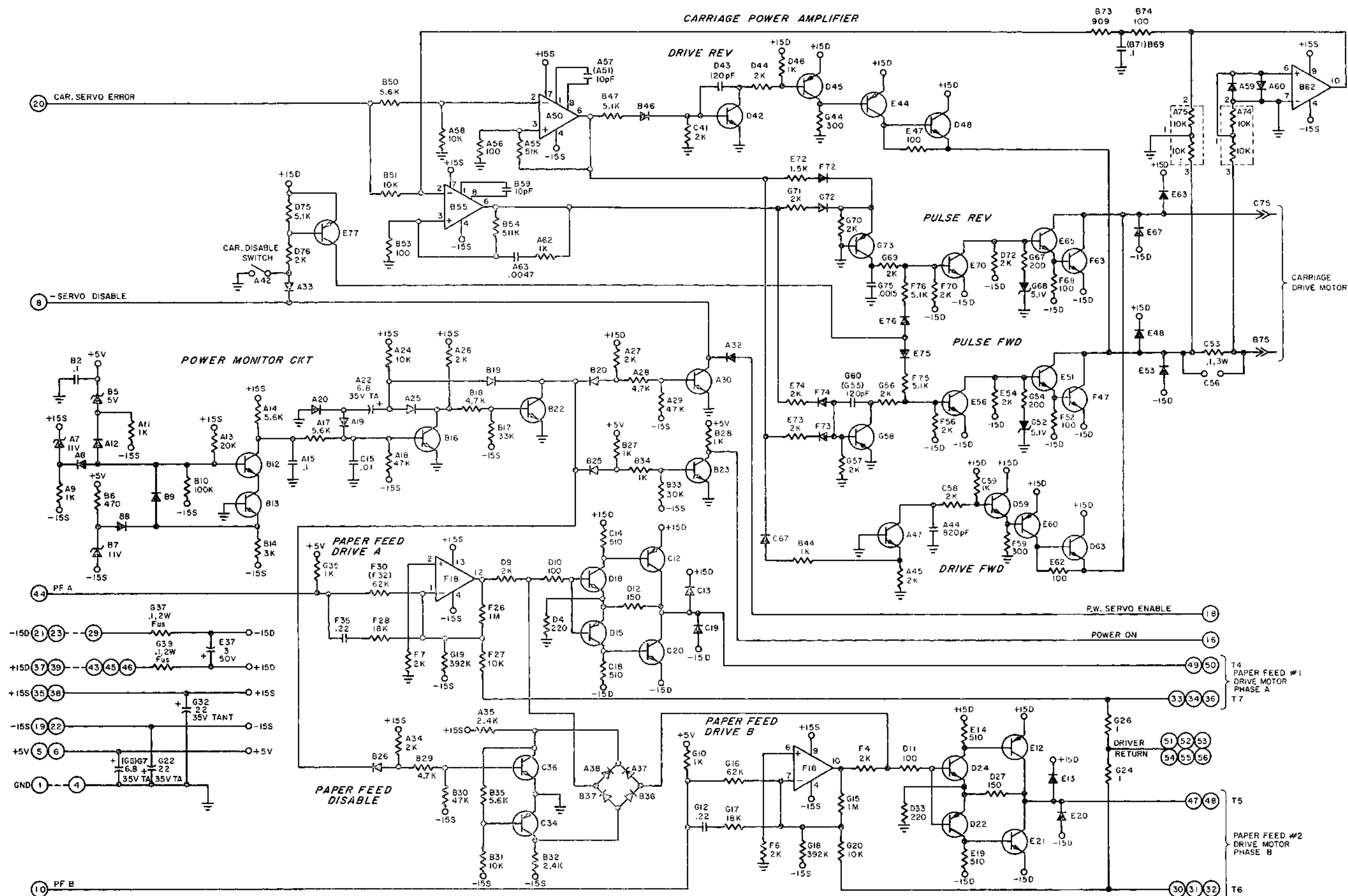
Figure 7-6a Car. Power Amp PCB Assy, Standard #40525-10 Rev C
