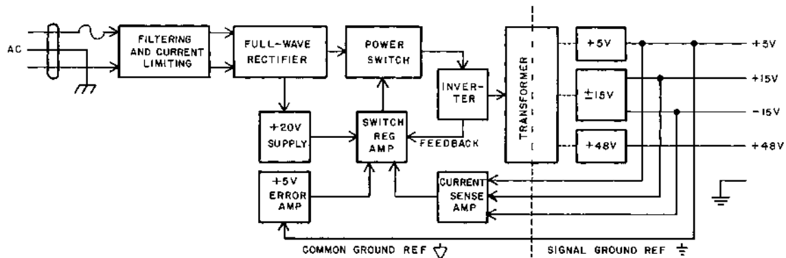
Figure 4-32 OPTIONAL INTERNAL POWER SUPPLY BLOCK DIAGRAM (U)
