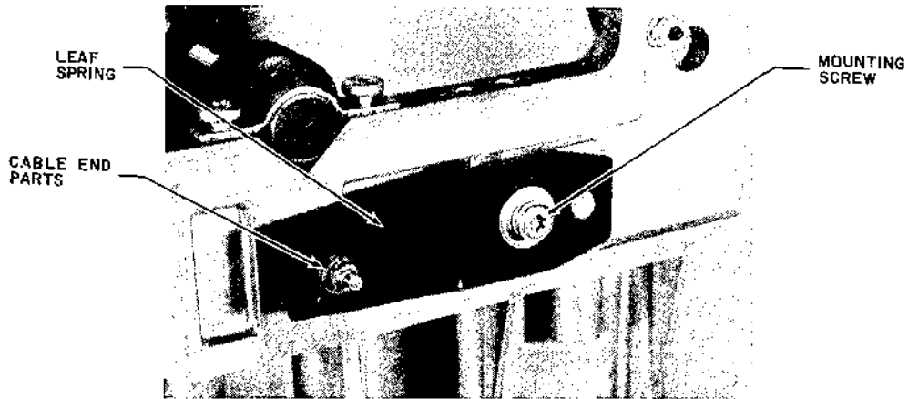
Figure 5-33 DRIVE CABLE TENSION SPRING
