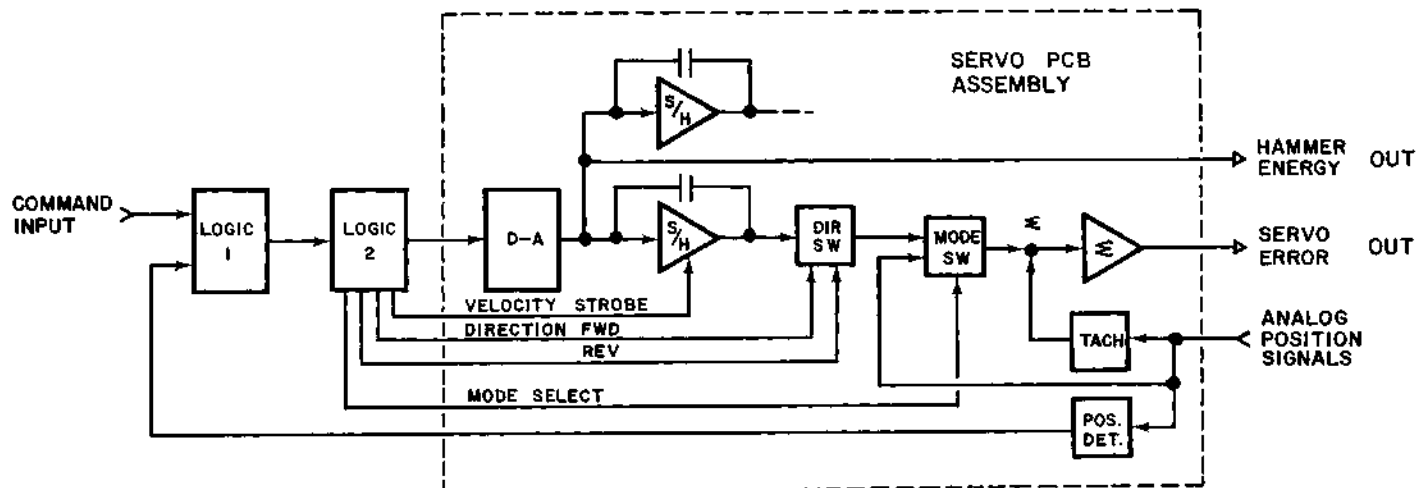
Figure 4-15 SERVO PCB BLOCK DIAGRAM
