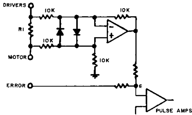
Figure 4-22 FEEDBACK INSTRUMENTATION CIRCUIT
