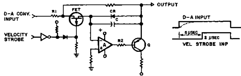
Figure 4-17 TYPICAL SAMPLE AND HOLD CIRCUIT
