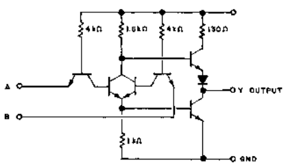
QUADRUPLE 2-INPUT POSITIVE NOR GATES 7402 / SN7402
