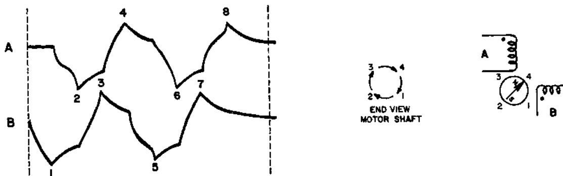
Figure 4-27 TYPICAL STEPPER MOTOR ROTATION
