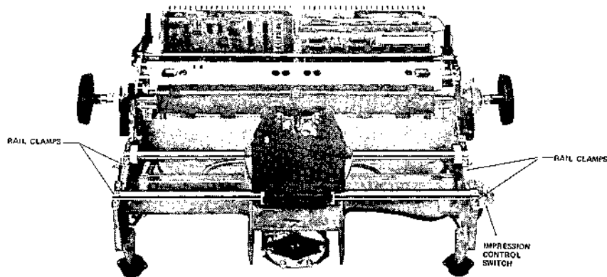
Figure 5-18 CARRIAGE RAIL CLAMPS
