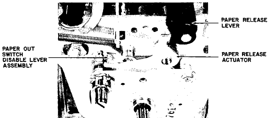
Figure 5-48 TOP PAPER OUT SWITCH DISABLE ASSEMBLY
