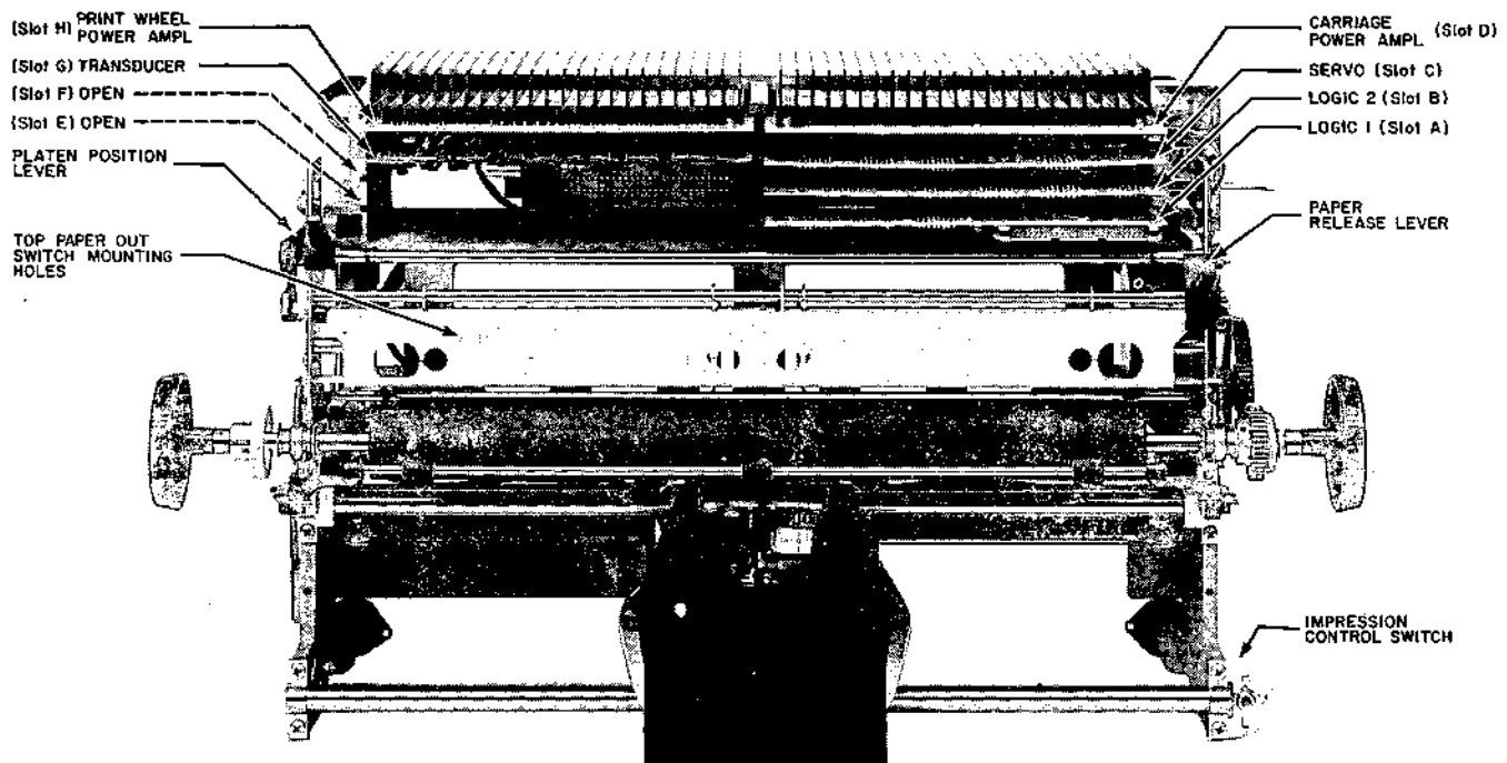
Figure 4-2 COMPONENT LOCATIONS
