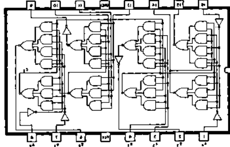
4 BIT BINARY FULL ADDER 7483/N7483B/DM7483N/SN7483A-N 10140
