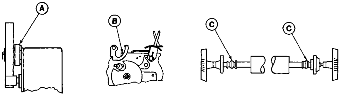
Figure 5-4 PLATEN SYSTEM LUBRICATION POINTS
