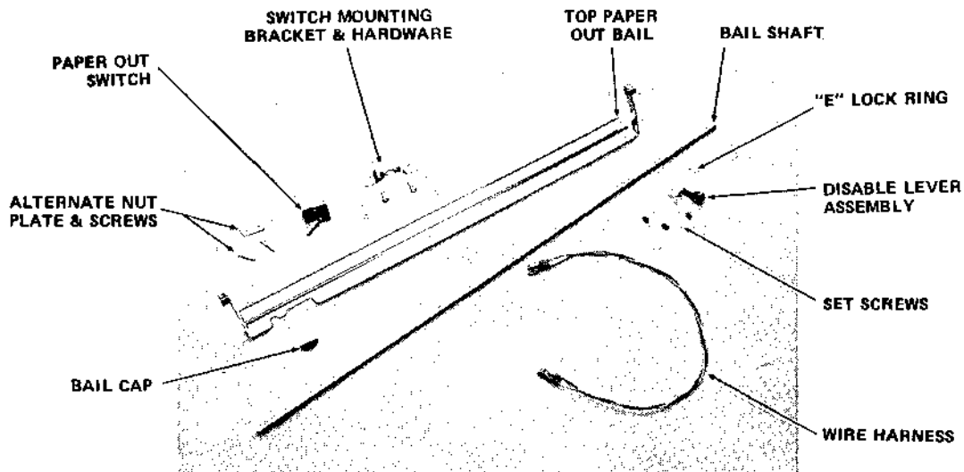
Figure 5-45 TOP FEED PAPER OUT SWITCH ASSEMBLY PARTS
