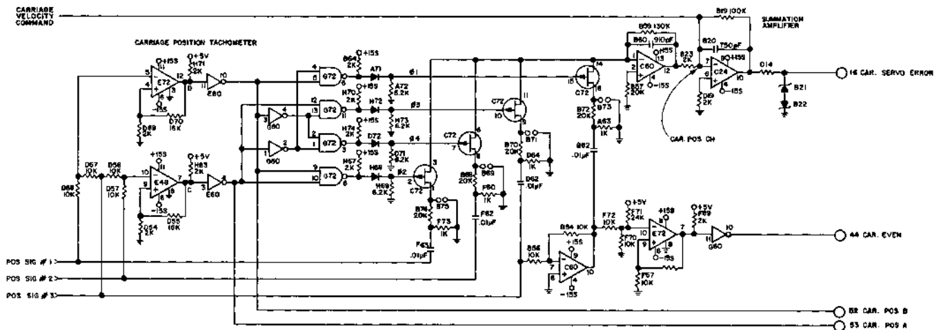
Figure 4-18 CARRIAGE POSITION TACHOMETER CIRCUIT
