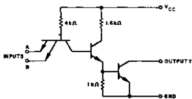
SCHEMATIC (each gate)
