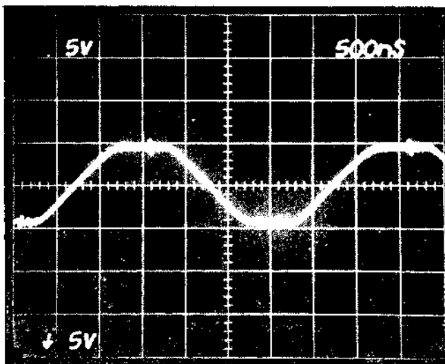
Figure 4-11 SERVO FEEDBACK AMPLIFIER WAVEFORMS
