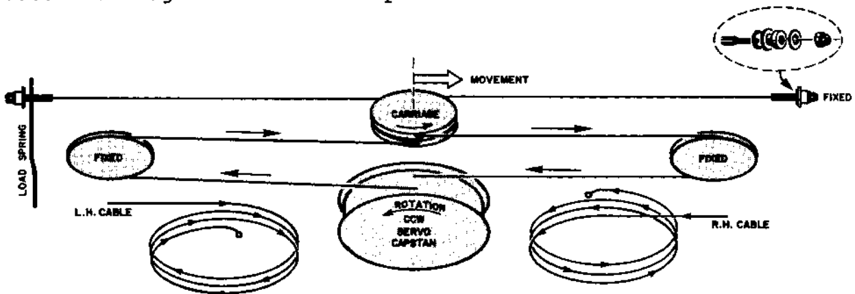
Figure 5-35 CARRIAGE CABLE DRIVE SYSTEM SCHEMATIC
