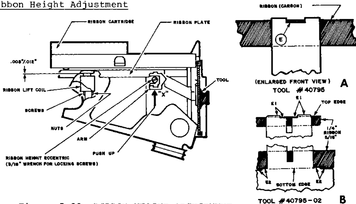
Figure 5-23 RIBBON HEIGHT ADJUSTMENT
