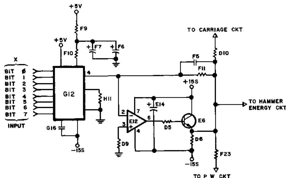
Figure 4-16 D-A CONVERTER CIRCUIT
