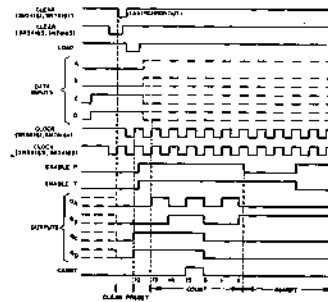
SYNCHRONOUS 4-BIT COUNTER 74161/9316PC / N74161F / SN74161N
