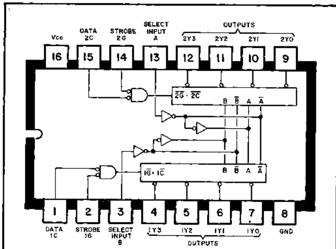
2-LINE-TO-4-LINE DECODER OR 1-LINE-TO-4-LINE DEMULTIPLEXER
