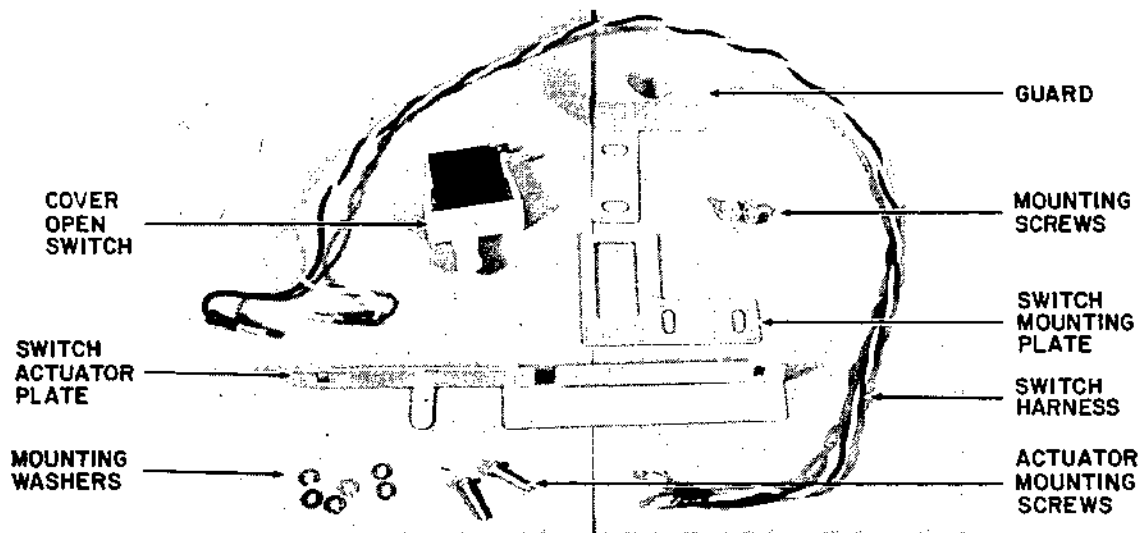
Figure 5-49 COVER OPEN SWITCH ASSEMBLY PARTS
