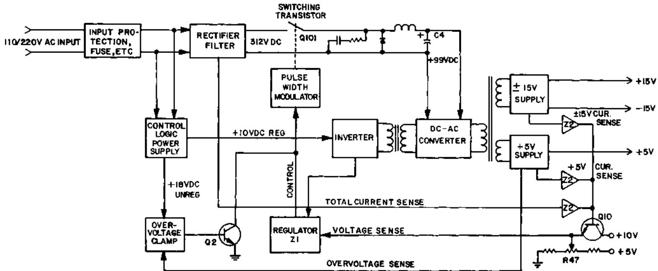
Figure 4-30 OPTIONAL INTERNAL POWER SUPPLY BLOCK DIAGRAM (DP)
