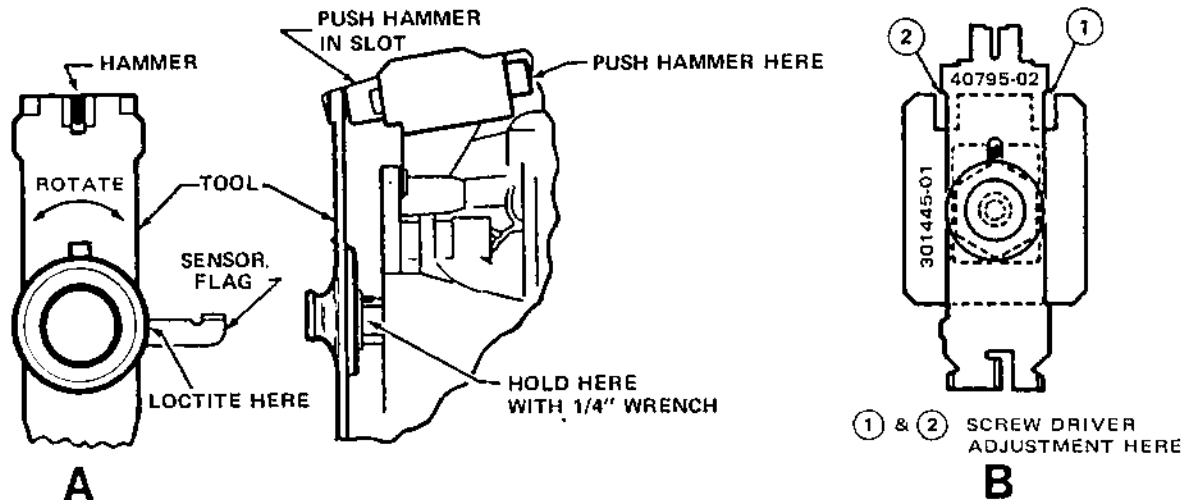
Figure 5-28 PRINT WHEEL TO HAMMER ALIGNMENT
