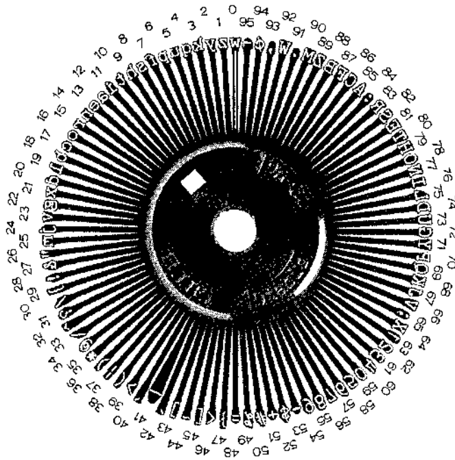
Figure 3-1 96 CHARACTER PLASTIC PRINT WHEEL PHYSICAL SPOKE POSITION
