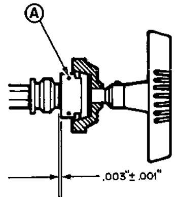
Figure 5-14 PLATEN KNOB END PLAY ADJUSTMENT
