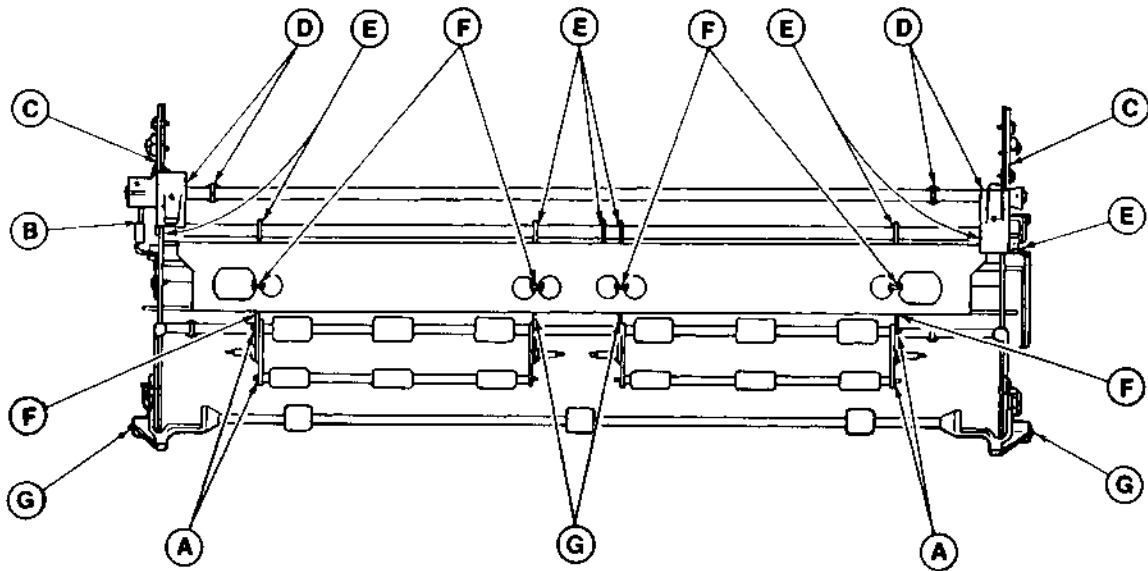
Figure 5-3 CARRIER SYSTEM LUBRICATION POINTS
