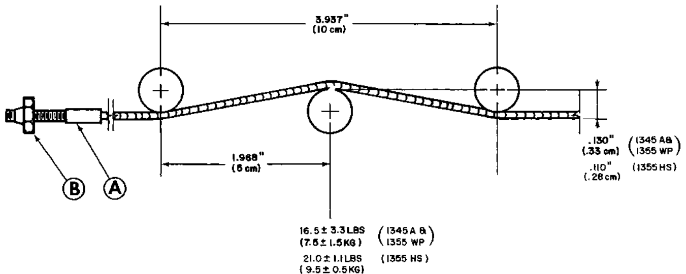
Figure 5-38 CARRIAGE DRIVE CABLE ADJUSTMENT
