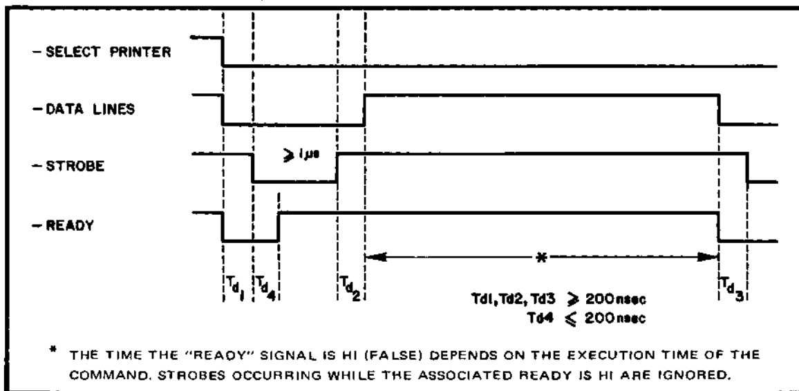
Figure 3-3 TYPICAL COMMAND SEQUENCE
