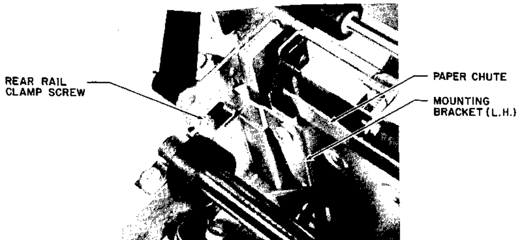
Figure 5-42 UPPER PAPER CHUTE MOUNTING BRACKET INSTALLATION
