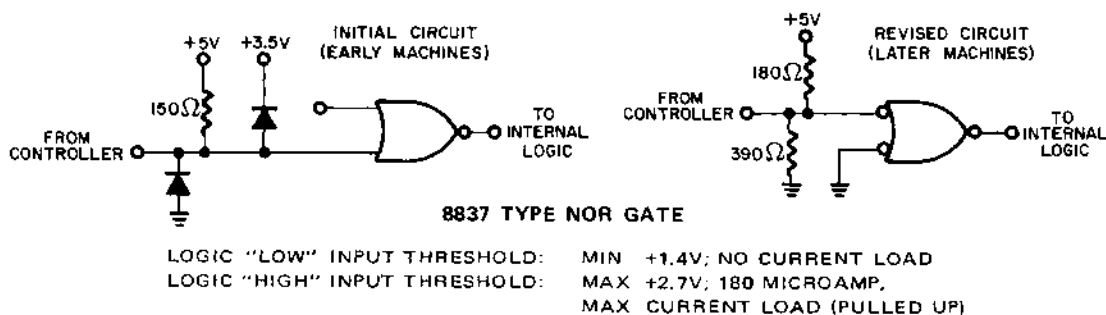
Figure 3-4 STANDARD INPUT CIRCUITS
