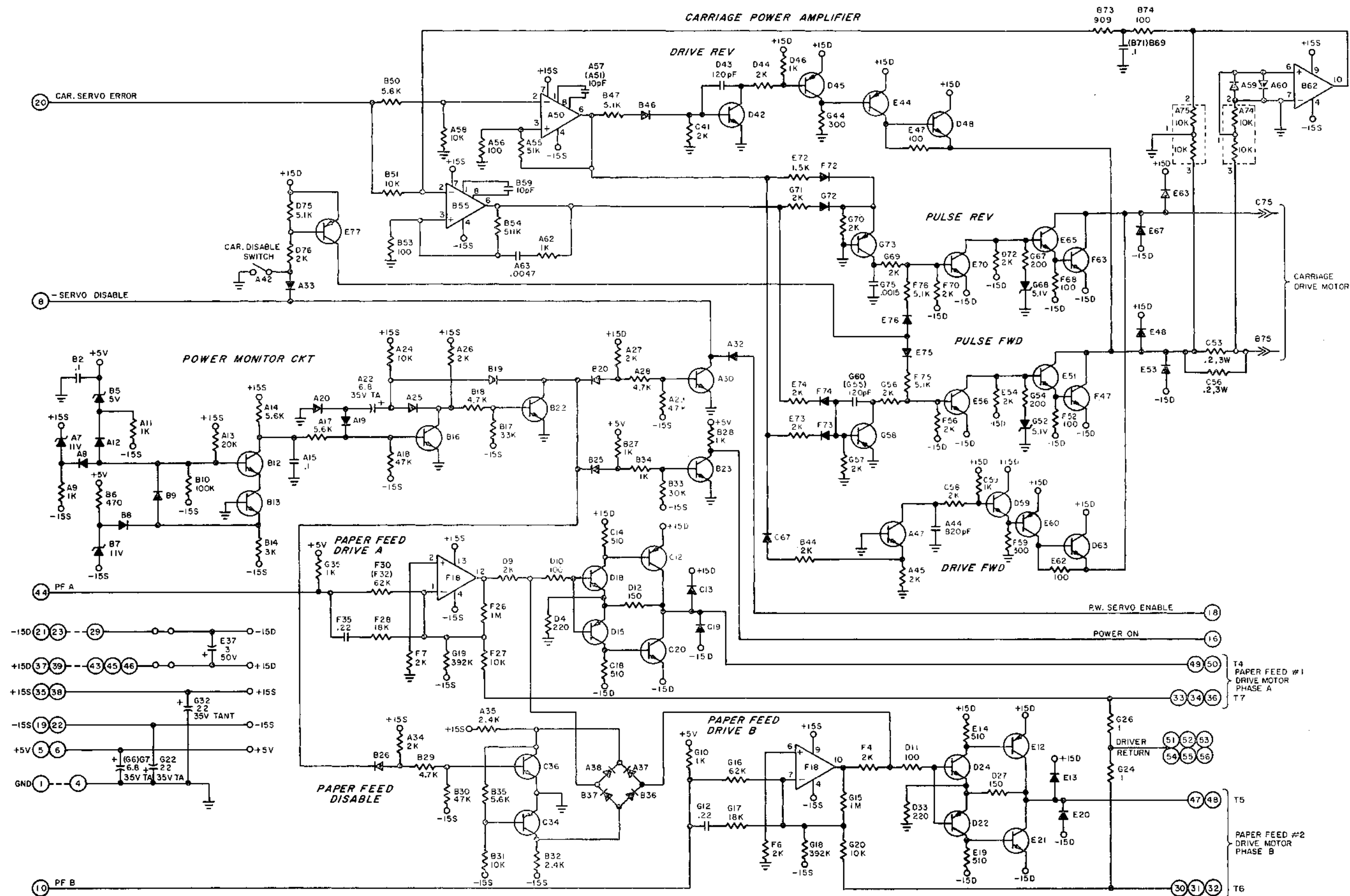
Figure 7-6b Car. Power Amp PCB Assy, 1355HS #46025-05 Rev C
