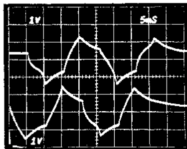
Figure 4-26 PAPER DRIVE WAVEFORMS
