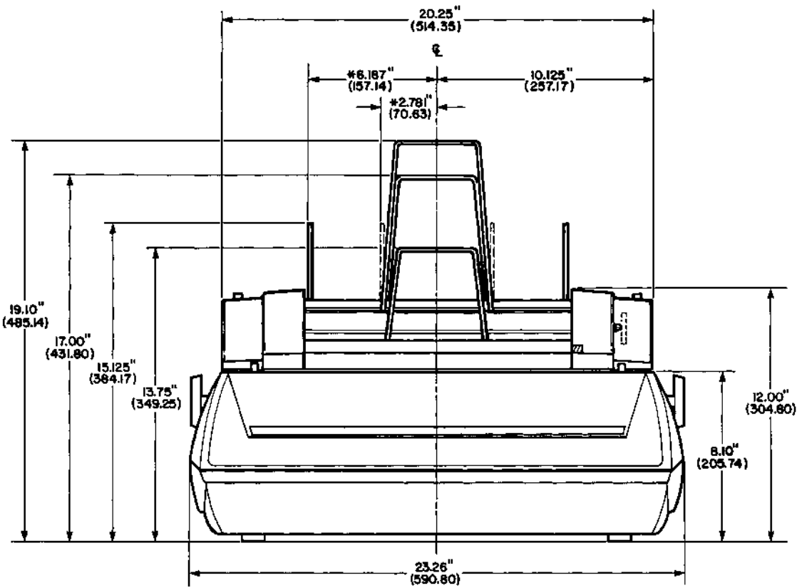
Figure 2-6 HyFEED SHEET FEEDER
