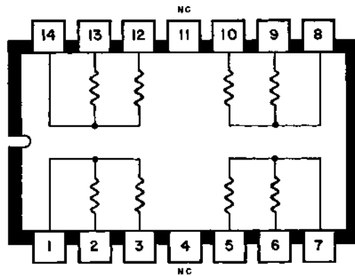
PAIRED CLOSE TOLERANCE ( \pm .0015%) RESISTOR NETWORK 10 K \Omega
