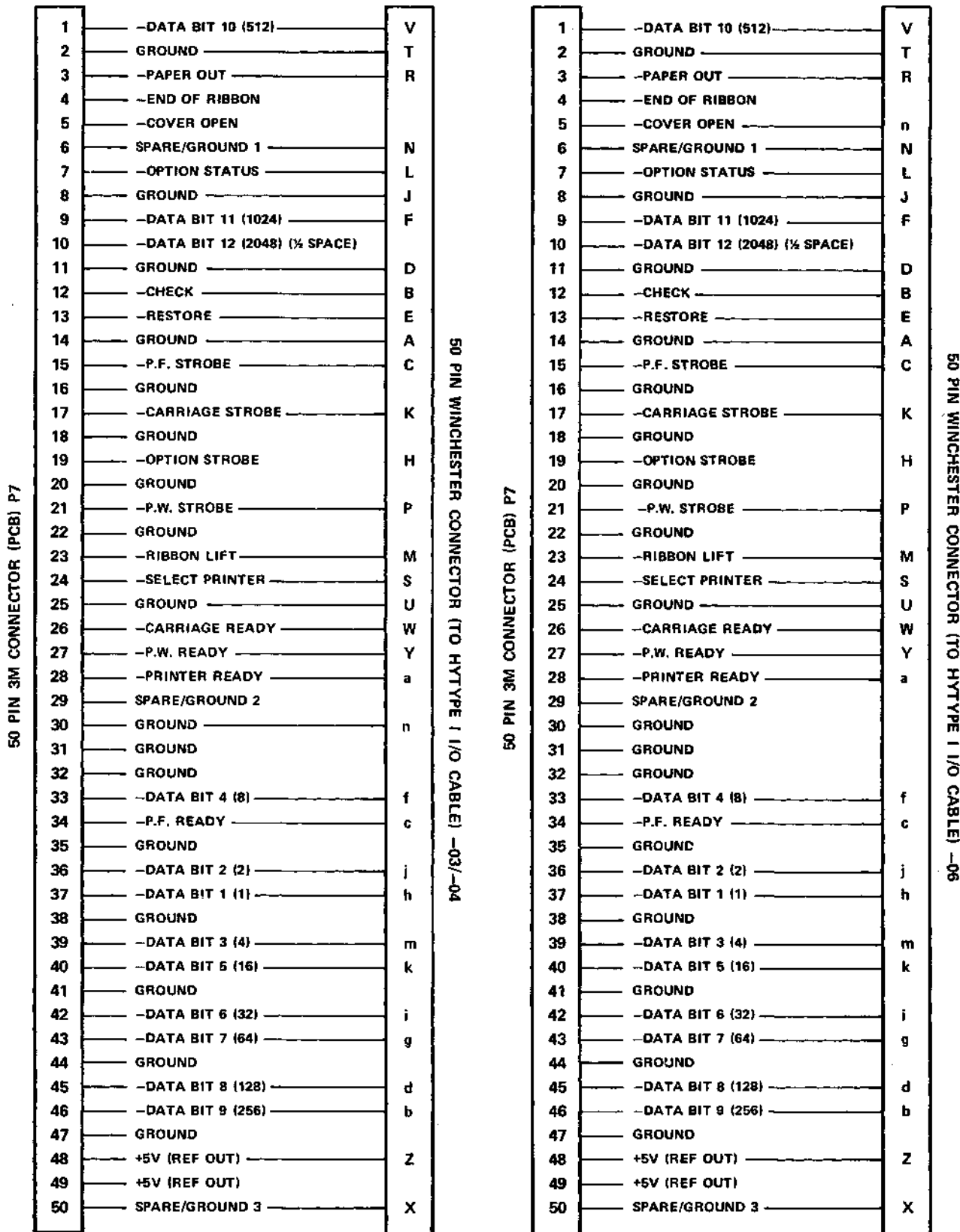
Figure 2-13 HyTYPE II to HyTYPE I ADAPTER CABLE MATING PLUG PIN ASSIGNMENT
