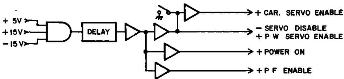
Figure 4-23 POWER MONITOR CIRCUIT BLOCK DIAGRAM
