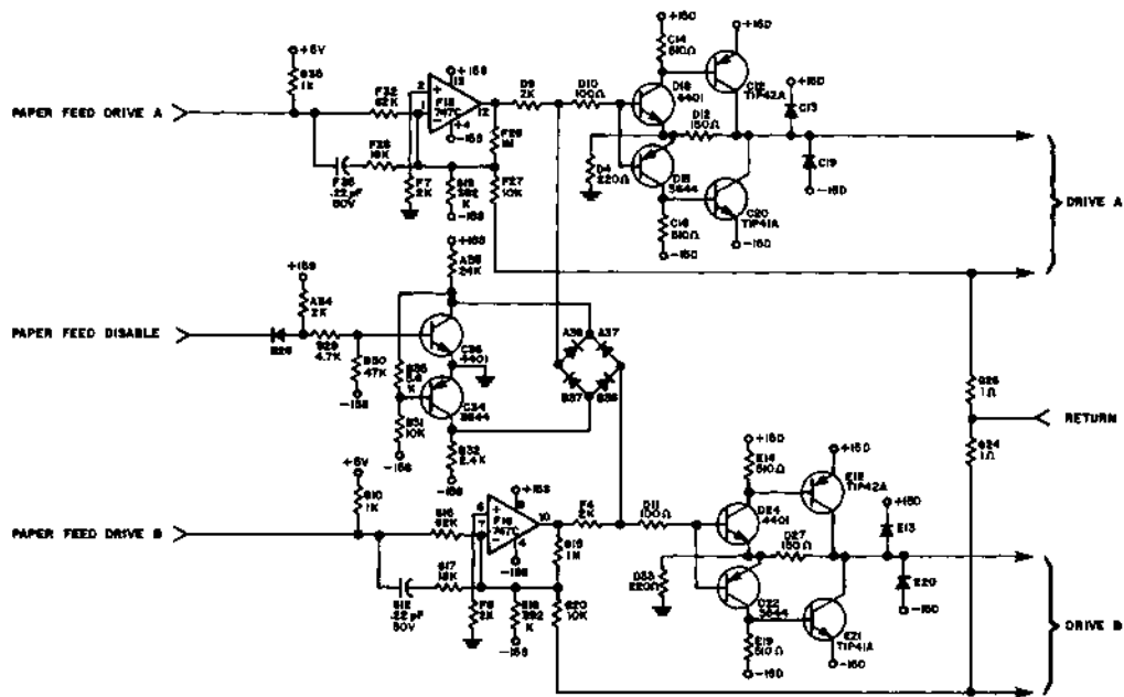
Figure 4-25 PAPER FEED DRIVE CIRCUIT
