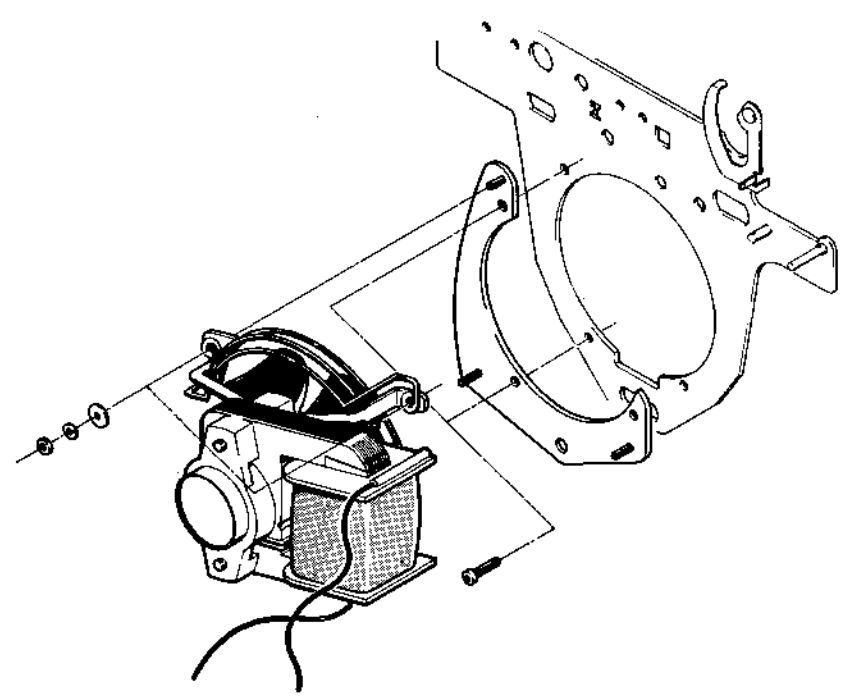
Figure 5-62 COOLING FAN ASSEMBLY INSTALLATION
