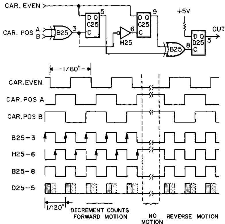
Figure 4-5 CARRIAGE DIFFERENCE COUNTER DECREMENT DRIVE
