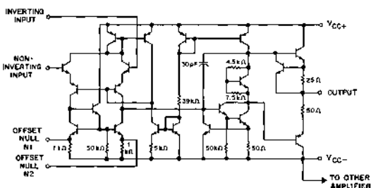
DUAL HIGH PERFORMANCE OP-AMPL. 747C / SN72747N
