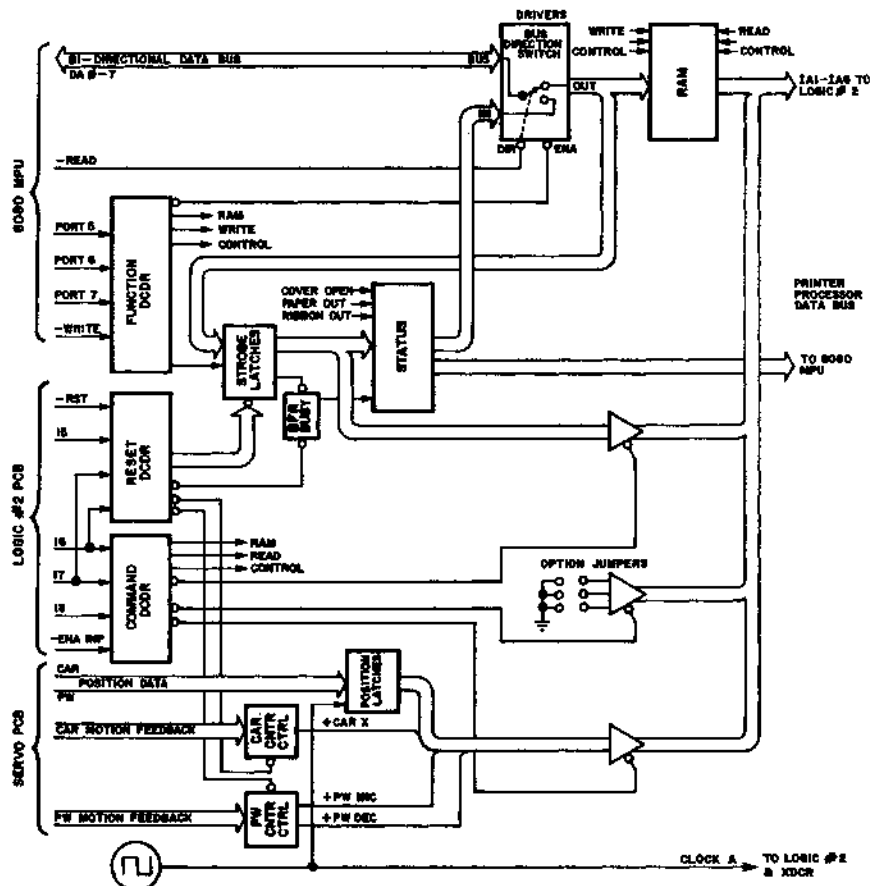
Figure 4-6 8080 LOGIC #1 BLOCK DIAGRAM
