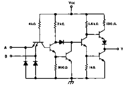
SCHMATIC (each gate)
