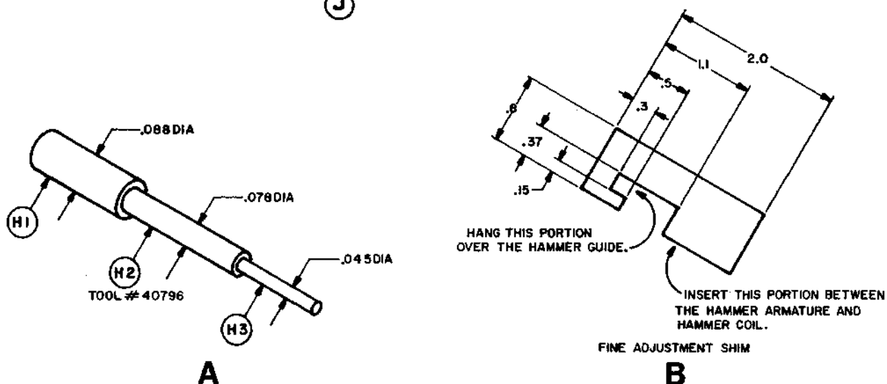
Figure 5-32 HAMMER ADJUSTMENT TOOL #40796 and SHIM
