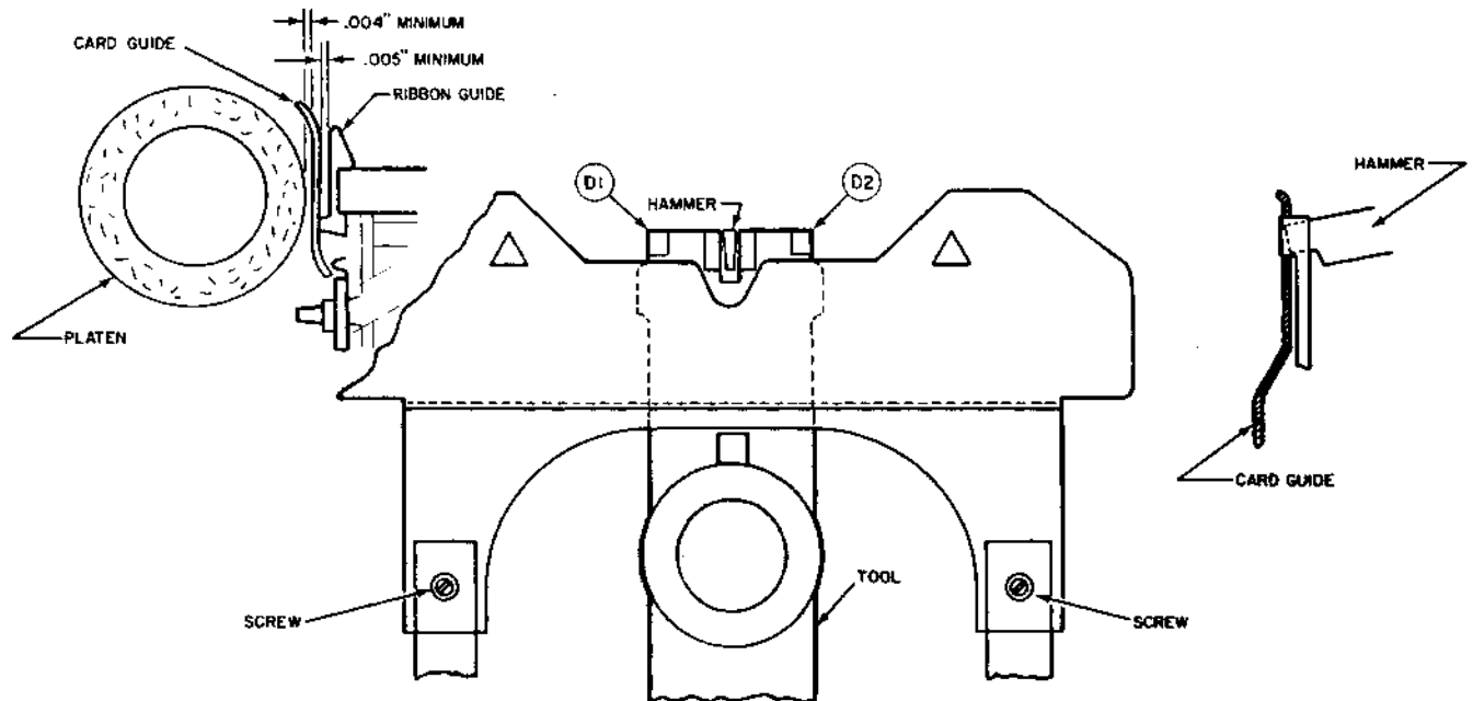
Figure 5-22 CARD GUIDE ADJUSTMENTS
