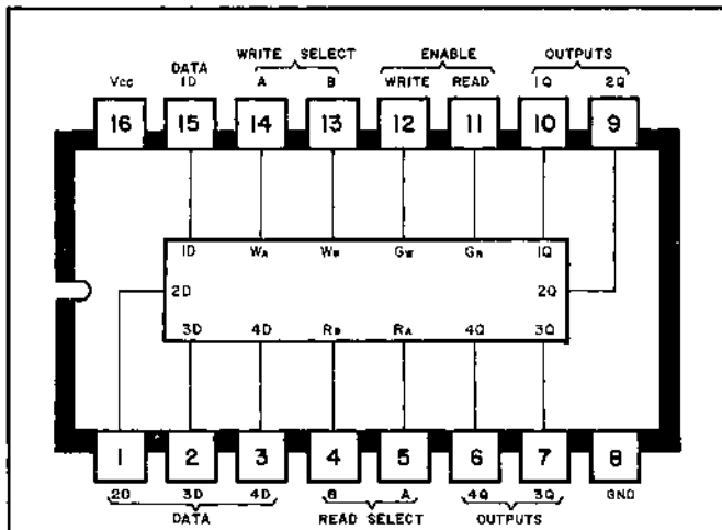
WRITE FUNCTION TABLE (SEE NOTES A, B, & C)
