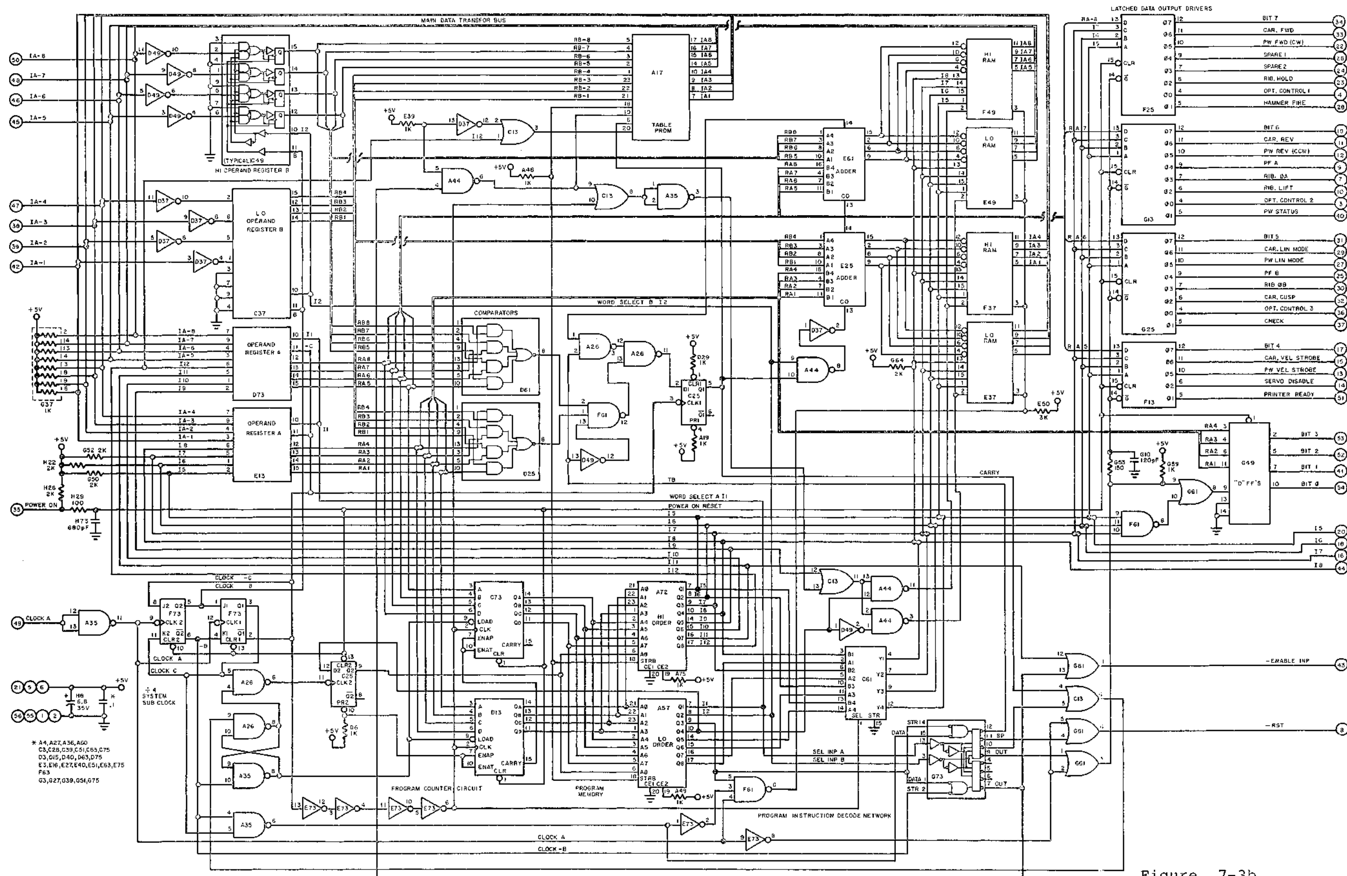
Figure 7-3b Logic #2 PCB Assy, Std ESD #301850-XX Rev C
