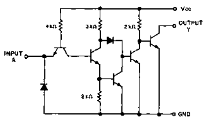
SCHMATIC (each inverter)
