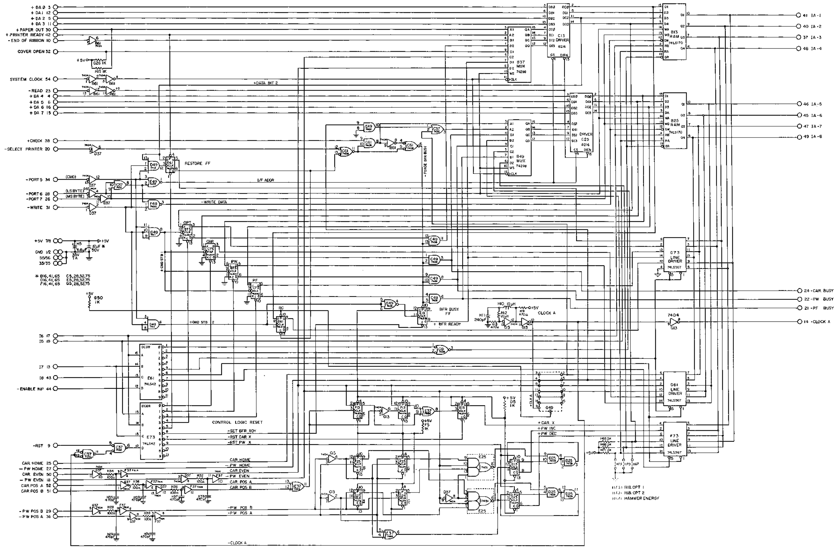
Figure 7-2b Logic #1 PCB Assy, 8080 #40644-05 Rev B
