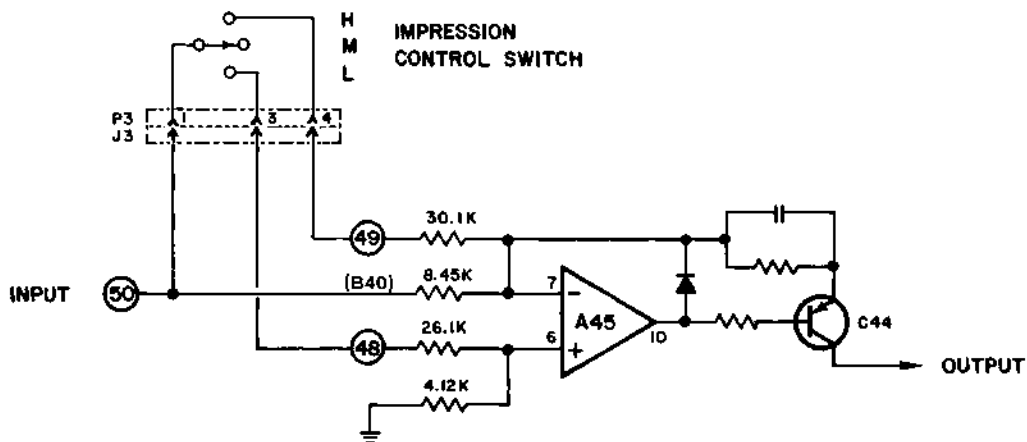
Figure 4-29 HAMMER ENERGY CONTROL CIRCUIT
