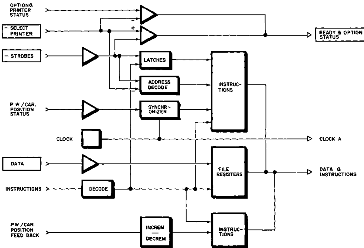
Figure 4-3 LOGIC #1 BLOCK DIAGRAM
