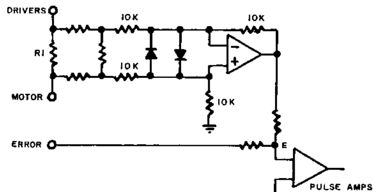
Figure 4-28 PRINT WHEEL FEEDBACK INSTRUMENTATION CIRCUIT
