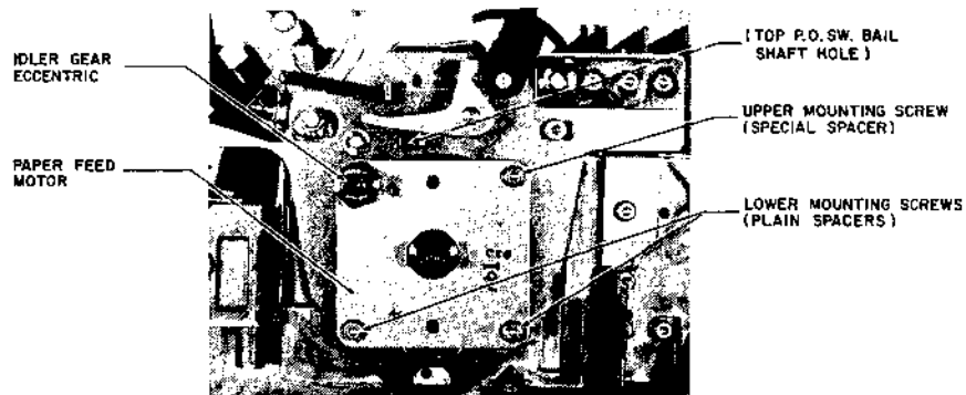
Figure 5-9 PAPER FEED MOTOR REMOVAL
