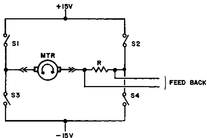
Figure 4-21 CARRIAGE POWER AMPLIFIER SIMPLIFIED DIAGRAM
