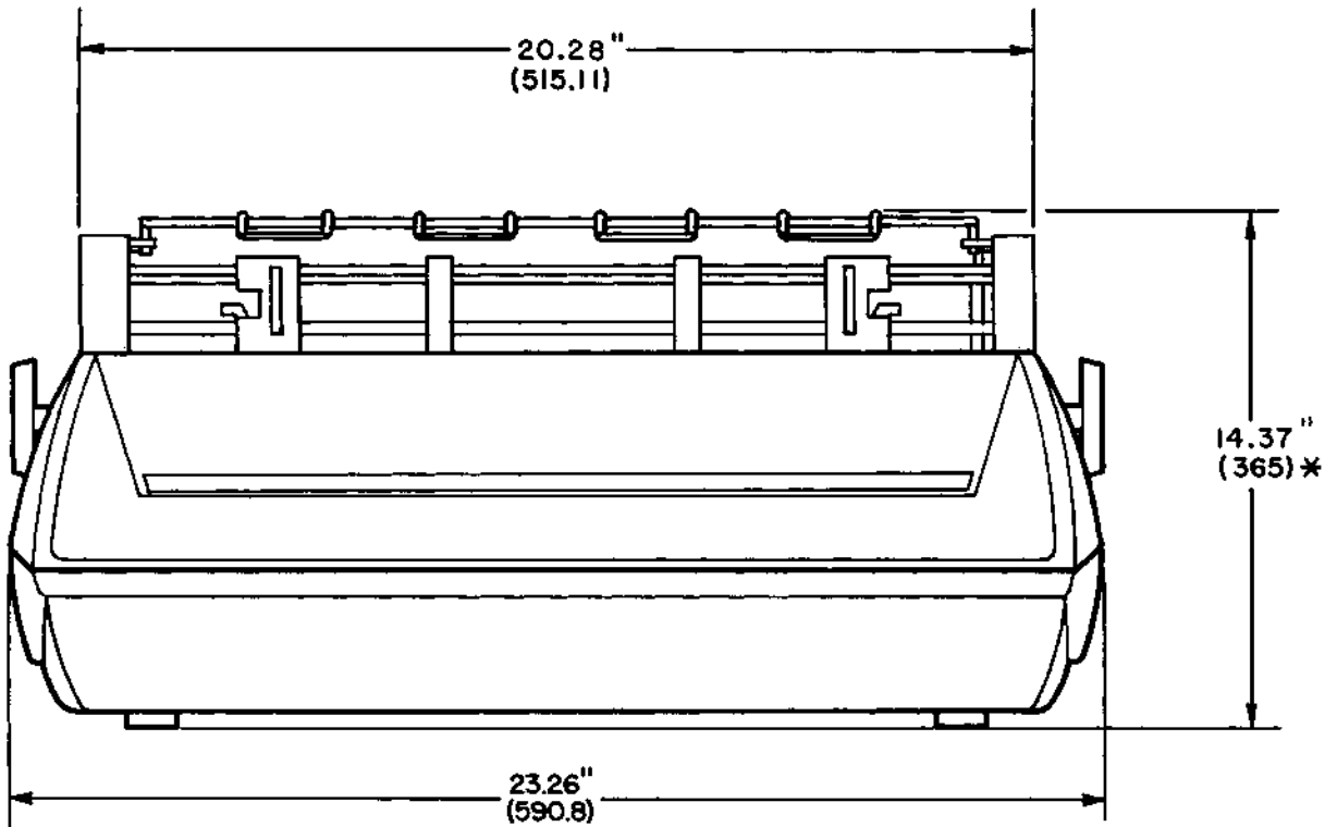
Figure 2-3 DIABLO BIDIRECTIONAL FORMS TRACTOR
