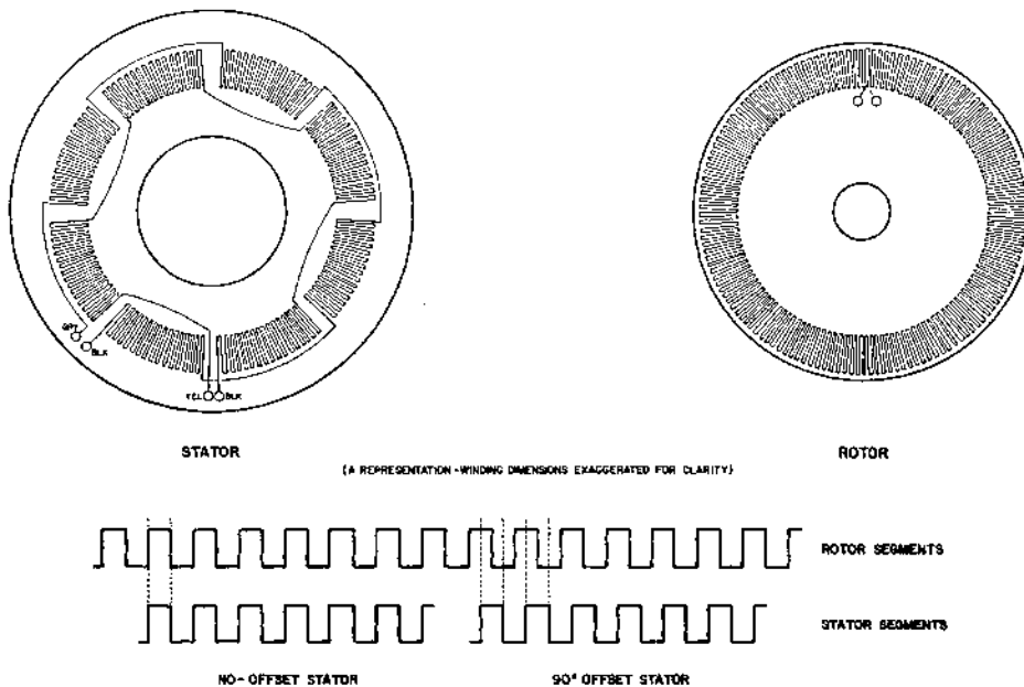
Figure 4-9 SERVO POSITION TRANSDUCER
