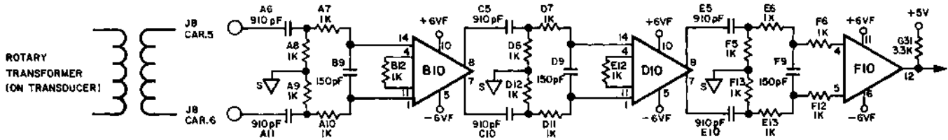
Figure 4-10 SERVO FEEDBACK AMPLIFIER
