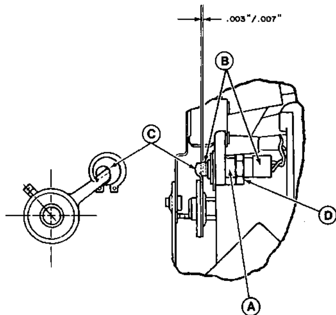
Figure 5-29 PRINT WHEEL "HOME" ALIGNMENT
