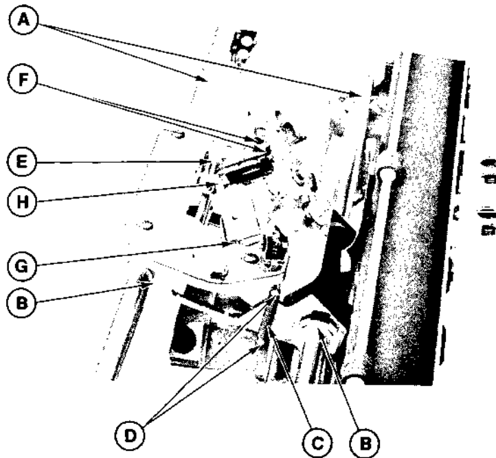
Figure 5-2 CARRIAGE SYSTEM LUBRICATION POINTS
