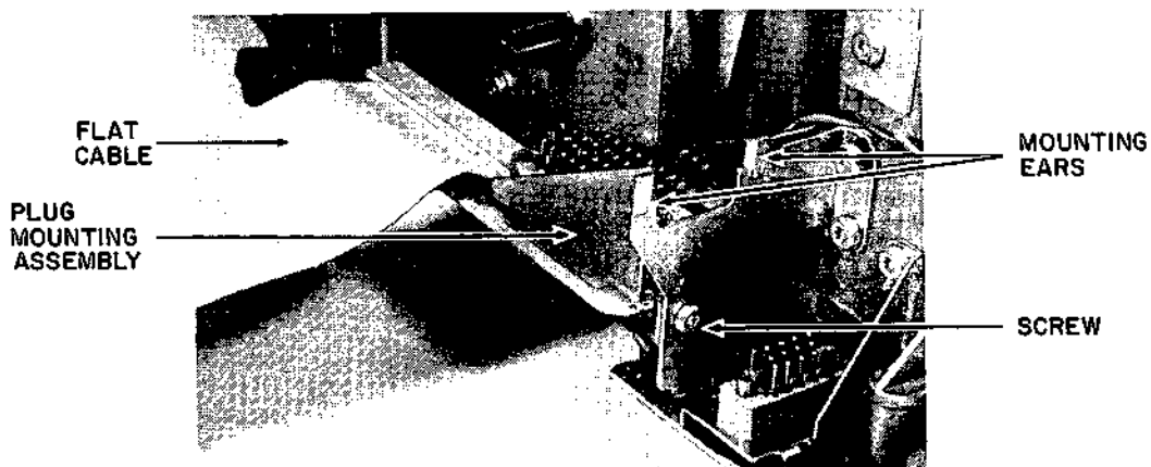
Figure 5-53 ADAPTER CABLE OPTION INSTALLATION
