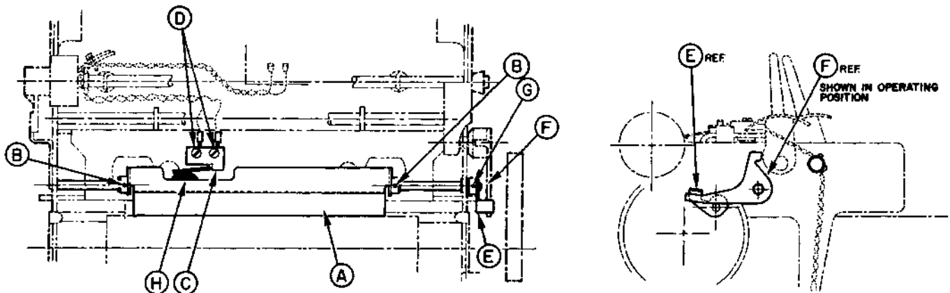
Figure 5-47 TOP PAPER OUT SWITCH AND BAIL INSTALLATION LOCATIONS
