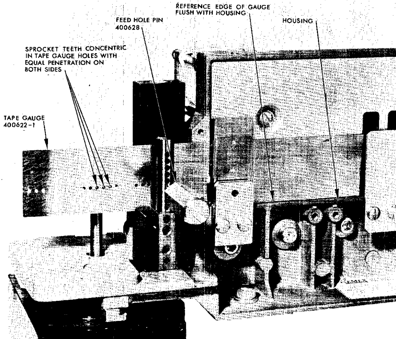
Figure 5-3. Sprocket Alignment Using Tape Gauge.
