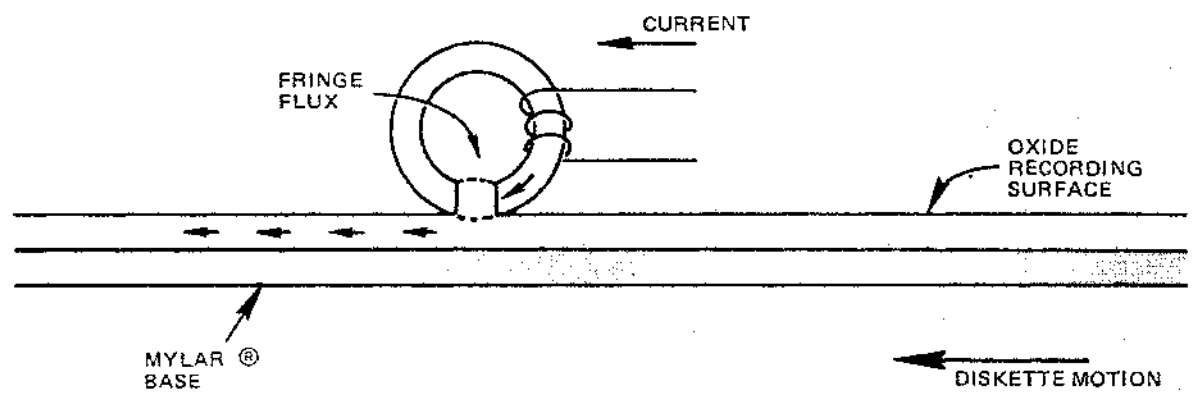
Figure 24 Basic R/W Head
