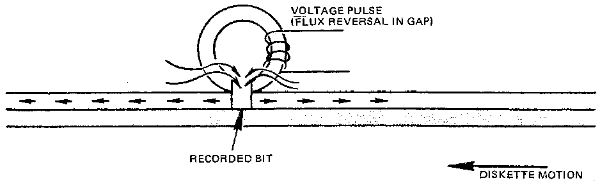
Figure 26 Reading a Bit
