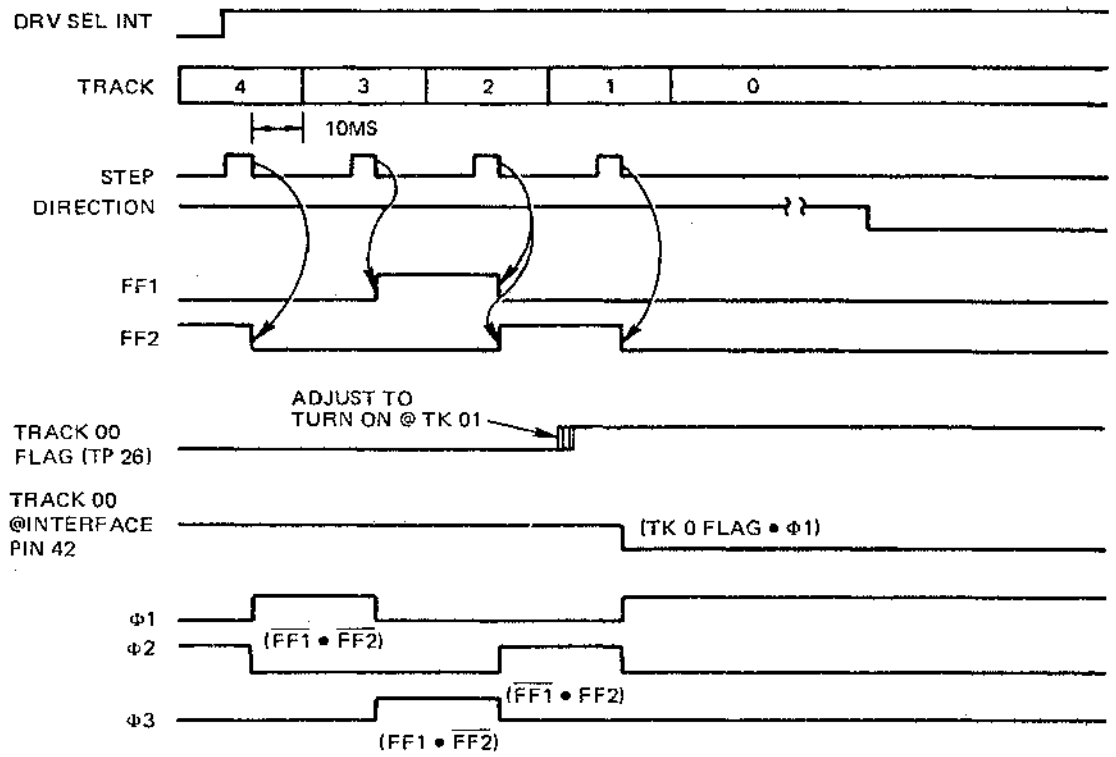
Figure 22 Track 00 Timing
