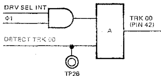
Figure 21 Track 00 Flag
