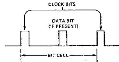
Figure 3 Bit Cell
