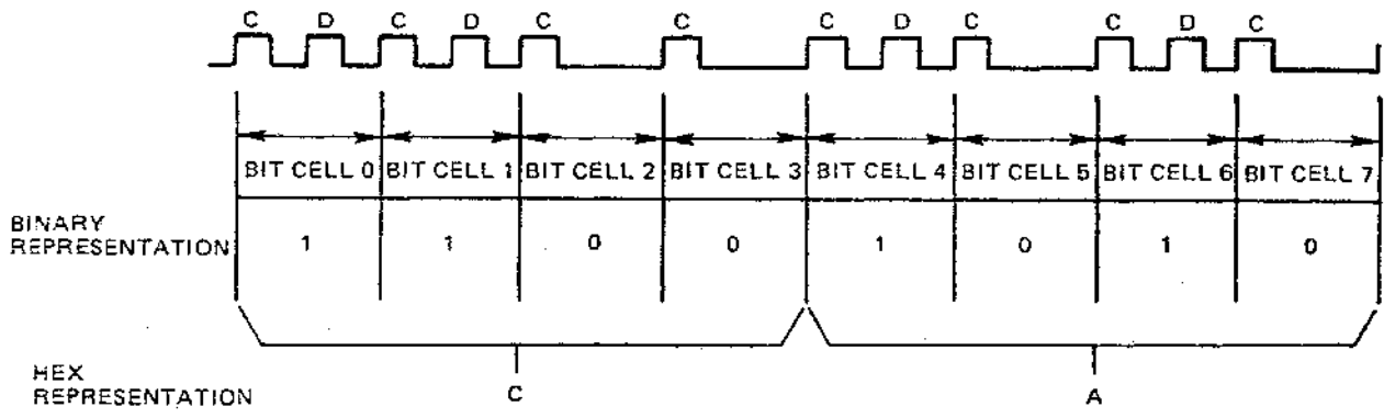
Figure 23 Bit Cell
