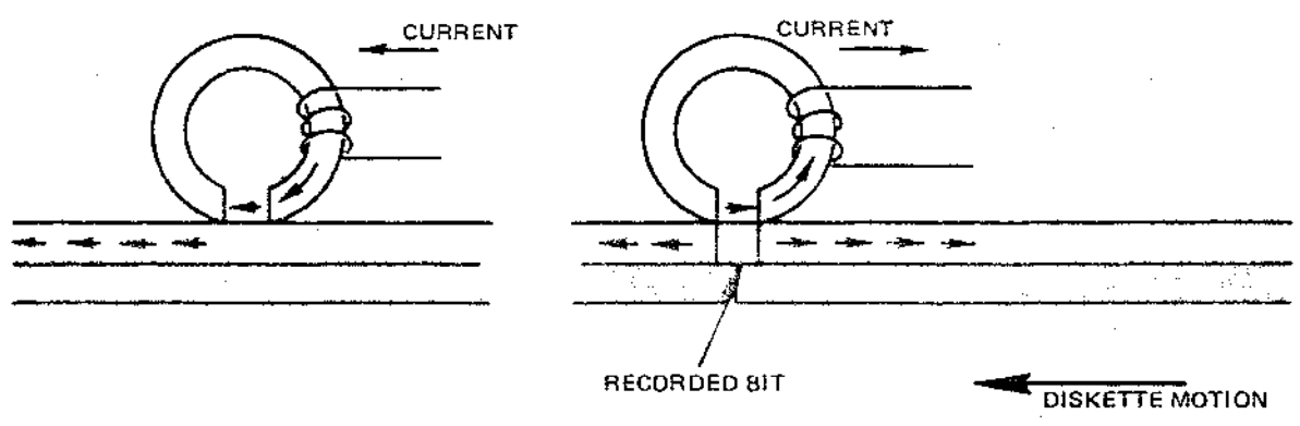
Figure 25 Recorded Bit
