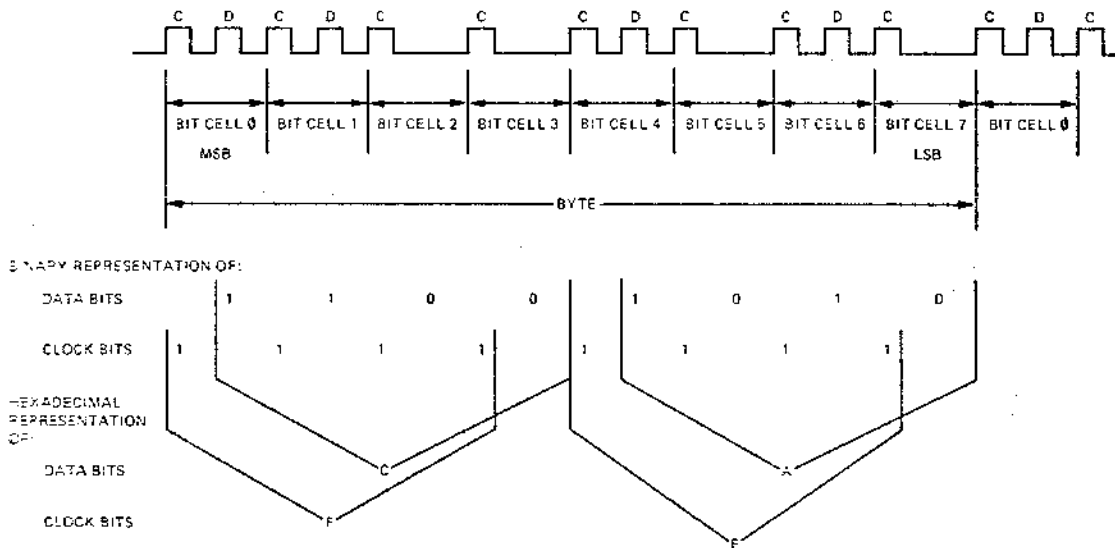
Figure 4 Byte
