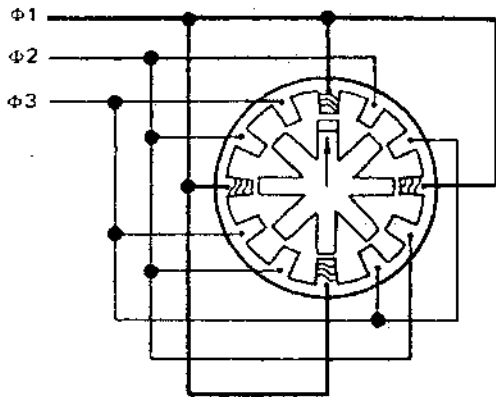
Figure 14 Position 1 (Trk 00)
