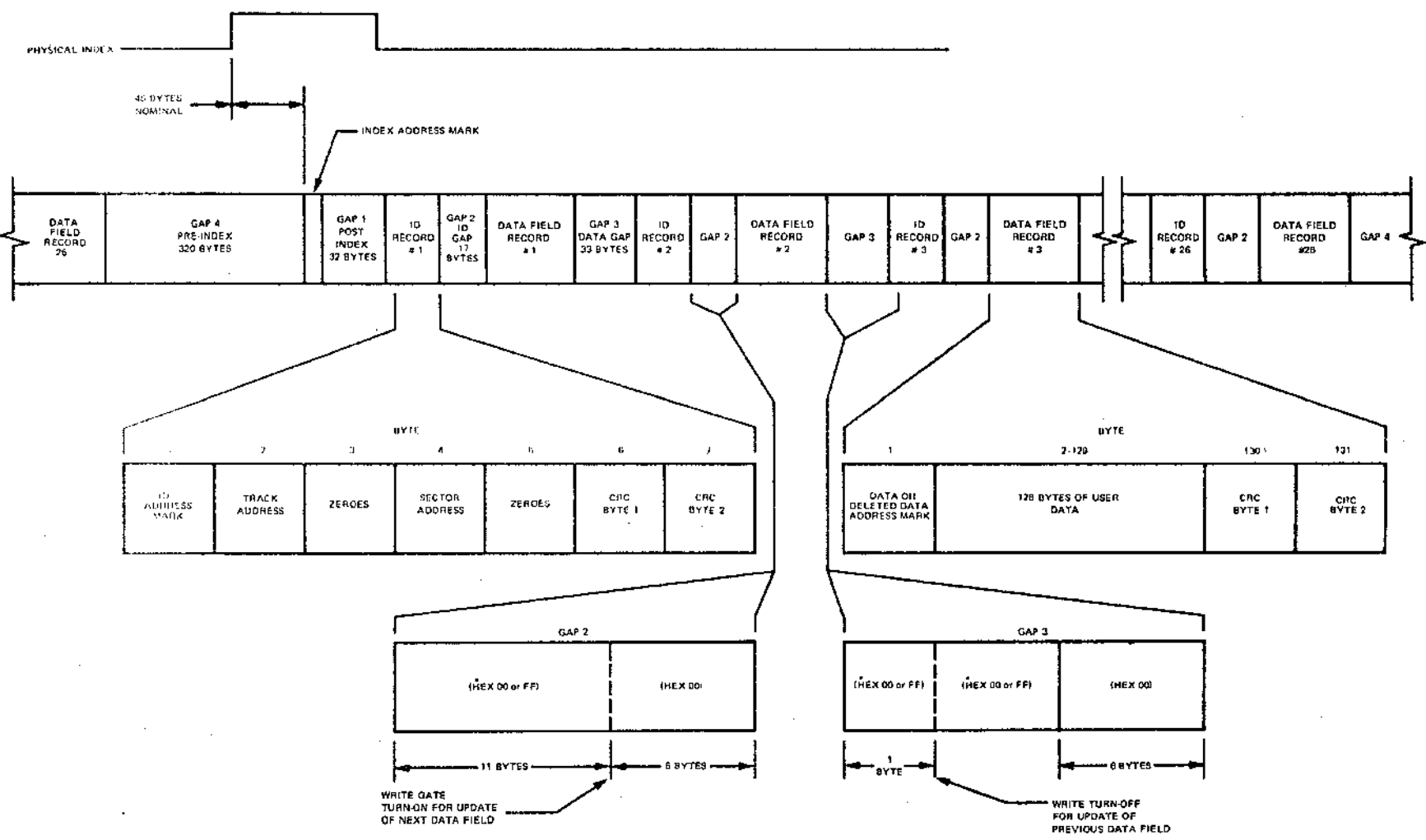
Figure 8 Track Format
