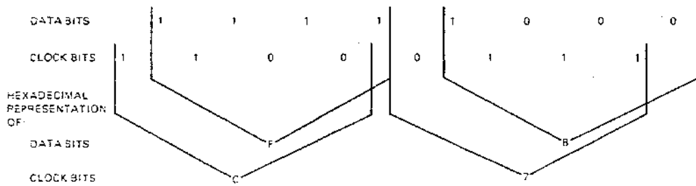
Figure 12 Deleted Data Address Mark
