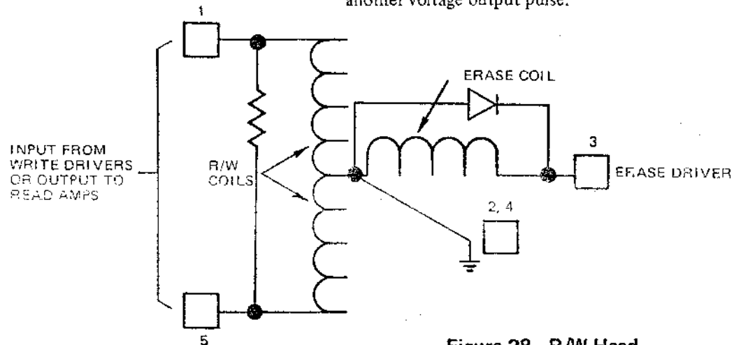
Figure 28 R/W Head
