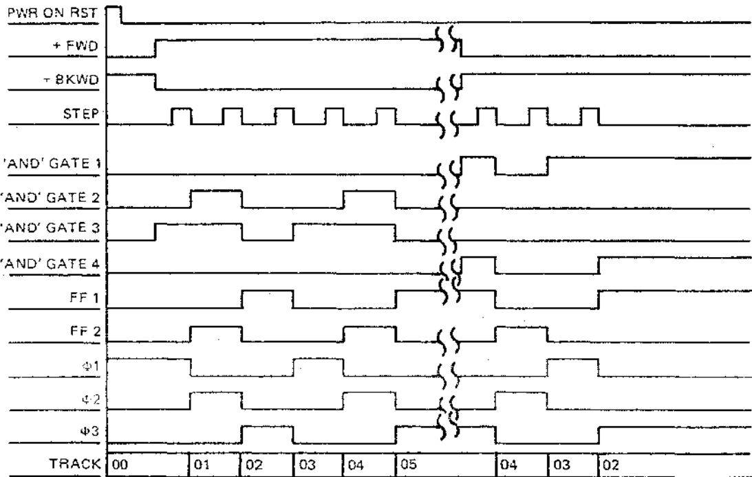
Figure 18 Track Accessing
