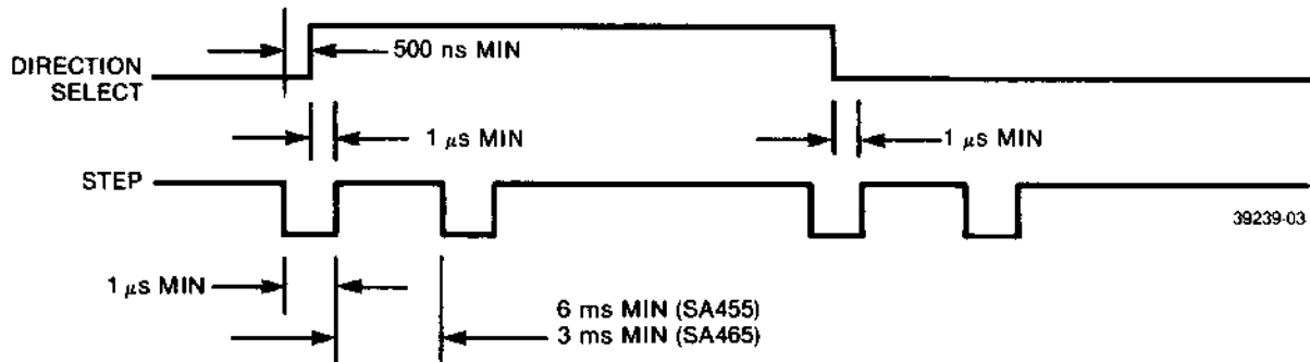
FIGURE 4-10. STEPPER TIMING
