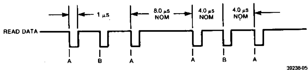
FIGURE 1-6. READ DATA TIMNG (FM)
