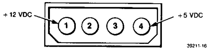
FIGURE 3-3. J2 CONNECTOR
