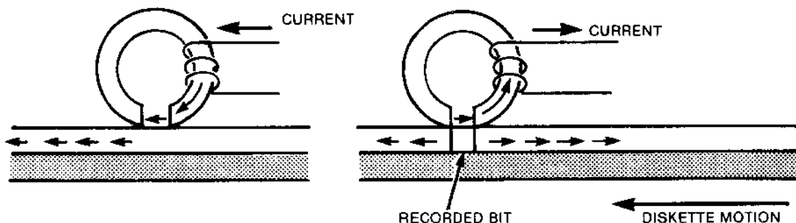
FIGURE 4-3. RECORDED BIT
