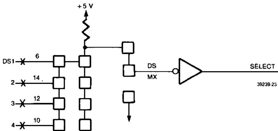
FIGURE 4-12. DRIVE SELECT
