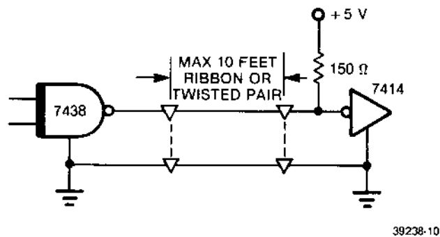
FIGURE 2-2. INTERFACE SIGNAL DRIVER/RECEIVER
