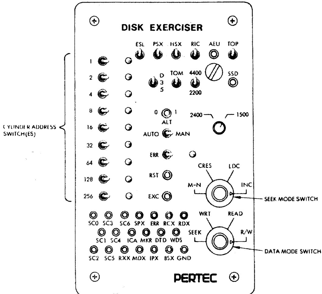
Figure 1. Disk Exerciser Control Panel
