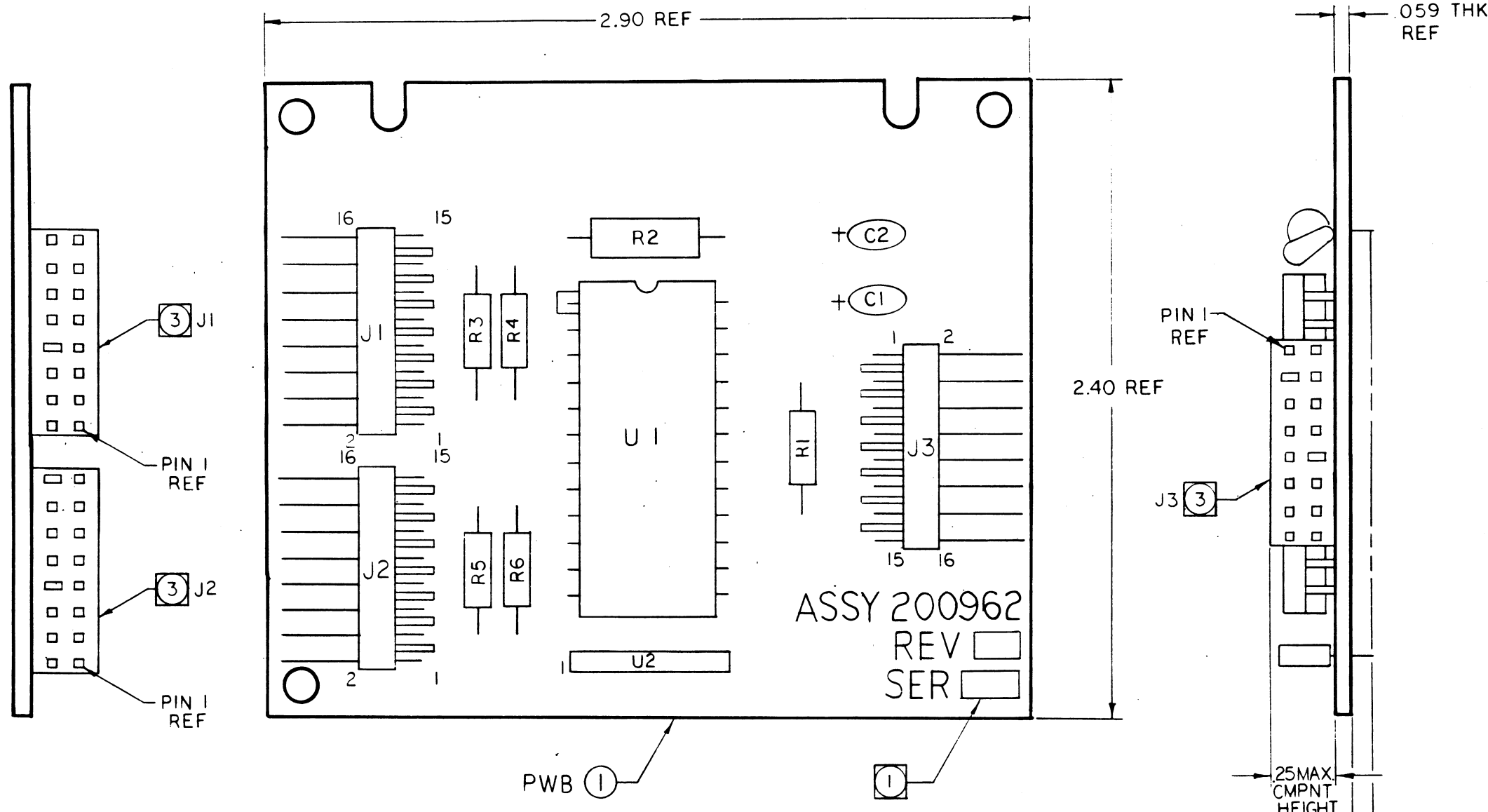
COMPONENT (FRONT) SIDE SHOWN
