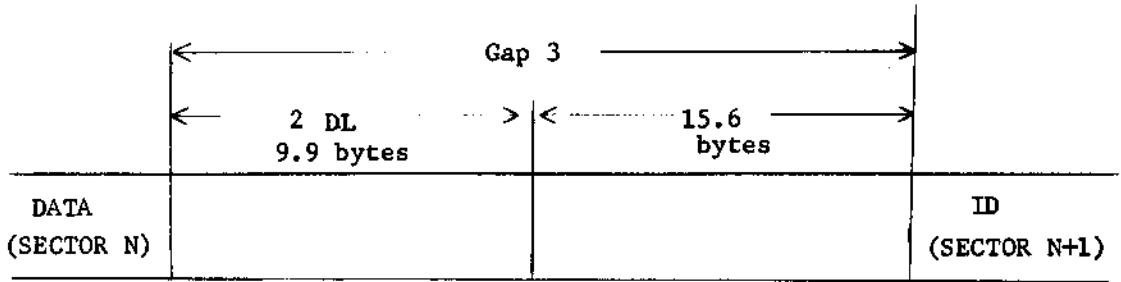
a) Nominal Positions
