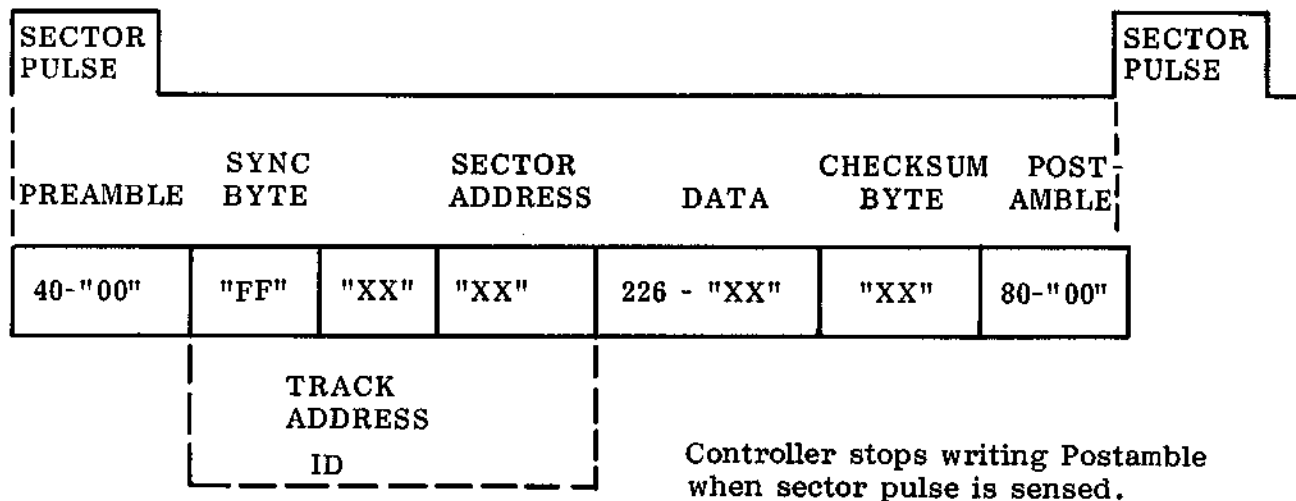
FIGURE 6 MICROPOLIS HARD SECTOR DOUBLE DENSITY FORMAT
