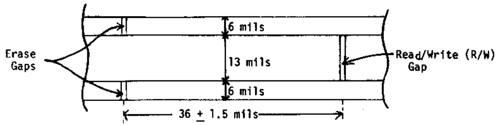
Tunnel Erase Head (Used by IBM and most drive manufacturers)
