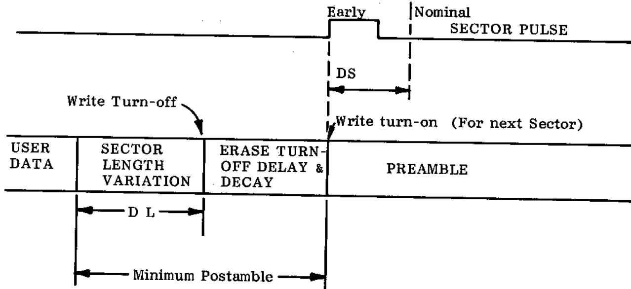
FIGURE 16. Minimum Postamble Length (For Postamble Left Blank)
