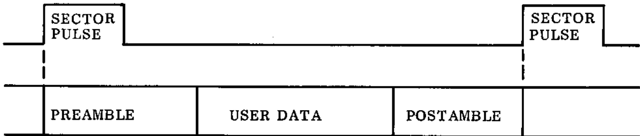
FIGURE 4 - TYPICAL HARD SECTOR FORMAT
