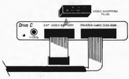
Internal Monitor
