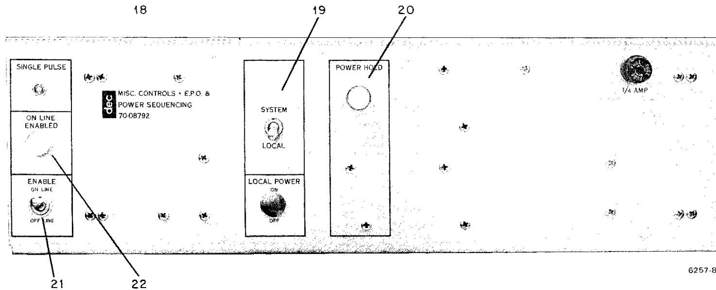
Figure 3-1 DX11-B Controls and Indicators
