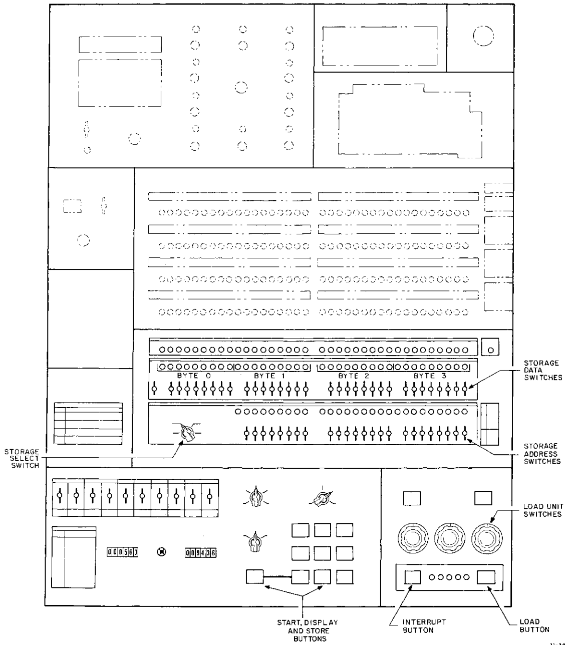
Figure 2-20 IBM 360/370 Console
