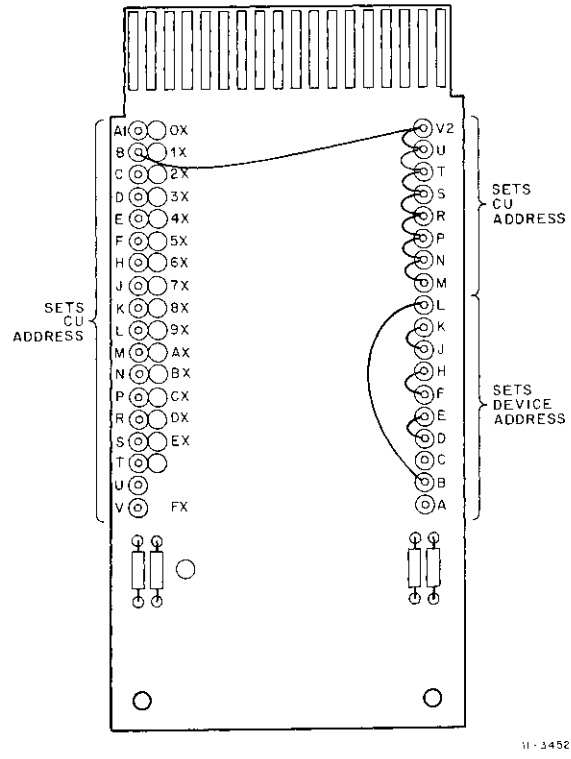
Figure 2-9 Example of Wiring for One Device (10) (Not Supported by DX11-B Diagnostics)
