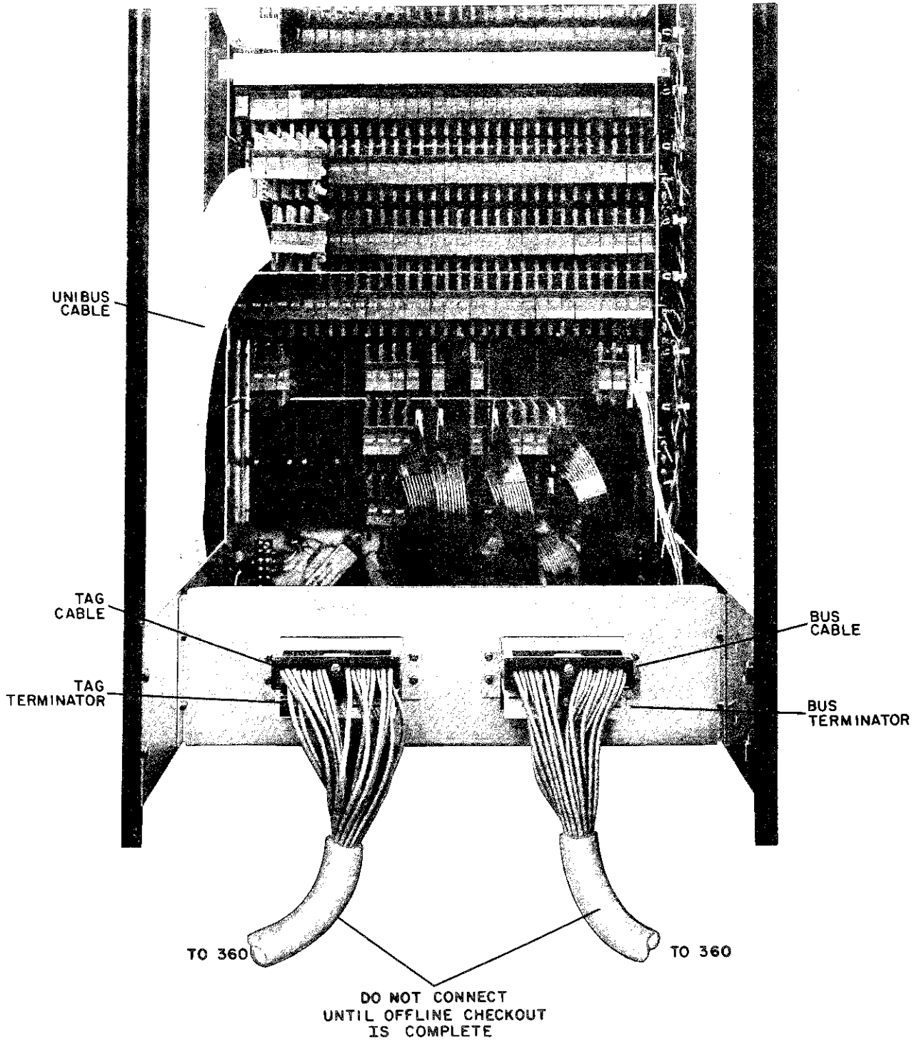
Figure 2-17 Normal Cable Connections to Channel Bus if on End of Bus
