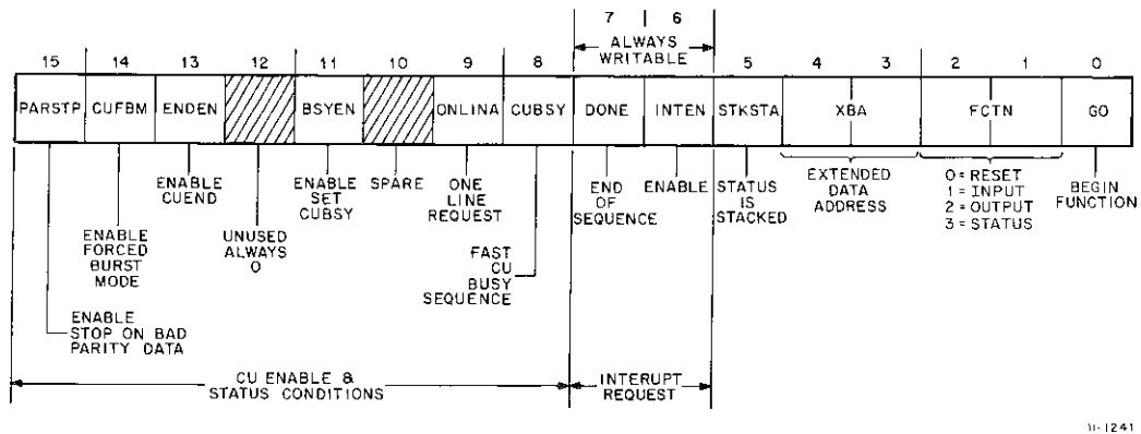
Figure 4-5 Control Unit Status Register (DXCS) Bit Assignments
