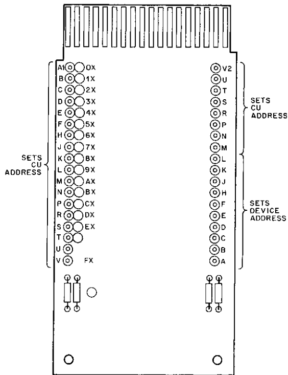
Figure 2-4 M908 Module Before Wiring
