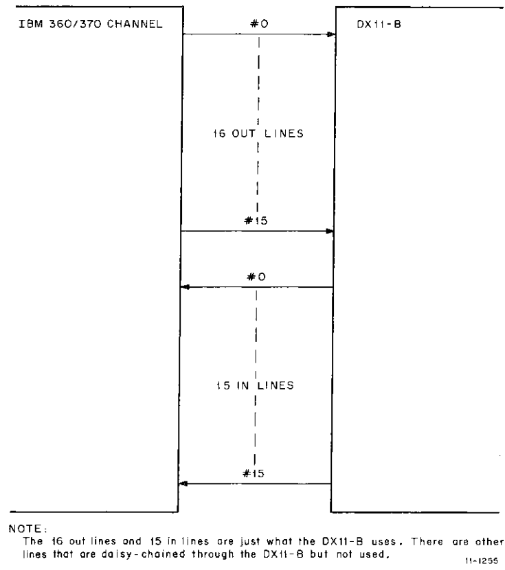
Figure 5-4 Channel/DX11-B Interface
