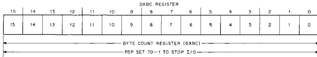
Figure 4-8 Byte Count Register (DXBC) Bit Assignments
