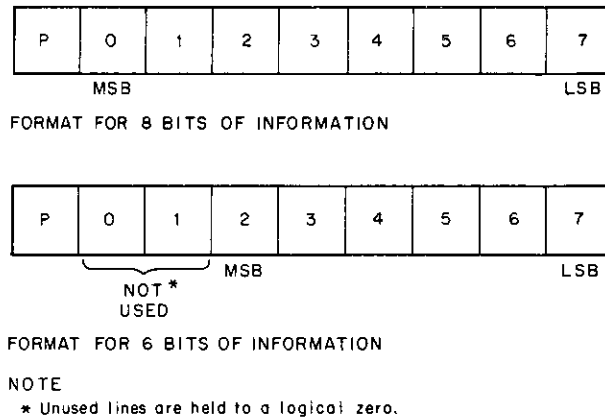
Figure 2-25 Formats for Transmission of Information on the Buses
