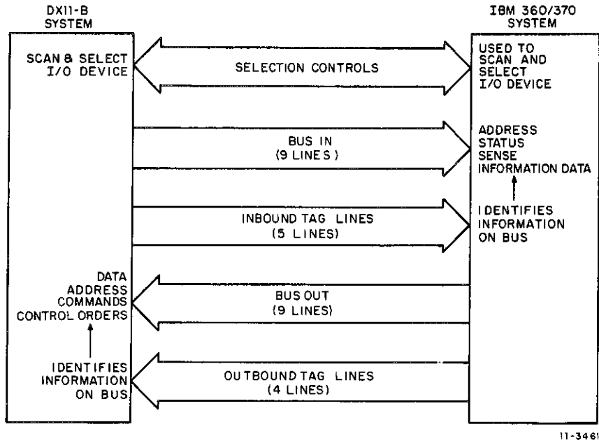
Figure 2-24 Input/Output Signals
