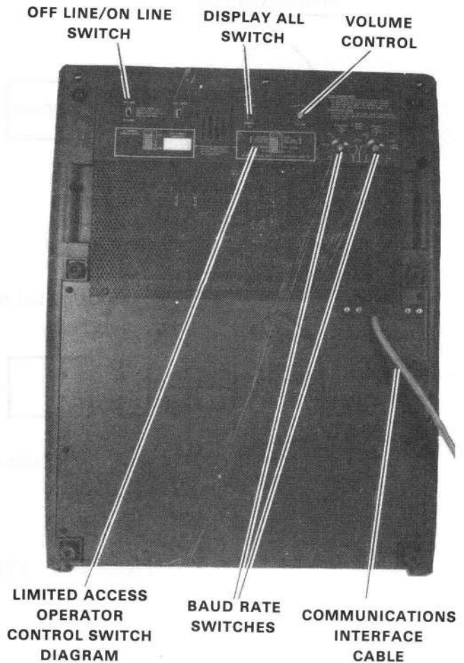
Figure 2-11 Operator Controls Access Position
