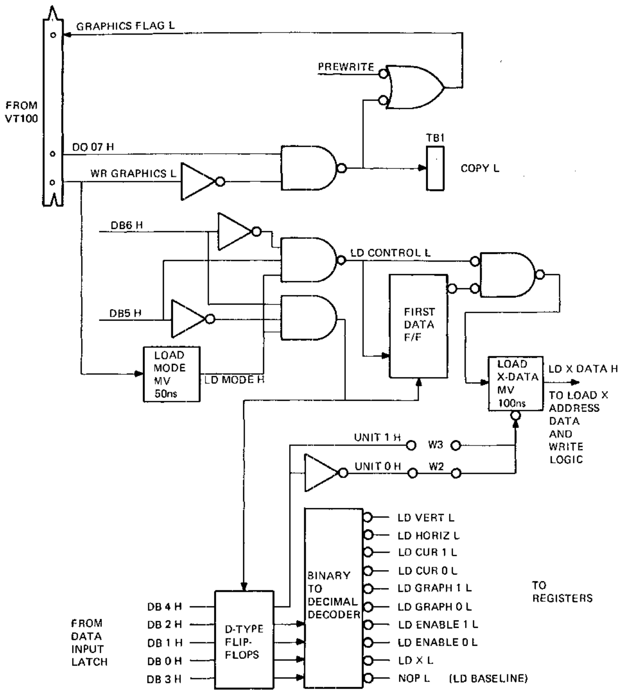
Figure 6-17 Decoding the Control Character
