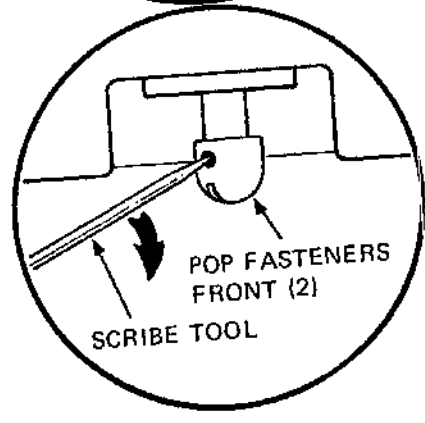
Figure 5-21 Top Cover Removal
