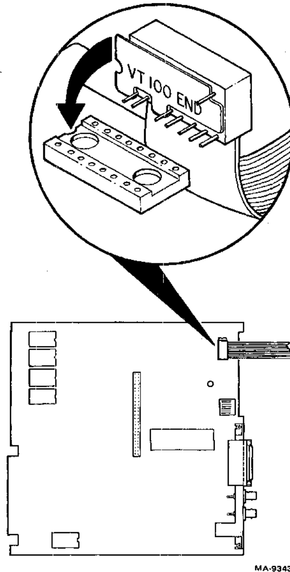
Figure 6-46 16-Pin Flat Cable on Terminal Controller
