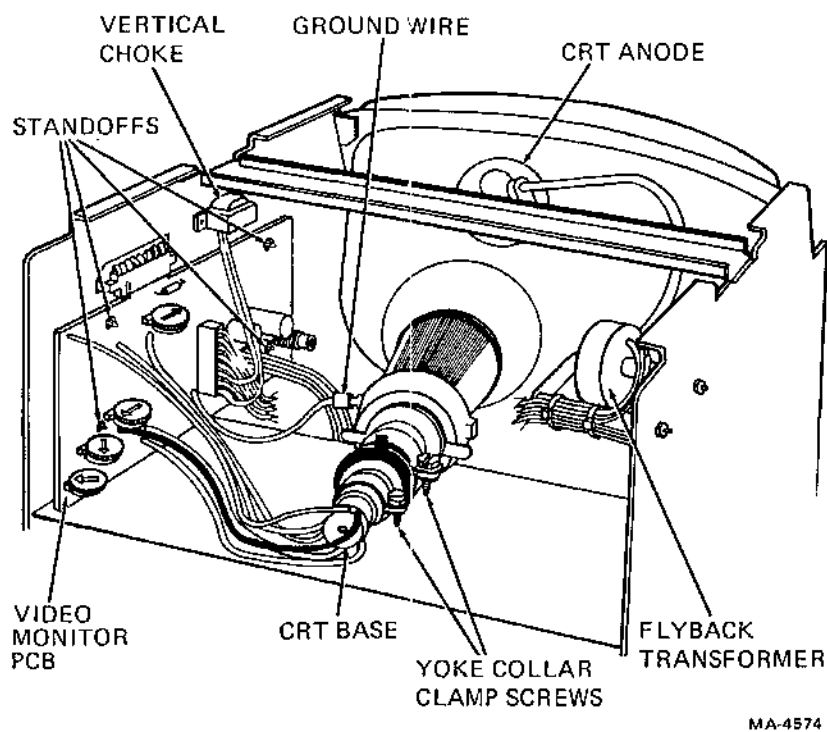
Figure 5-23 Elston/DIGITAL Video Monitor Board Removal
