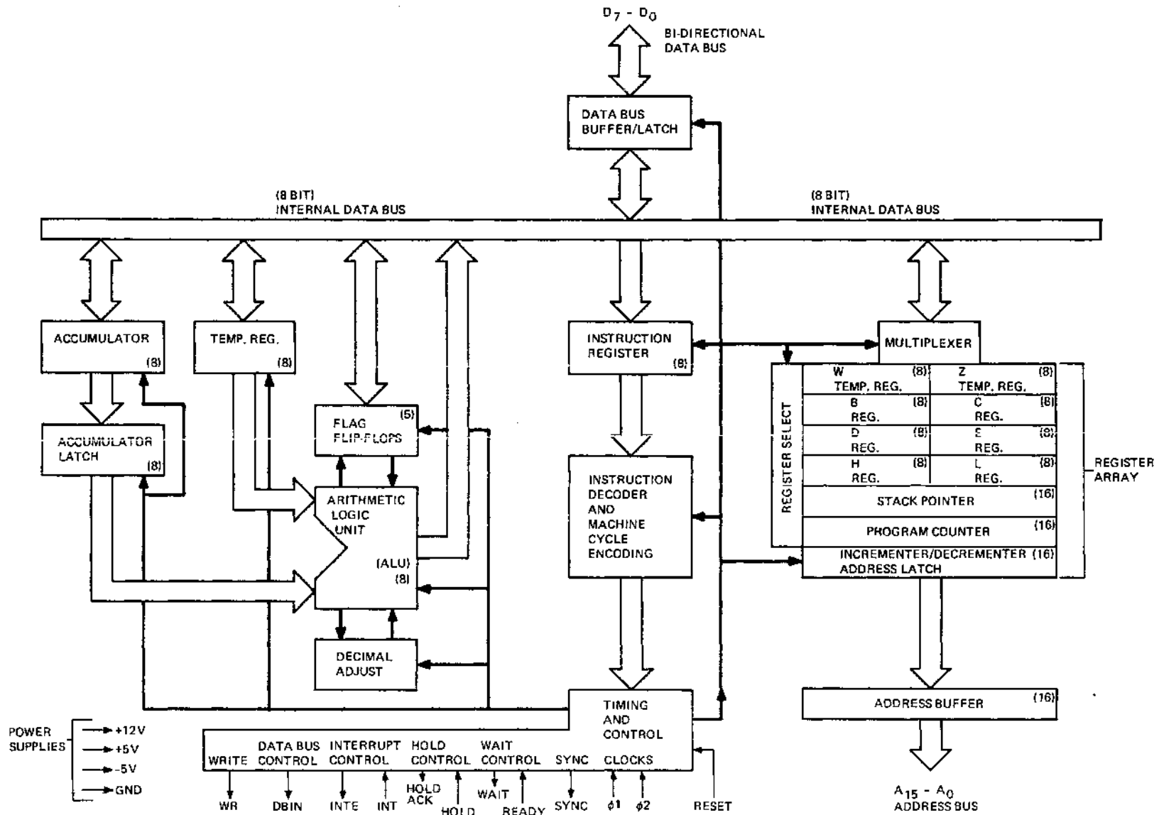
Figure 4-2-1 8080 Block Diagram
