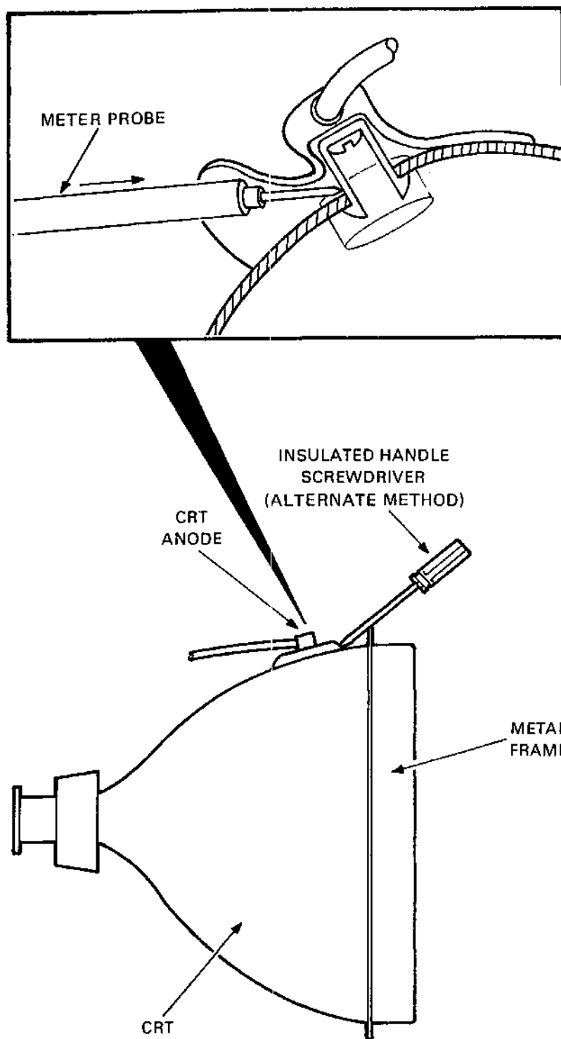
Figure 5-29 CRT Anode Discharging
