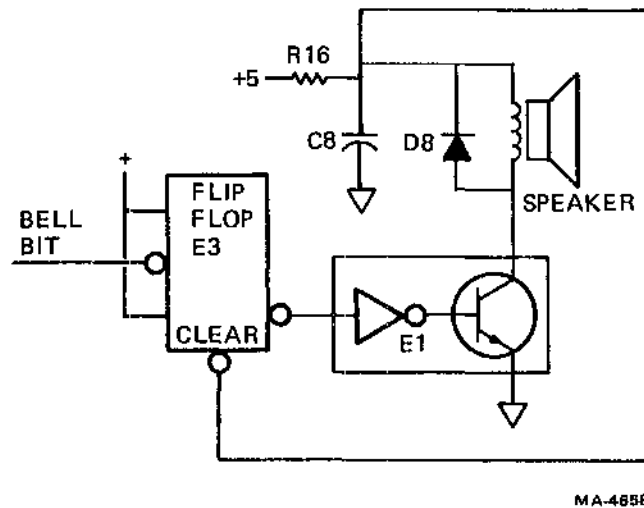
Figure 4-4-9 Bell Circuit
