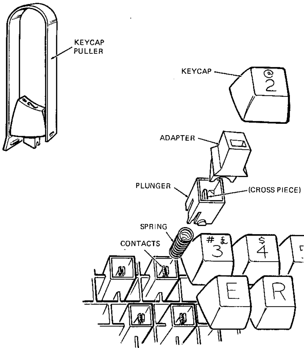
Figure 5-20 Keycap Removal
