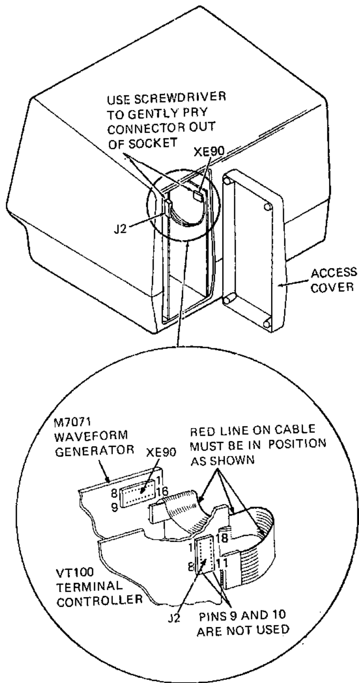
Figure 5-16 VT105 Interconnections
