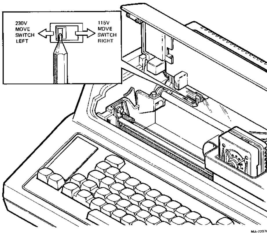
Figure 1-1 Voltage Selector Switch
