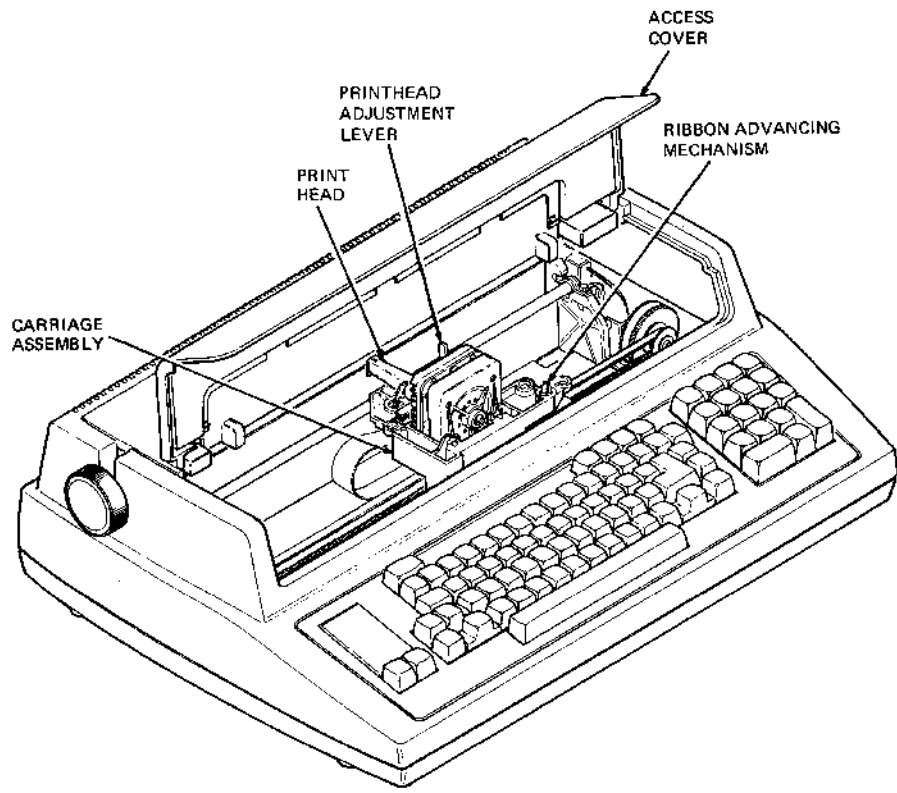
Figure 2-1 Carriage Assembly
