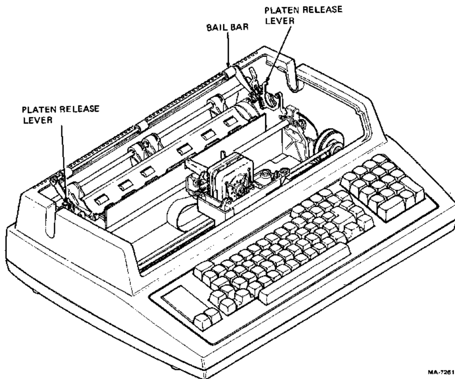
Figure 4-2 Platen Removal
