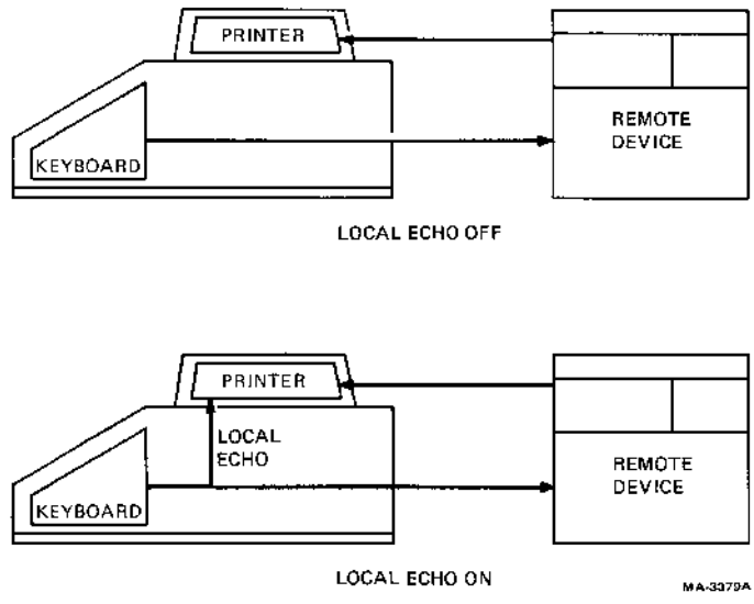
Figure 3-6 Local Echo Feature
