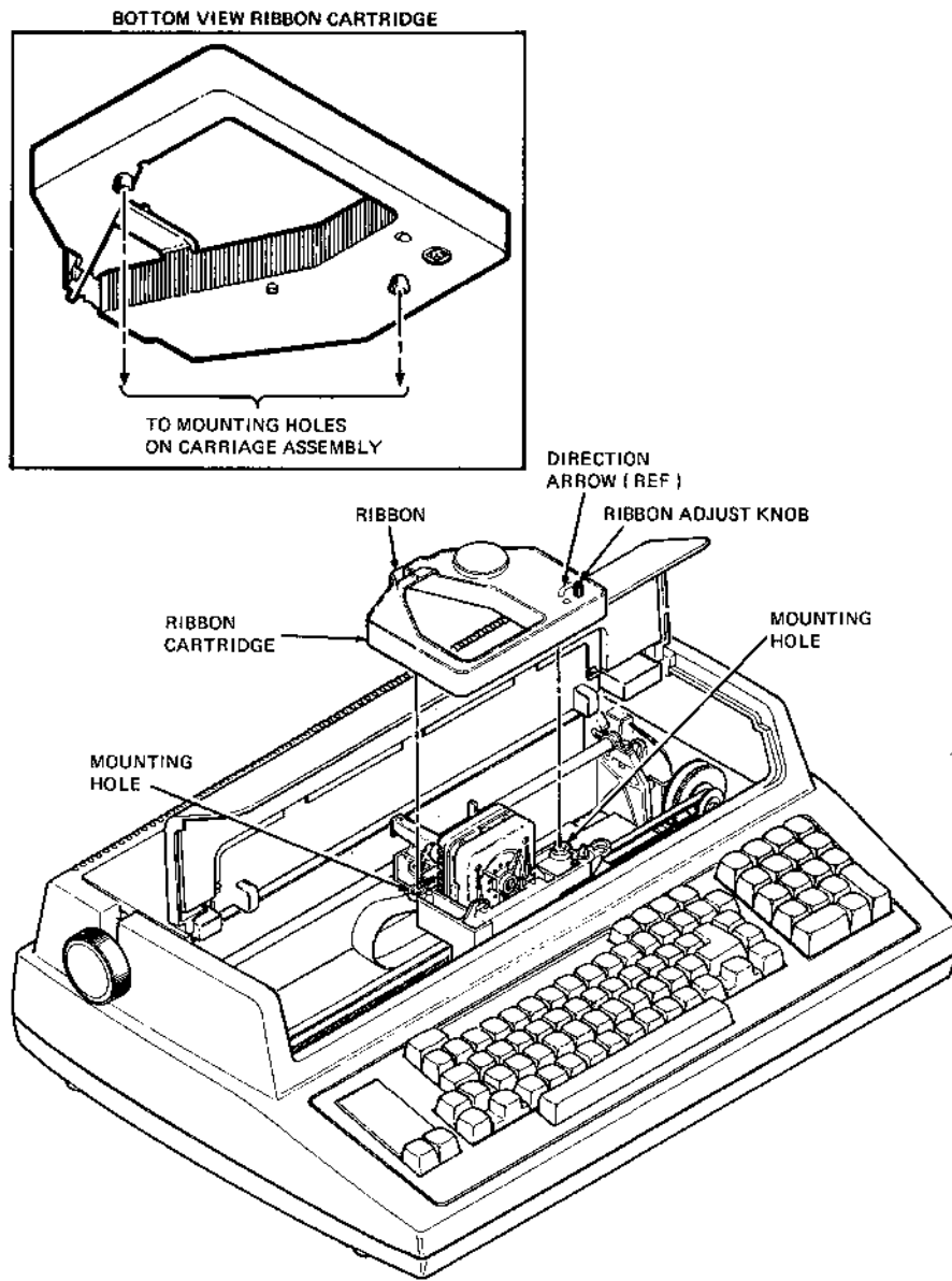
Figure 2-2 Ribbon Cartridge
