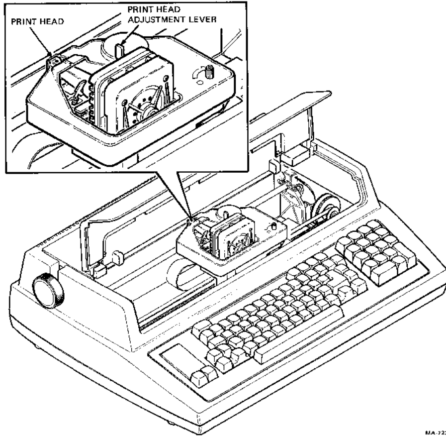
Figure 2-10 Printhead Adjustment
