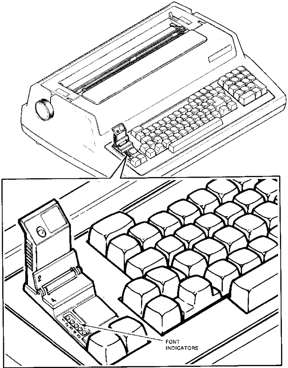
Figure 1-18 Font Indicators
