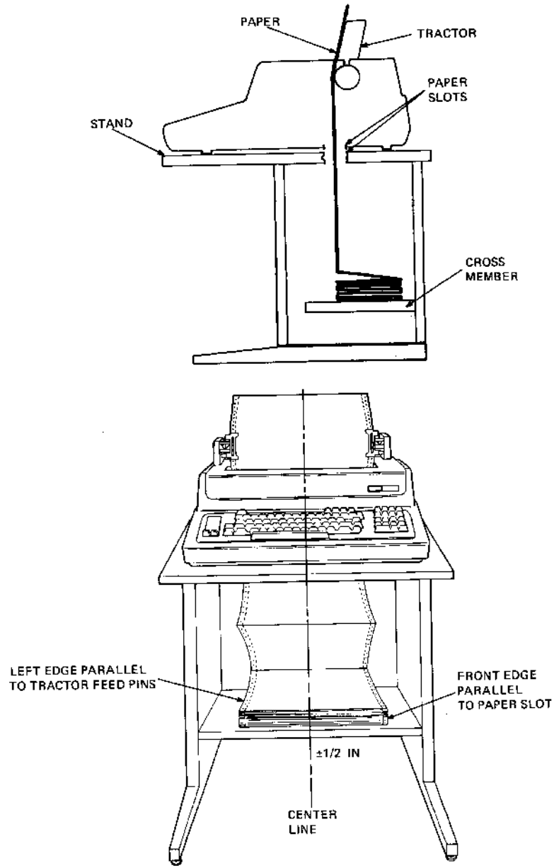
Figure 2-9 Tractor Feed Paper Path (With Stand)
