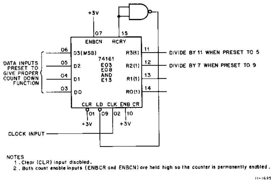
Figure 4-8 74161 Synchronous 4-Bit Counter
