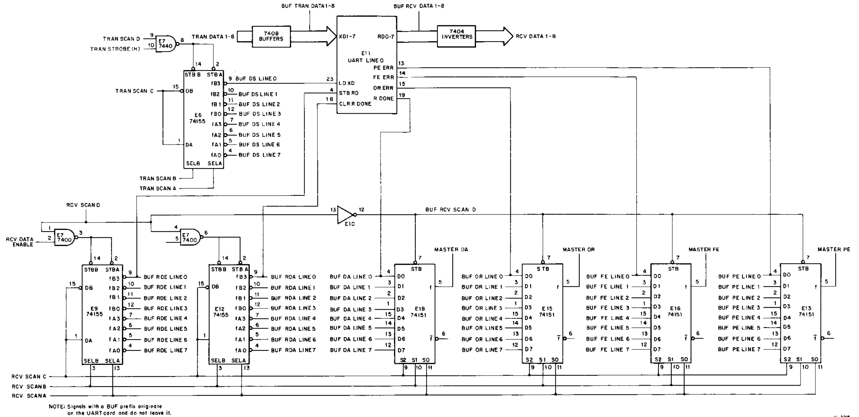
Figure 4-33 Block Diagram of Single UART Showing Decoding of Control Signals and Multiplexing of Flag Signals
