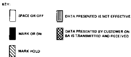
Figure F-4 Data Set 103E Type Sequence Chart for a Call Originated in the Semiautomatic Manner and Answered Automatically
