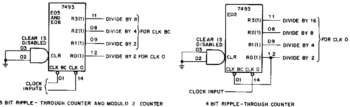
Figure 4-7 7493 4-Bit Binary Counter
