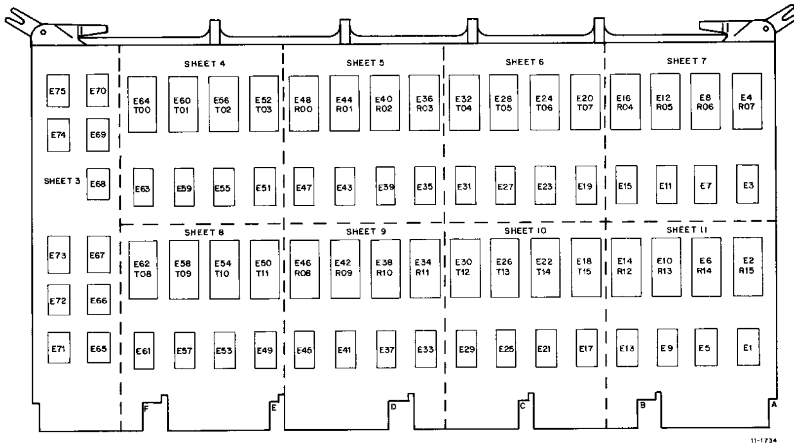
Figure 4-12 Component Layout of M7288 Module
