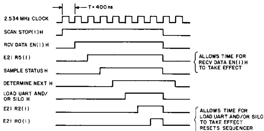
Figure 4-26 Timing Diagram for Receiver Sequencer
