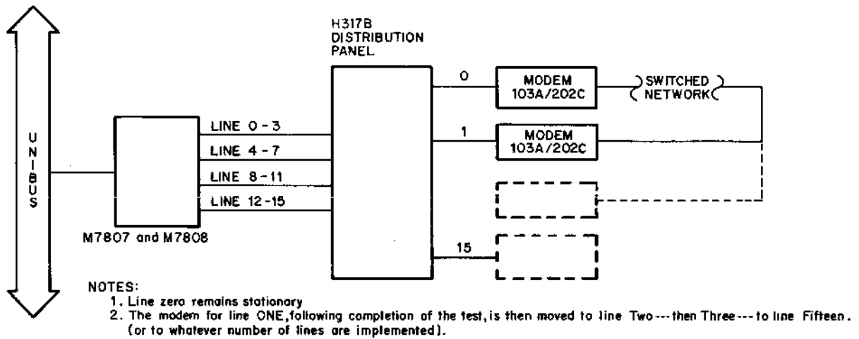
Figure E-6 Test Configuration (ON LINE Modem Loop Back)
