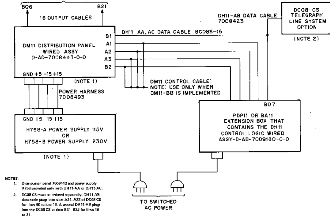
Figure 2-2 DH11-AA, AB, and AC Interconnection Diagram
