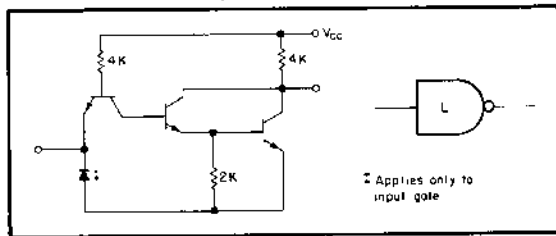
LOW-LEVEL GATE
