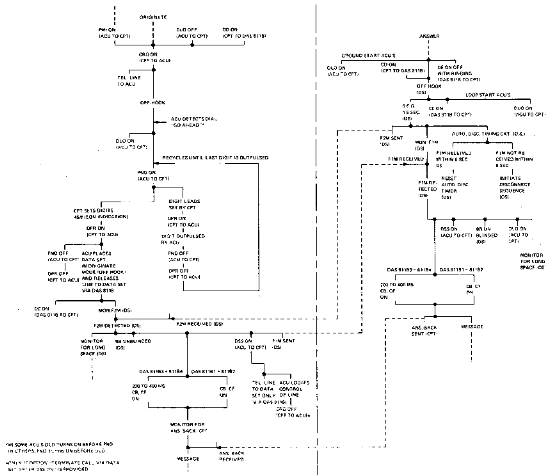
Figure F-9 811B Originating and Answering Flow Chart for CPT for 3 or 4 Row TWX Service Data Set Tone Detection with EON
