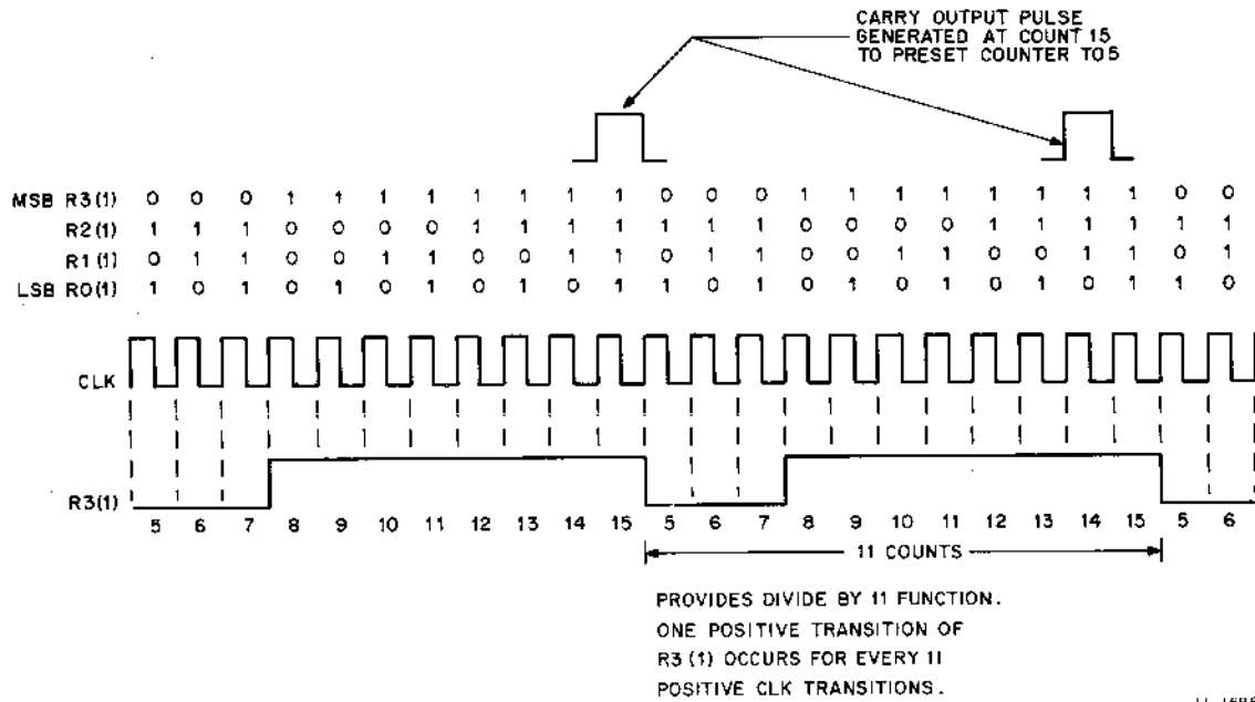
Figure 4-9 Divide by 11 Function of 74161 Counter E03
