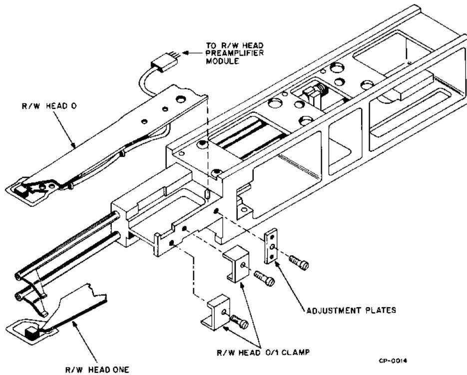
Figure 2-4 Read/Write Carriage Assembly Diagram
