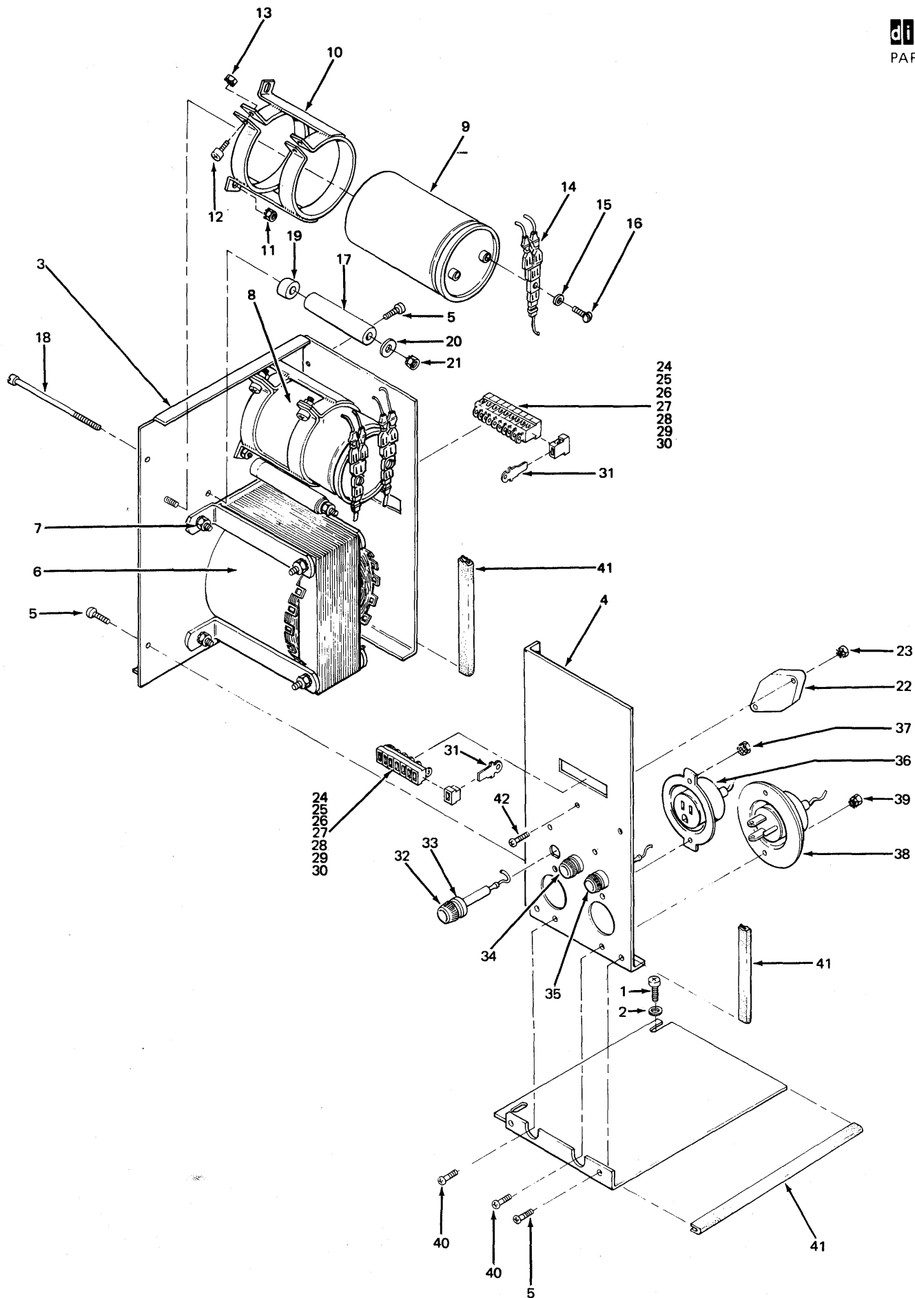
Figure 5. H725 Power Supply
