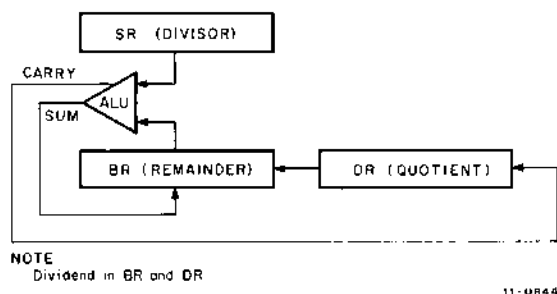
Figure 1-9 Divide Instructions
