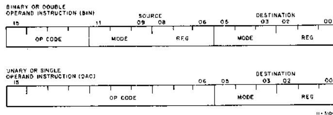
Figure 1-5 Source and Destination Mode Formats
