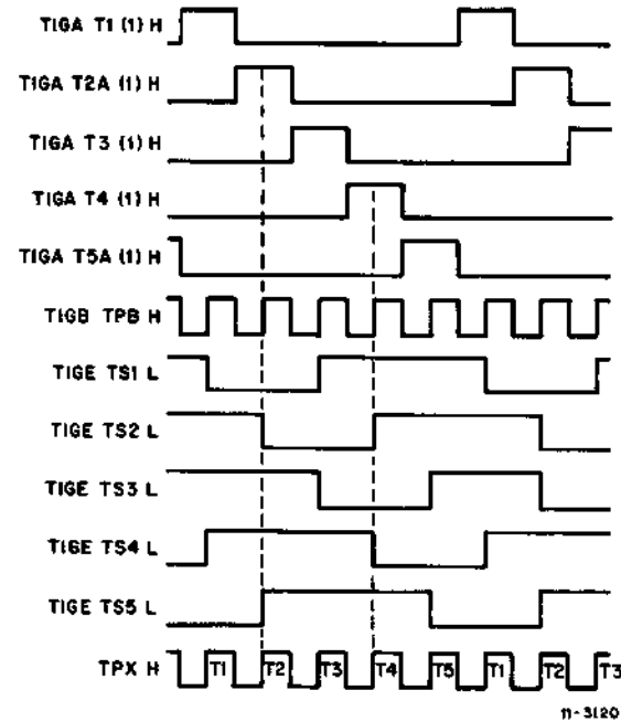
Figure 4-6 Time States
