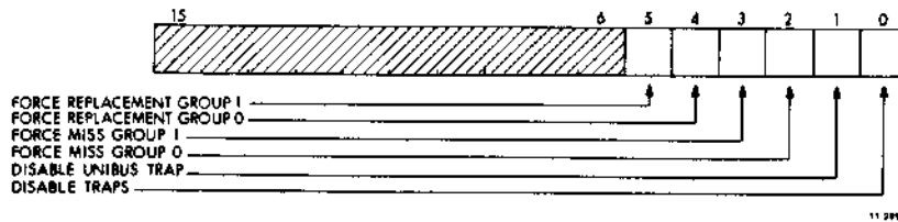
Figure 4-11 Control Register
