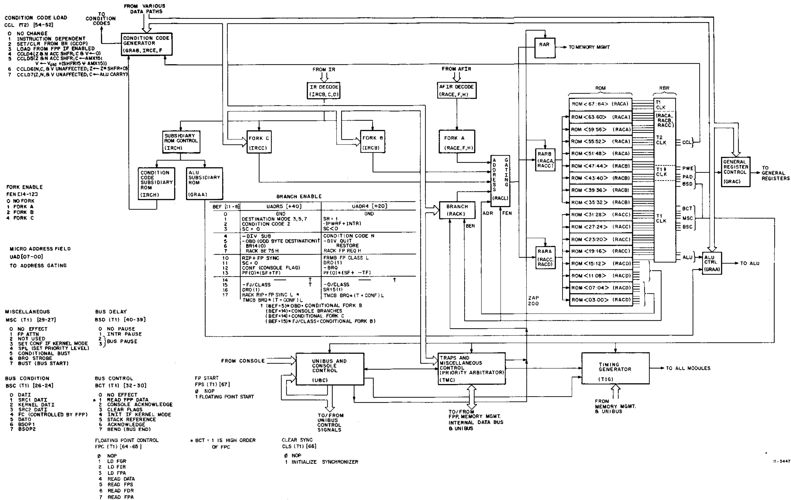
Figure 1-1 Block Diagram
