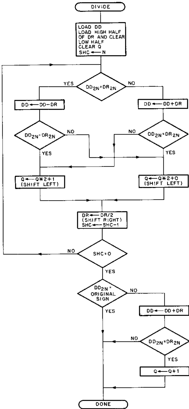
Figure I-8 Divide Algorithm
