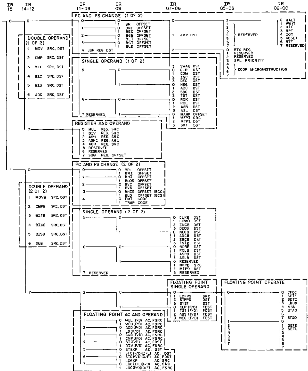
Figure I-10 Determination of an Instruction from the Binary Code
