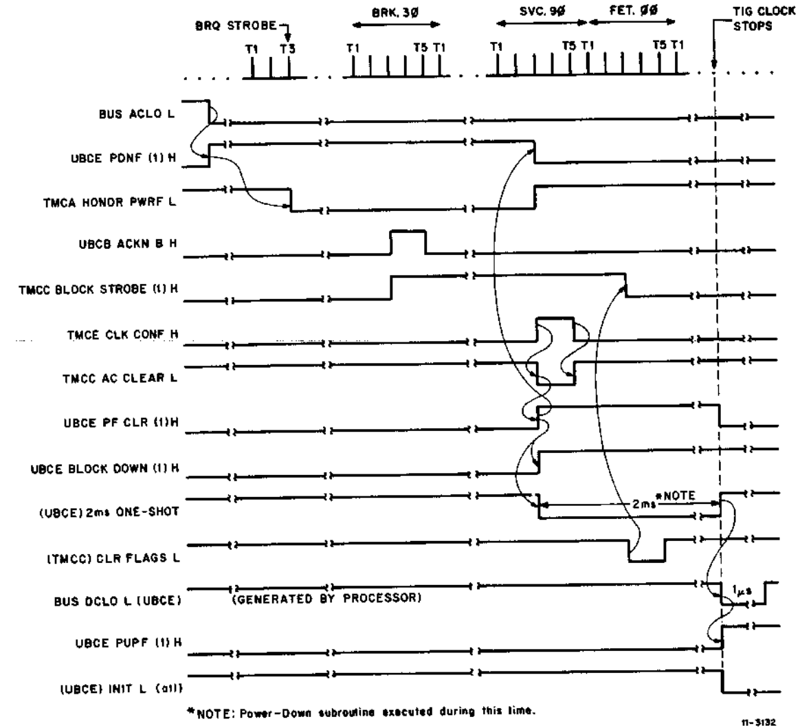
Figure 6-10 Power-Down
