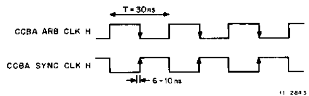
Figure 4-1 Cache Clock Waveforms
