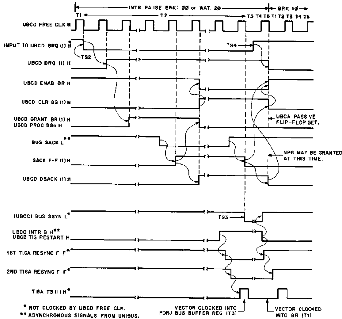
Figure 6-9 INTR Sequence
