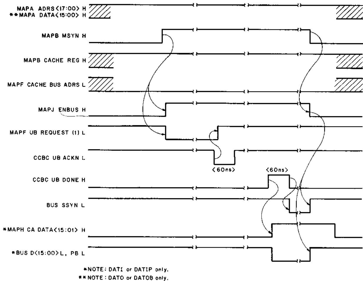
Figure 2-4 Cache/Unibus Transactions
