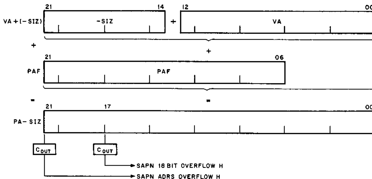
Figure 5-2 18- and 22-Bit Overflow
