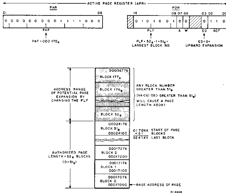
Figure 6-3 Upward Expansion
