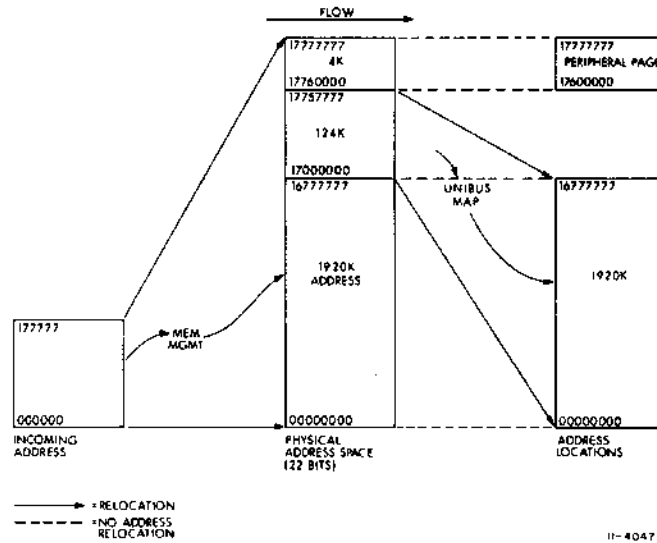
Figure 4-6 22-Bit Mapping
