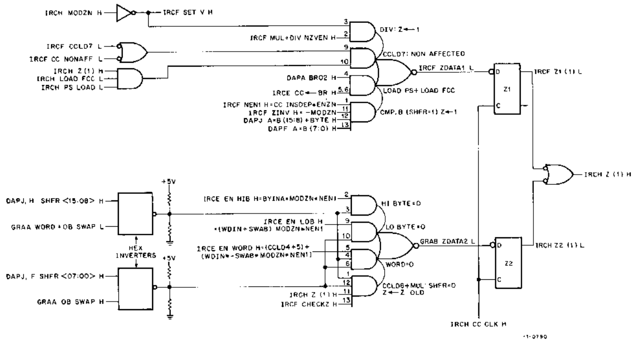
Figure I-15 Sources of Z Bit Data, Simplified Diagram
