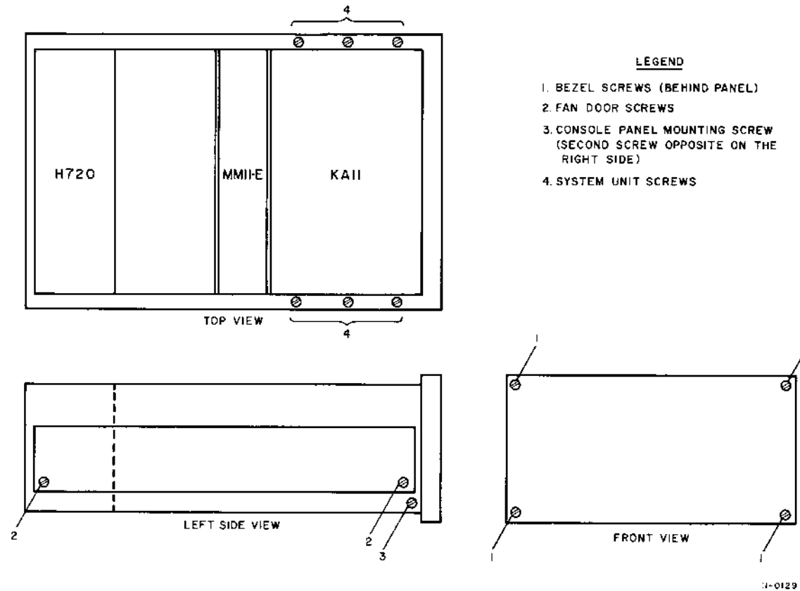
Figure 5-2 Mounting Hardware
