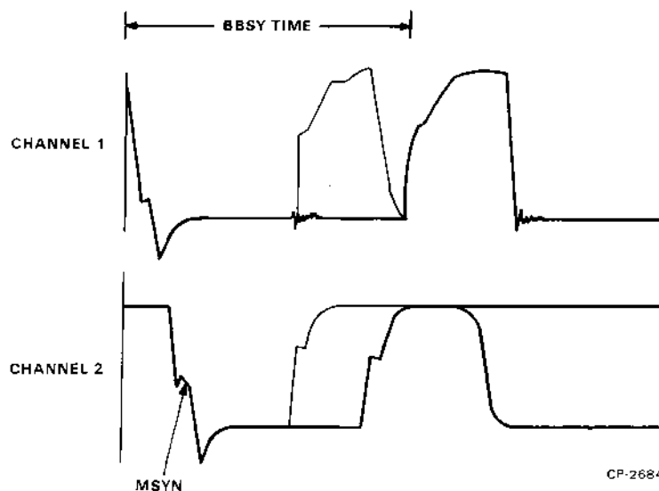
Figure 2-22 Single-Cycle Transaction
