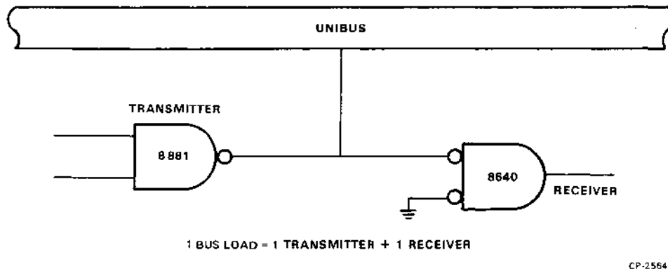
Figure 2-4 Bus Load Example
