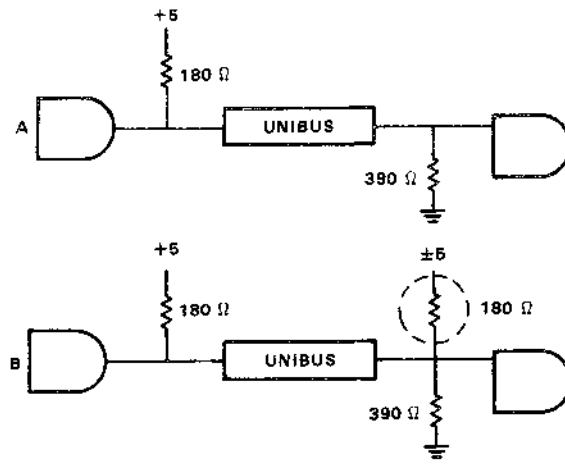
Figure A-3 Grant Line Termination
