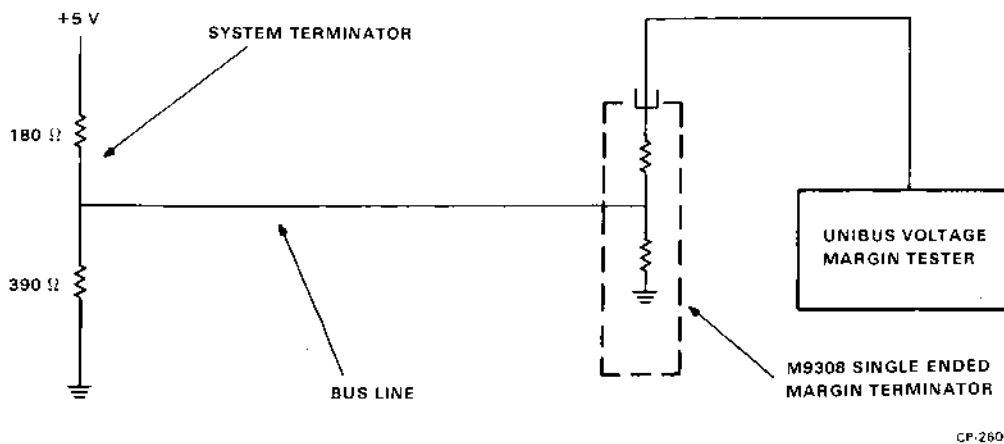
Figure 4-14 Single-Ended Circuit Example
