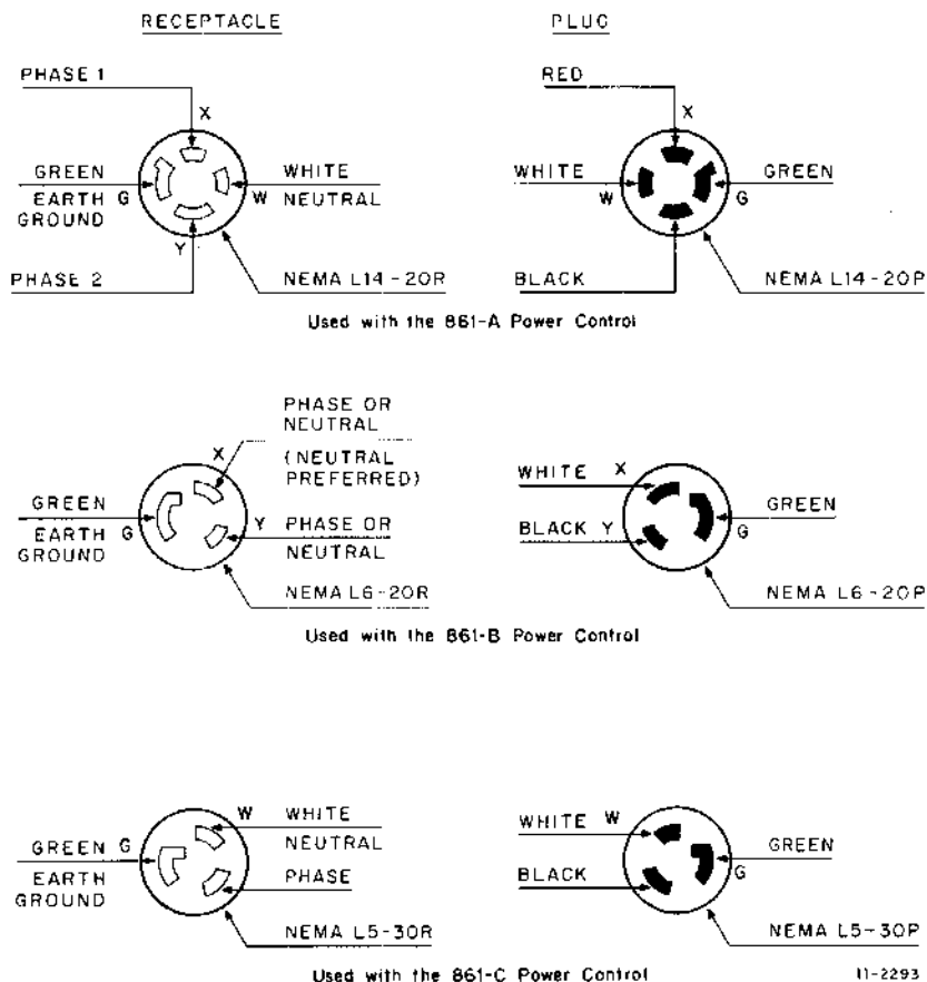
Figure 4-1 Power Connectors
