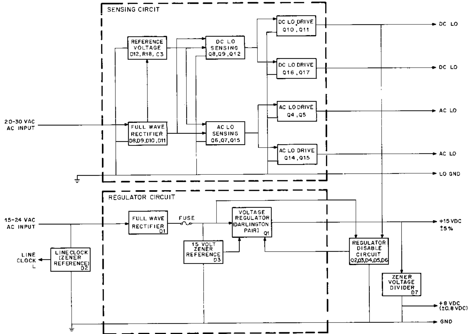
Figure 5-11 5409730 Block Diagram
