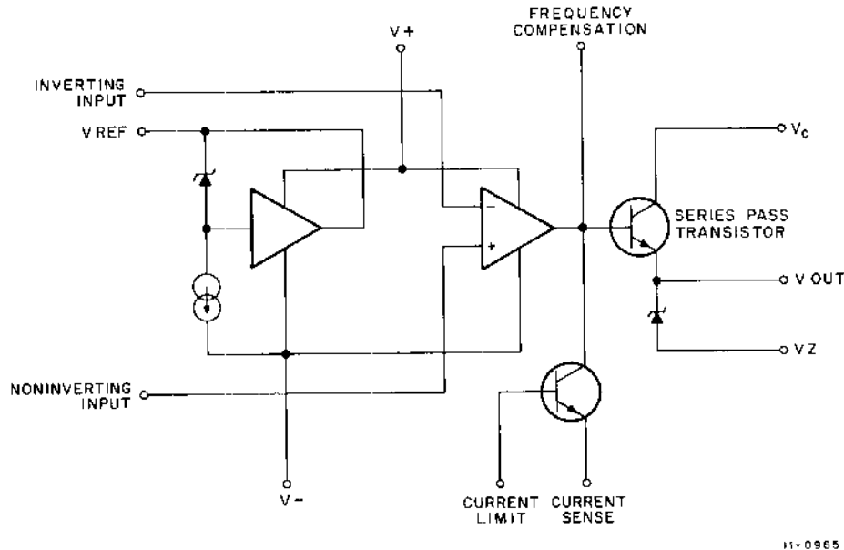
Figure 5-13 Voltage Regulator E1, Simplified Diagram
