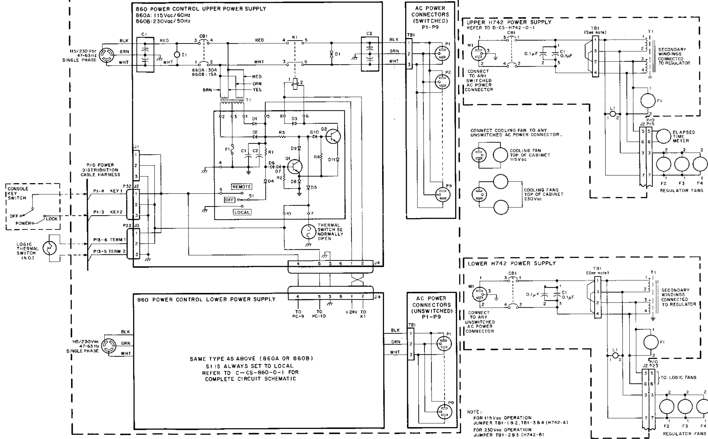
Figure 4-8 AC Power Interconnections (H742 and 860)
