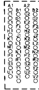
PIN ASSIGNMENTS ONE ROW-ONE SLOT SECTION
