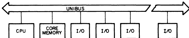
Figure 1-1 PDP-11 System Simplified Block Diagram
