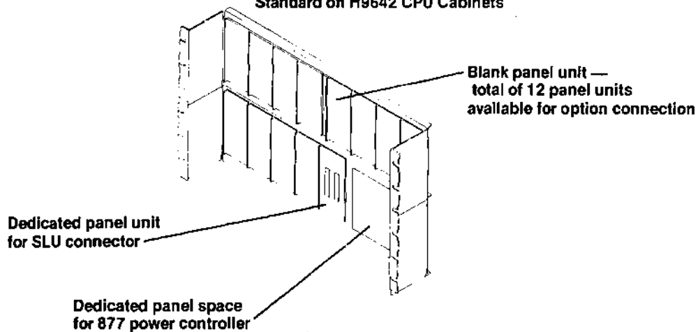
Horizontal I/O Connection Panel
