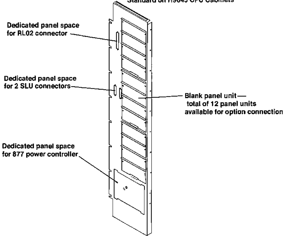
Vertical I/O Connection Panel Standard on H9645 CPU Cabinets
