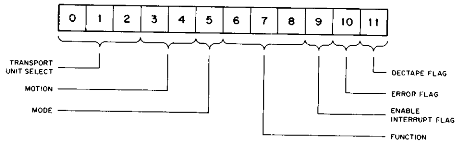
Figure 2-5 Status Register A, Format
