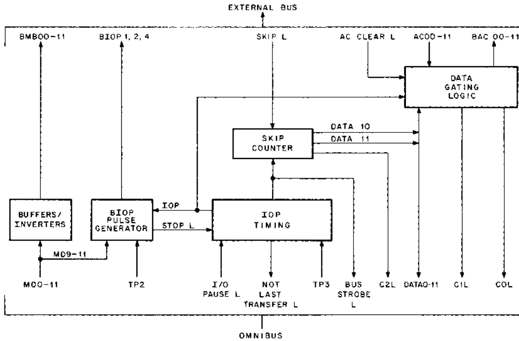
Figure 1-1 Positive I/O Bus Interface, Block Diagram
