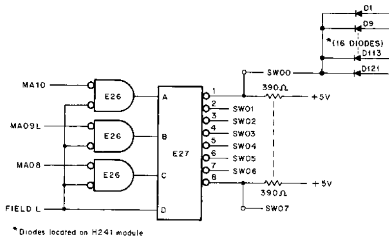
Figure 3-4 Switch Select Logic
