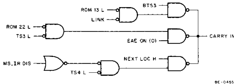
Figure 1-34 EAE Carry In Logic
