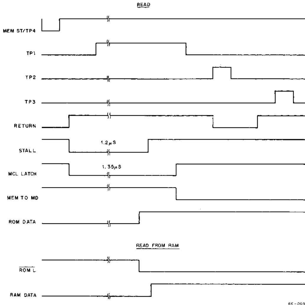
Figure 1-3 Read Timing
