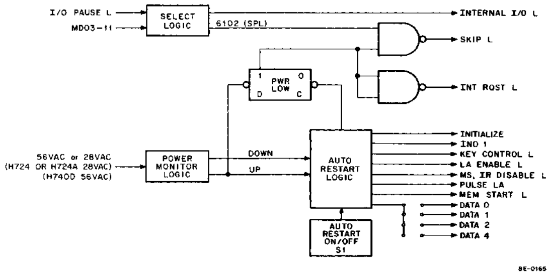
Figure 1-1 M848 Power-Fail and Auto-Restart Option, Block Diagram
