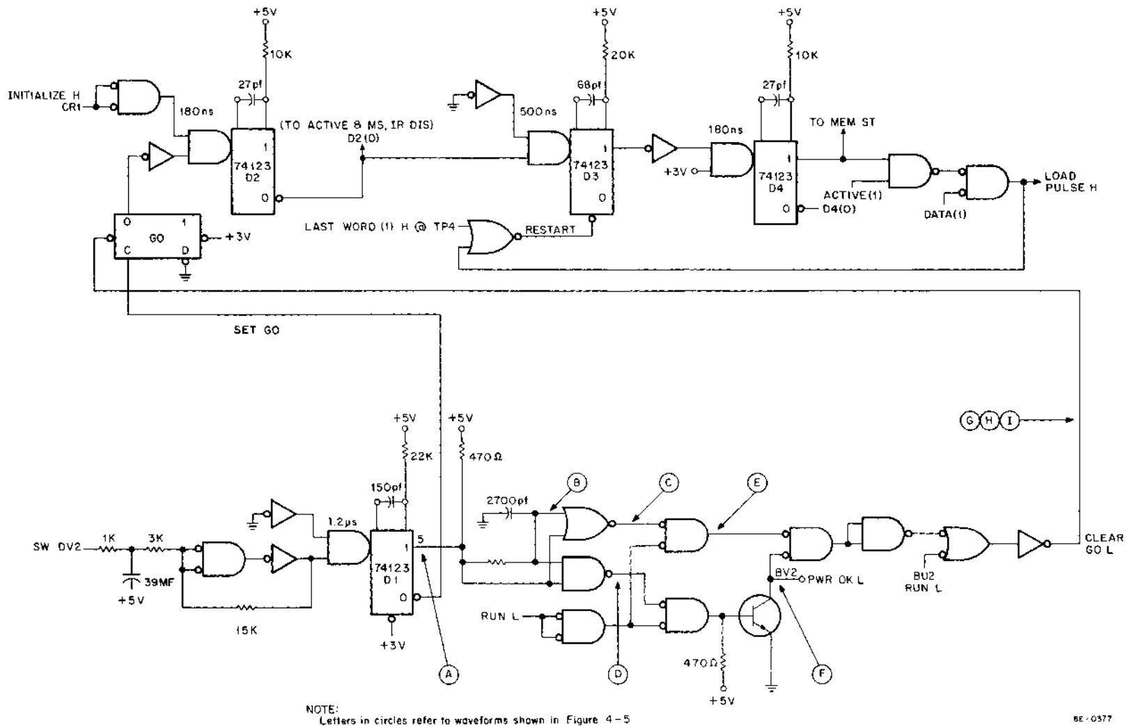
Figure 4-3 Bootstrap Timing Logic
