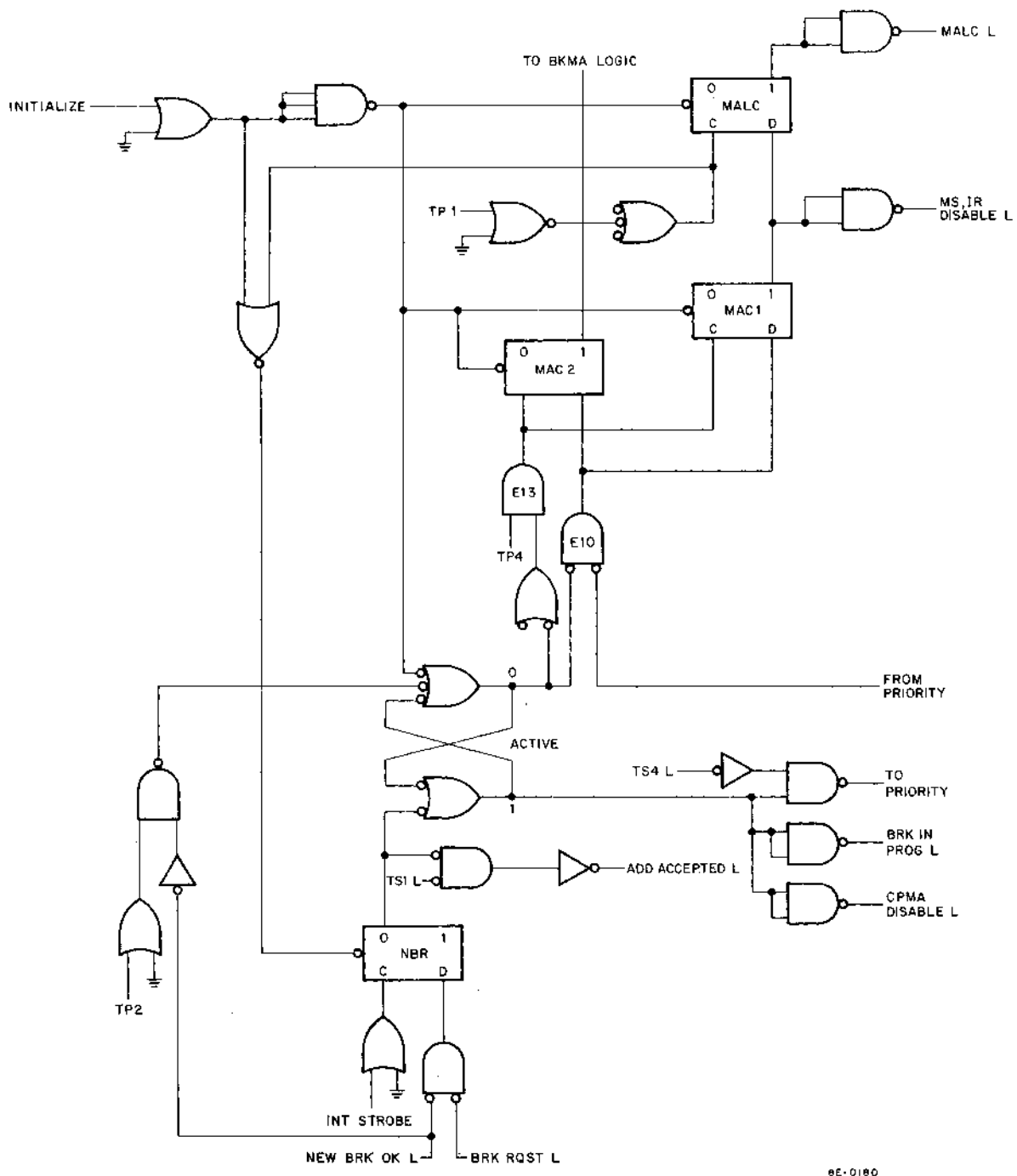
Figure 2-2 CP Register Control Logic
