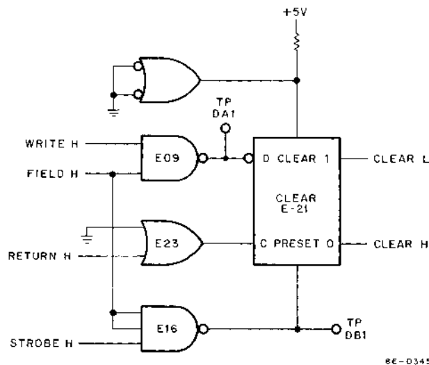
Figure 3-8 Clear Logic
