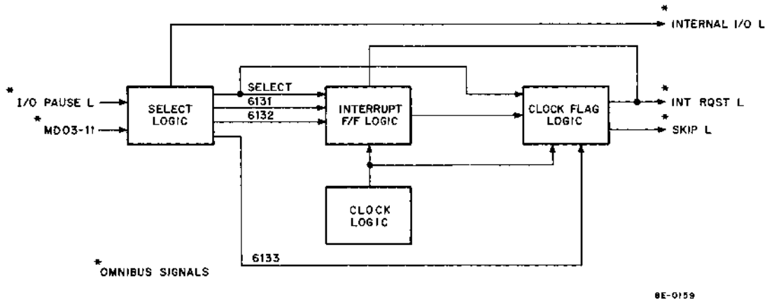
Figure 1-1 Real-Time Clock (DK8-EA, DK8-EC), Block Diagram
