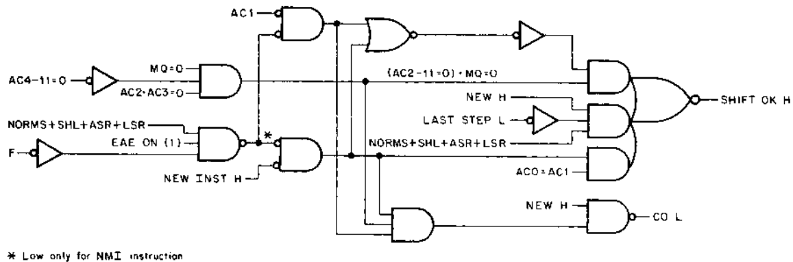
Figure 1-33 Shift OK Logic
