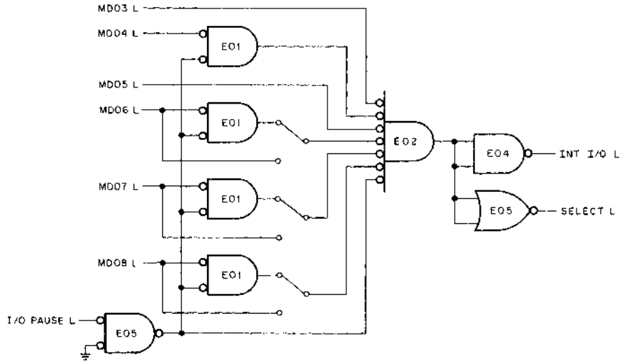
Figure 1-2 Device Select Logic
