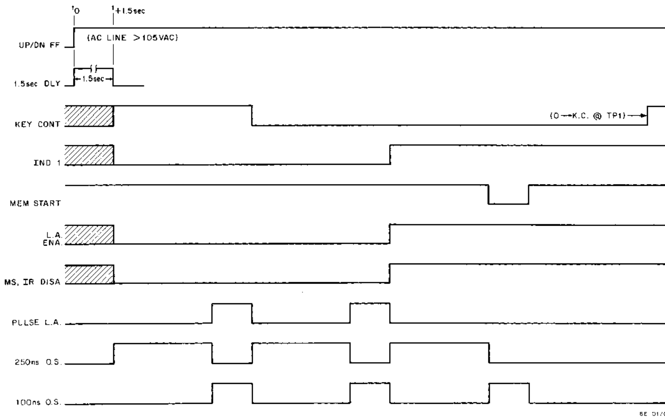
Figure 1-6 Auto-Restart Timing
