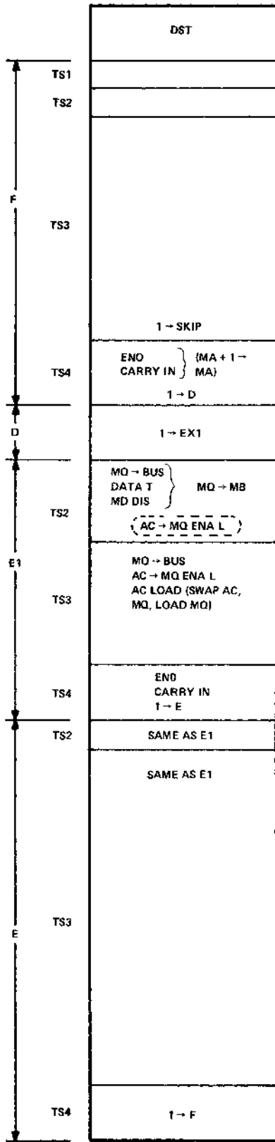
Figure 1-10 DST Instruction, Flow Diagram
