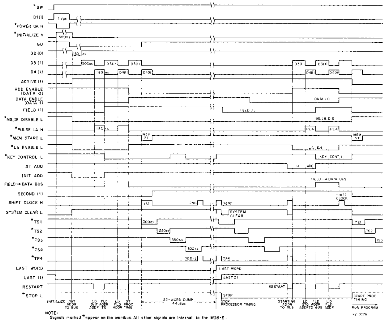
Figure 4-2 Bootstrap Timing
