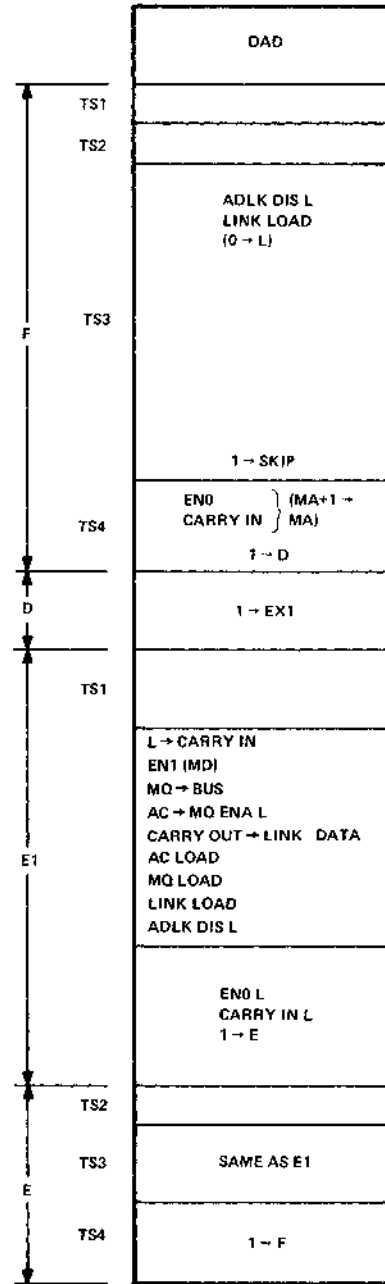
Figure 1-11 DAD Instruction, Flow Diagram
