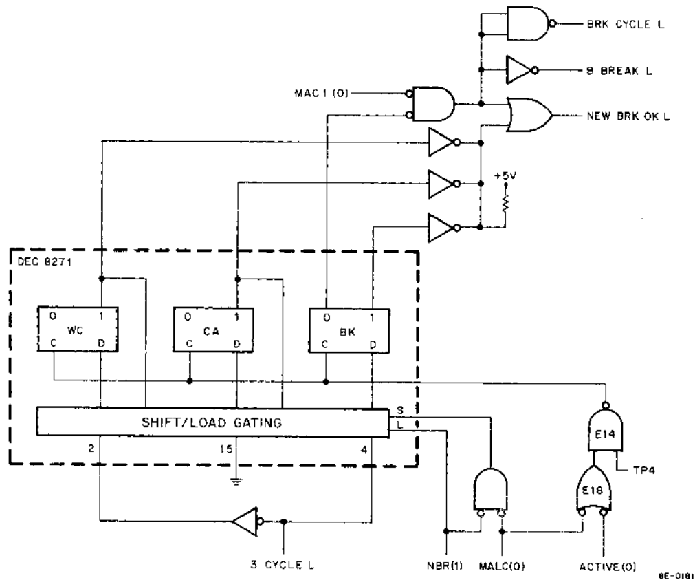
Figure 2-3 Cycle Select Logic
