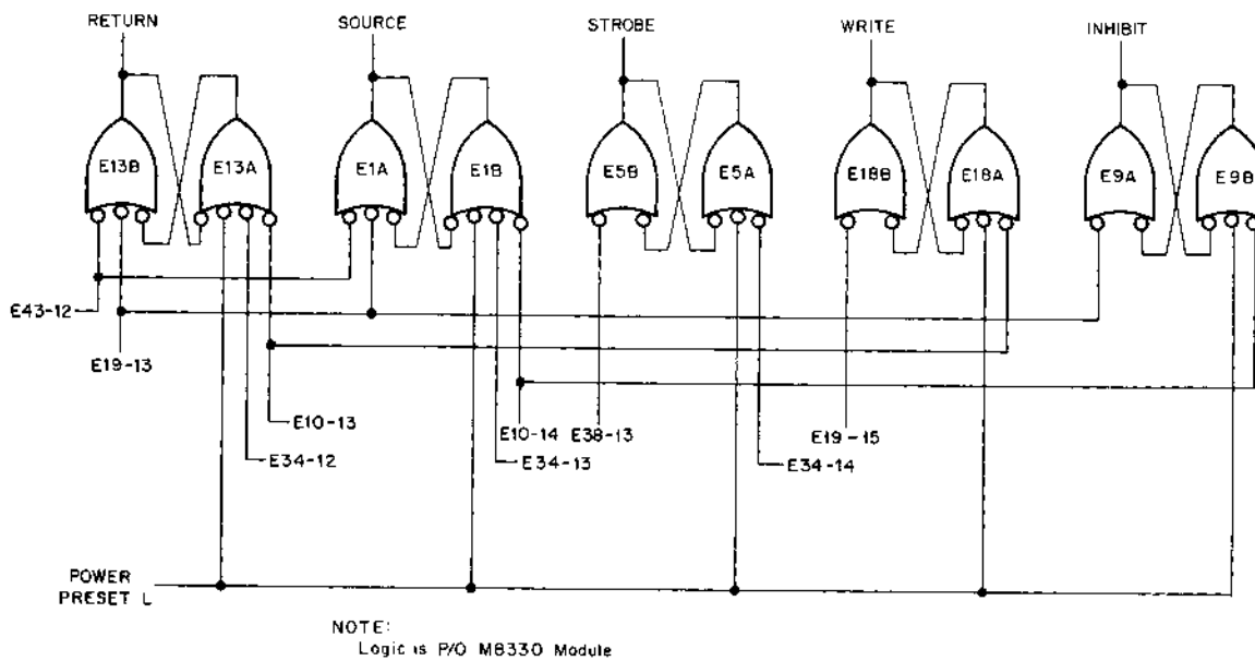
Figure 3-28 Memory Timing Signal Logic
