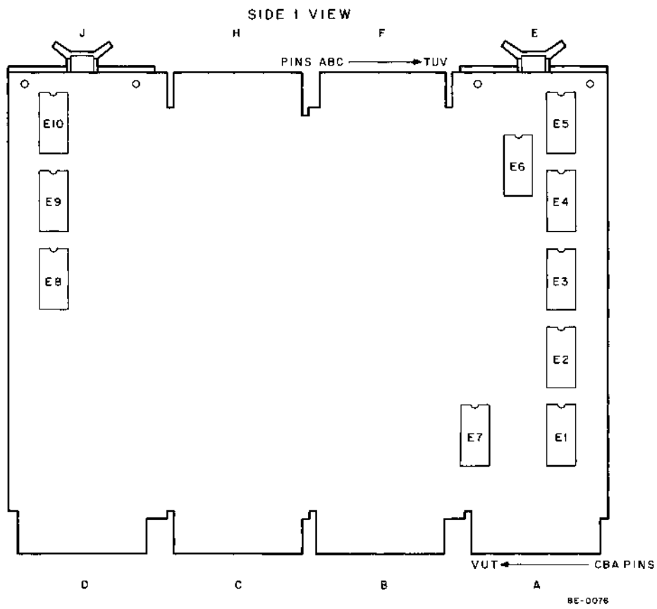
Figure 4-2 IC Location
