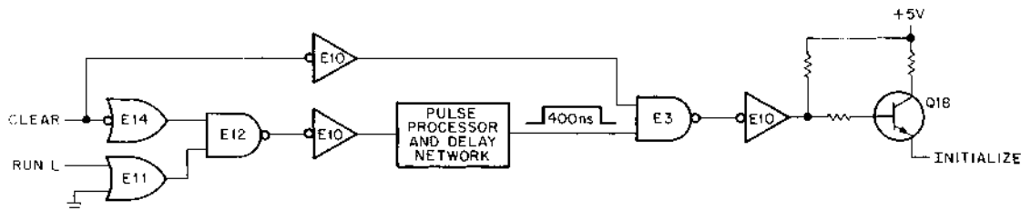
Figure 3-74 CLEAR Key Logic
