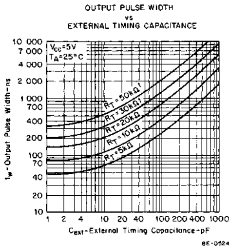
Figure A-22 DEC 74123 IC Output Pulse width vs. External Timing Capacitance
