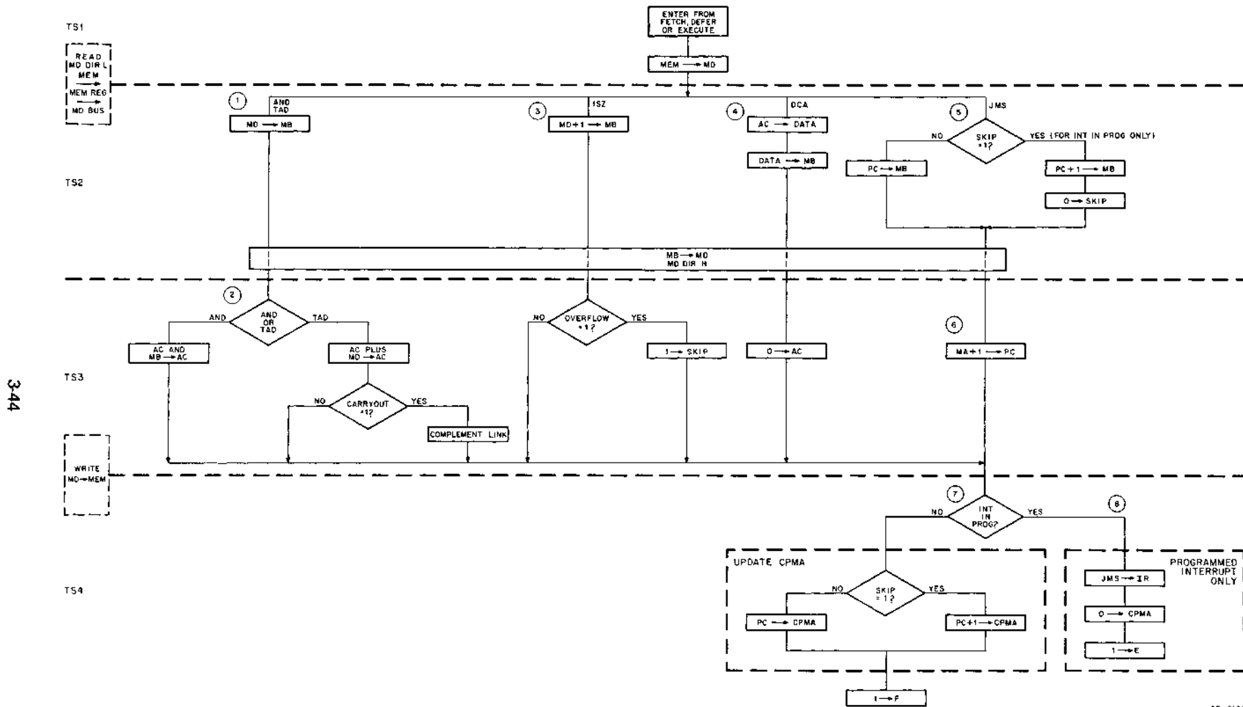
Figure 3-18 EXECUTE State Instruction Flow Diagram
