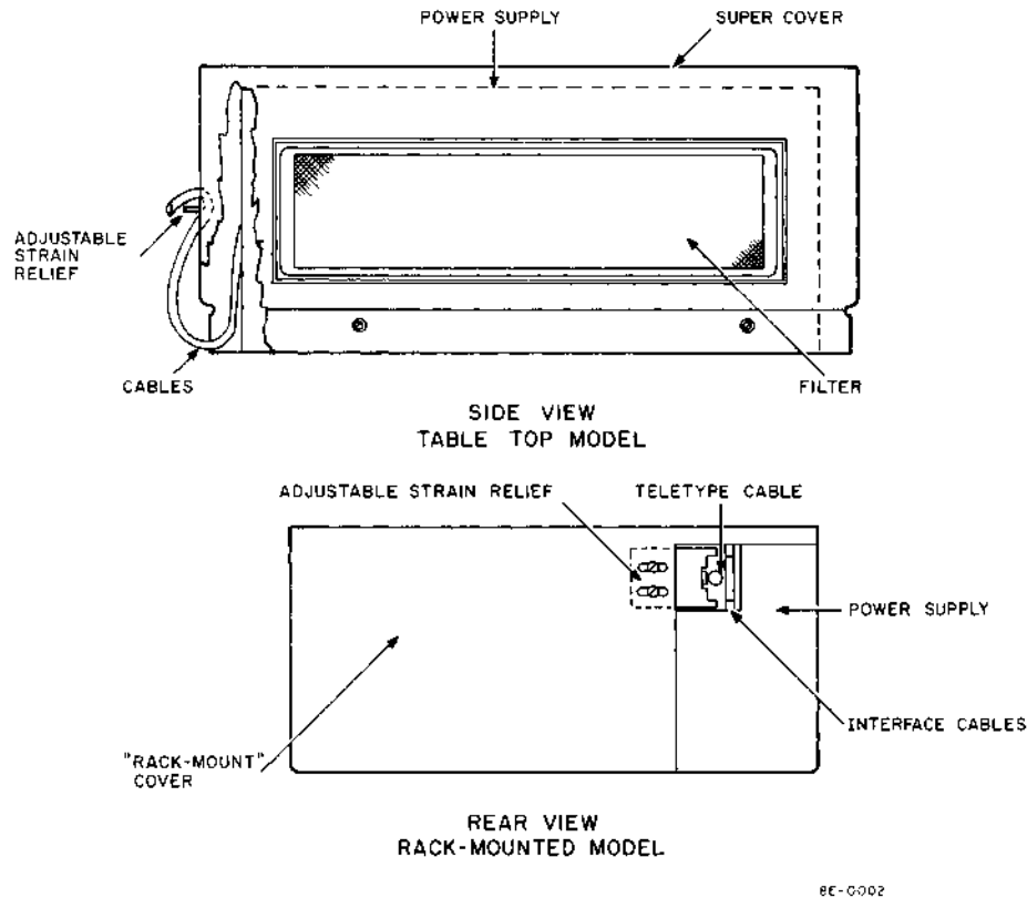
Figure 2-1 Rack-Mounted and Table-Top Models
