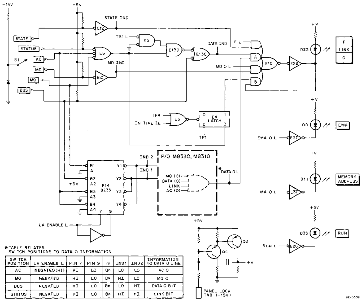
Figure 3-85 Display Logic
