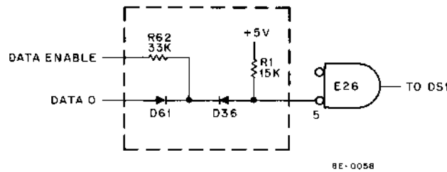
Figure 3-78 Enable Circuit
