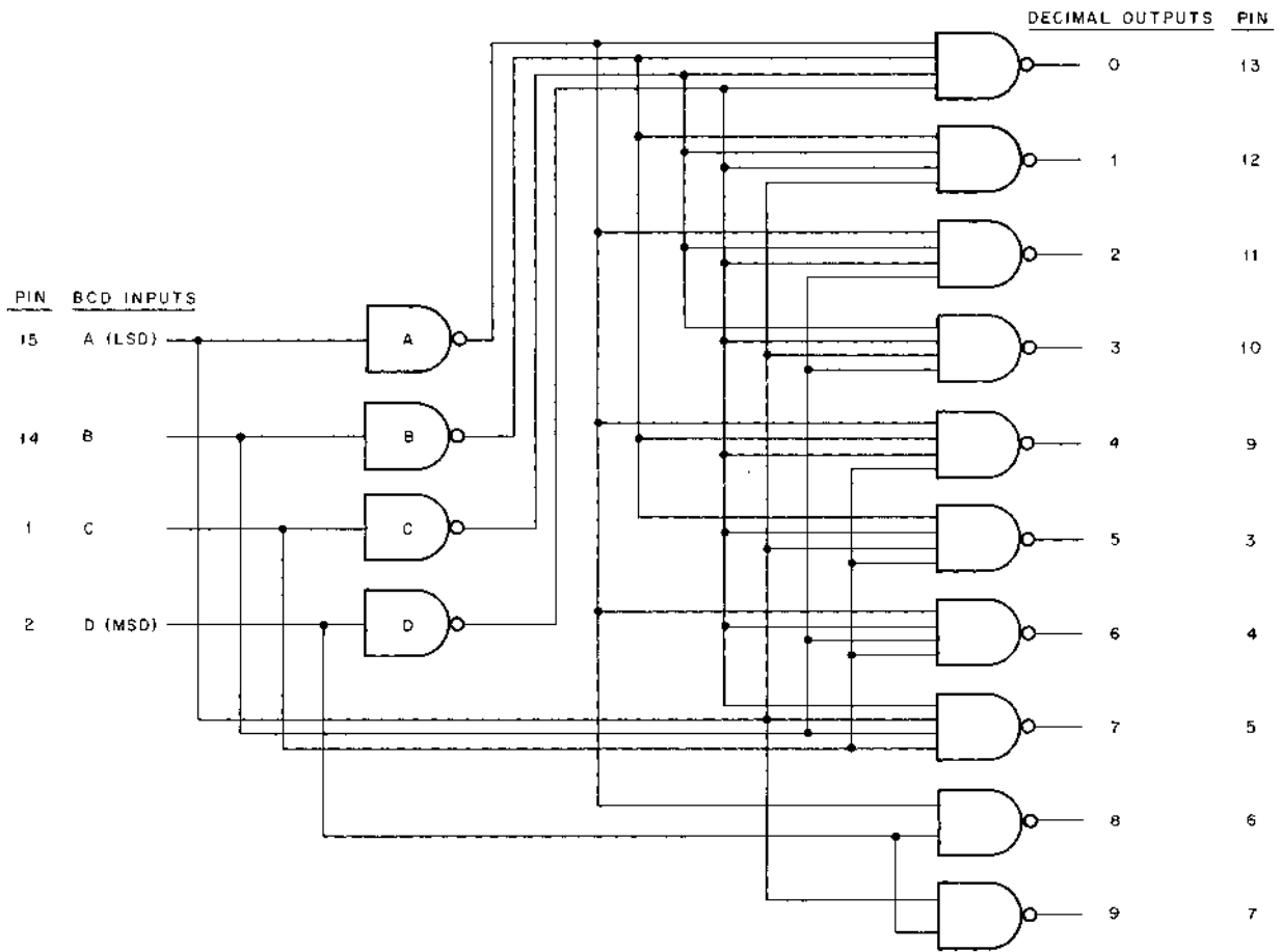
LOGIC DIAGRAM
