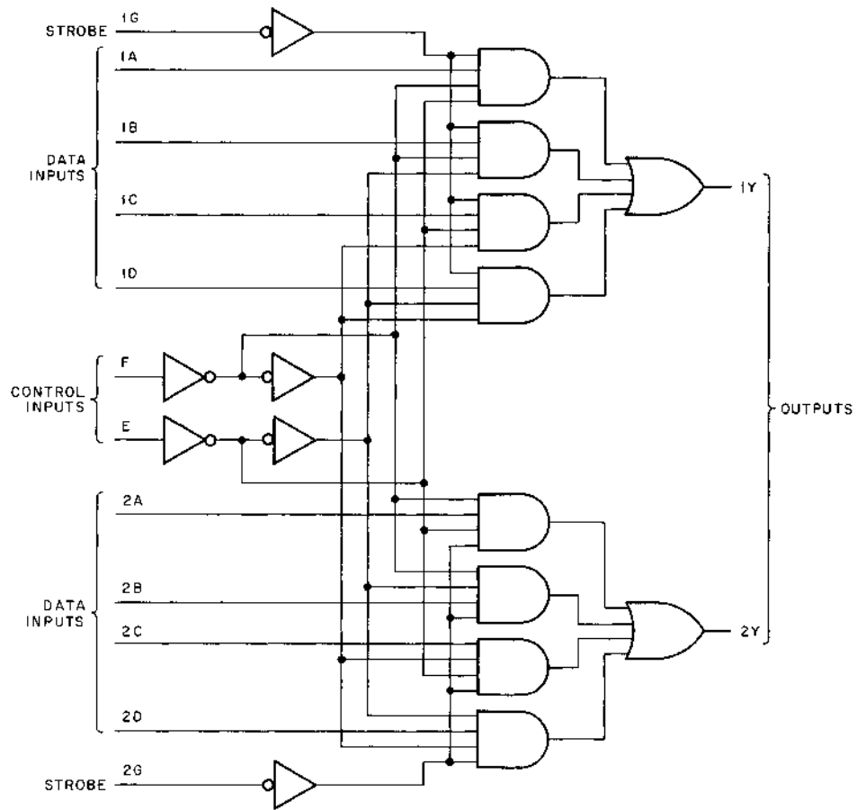
LOGIC DIAGRAM
