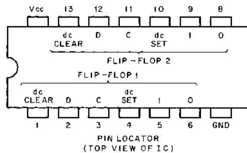
Figure A-1 DEC 7474 and 74H74 IC Illustrations
