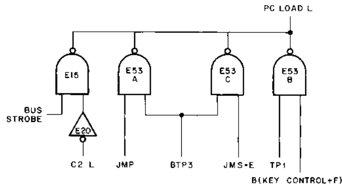
Figure 3-97 PC LOAD Logic
