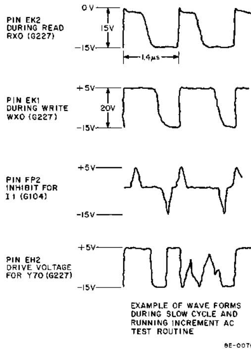
Figure 4-5 Memory Waveforms
