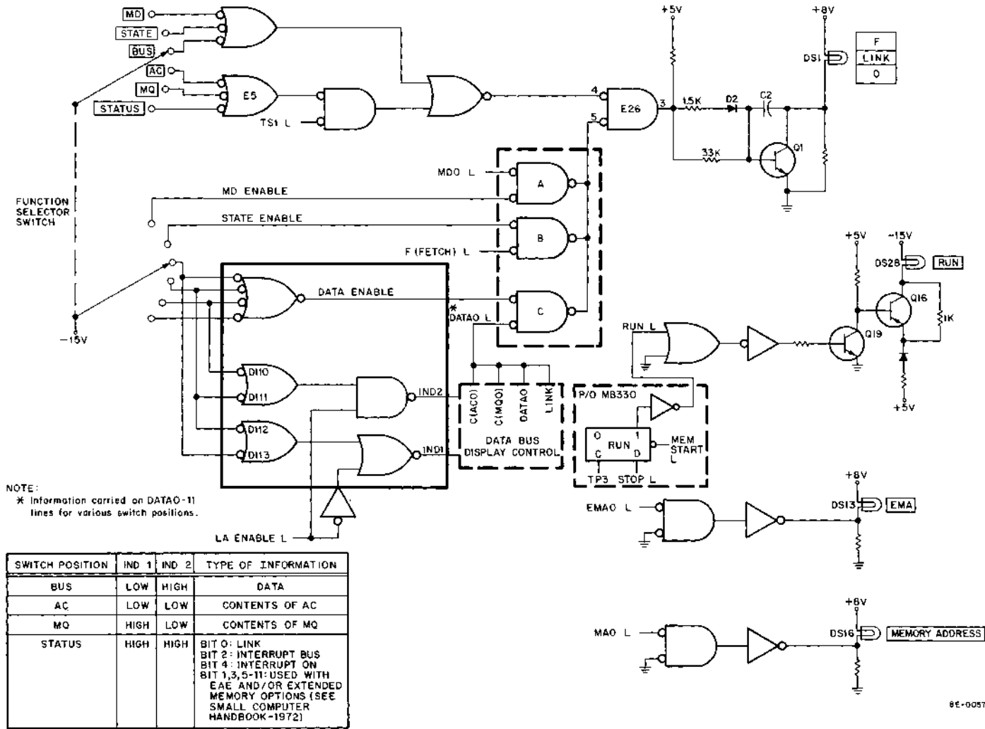
Figure 3-76 Display Logic
