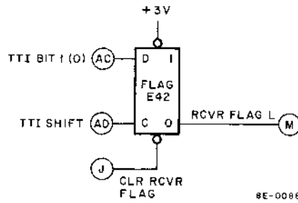
Figure 3-115 RCVR Flag
