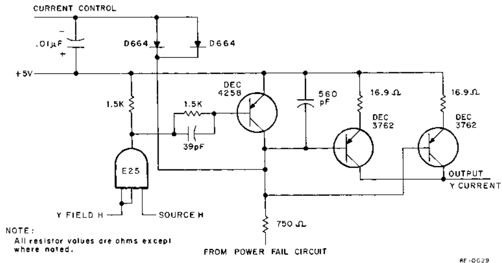
Figure 3-43 Y-Current Source
