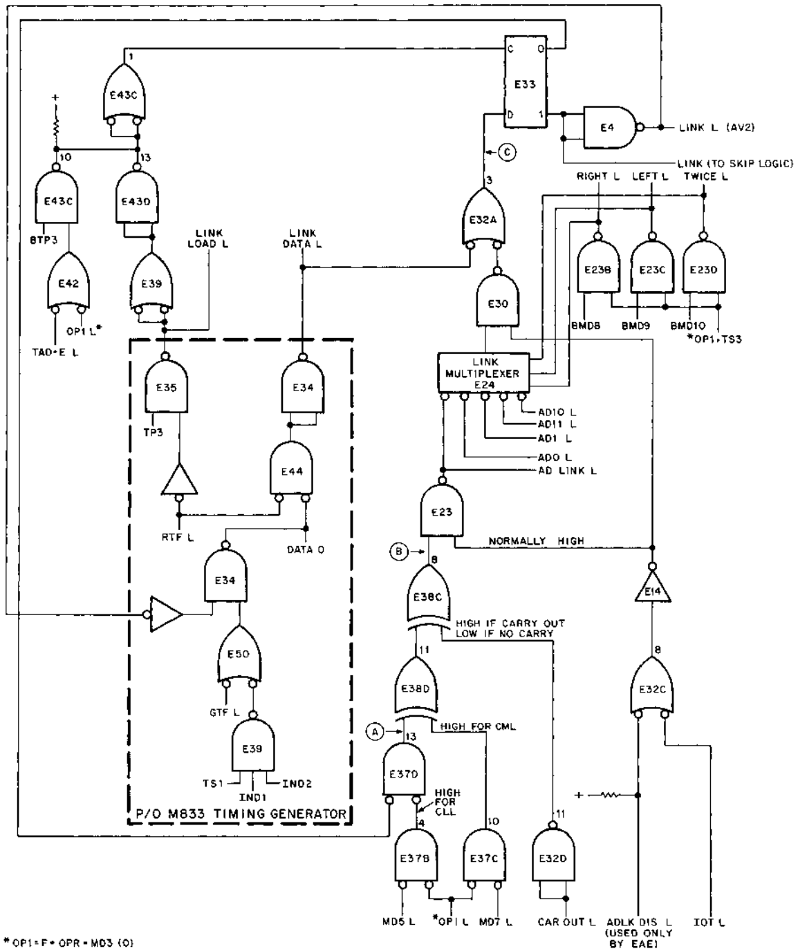
Figure 3-100 Link Logic
