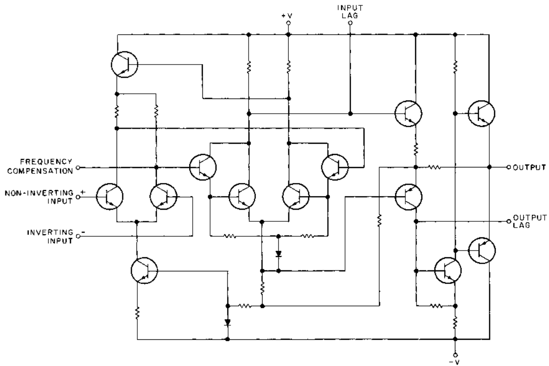
SCHMATIC
