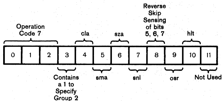
Figure 8 Group 2 Operate Instruction Bit Assignments
