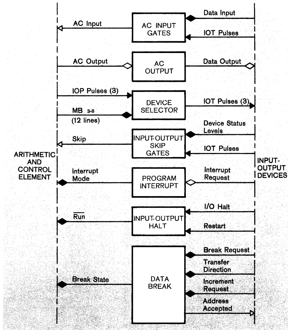
Figure 9 Input-Output Control Element
