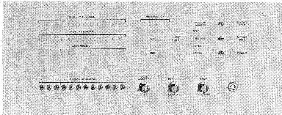
Figure 4 Operator Console
