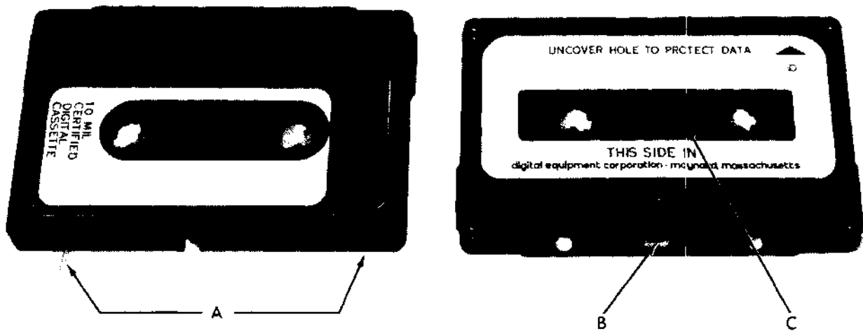
Figure 1-2 CAPS-8 Cassette
