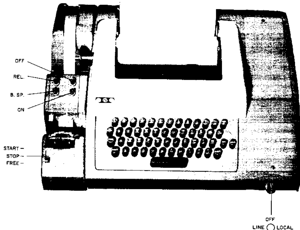
Figure INTRO-2 ASR33 Teletype Console
