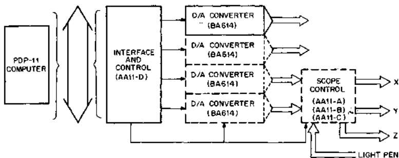
AA11-D Subsystem
