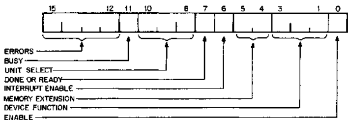
Figure 2-2 Control & Status Register
