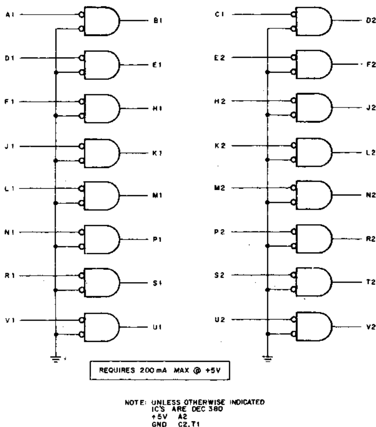
Figure 6-14 M784 UNIBUS Receiver (schematic diagram)
