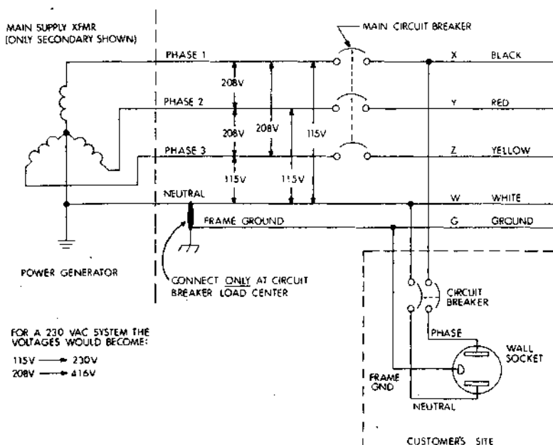
Figure 8-4 Power Wiring Schematic for 115 VAC
