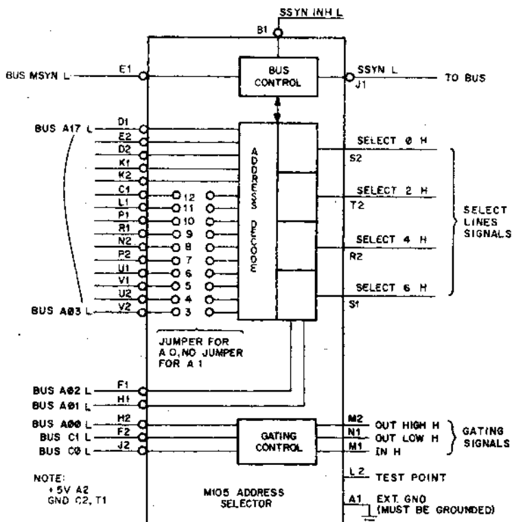
Figure 6-10 M105 Address Selector
