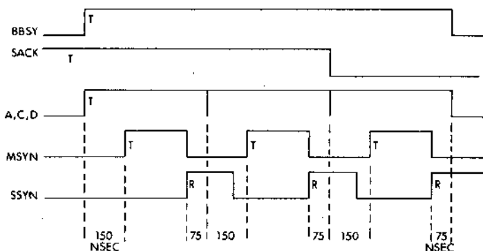
Figure 5-14 Device Multi-Word Transfers
