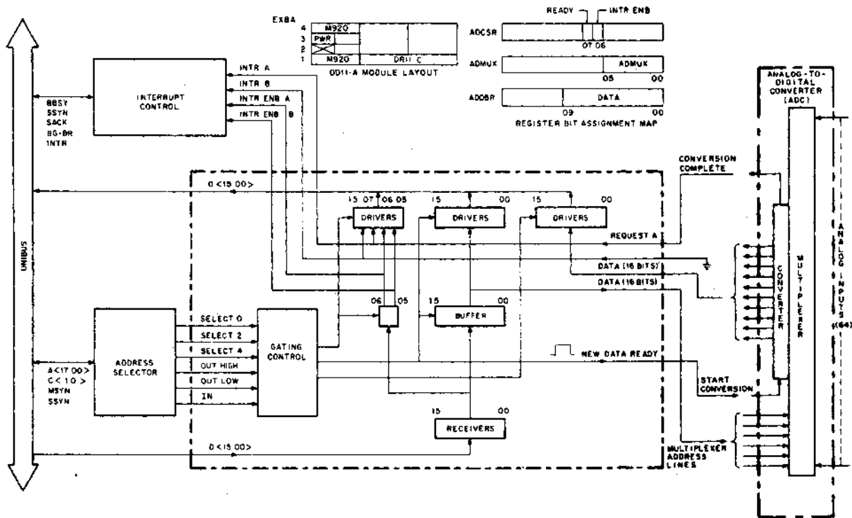
Figure 7-6 DR11-C Implementation (block diagram)
