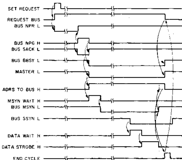
Figure 6-20 M796 Timing Diagram for DAT1
