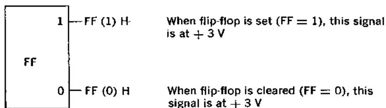
Figure 6-2 Flip-flop signals
