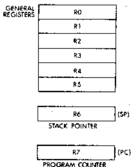
Figure 2-3 General Registers
