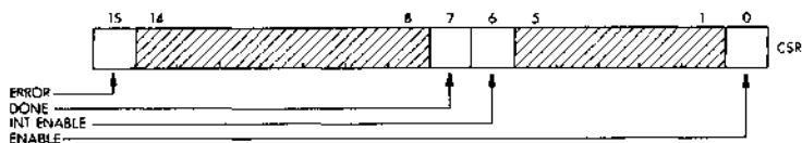
Figure 2-5 CSR Register
