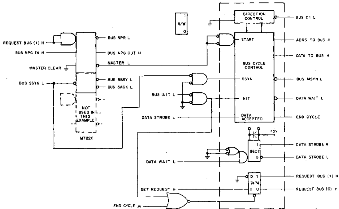
Figure 6-18 M796 UNIBUS Master Control (typical use)
