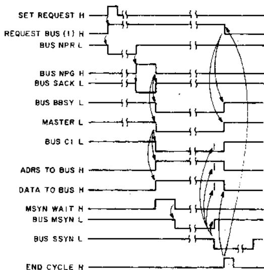
Figure 6-19 M796 Timing Diagram for DAT0
