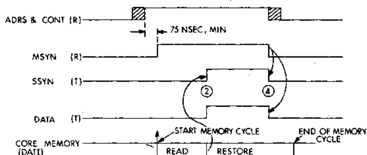
Figure 5-8 DATI & DATIP Timing Diagram
