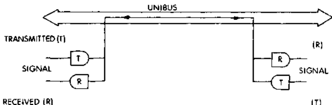
Figure 5-5 Bi-directional Signal
