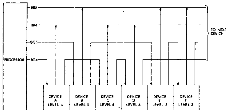
Figure 5-16 Priority Chaining Example
