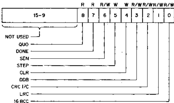
STATUS REGISTER
