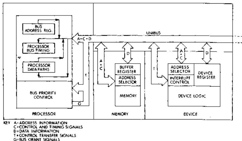
Figure 5-2 PDP-11 Interface Block Diagram
