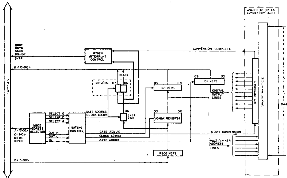
Figure 7-5 Interrupt Serviced Interface (block diagram)
