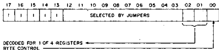
Figure 6-11 Device Register Select Address Format
