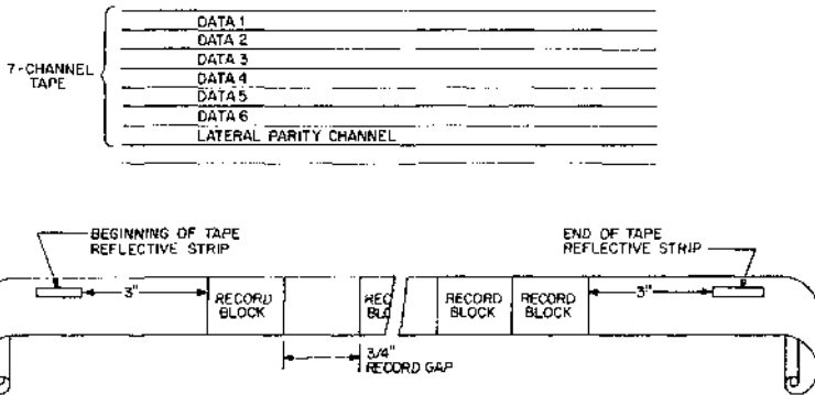
Figure 3-3 - Magtape Format
