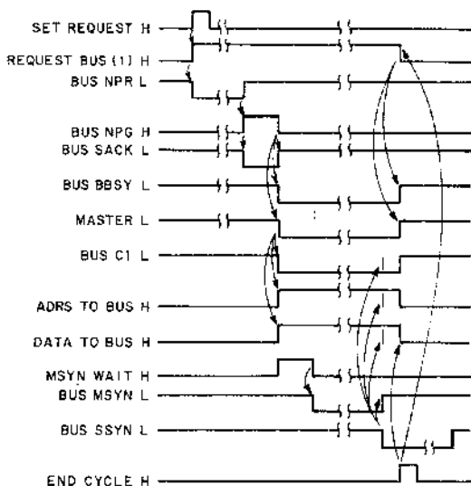
Figure 2-22 M796 Timing Diagram for DAT0
