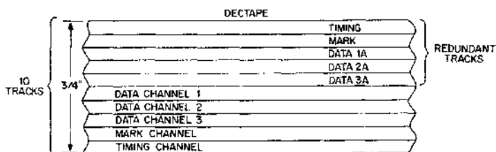
Figure 3-1 - DECTape Format
