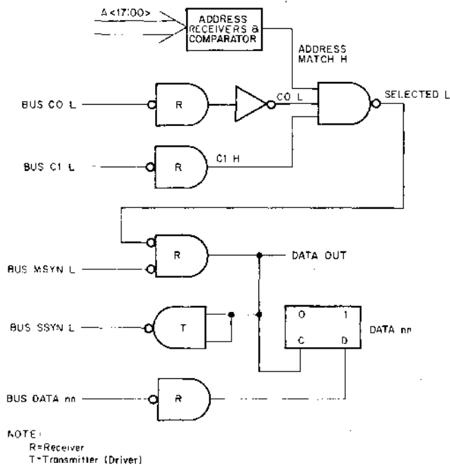
Figure 1-10 Slave Logic For DATO (Fast Response)
