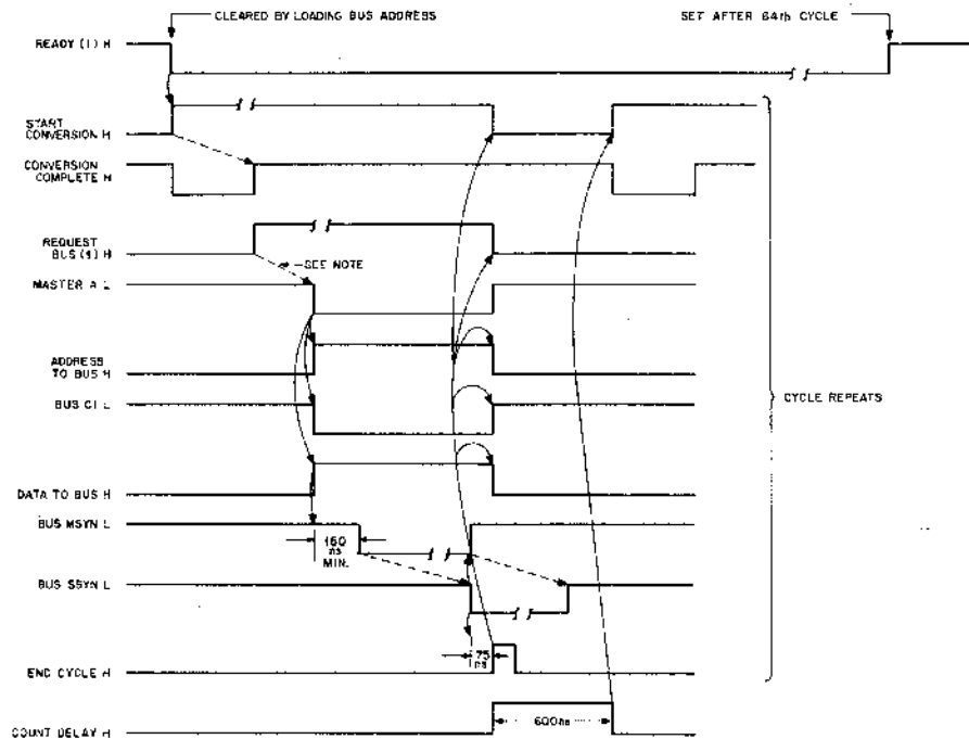
Figure 3-8 DMA Interface (timing diagram)
