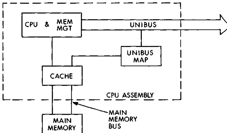
Figure 8-4 Overall Block Diagram PDP-11/44
