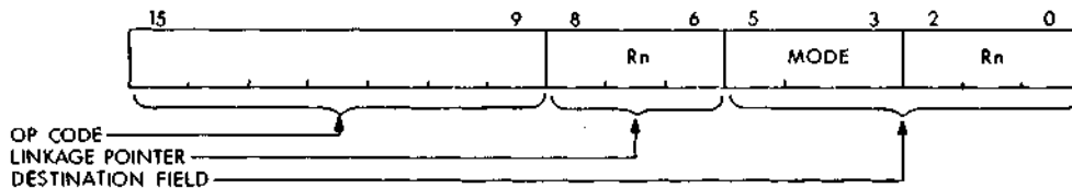
Figure 4-4 JSR Instruction Format
