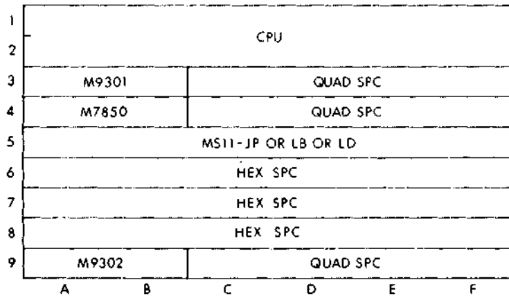
Figure 7-4 PDP-11/34A Backplane Configuration with MOS Memory
