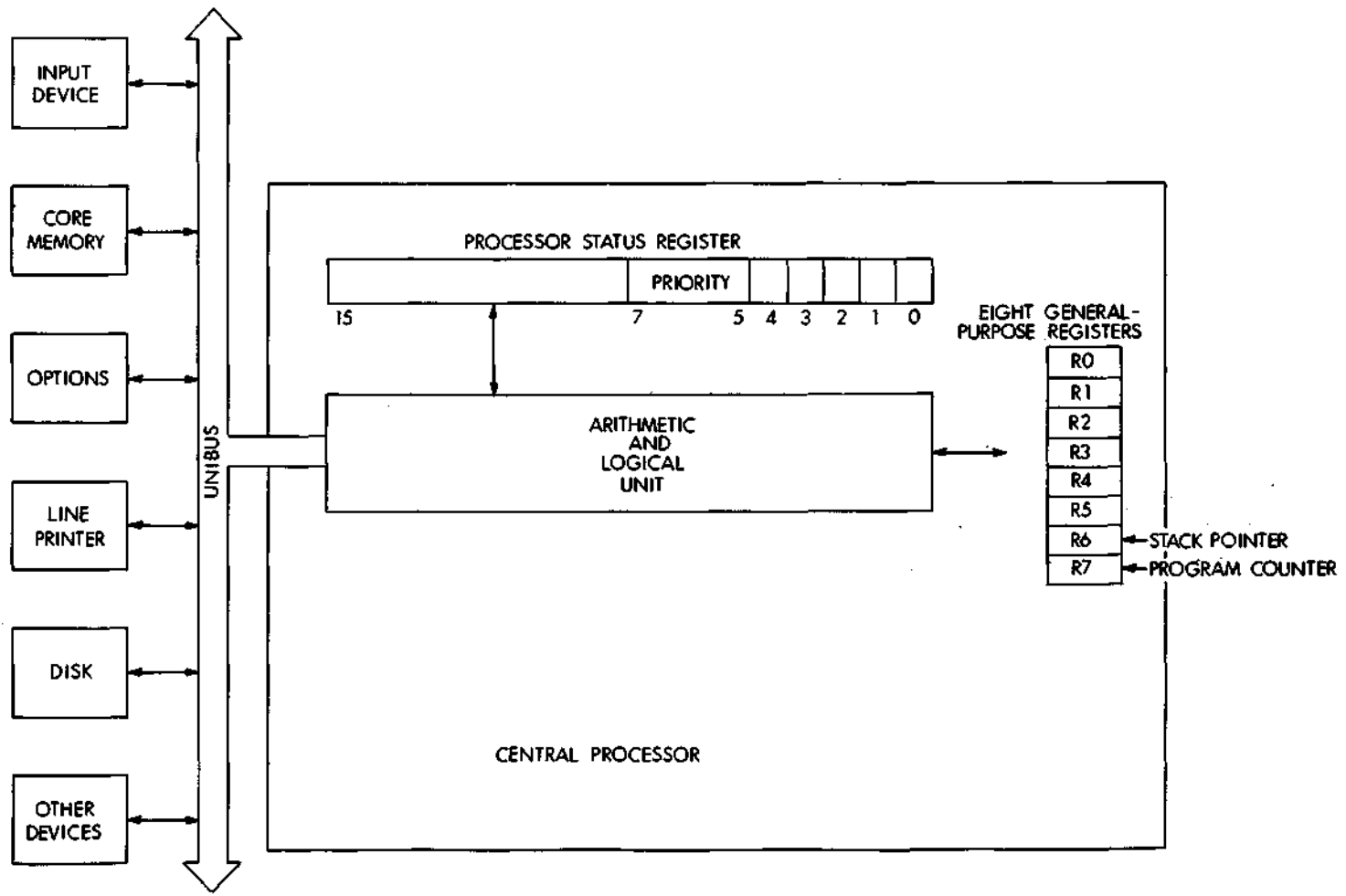
Figure 1-2 PDP-11 Block Structure
