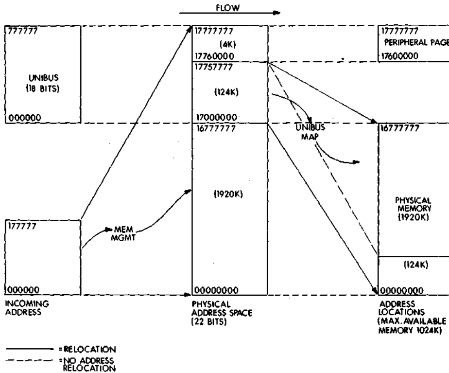
Figure 6-5 22-Bit Mapping on 11/44, 11/70
