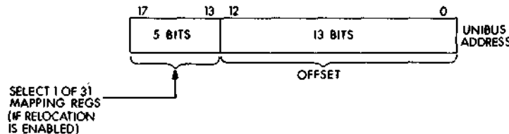
Figure 6-21 18-bit UNIBUS Address
