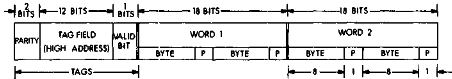
Figure 10-11 Block of Data plus Tags
