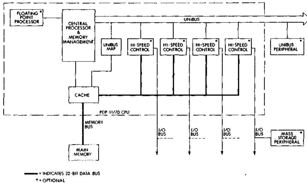
Figure 10-1 PDP-11/70 Block Diagram
