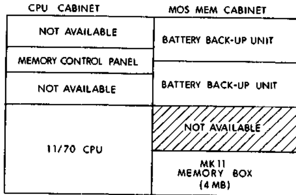
Figure 10-7 11/70 Equipment in H960 Cabinets
