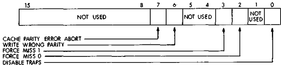
Figure 9-7 Cache Control Register 777746
