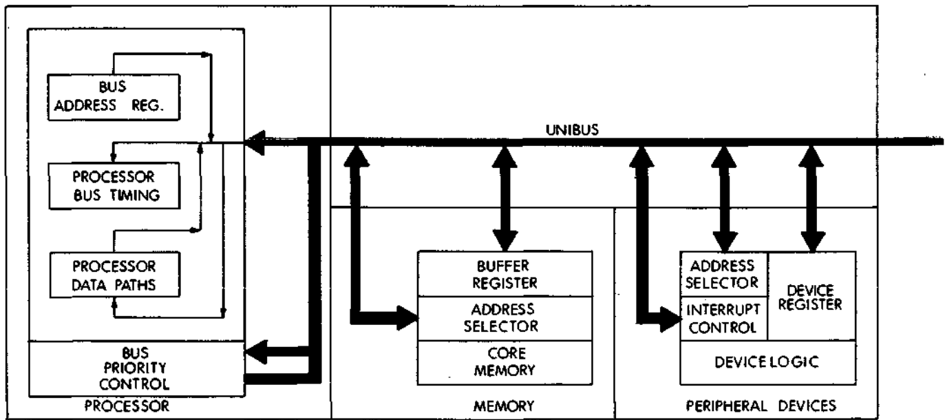
Figure 2-1 UNIBUS
