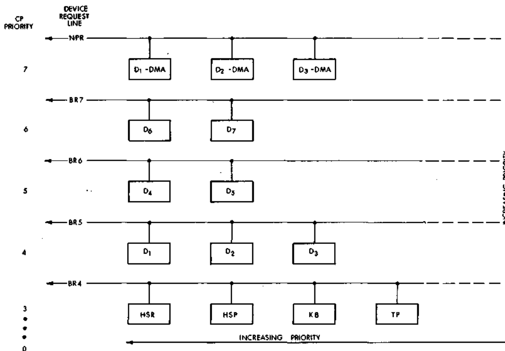
Figure 2-2 Priority Control
