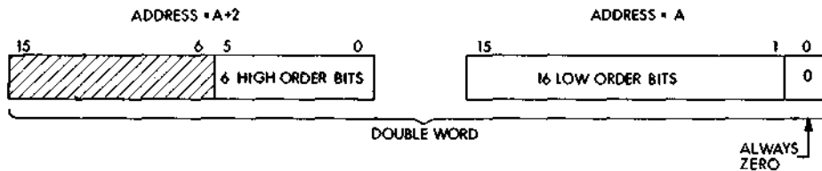
Figure 6-20 Single Mapping Register (1 or 31)
