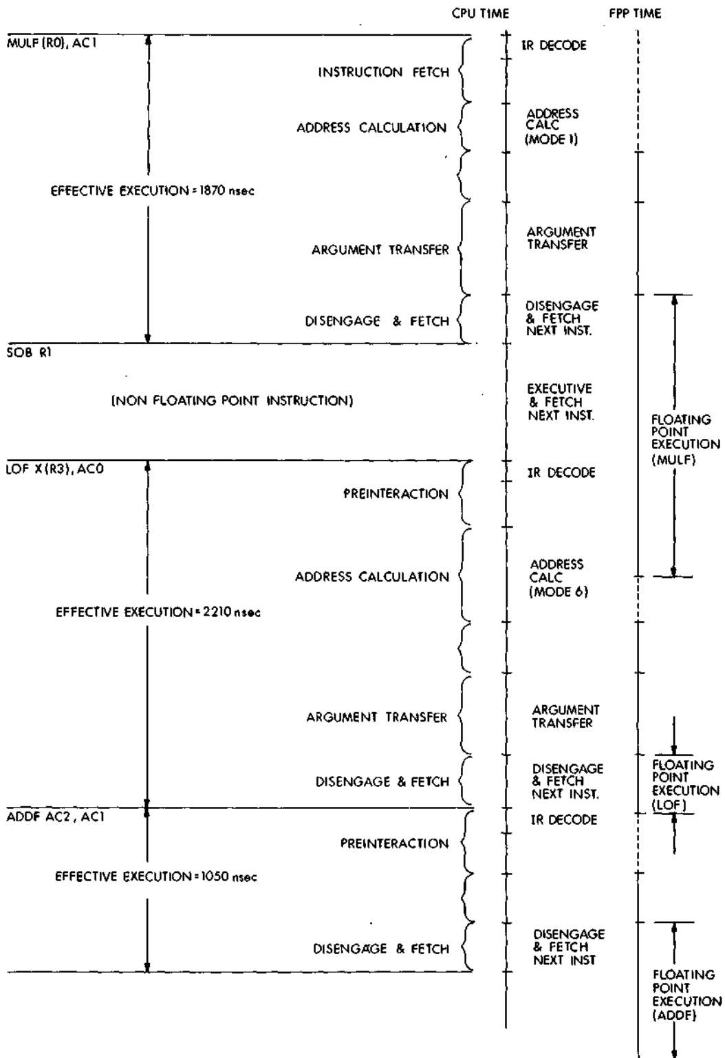
Calculation of Effective Execution Times for Load Class Instructions (FP11-E)
