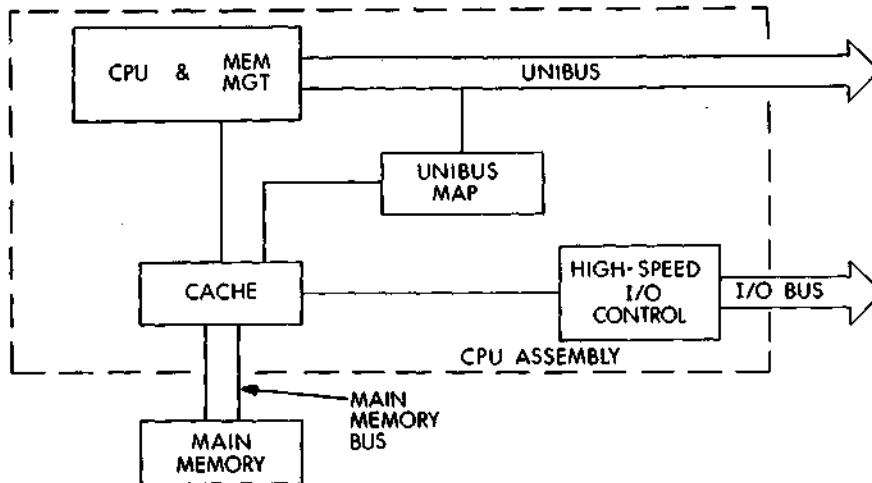
Figure 10-9 Block Diagram of PDP-11/70
