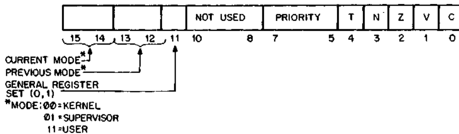
Figure 10-3 Processor Status Word
