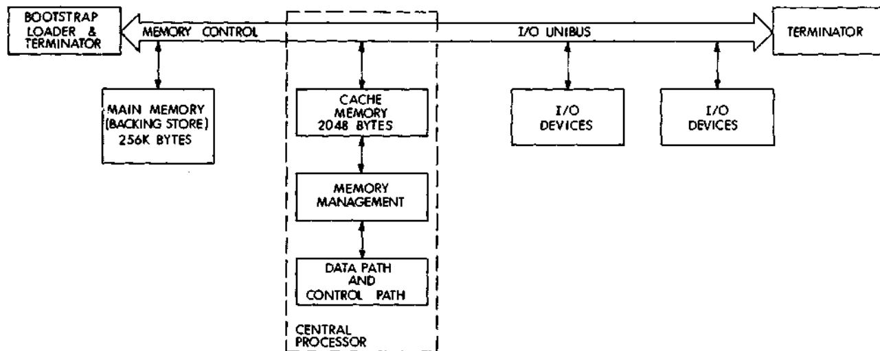
Figure 9-1 Simplified PDP-11/60 System
