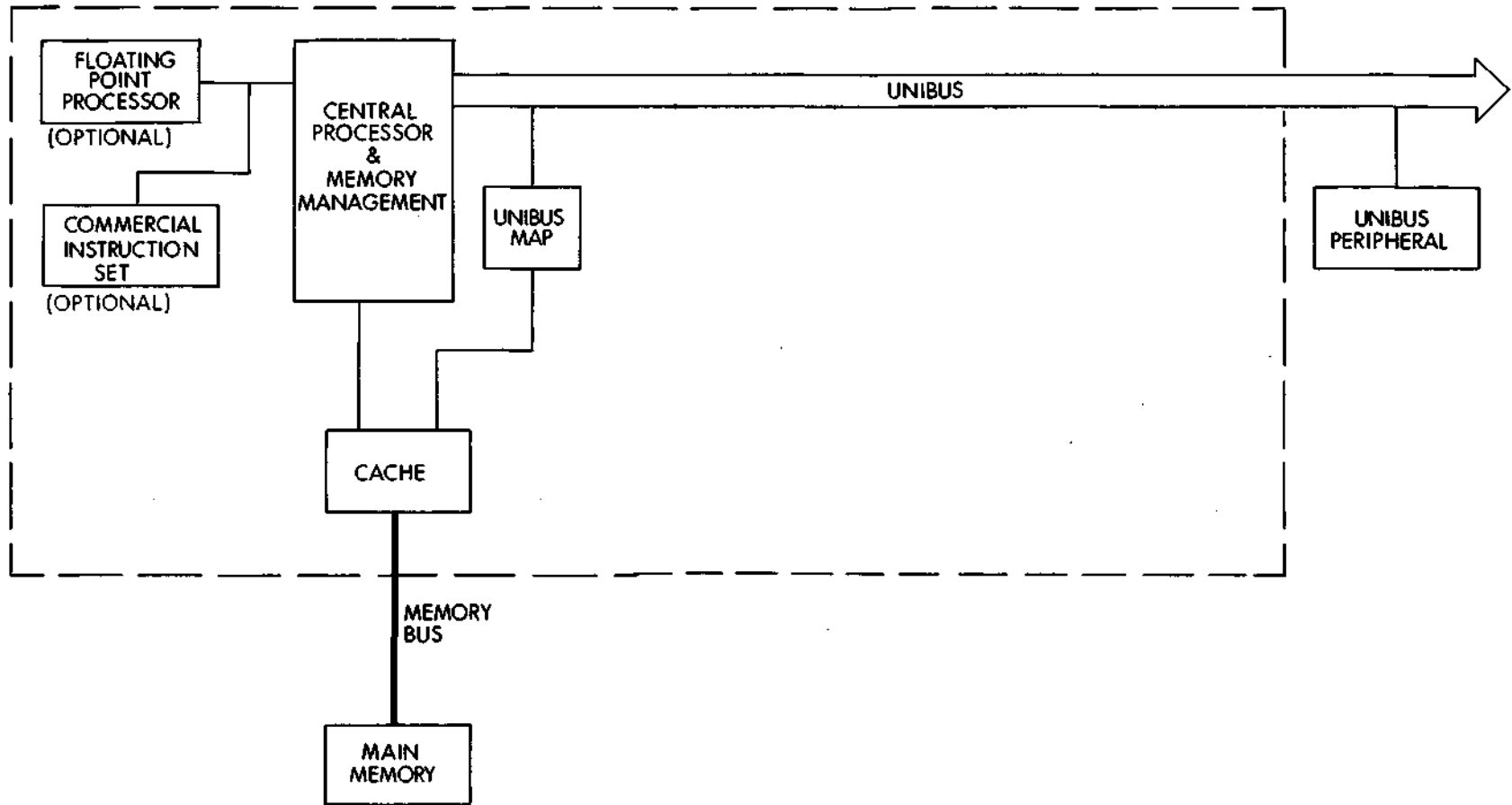
Figure 8-1 PDP-11/44 Block Diagram
