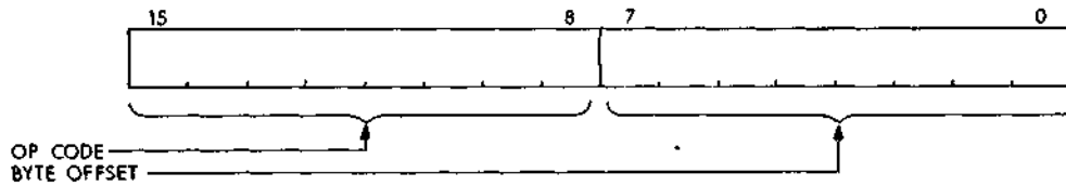
Figure 4-3 Branch Instruction Format
