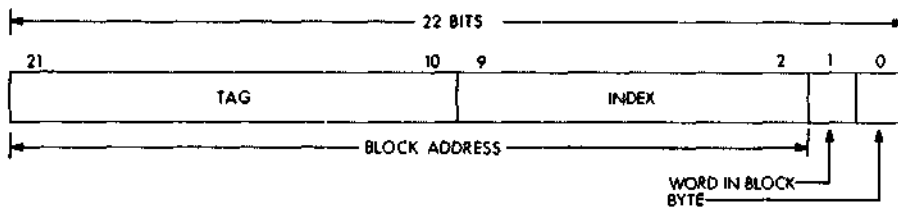
Figure 10-12 Physical Address
