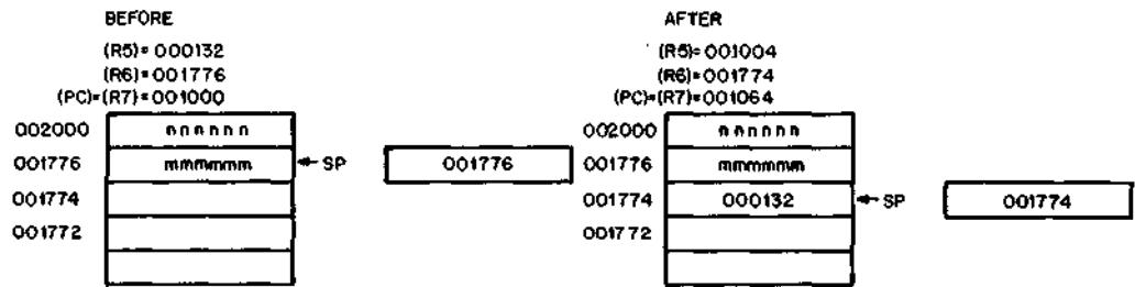
Figure 5-4 JSR
