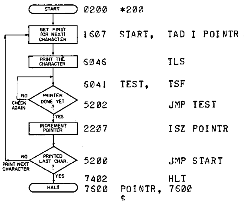
Figure 4-1 Program to Print ASCII Characters Using Programmed Data Transfer
