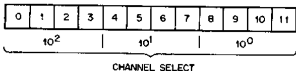
Figure 7-25 Control Word 2 (from Computer)
