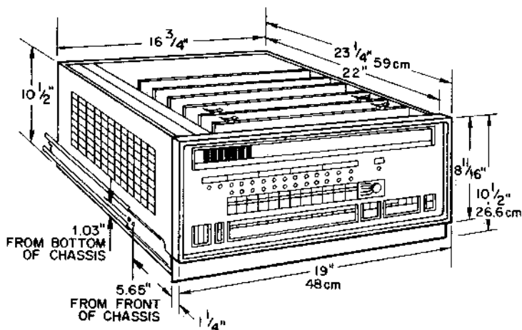
Figure 8-2. Rack-Mounted System Space Requirements
