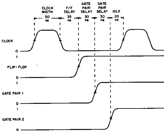
Figure 9-25 Delays Determining Total Operating Frequency Example
