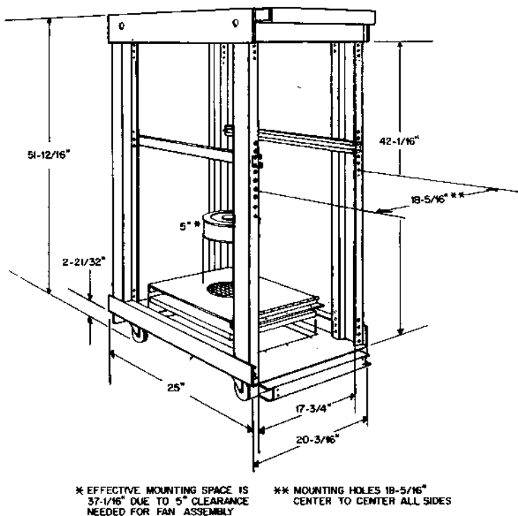
Figure 8-5. Short Basic Cabinet
