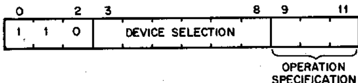
Figure 3-5. IOT Instruction Format
