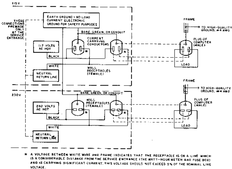
Figure 8-12. Recommended Receptacle Wiring
