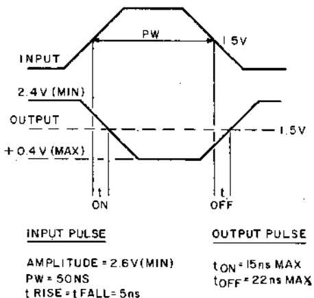
Figure 9-21 2 Input NAND Gate Typical Characteristics Example
