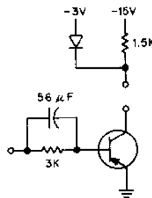
Figure 43 Inverter Circuit Schematic Diagram
