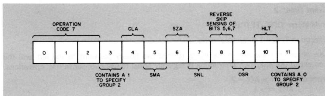
Figure 6 Group 1 Operate Instruction Bit Assignments
