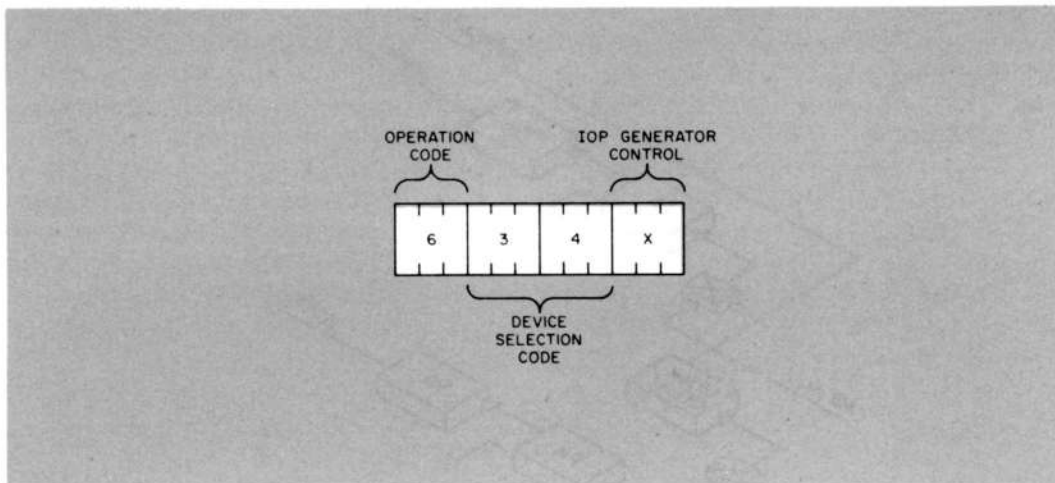
Figure 23 Typical IOT Instruction Decoding
