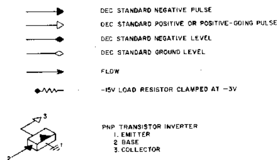
Figure 20 Logic Symbols
