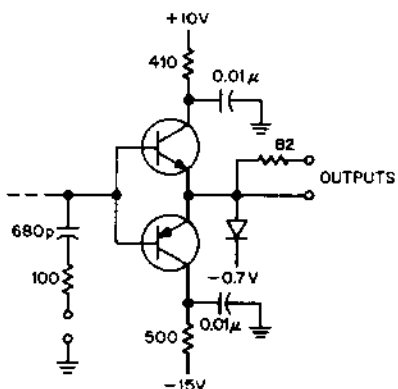
Figure 54 Bus Driver Output Circuit Schematic
