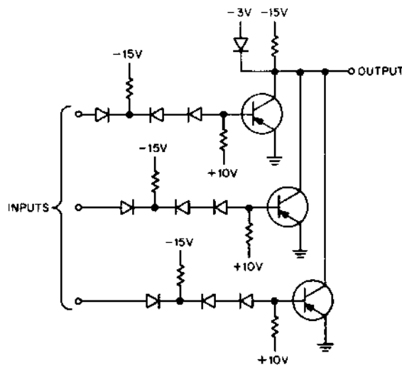
Figure 47 Parallel-Connected Diode Gate Circuit Schematic
