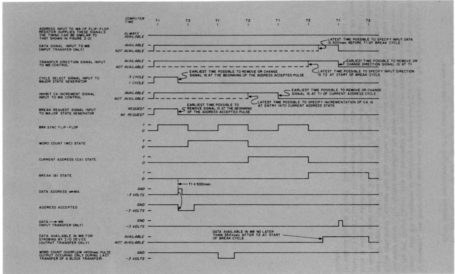
Figure 42 Three-Cycle Data Break Timing Diagram
