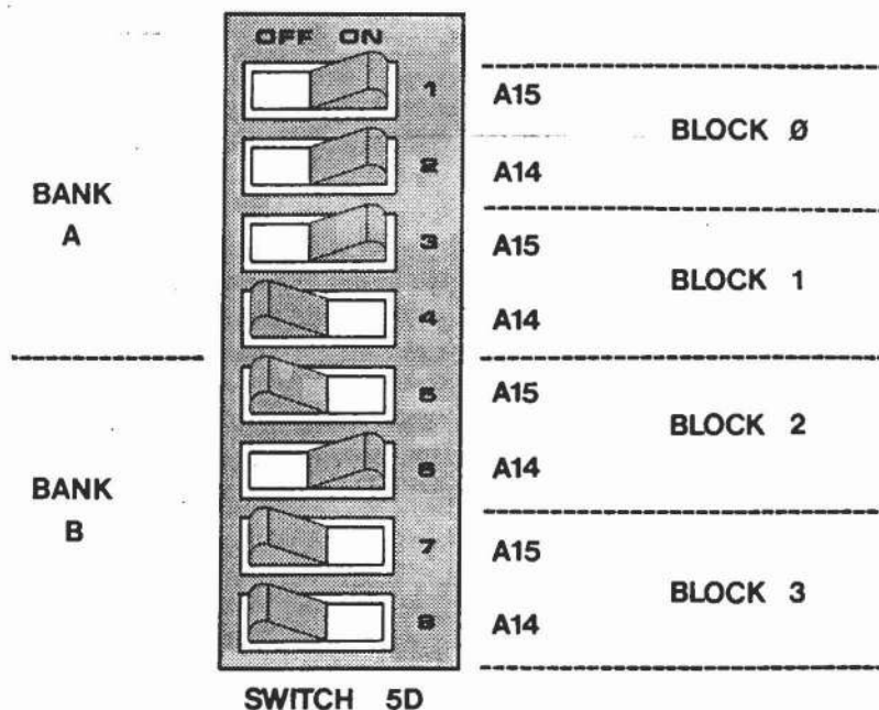
Figure 6-6: ASSIGNMENT OF INDIVIDUAL 16K BLOCKS OF MEMORY
