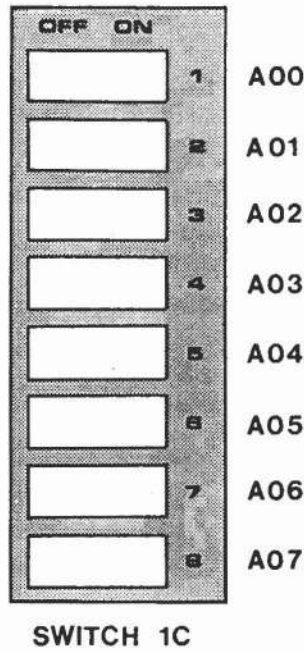
Figure 6-12: DIP SWITCH 1C USED WITH BANK SELECT
