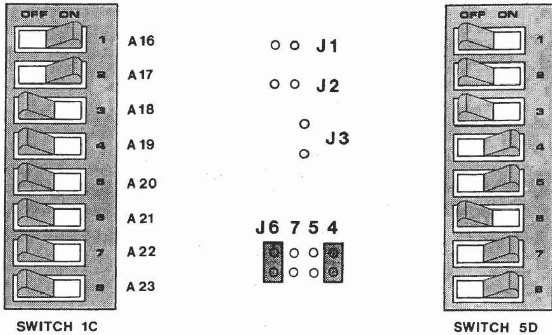
Figure 6-11: EXAMPLE OF EXTENDED ADDRESSING @ 030000H – 03FFFFH
